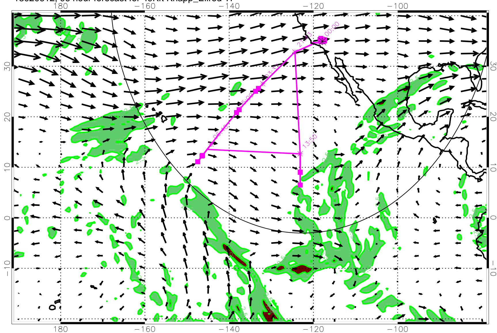
13020612, 96 hour forecast for 49Kft Knapp_Ellrod TI
