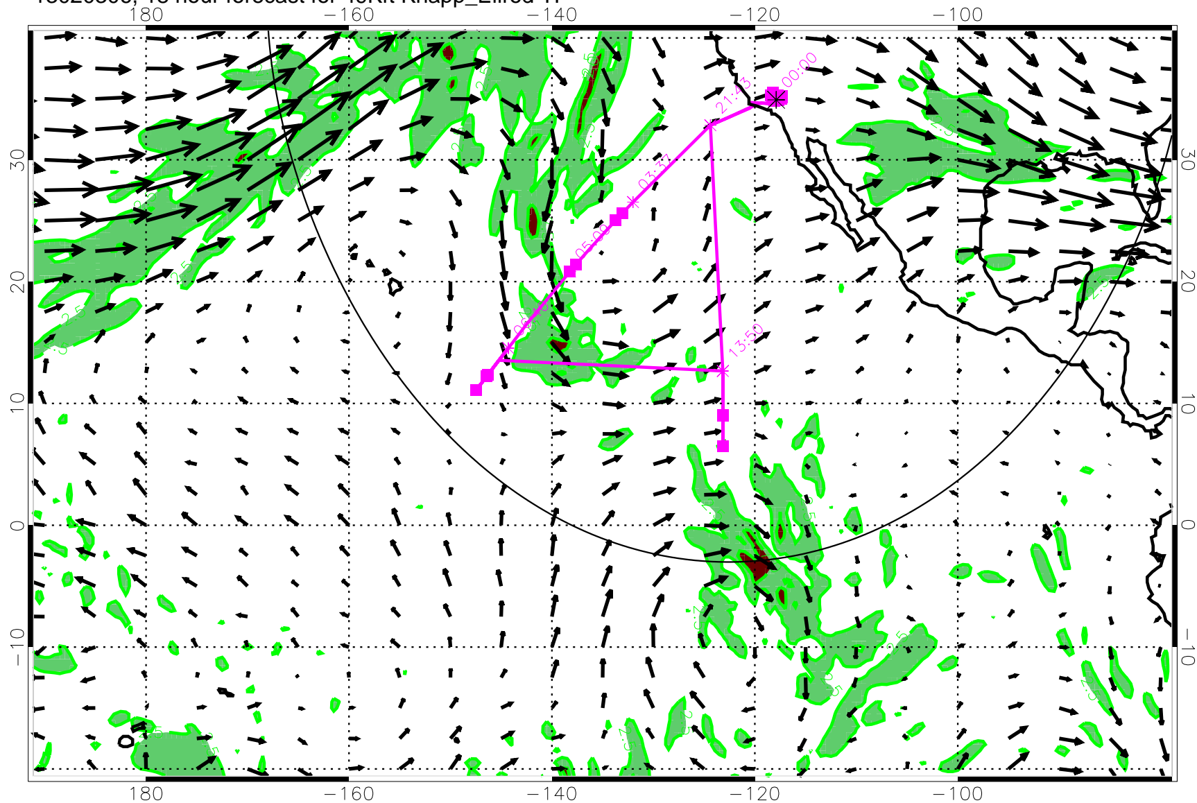
13020306, 18 hour forecast for 49Kft Knapp_Ellrod TI
