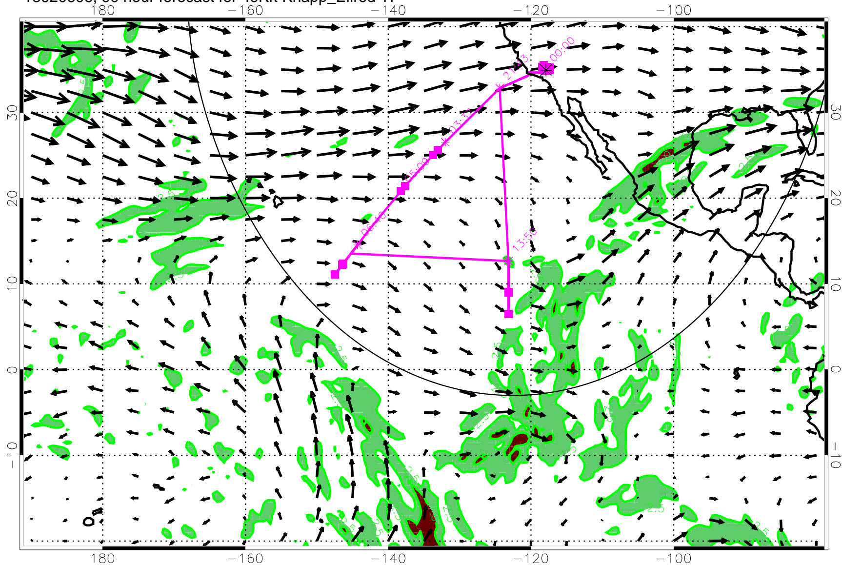
13020606, 90 hour forecast for 49Kft Knapp_Ellrod TI
