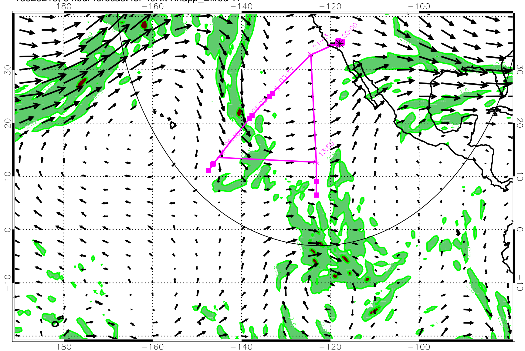
13020218, 6 hour forecast for 49Kft Knapp_Ellrod TI
