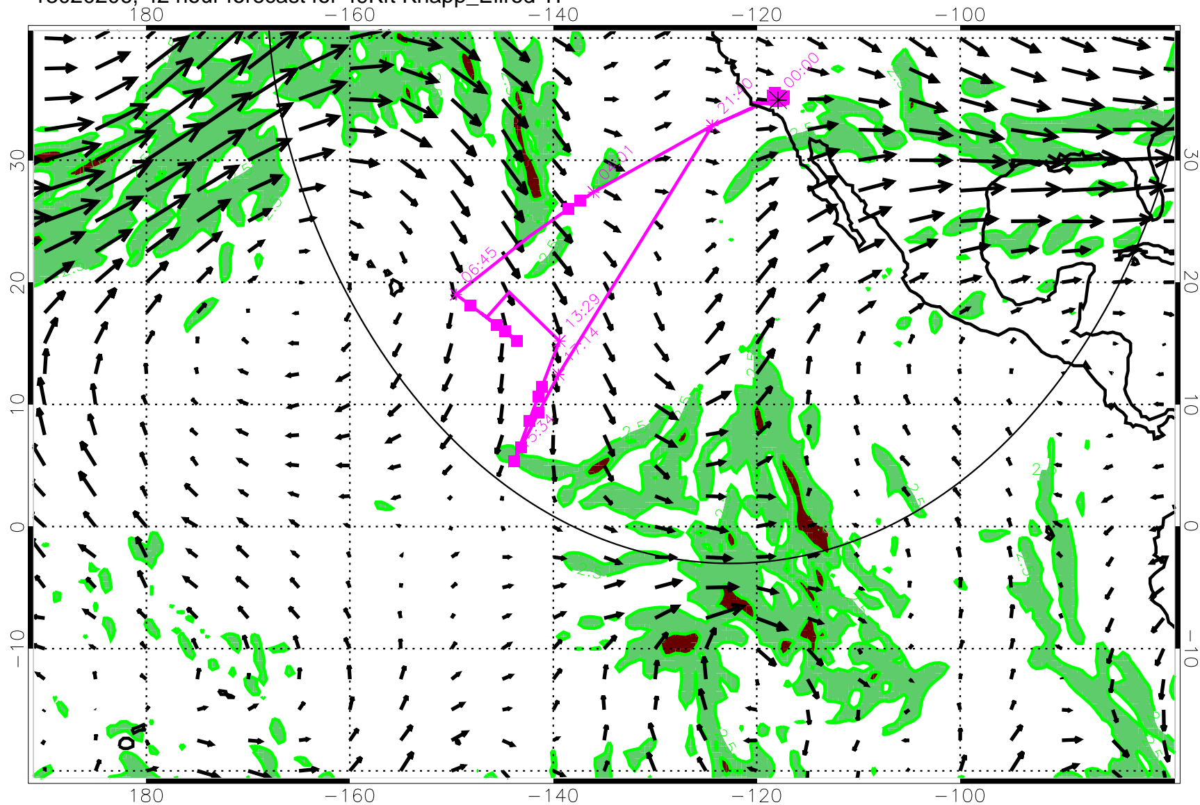
13020206, 42 hour forecast for 49Kft Knapp_Ellrod TI
