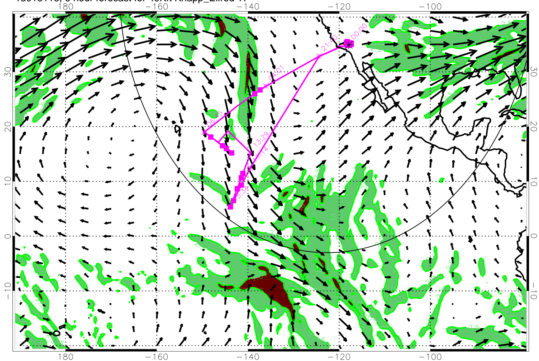
13013118, 6 hour forecast for 49Kft Knapp_Ellrod TI
