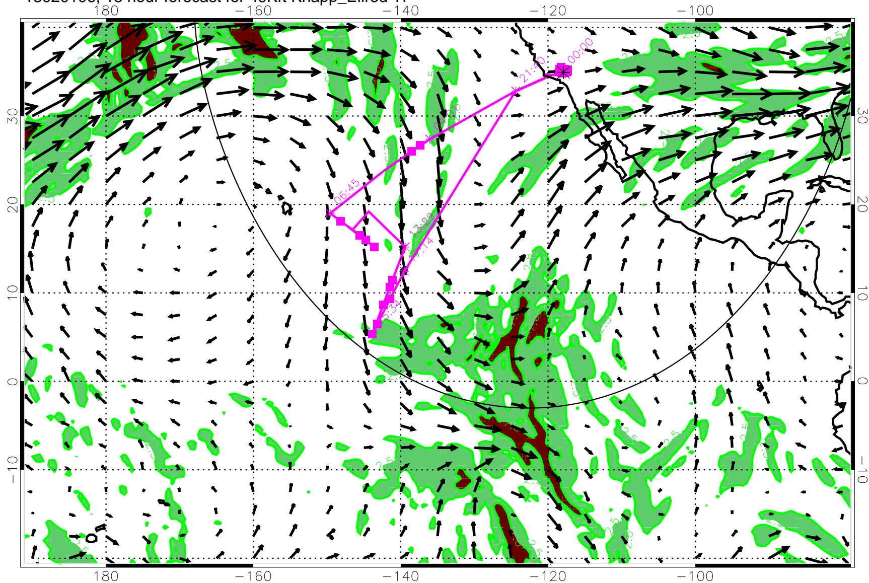
13020106, 18 hour forecast for 49Kft Knapp_Ellrod TI
