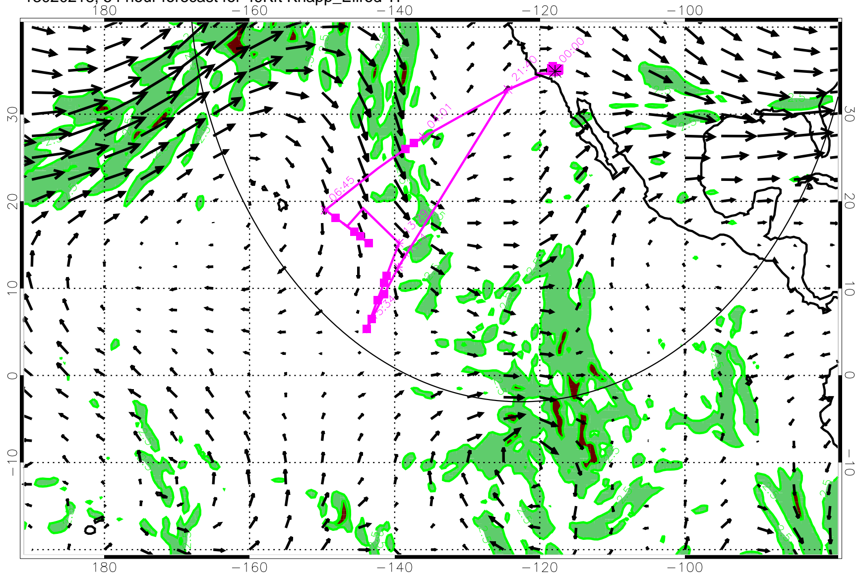
13020218, 54 hour forecast for 49Kft Knapp_Ellrod TI
