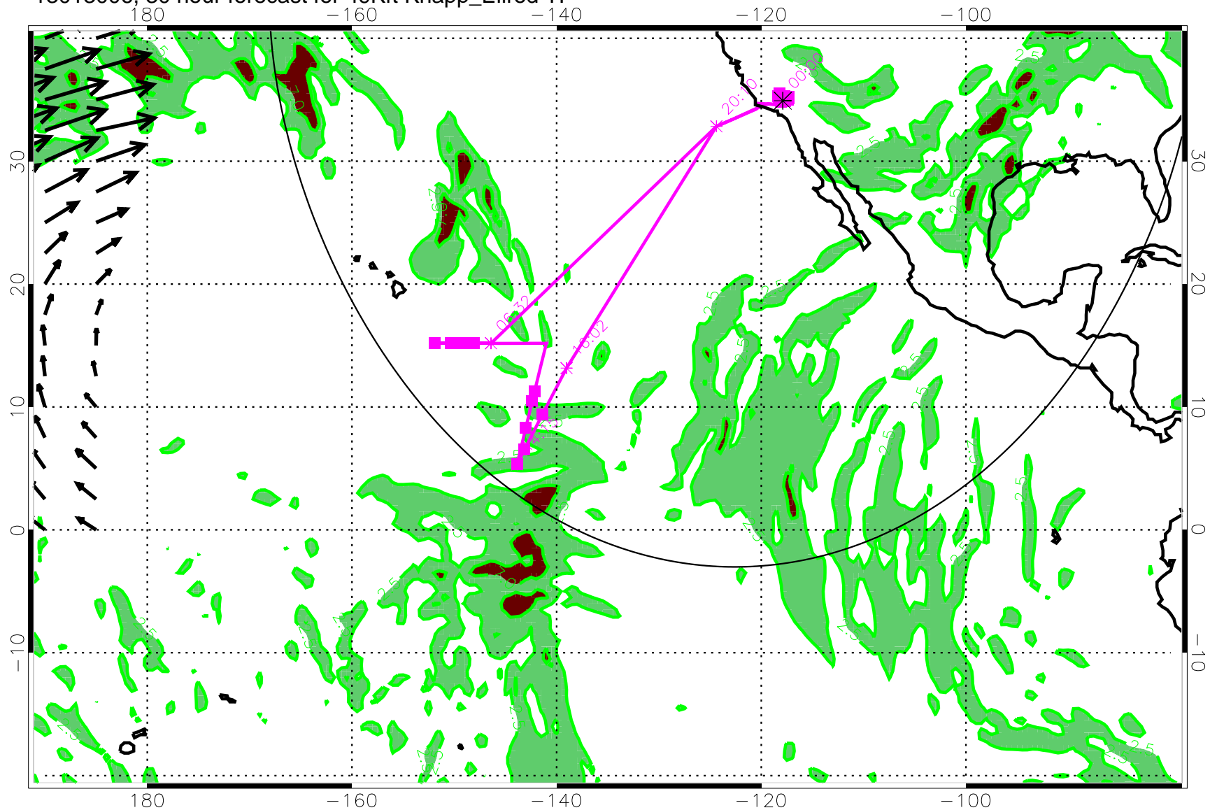
13013006, 30 hour forecast for 49Kft Knapp_Ellrod TI
