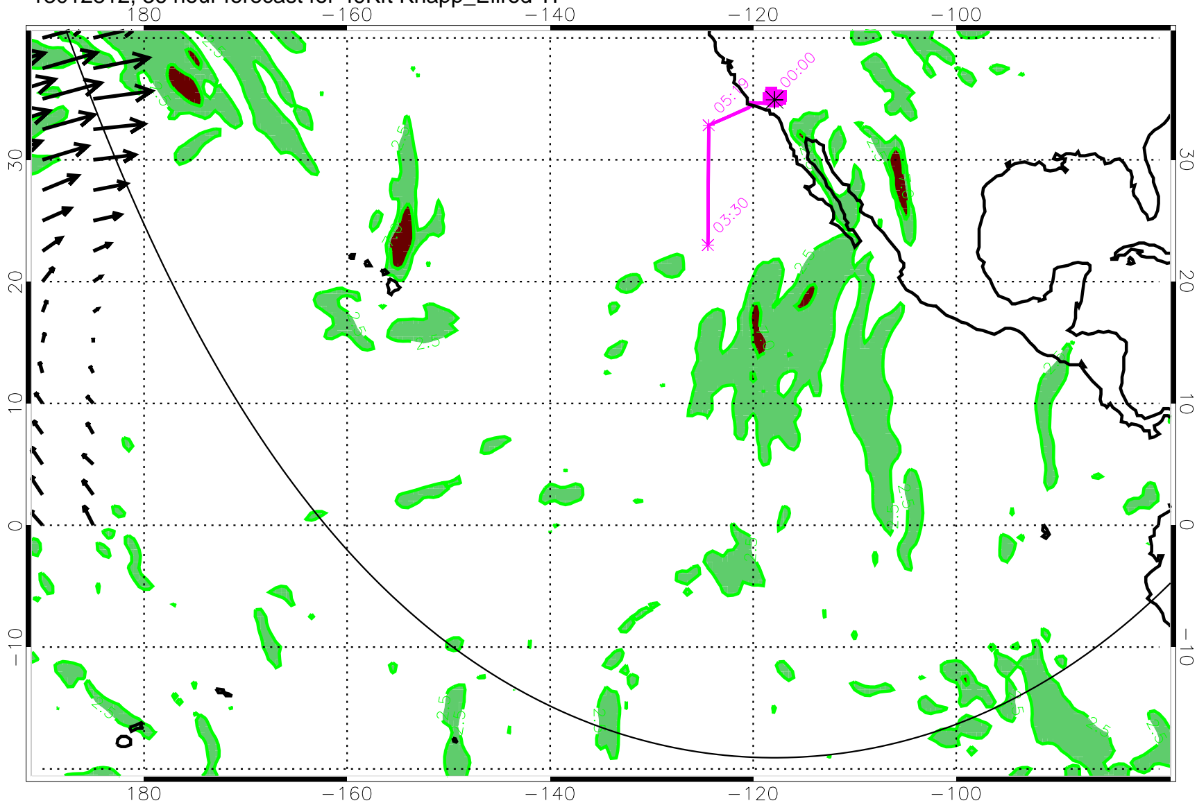
13012812, 36 hour forecast for 49Kft Knapp_Ellrod TI
