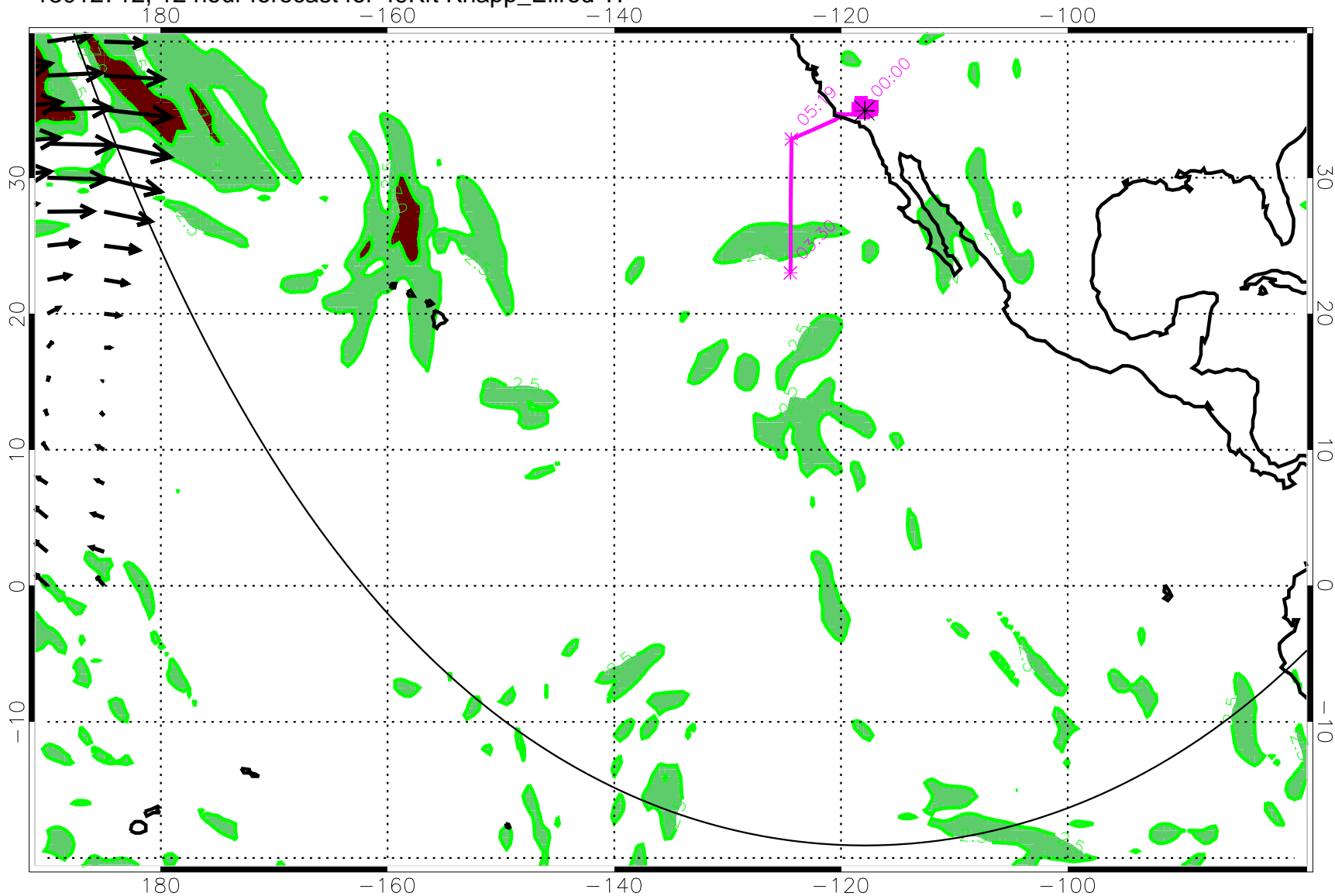
13012712, 12 hour forecast for 49Kft Knapp_Ellrod TI
