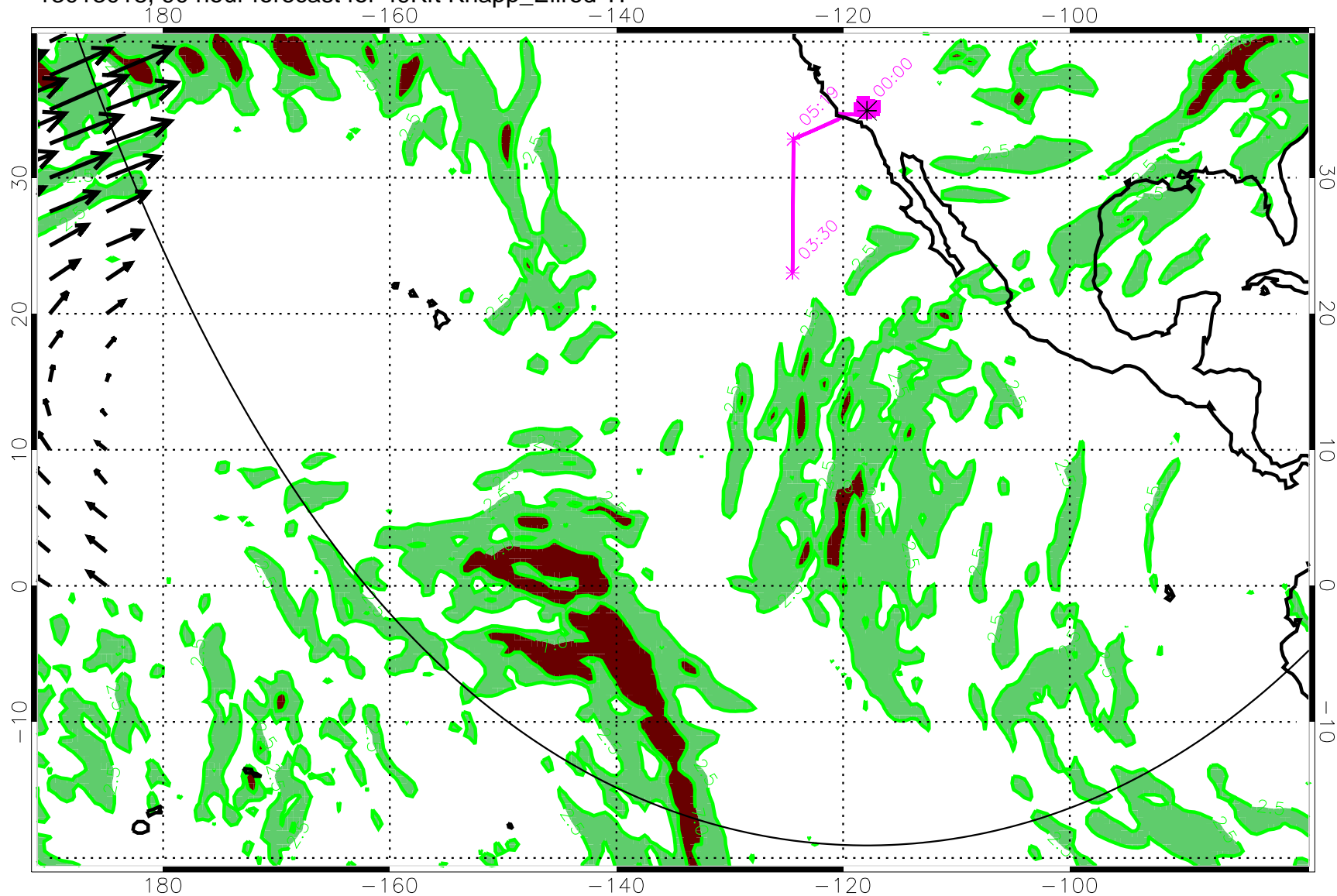
13013018, 90 hour forecast for 49Kft Knapp_Ellrod TI
