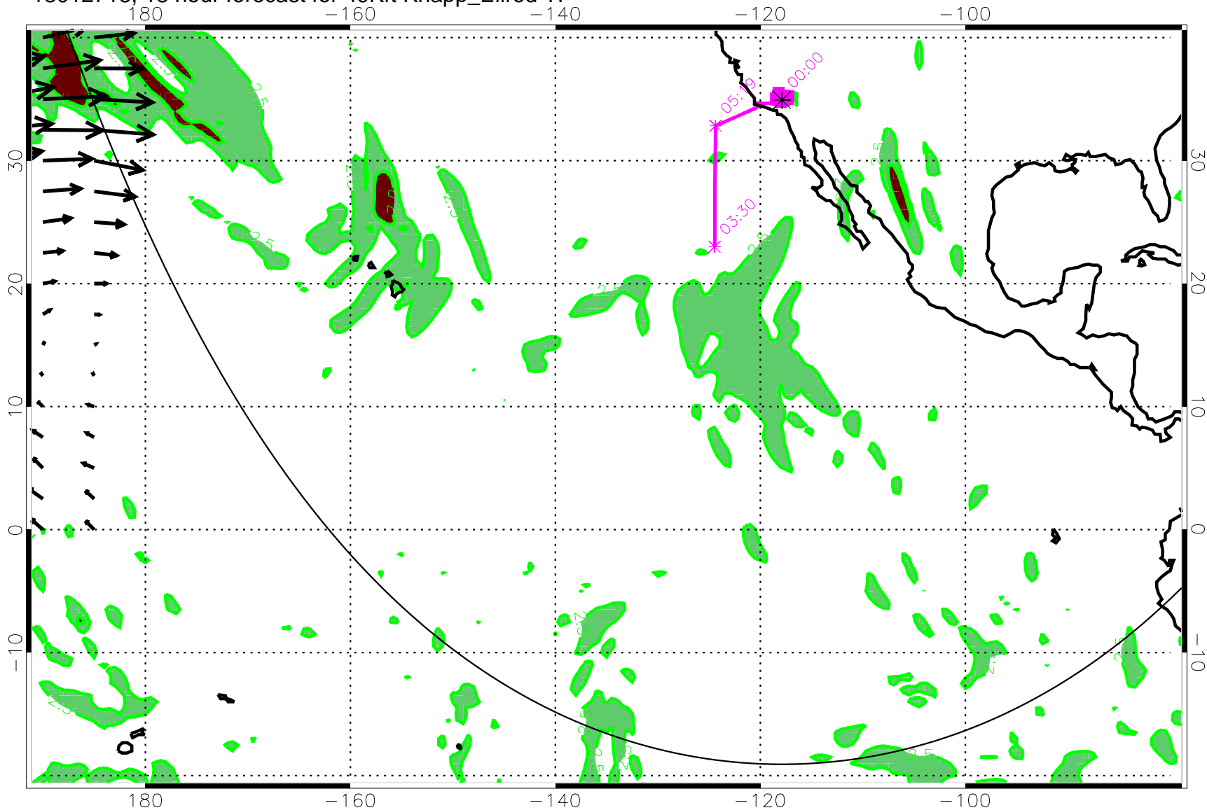
13012718, 18 hour forecast for 49Kft Knapp_Ellrod TI
