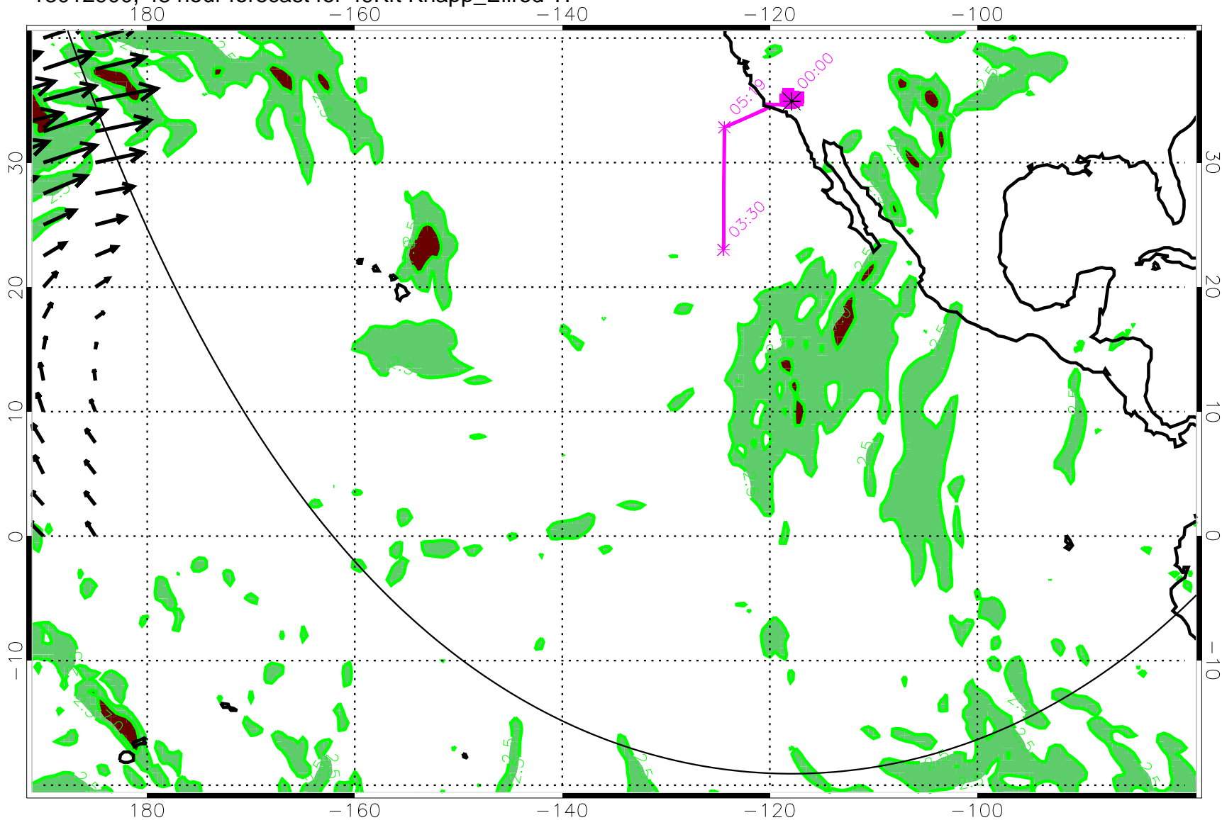
13012900, 48 hour forecast for 49Kft Knapp_Ellrod TI
