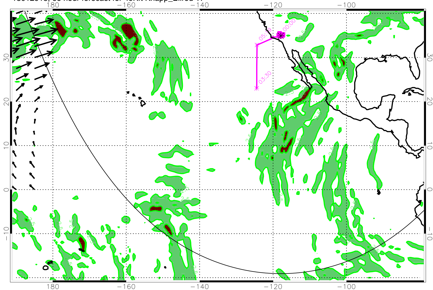
13012918, 66 hour forecast for 49Kft Knapp_Ellrod TI
