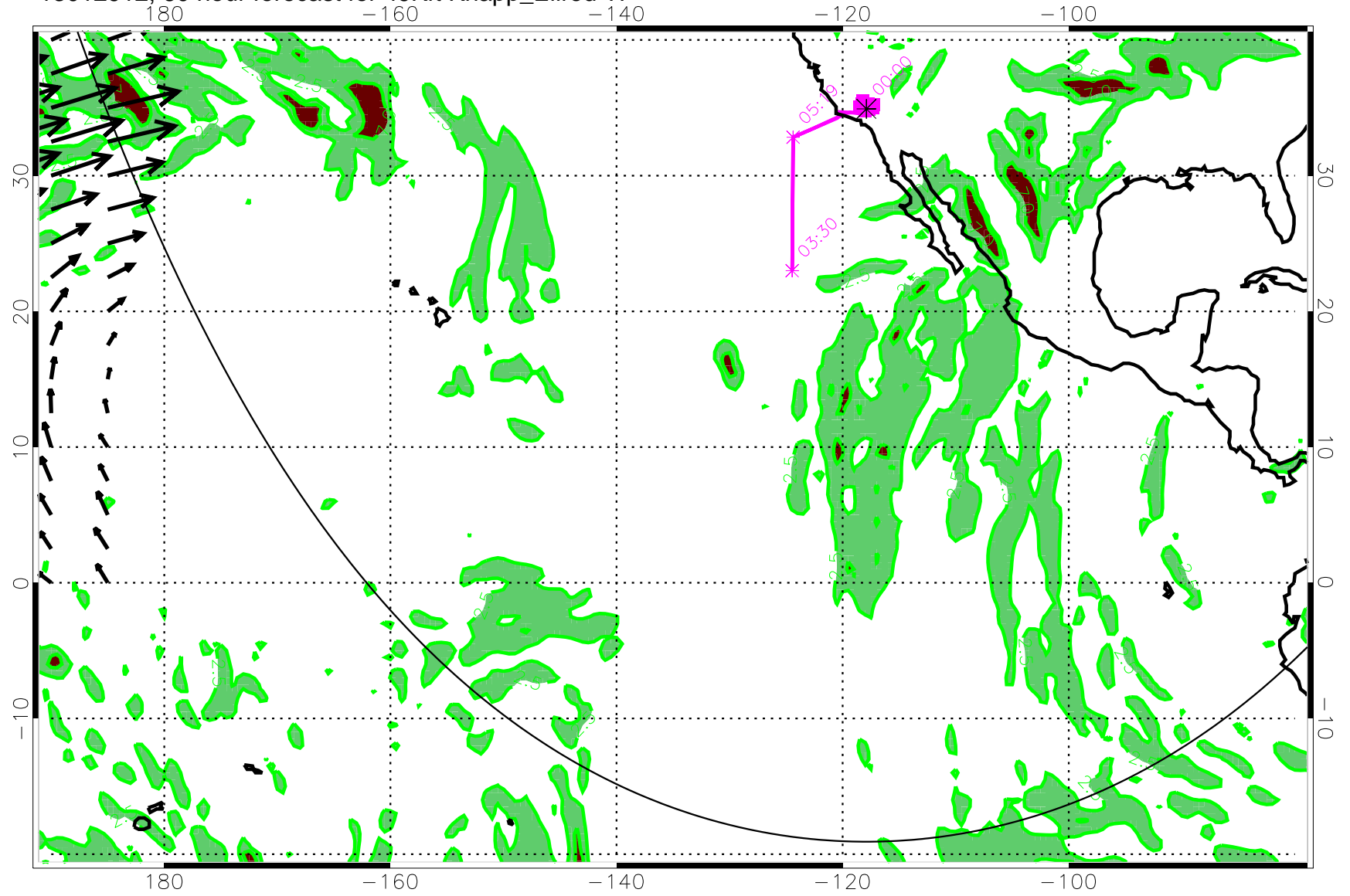
13012912, 60 hour forecast for 49Kft Knapp_Ellrod TI
