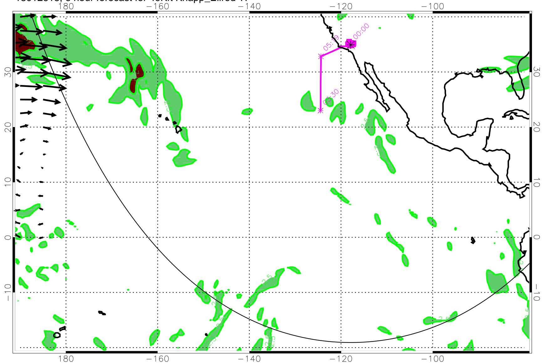
13012618, 6 hour forecast for 49Kft Knapp_Ellrod TI
