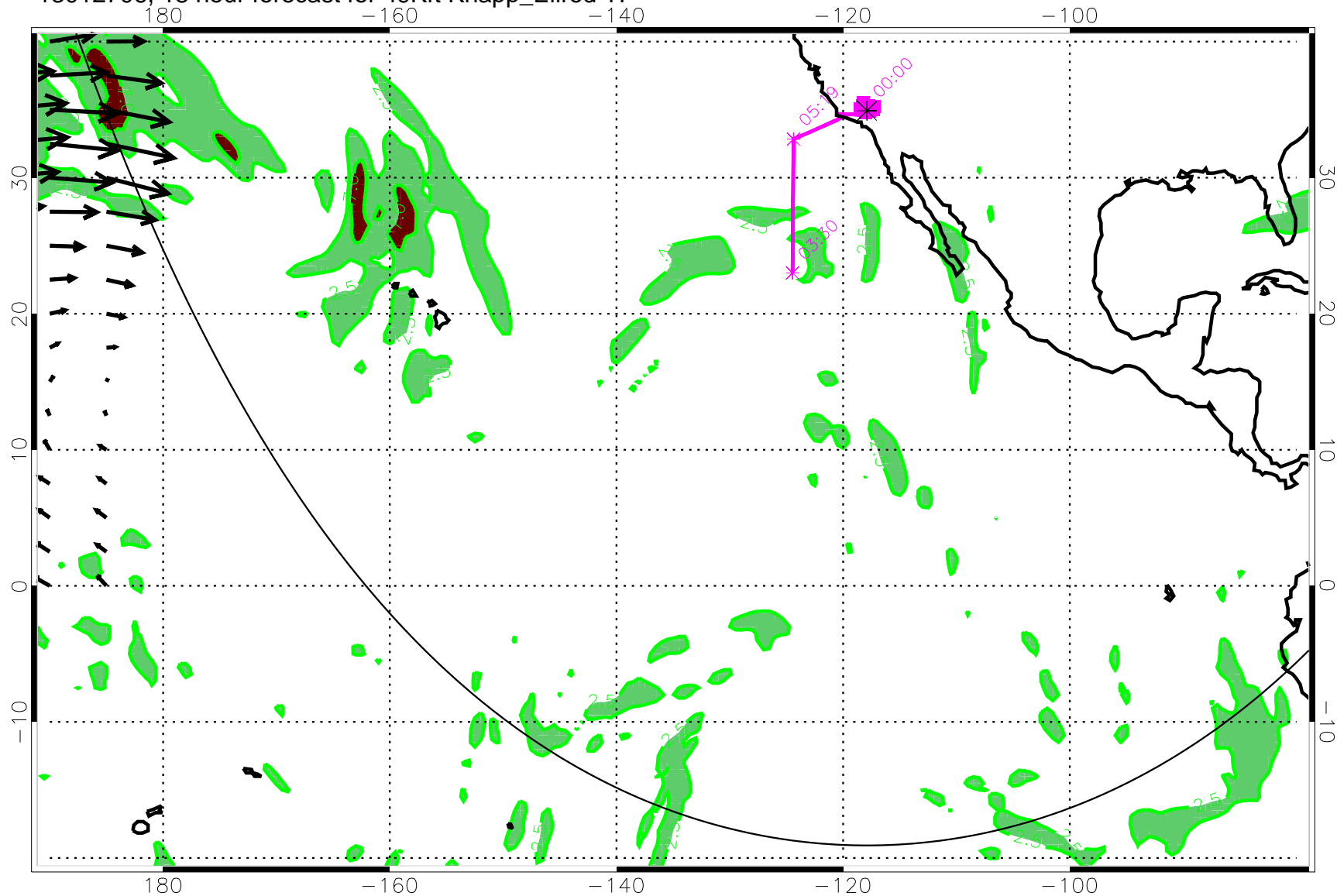
13012706, 18 hour forecast for 49Kft Knapp_Ellrod TI
