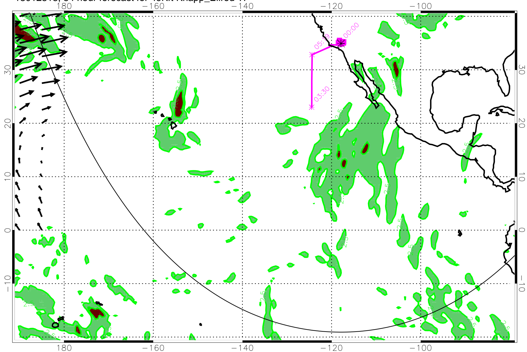
13012818, 54 hour forecast for 49Kft Knapp_Ellrod TI
