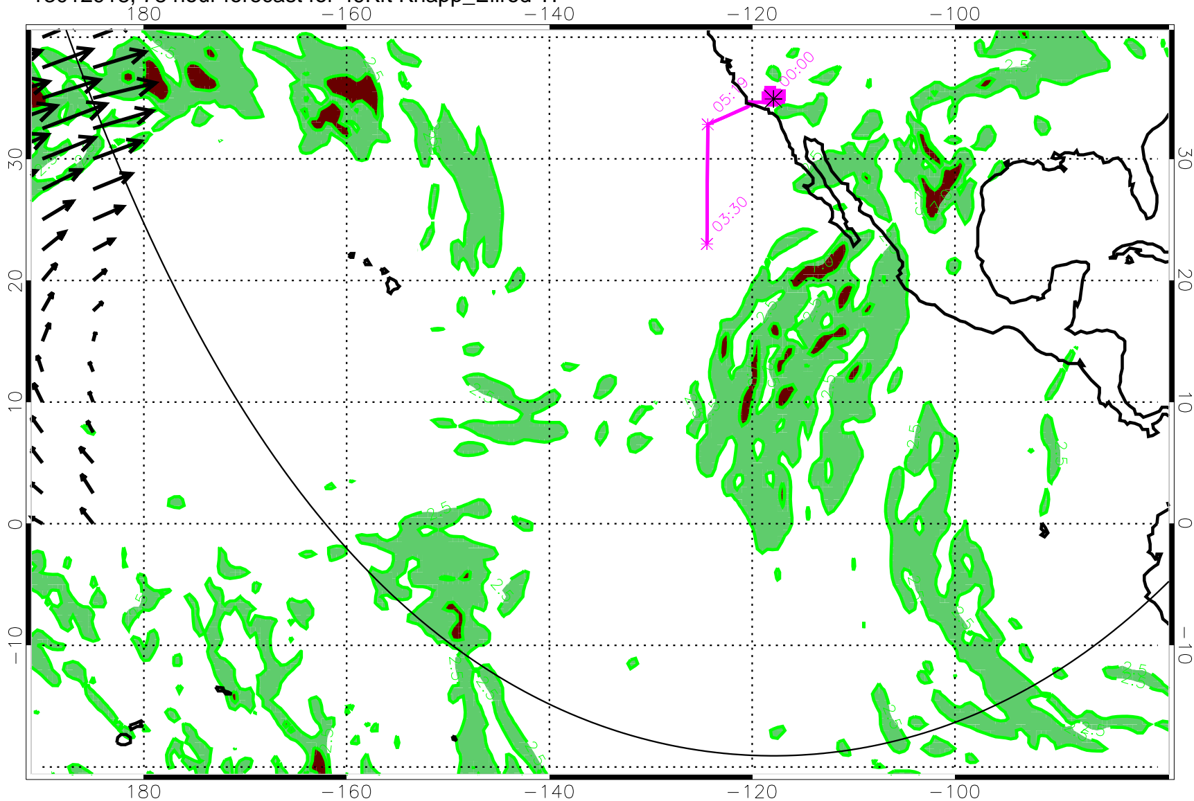
13012918, 78 hour forecast for 49Kft Knapp_Ellrod TI
