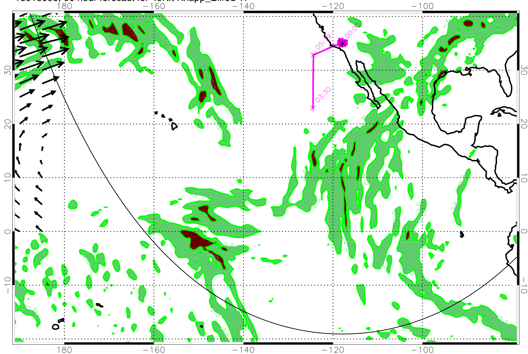
13013006, 90 hour forecast for 49Kft Knapp_Ellrod TI
