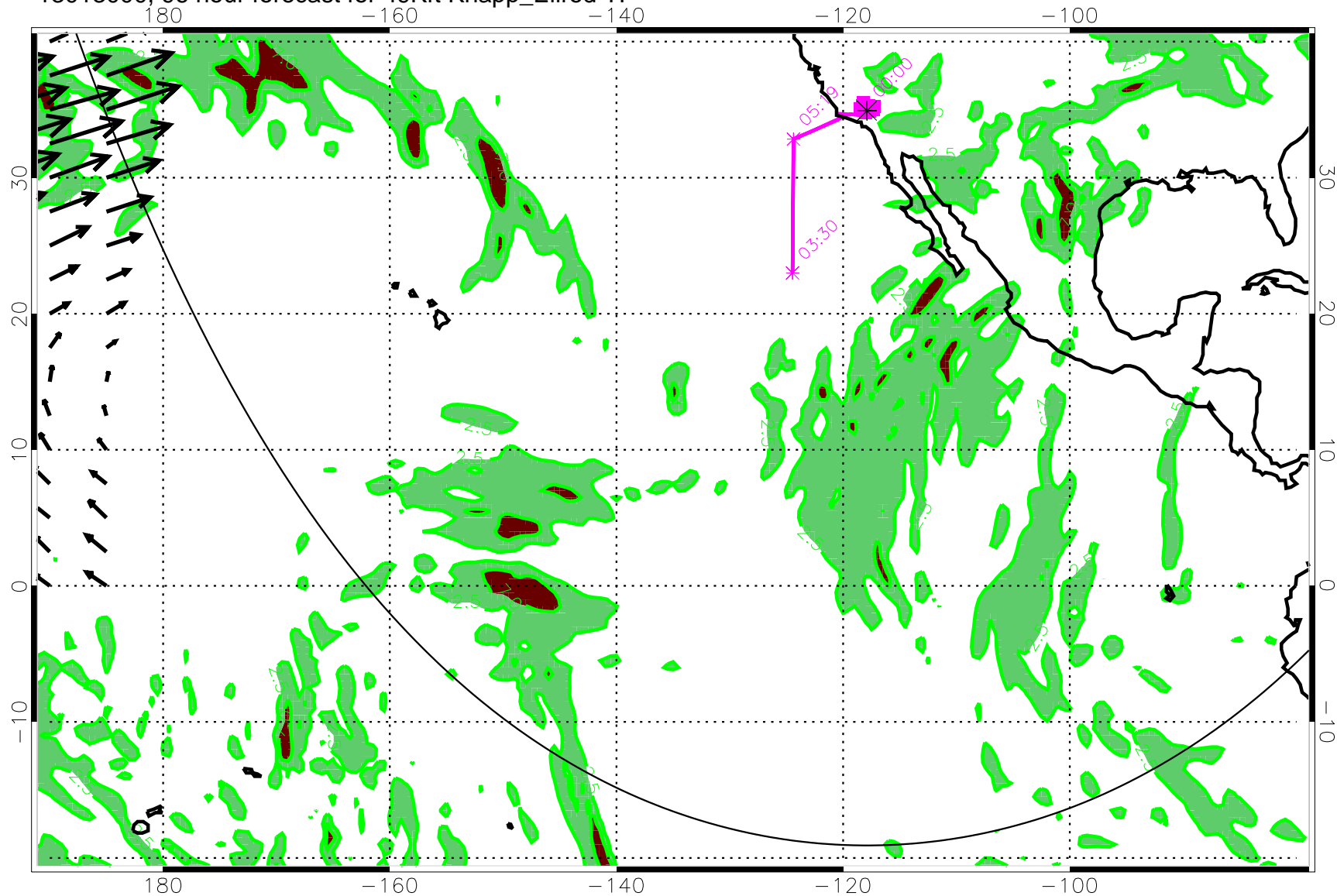
13013000, 96 hour forecast for 49Kft Knapp_Ellrod TI
