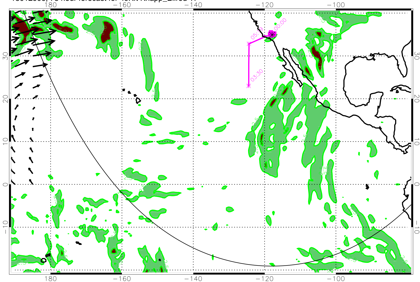
13012906, 78 hour forecast for 49Kft Knapp_Ellrod TI
