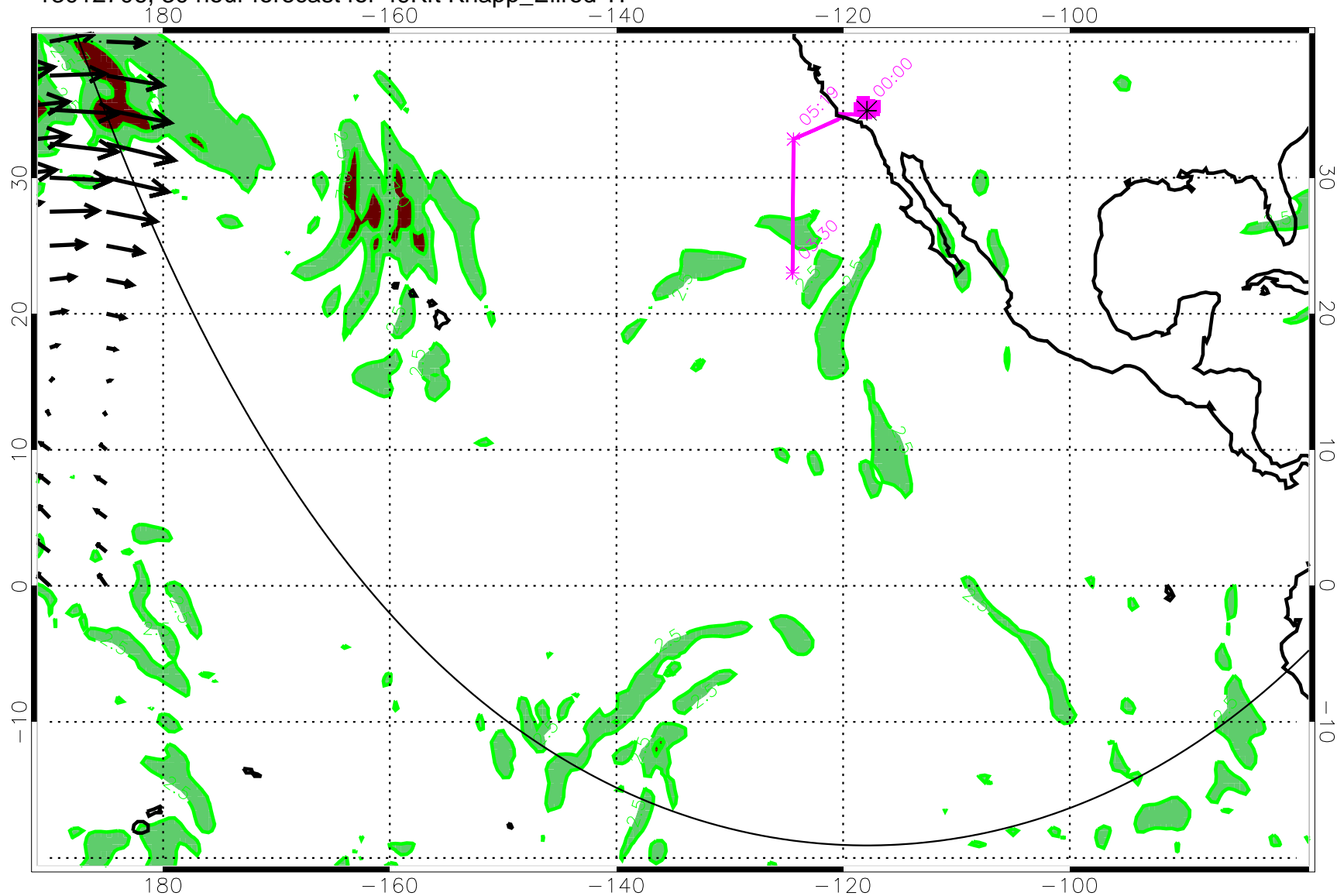
13012706, 30 hour forecast for 49Kft Knapp_Ellrod TI
