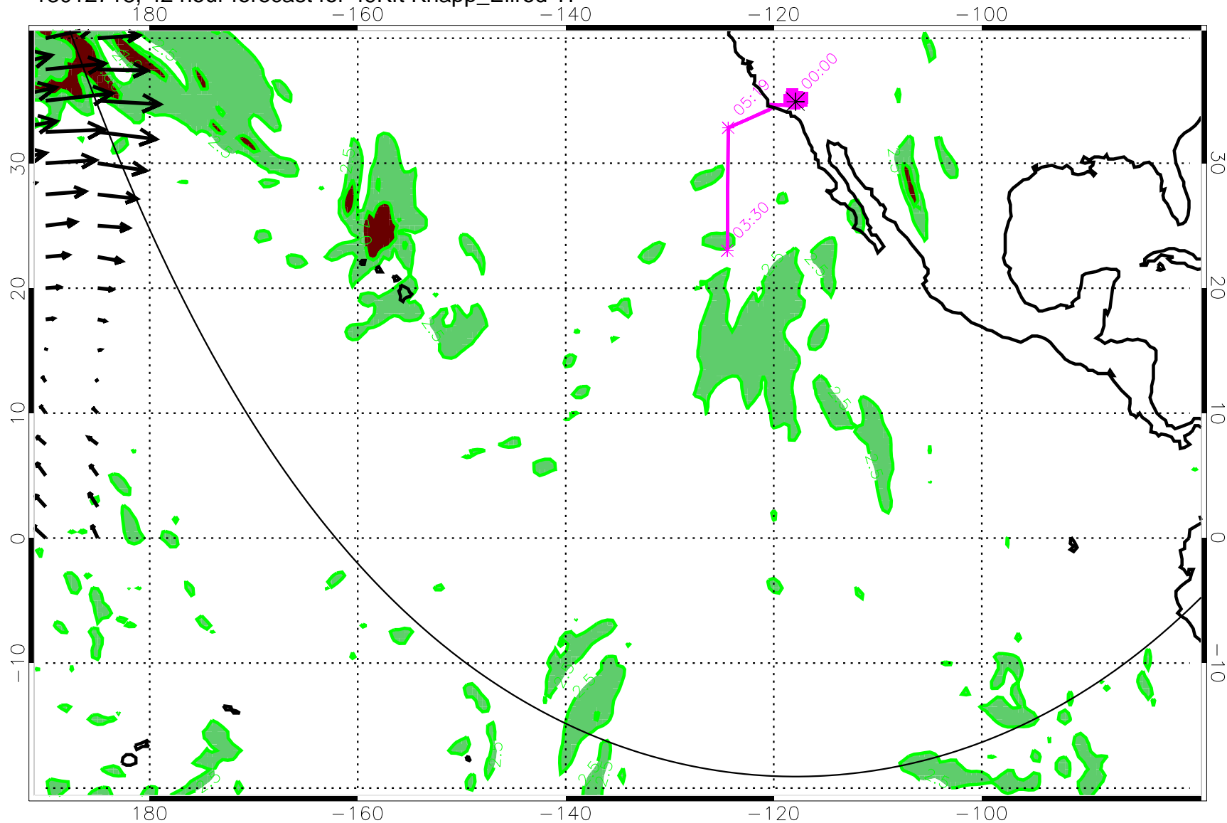
13012718, 42 hour forecast for 49Kft Knapp_Ellrod TI
