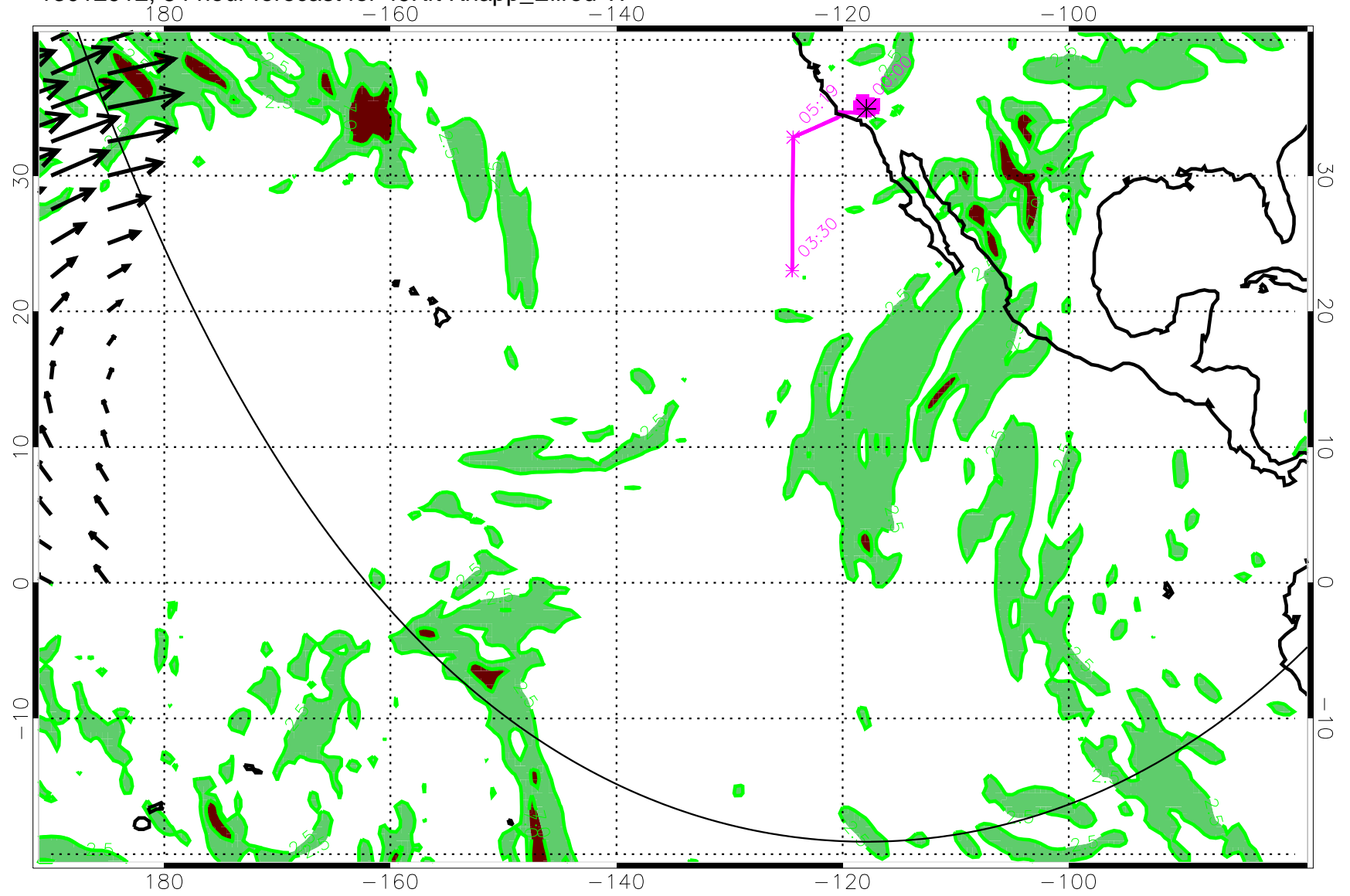
13012912, 84 hour forecast for 49Kft Knapp_Ellrod TI
