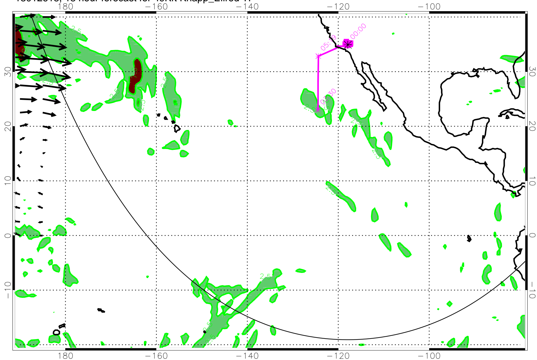
13012618, 18 hour forecast for 49Kft Knapp_Ellrod TI
