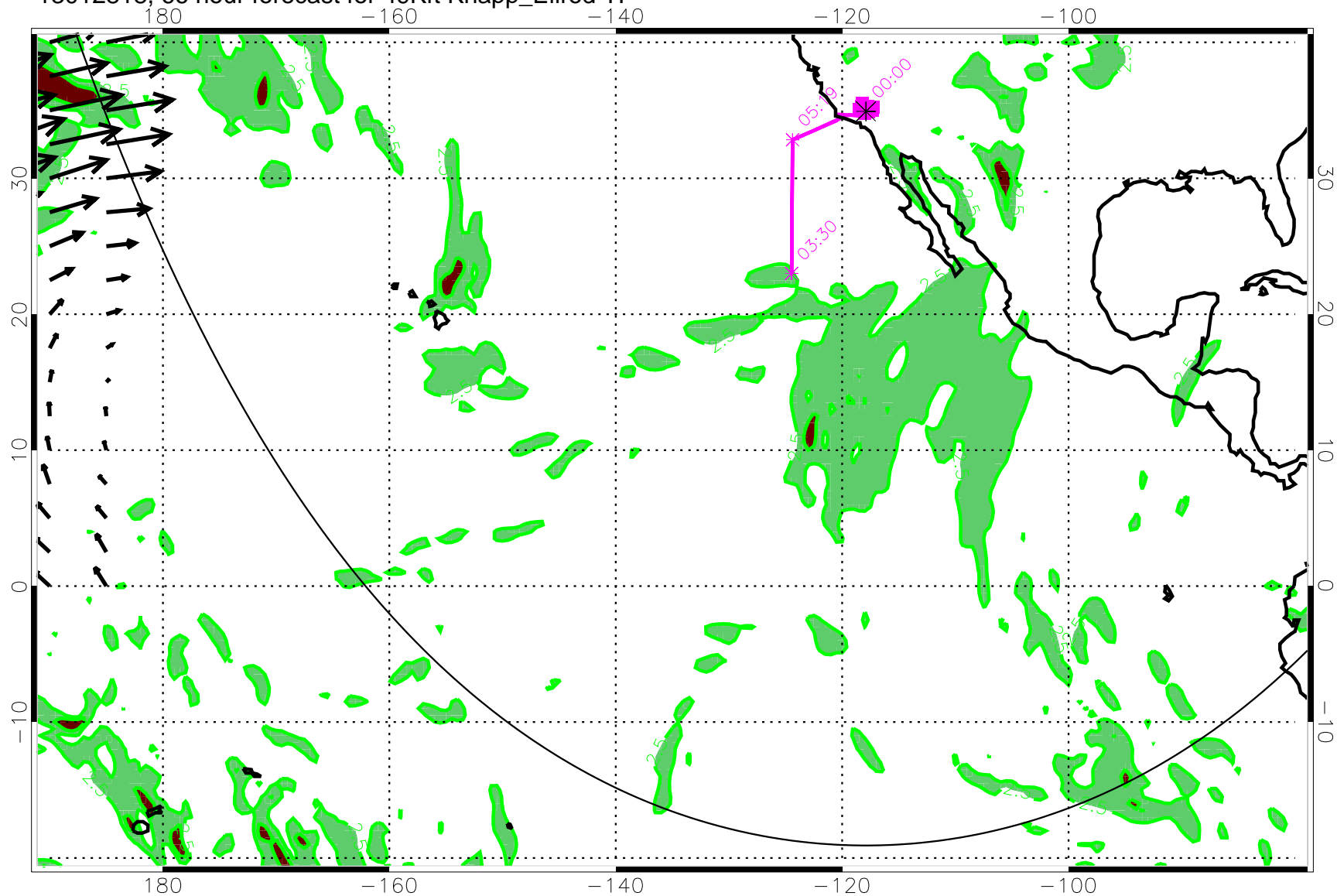
13012818, 66 hour forecast for 49Kft Knapp_Ellrod TI
