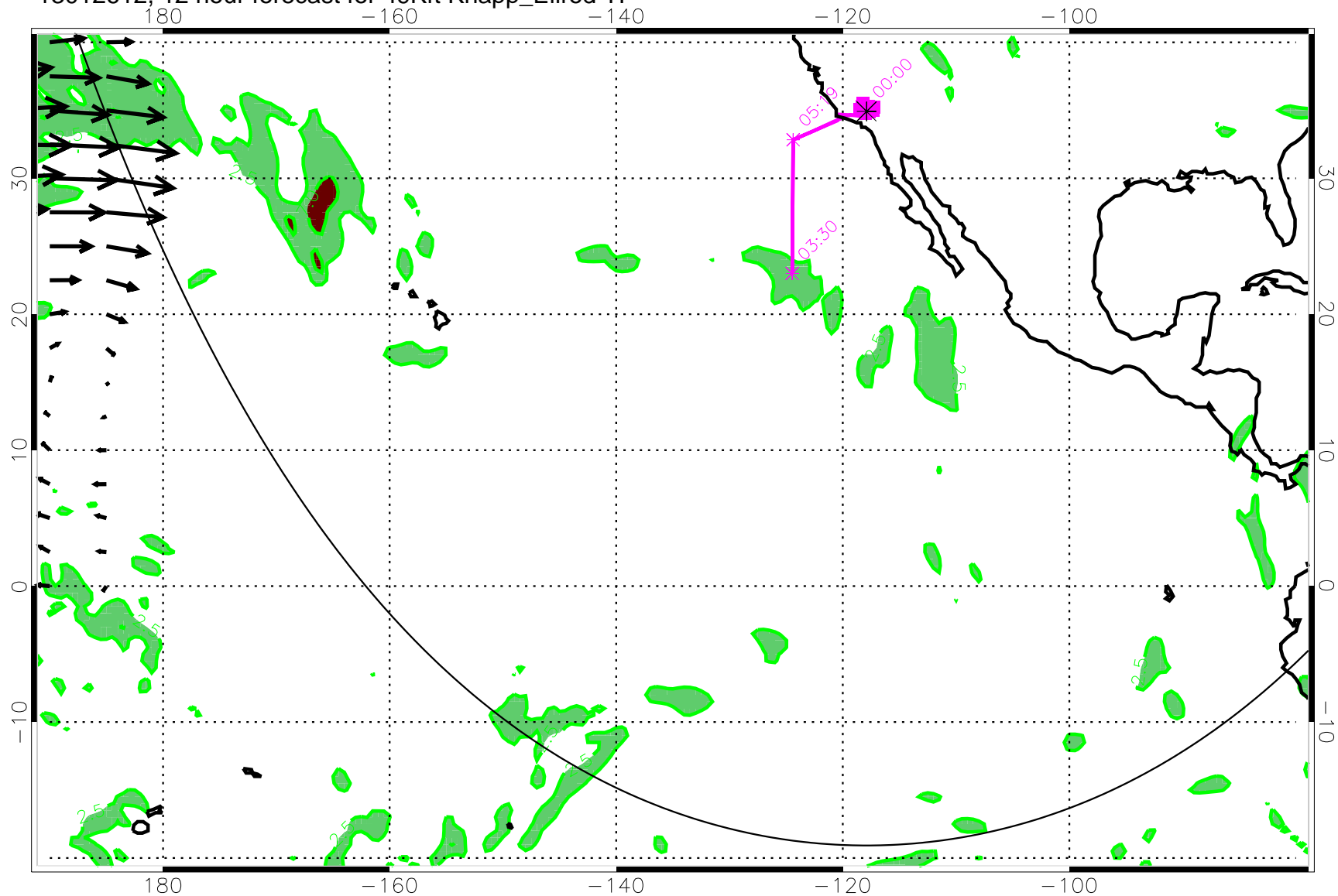
13012612, 12 hour forecast for 49Kft Knapp_Ellrod TI
