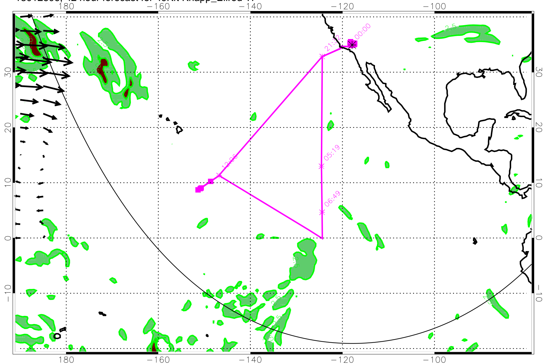
13012606, 42 hour forecast for 49Kft Knapp_Ellrod TI
