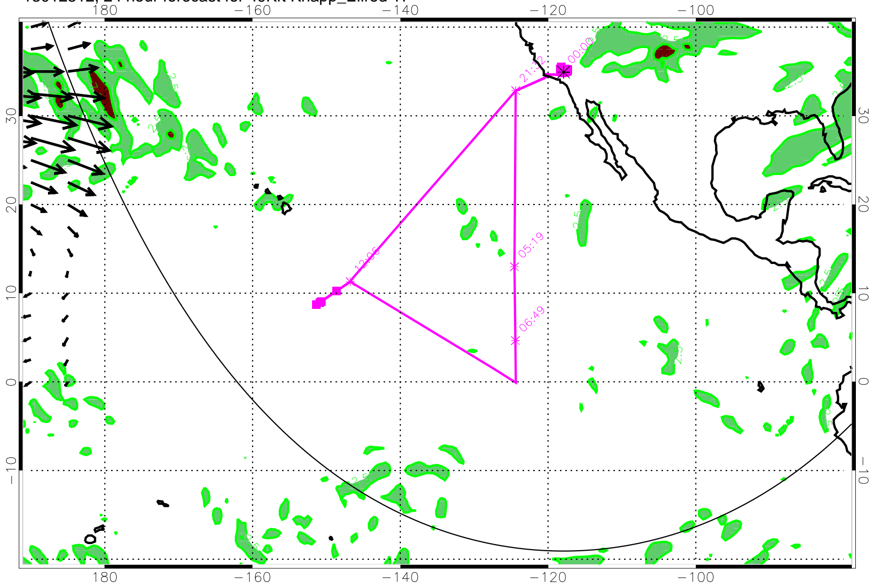
13012512, 24 hour forecast for 49Kft Knapp_Ellrod TI
