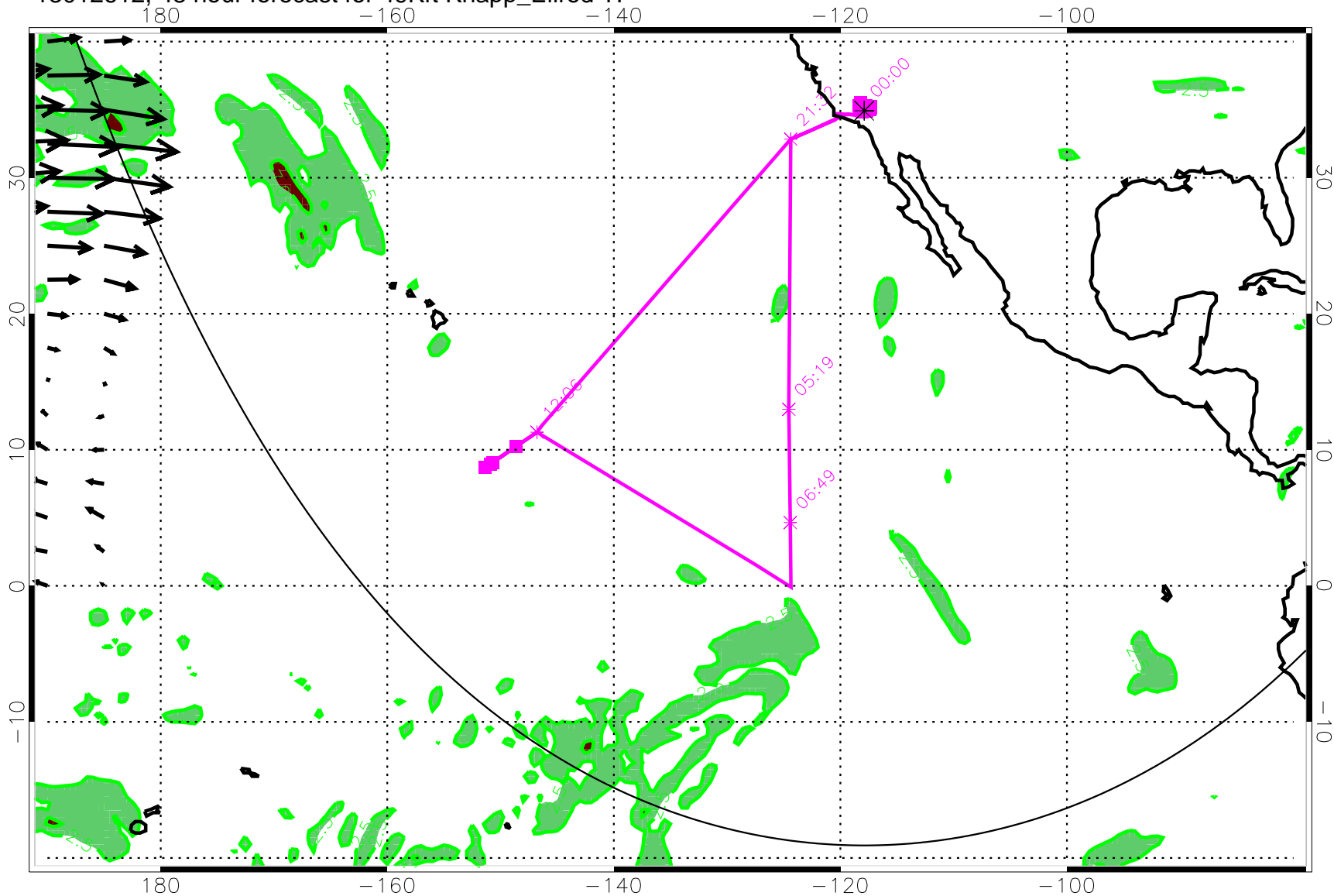
13012612, 48 hour forecast for 49Kft Knapp_Ellrod TI
