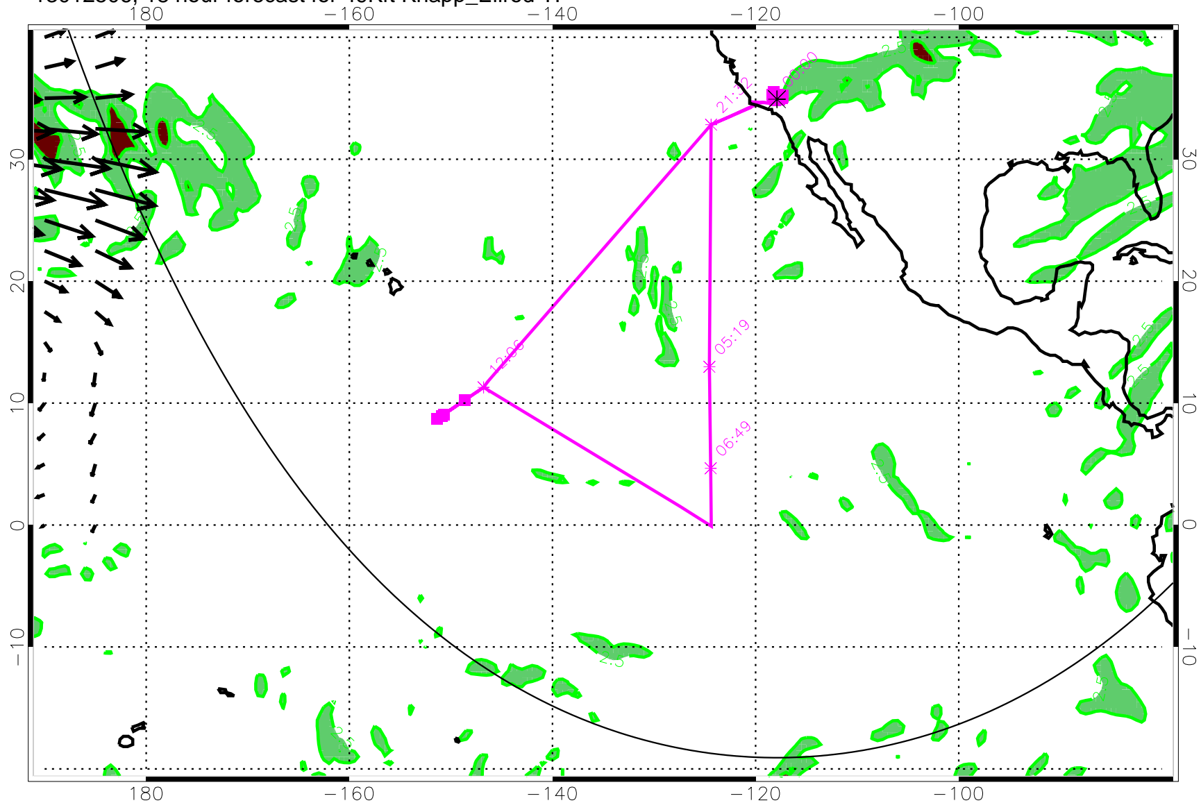
13012506, 18 hour forecast for 49Kft Knapp_Ellrod TI
