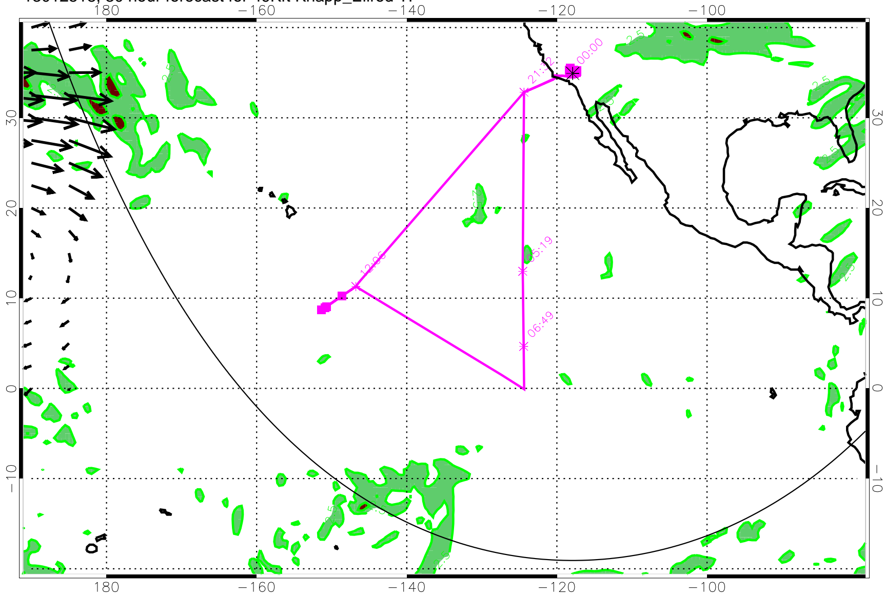
13012518, 30 hour forecast for 49Kft Knapp_Ellrod TI
