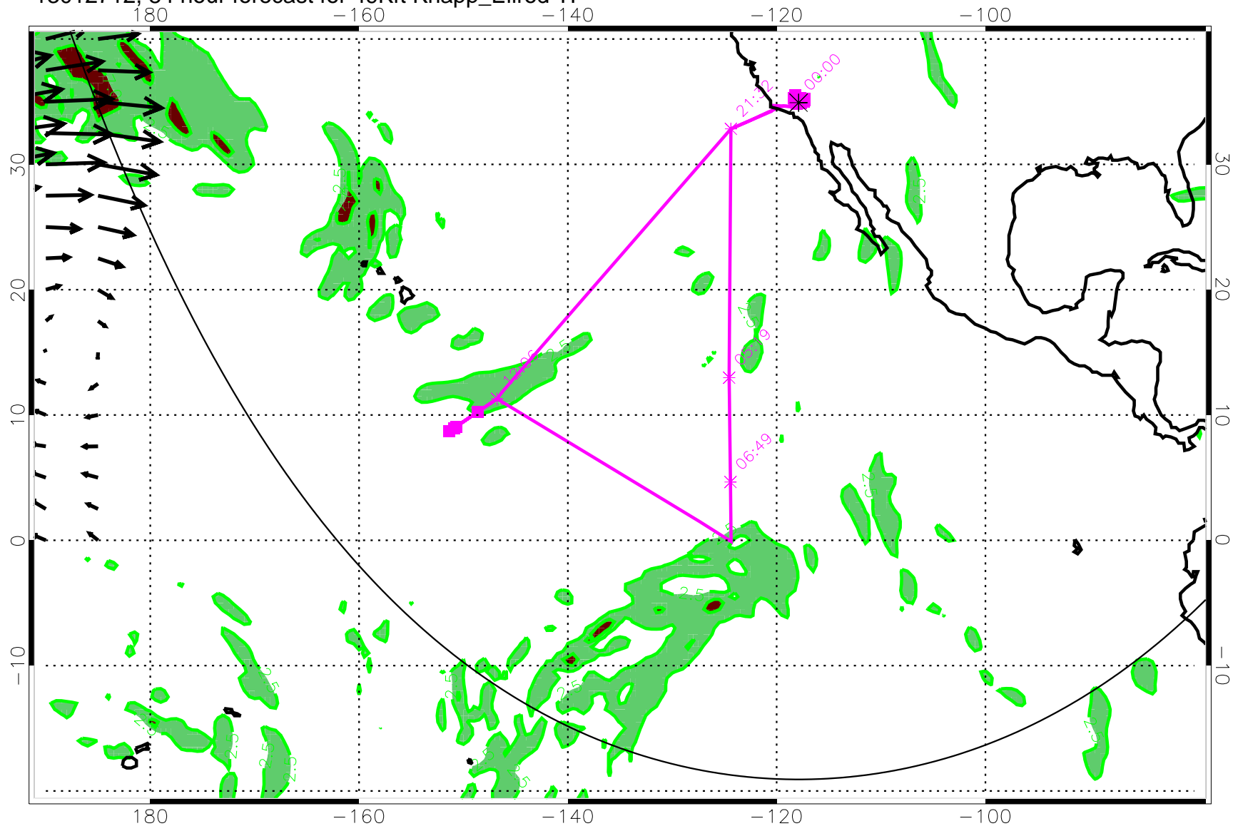
13012712, 84 hour forecast for 49Kft Knapp_Ellrod TI
