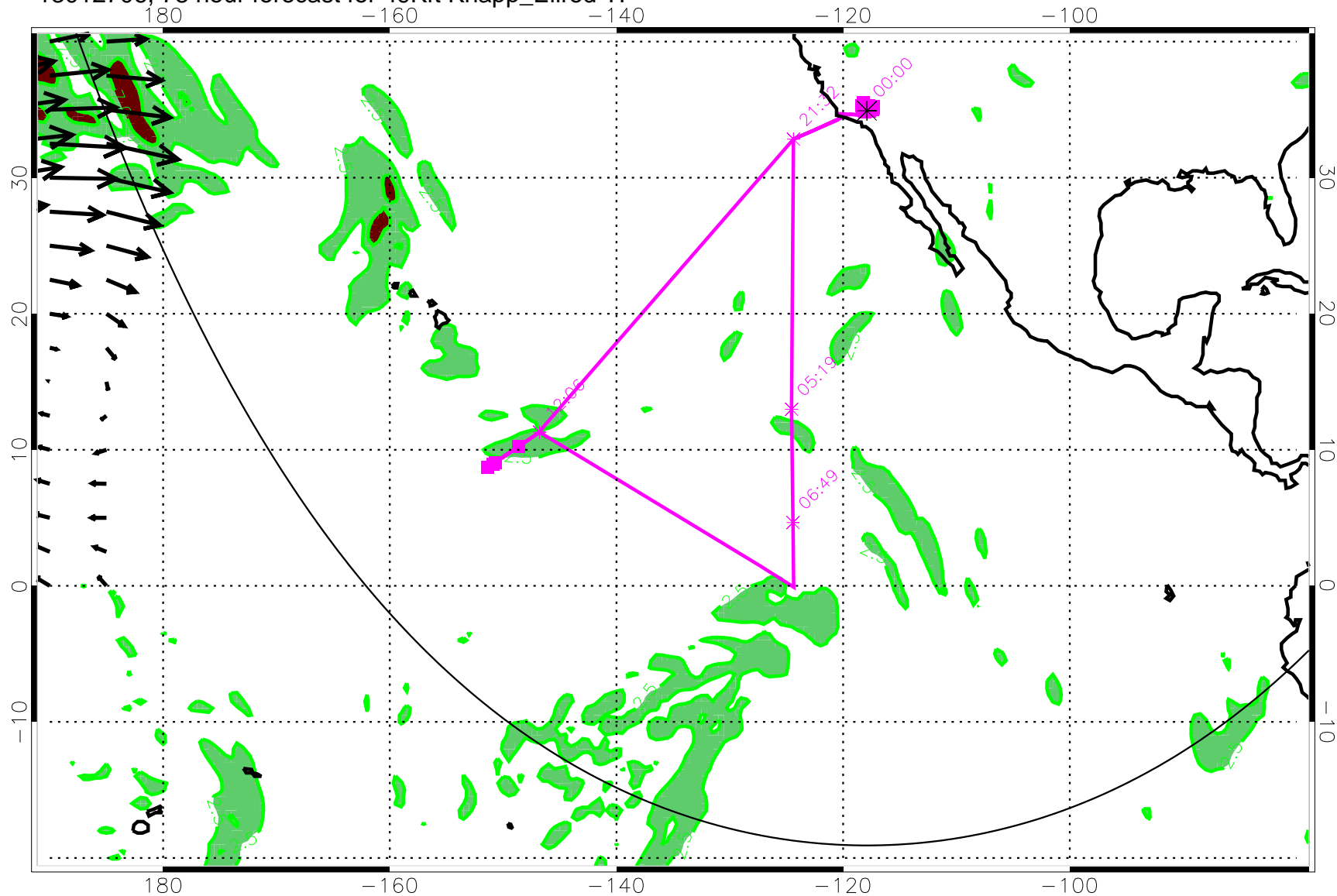
13012706, 78 hour forecast for 49Kft Knapp_Ellrod TI
