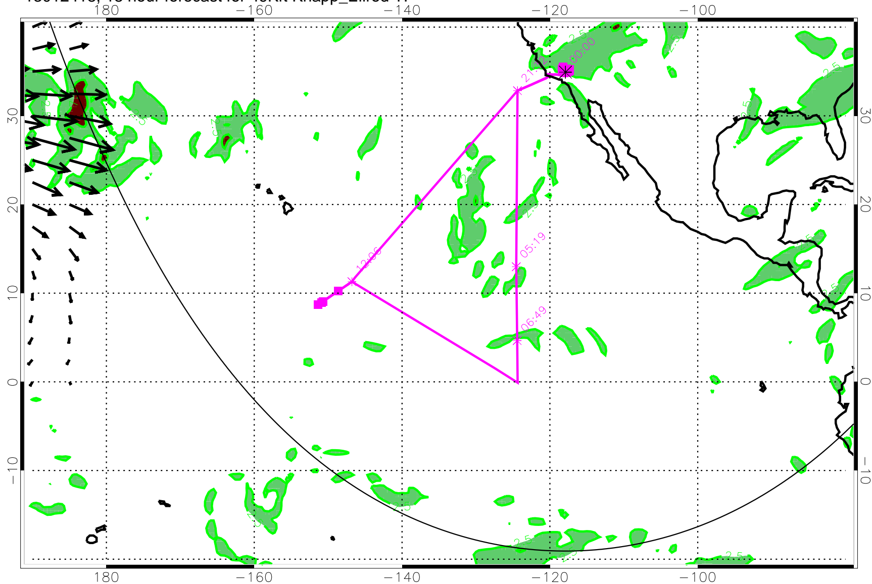
13012418, 18 hour forecast for 49Kft Knapp_Ellrod TI
