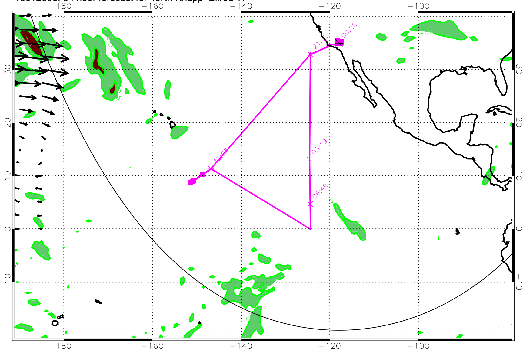
13012606, 54 hour forecast for 49Kft Knapp_Ellrod TI
