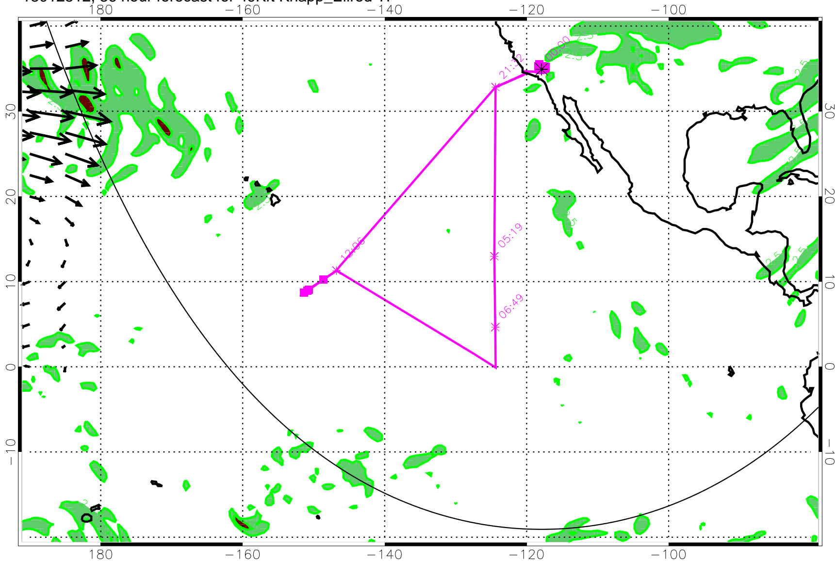
13012512, 36 hour forecast for 49Kft Knapp_Ellrod TI
