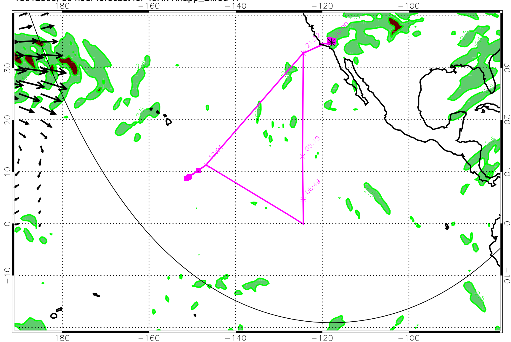
13012506, 30 hour forecast for 49Kft Knapp_Ellrod TI
