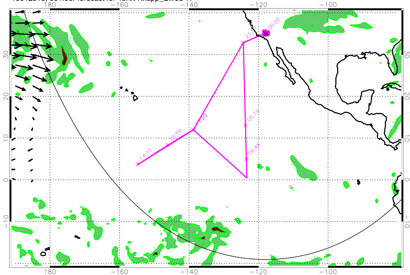
13012518, 66 hour forecast for 49Kft Knapp_Ellrod TI
