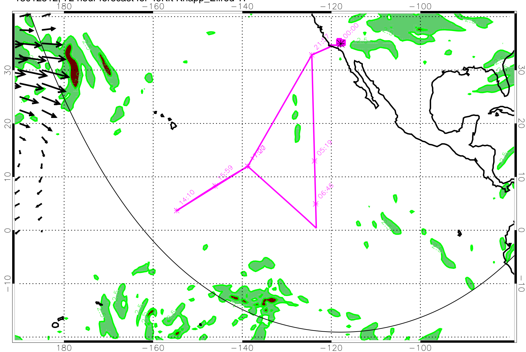
13012512, 72 hour forecast for 49Kft Knapp_Ellrod TI
