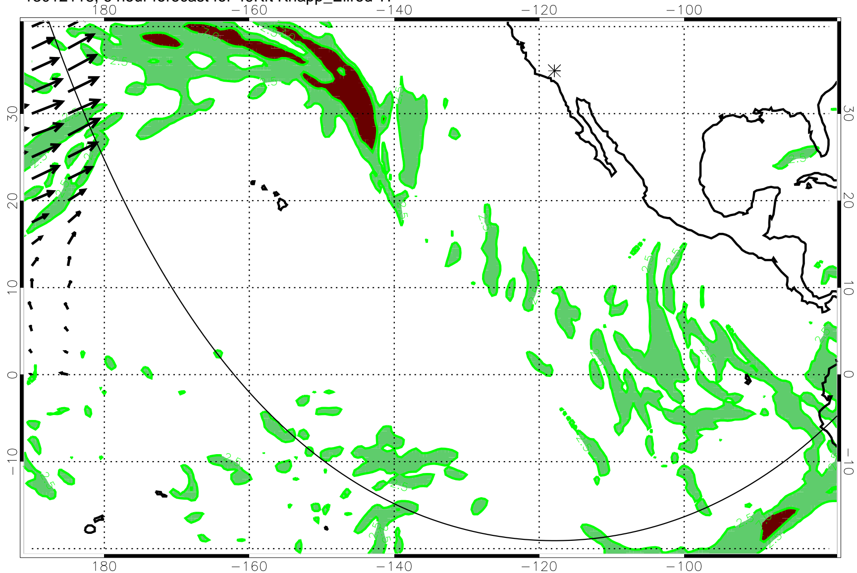
13012118, 6 hour forecast for 49Kft Knapp_Ellrod TI
