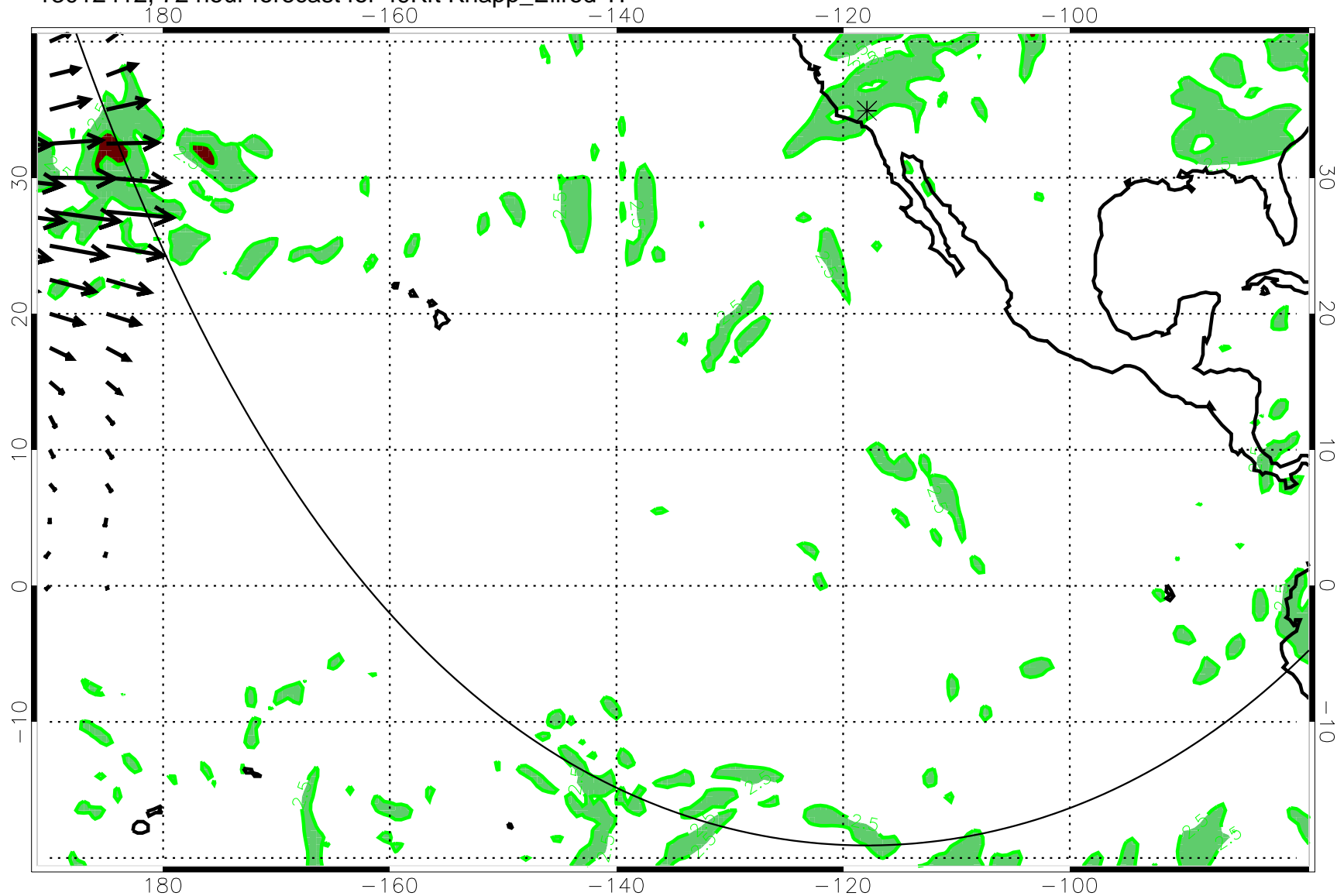
13012412, 72 hour forecast for 49Kft Knapp_Ellrod TI
