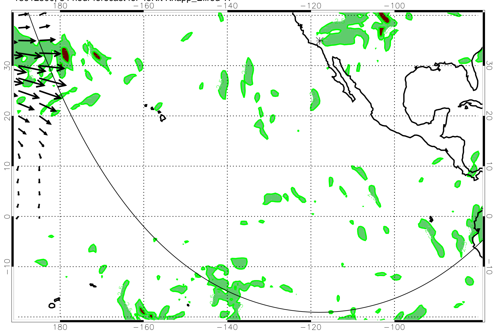
13012500, 84 hour forecast for 49Kft Knapp_Ellrod TI
