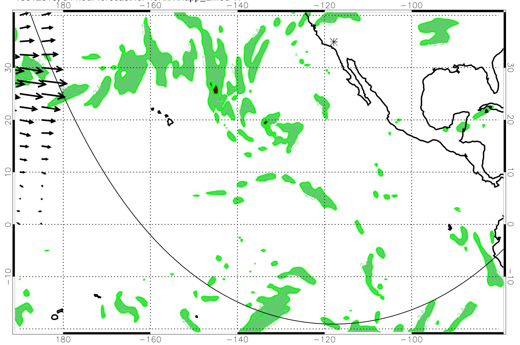
13012318, 54 hour forecast for 49Kft Knapp_Ellrod TI
