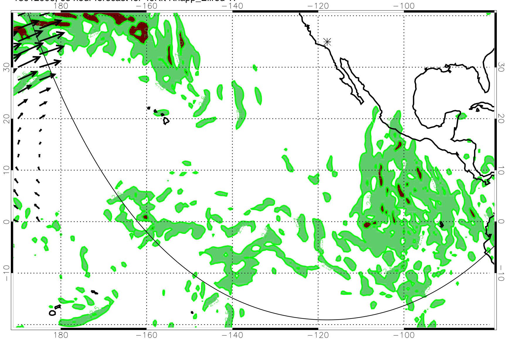
13012006, 66 hour forecast for 49Kft Knapp_Ellrod TI
