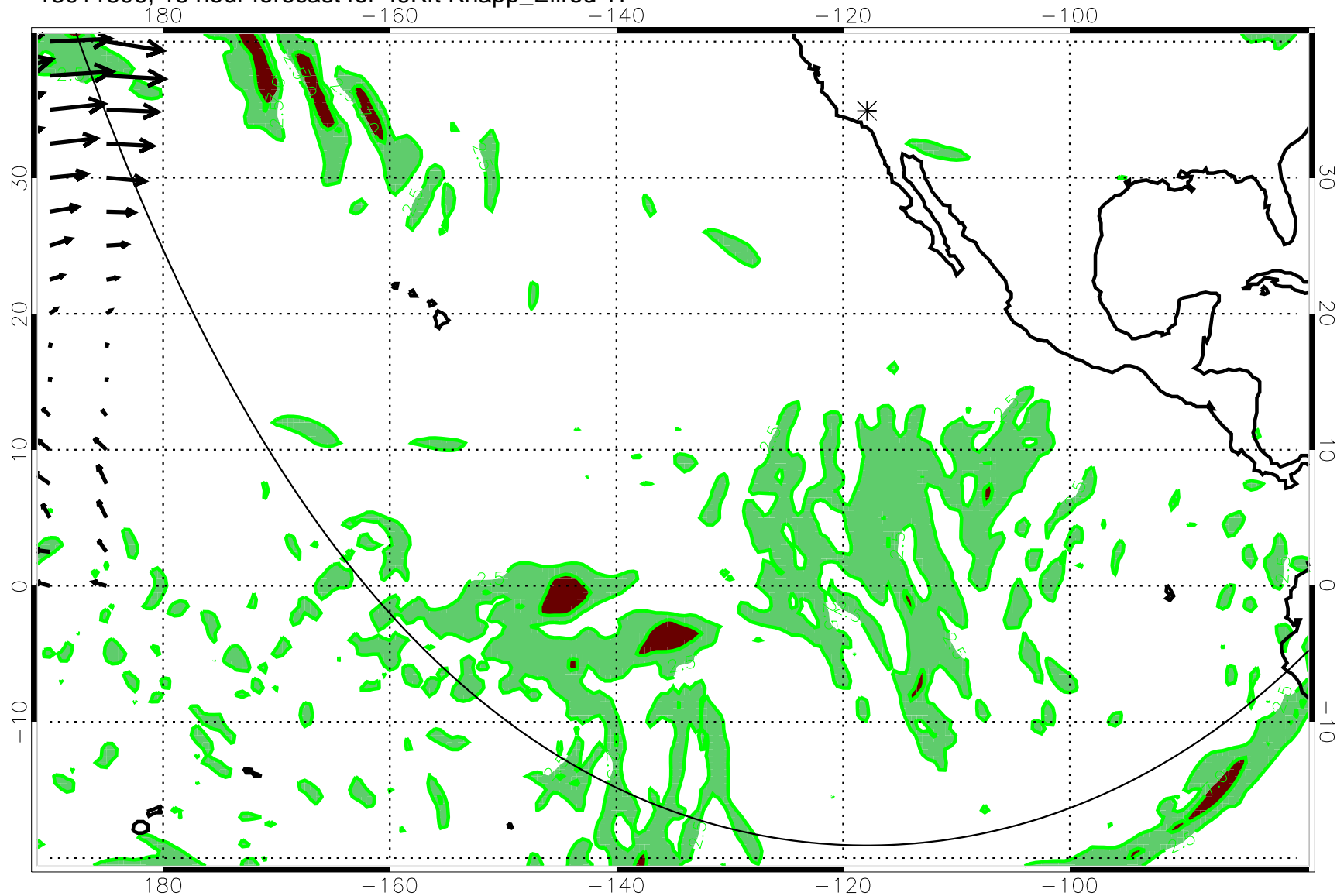
13011806, 18 hour forecast for 49Kft Knapp_Ellrod TI
