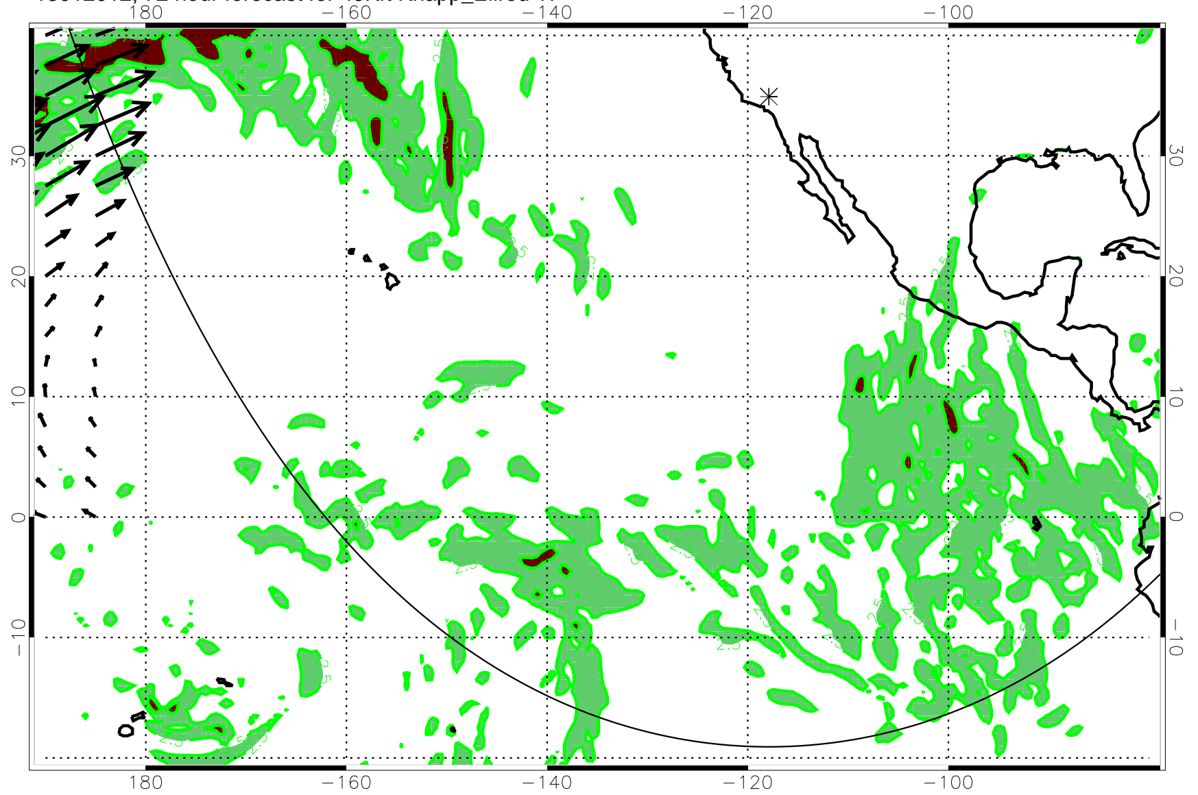
13012012, 72 hour forecast for 49Kft Knapp_Ellrod TI
