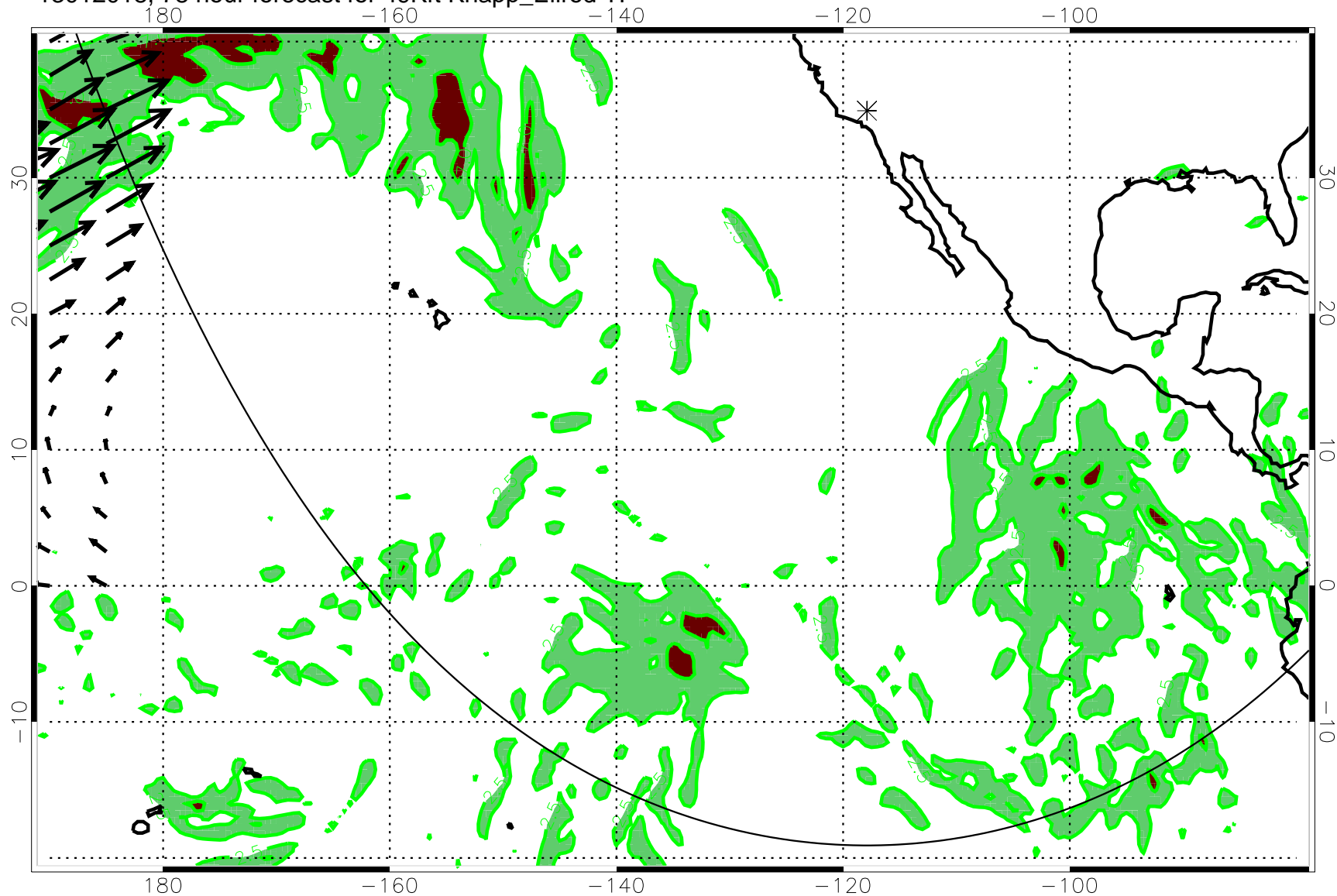
13012018, 78 hour forecast for 49Kft Knapp_Ellrod TI
