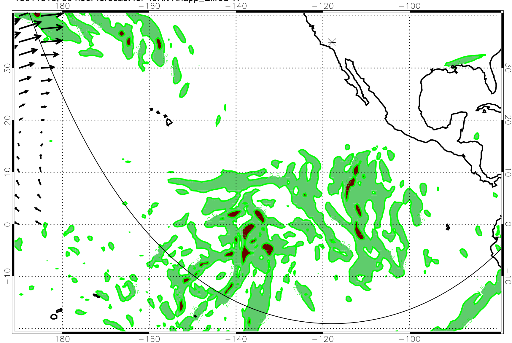
13011818, 30 hour forecast for 49Kft Knapp_Ellrod TI
