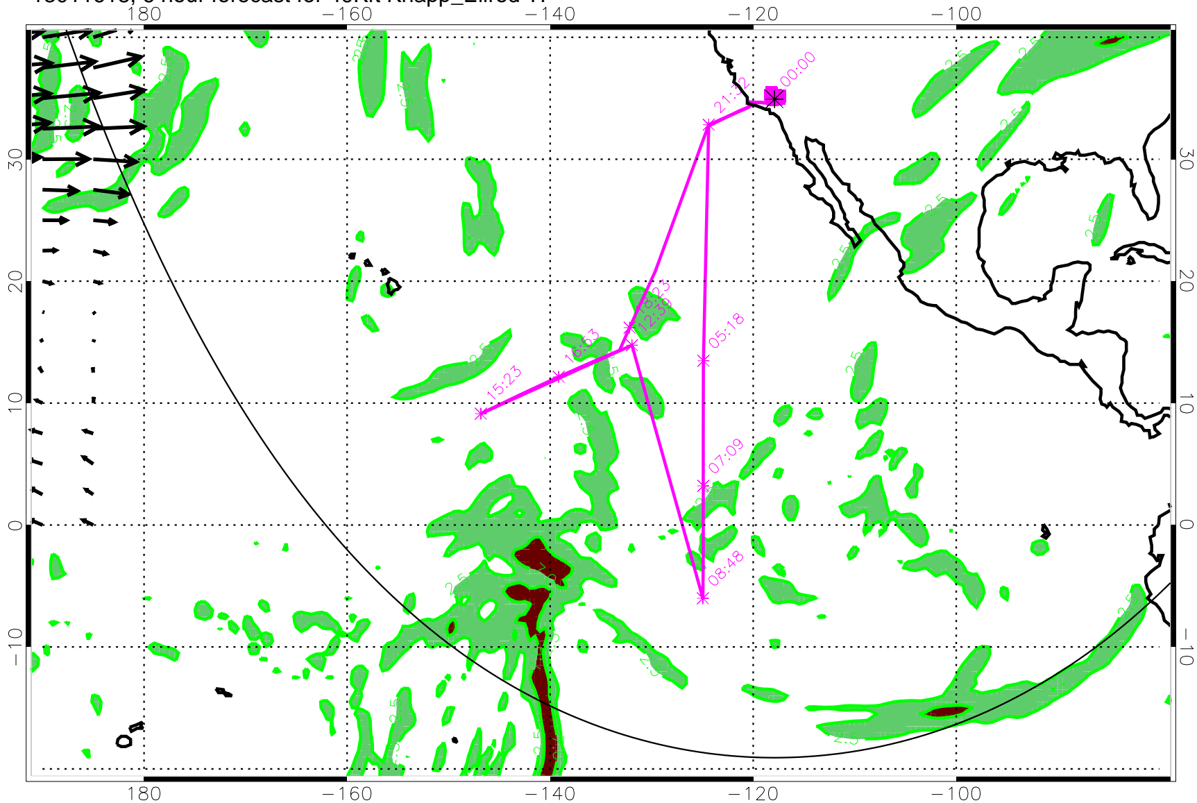
13011618, 6 hour forecast for 49Kft Knapp_Ellrod TI
