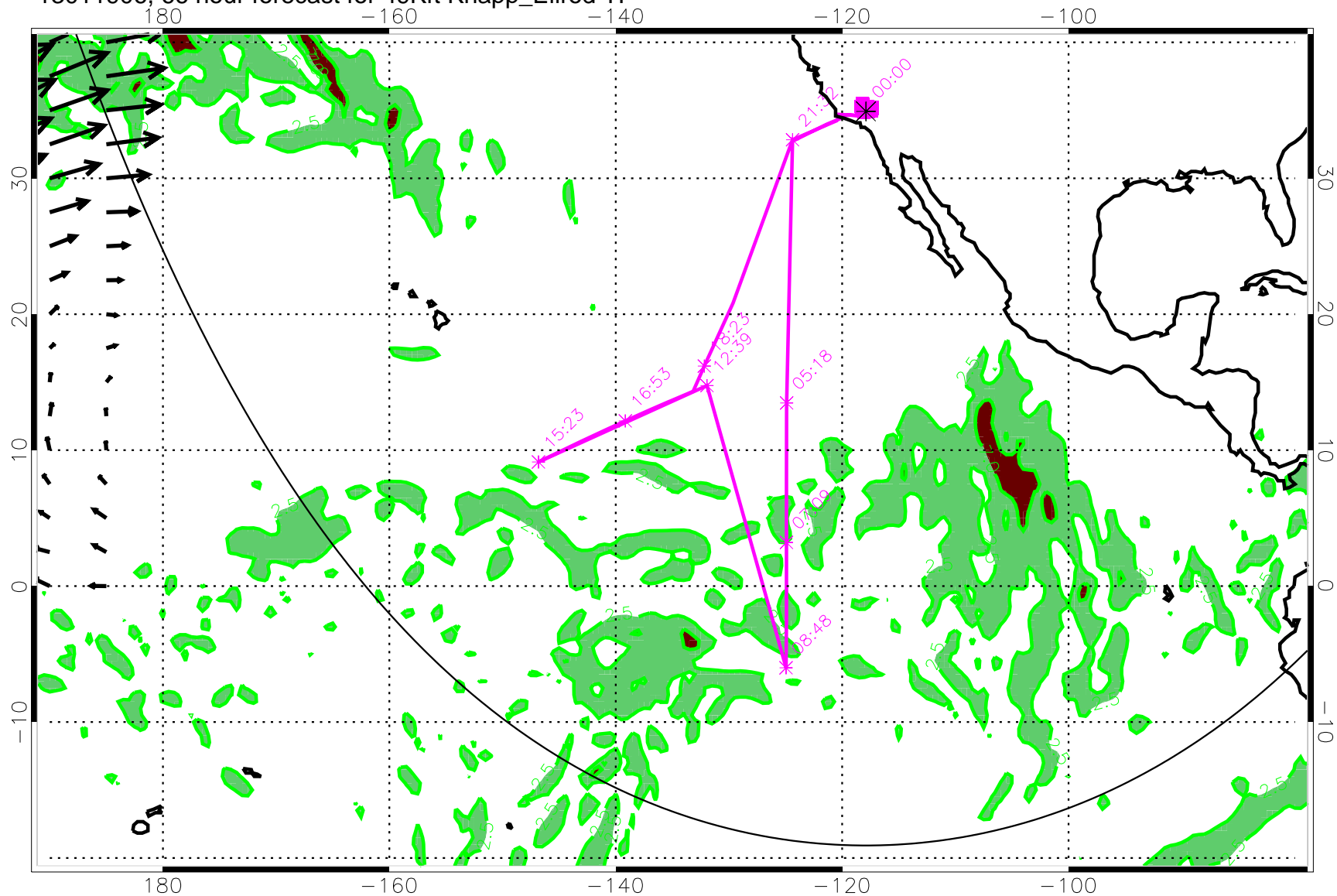
13011906, 66 hour forecast for 49Kft Knapp_Ellrod TI
