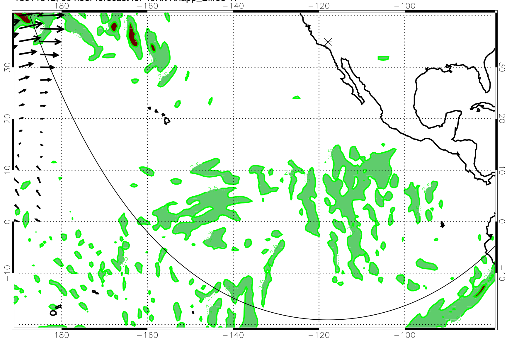
13011812, 60 hour forecast for 49Kft Knapp_Ellrod TI
