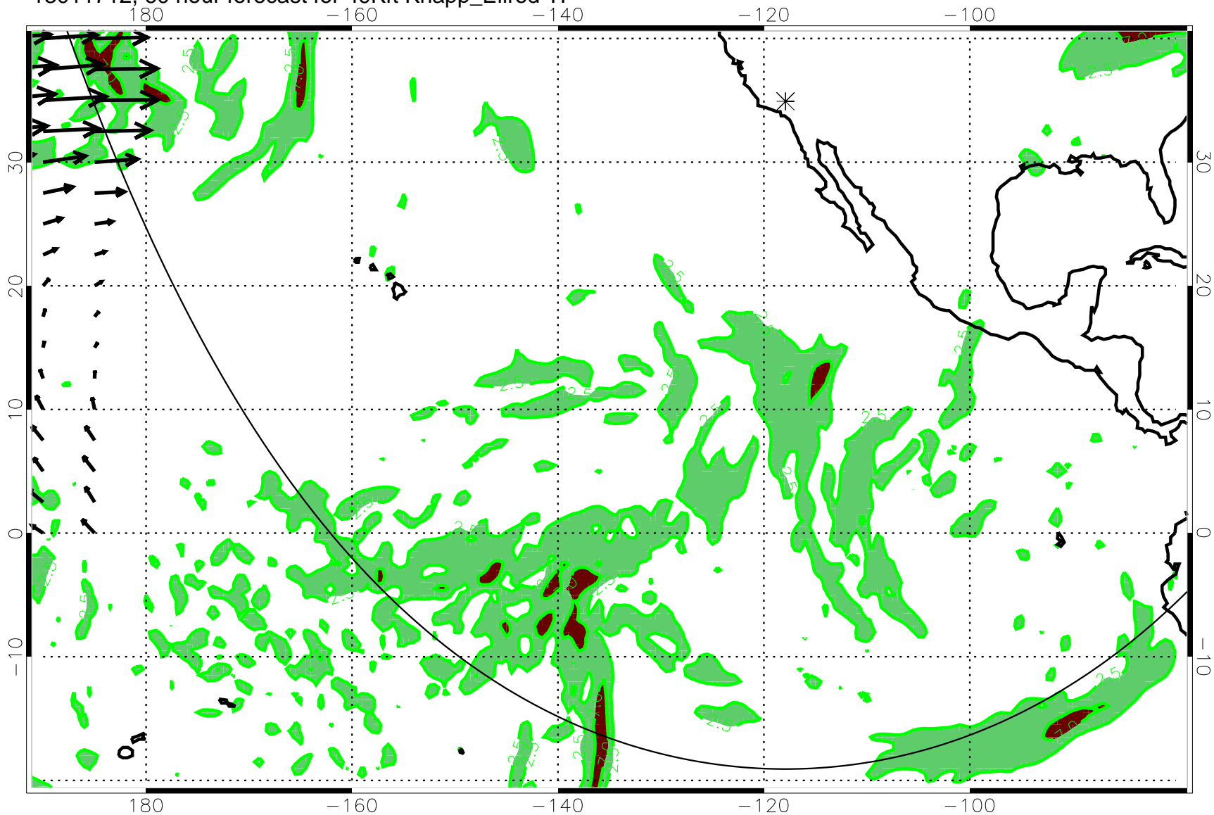
13011712, 60 hour forecast for 49Kft Knapp_Ellrod TI
