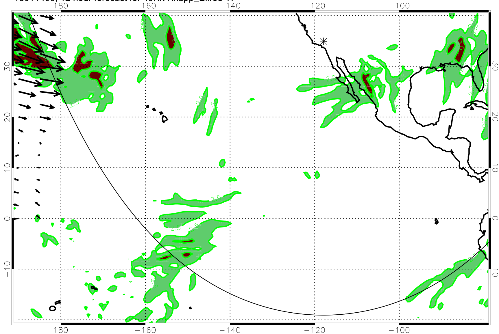
13011400, 12 hour forecast for 49Kft Knapp_Ellrod TI
