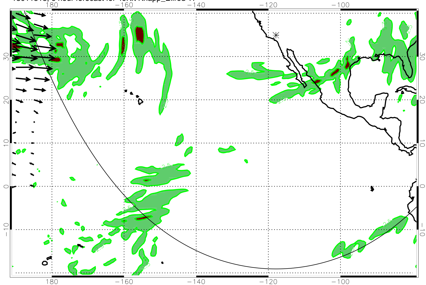
13011318, 6 hour forecast for 49Kft Knapp_Ellrod TI
