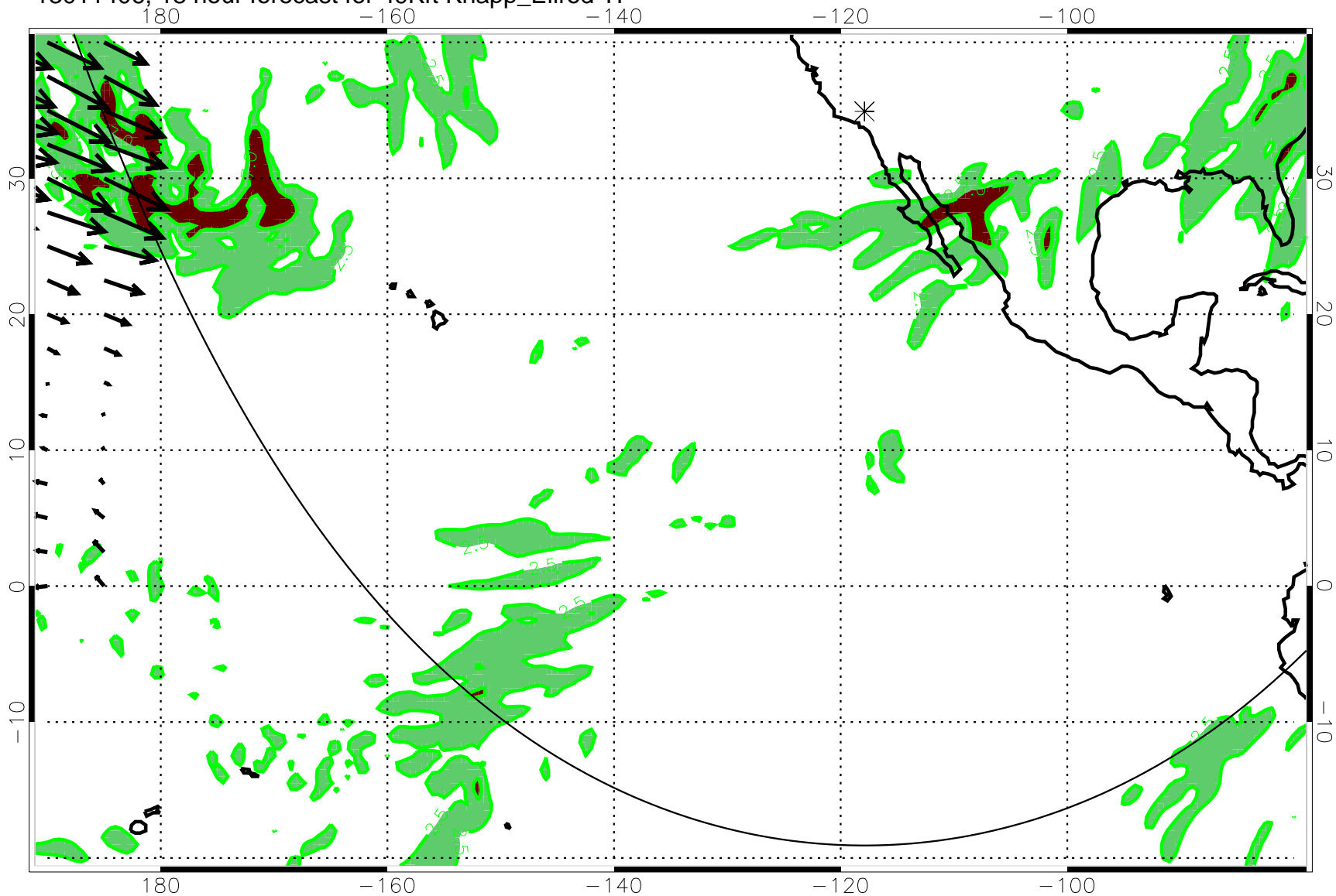
13011406, 18 hour forecast for 49Kft Knapp_Ellrod TI
