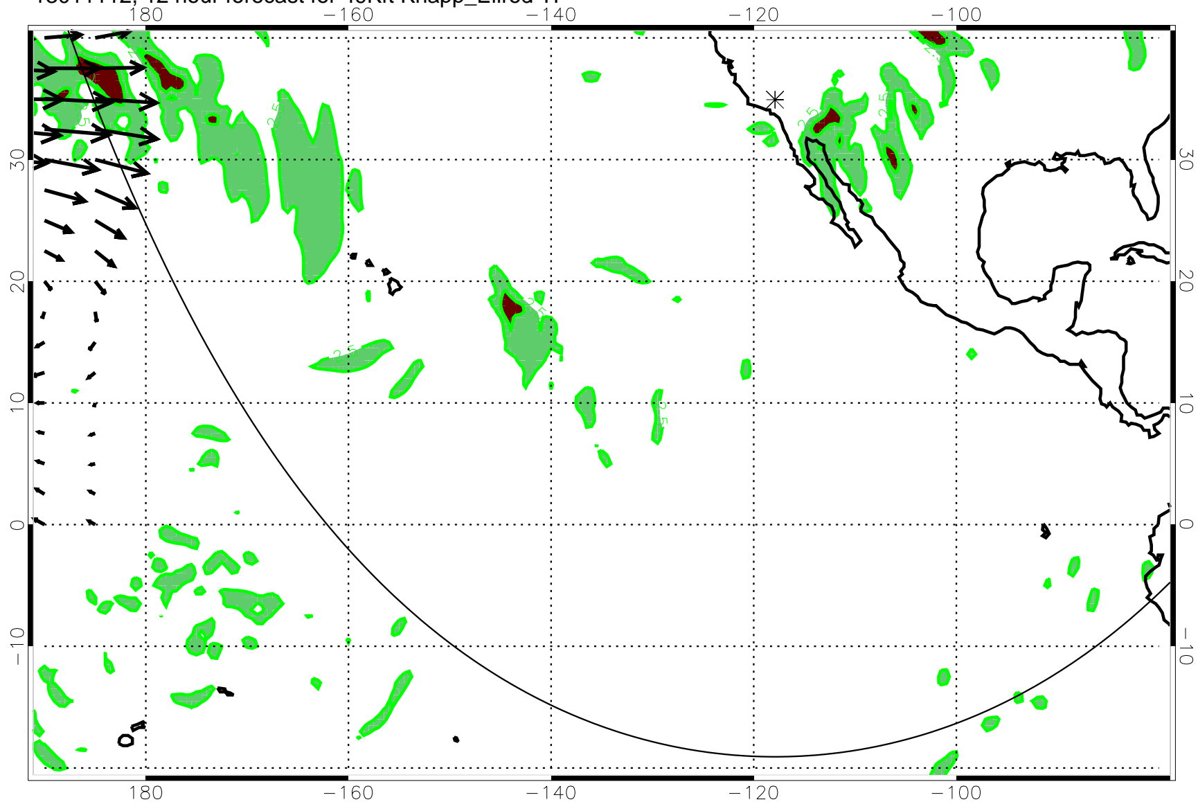
13011112, 12 hour forecast for 49Kft Knapp_Ellrod TI
