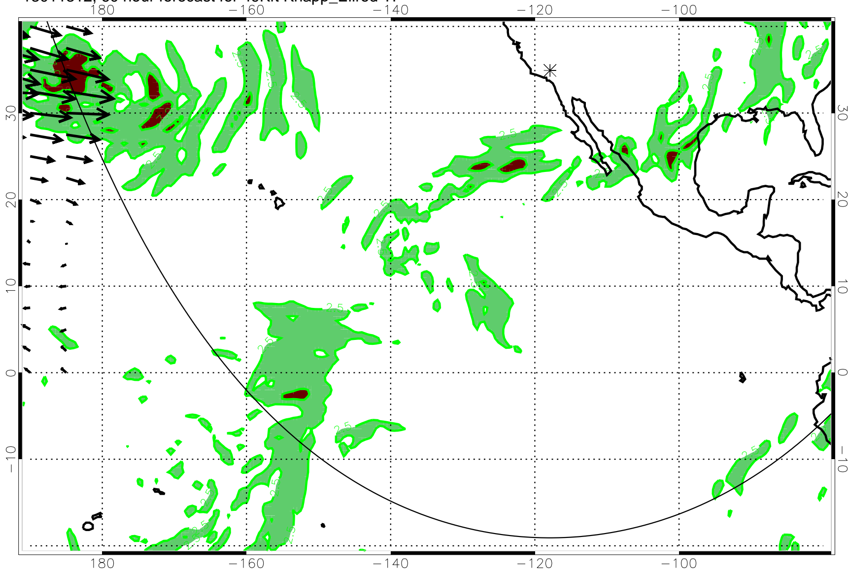
13011312, 60 hour forecast for 49Kft Knapp_Ellrod TI
