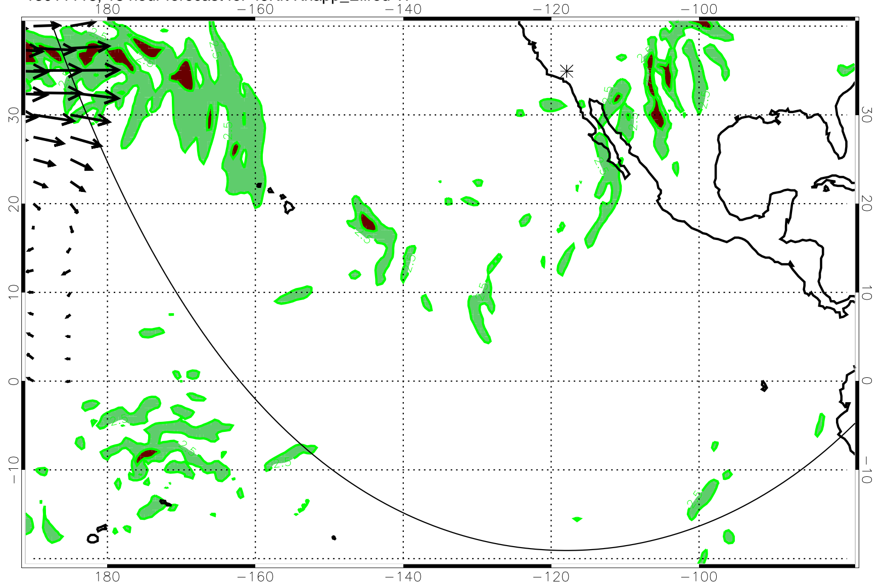
13011118, 18 hour forecast for 49Kft Knapp_Ellrod TI
