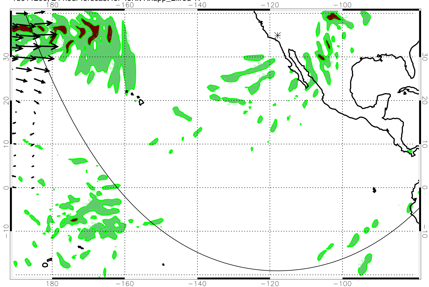
13011200, 24 hour forecast for 49Kft Knapp_Ellrod TI
