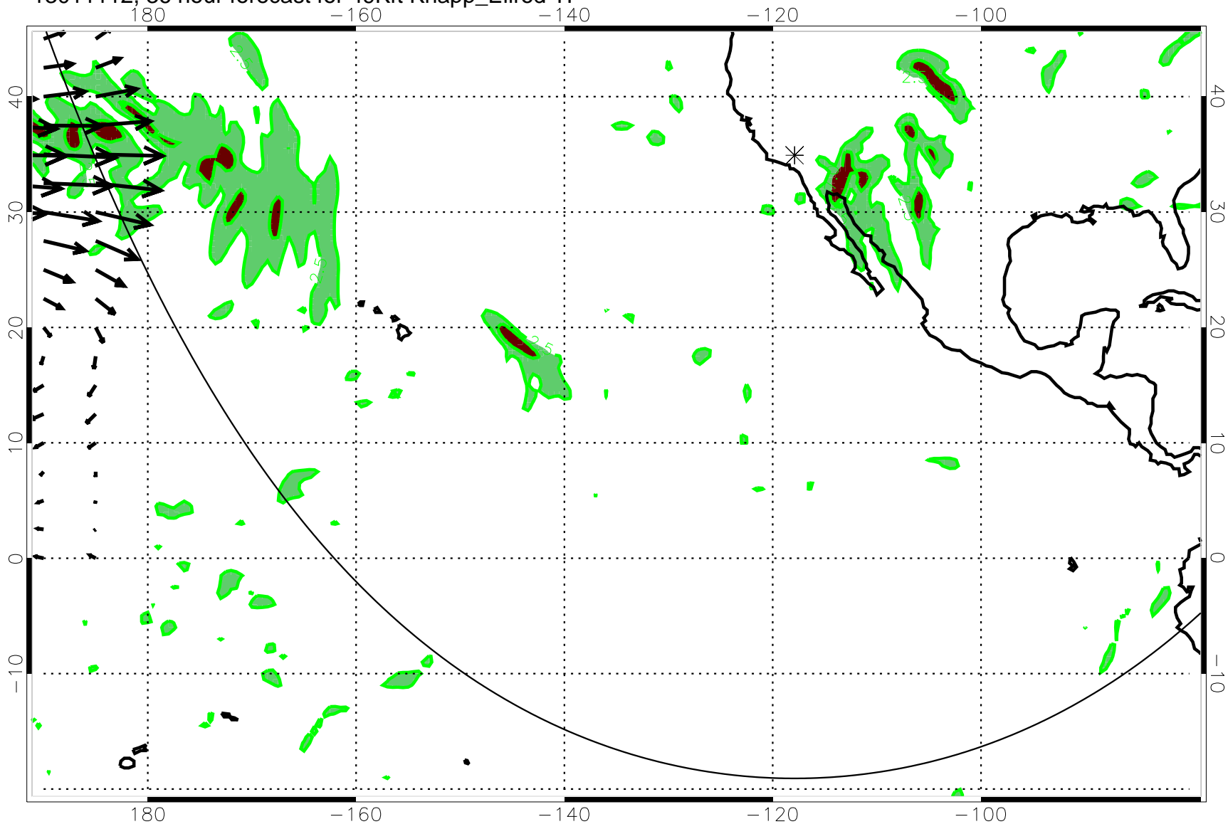
13011112, 36 hour forecast for 49Kft Knapp_Ellrod TI
