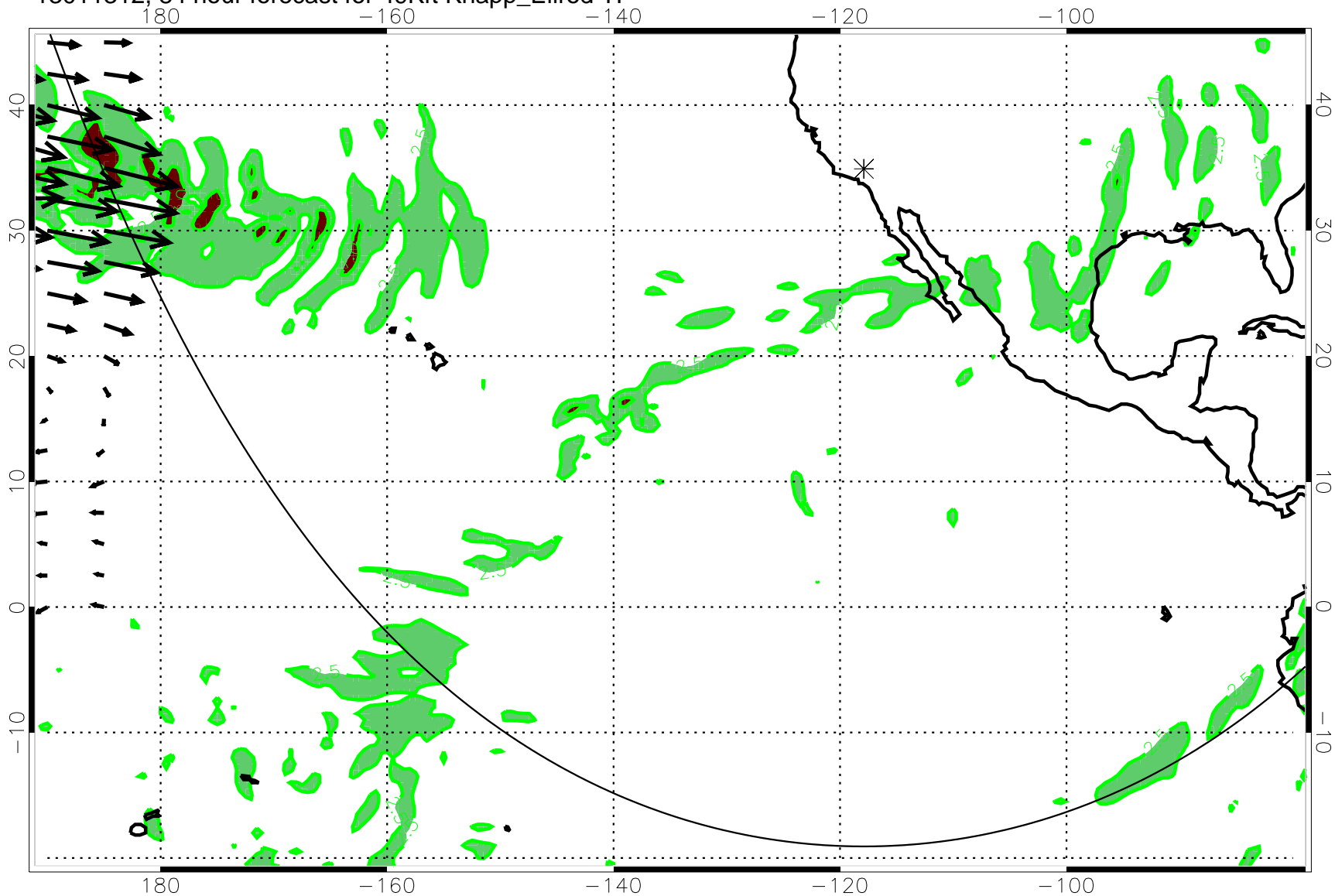
13011312, 84 hour forecast for 49Kft Knapp_Ellrod TI
