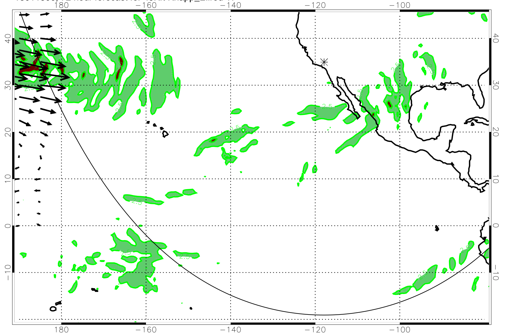
13011300, 72 hour forecast for 49Kft Knapp_Ellrod TI
