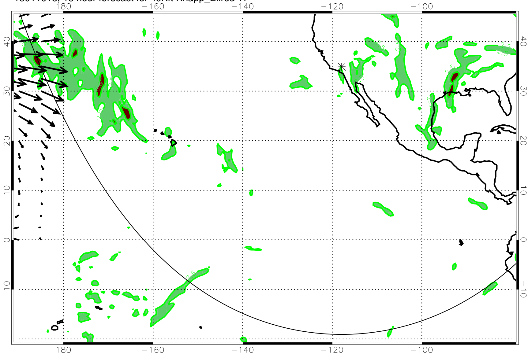
13011018, 18 hour forecast for 49Kft Knapp_Ellrod TI
