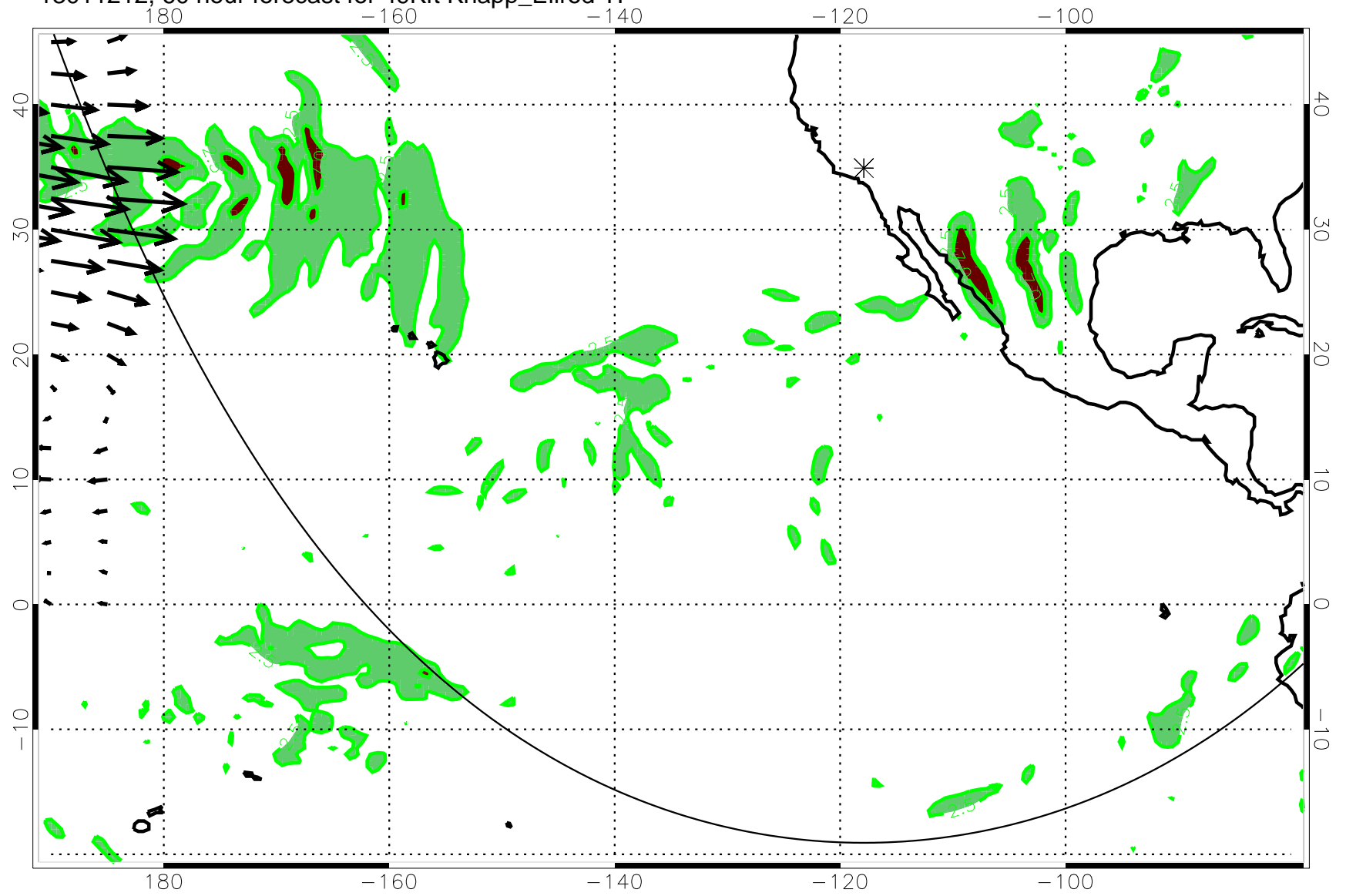
13011212, 60 hour forecast for 49Kft Knapp_Ellrod TI
