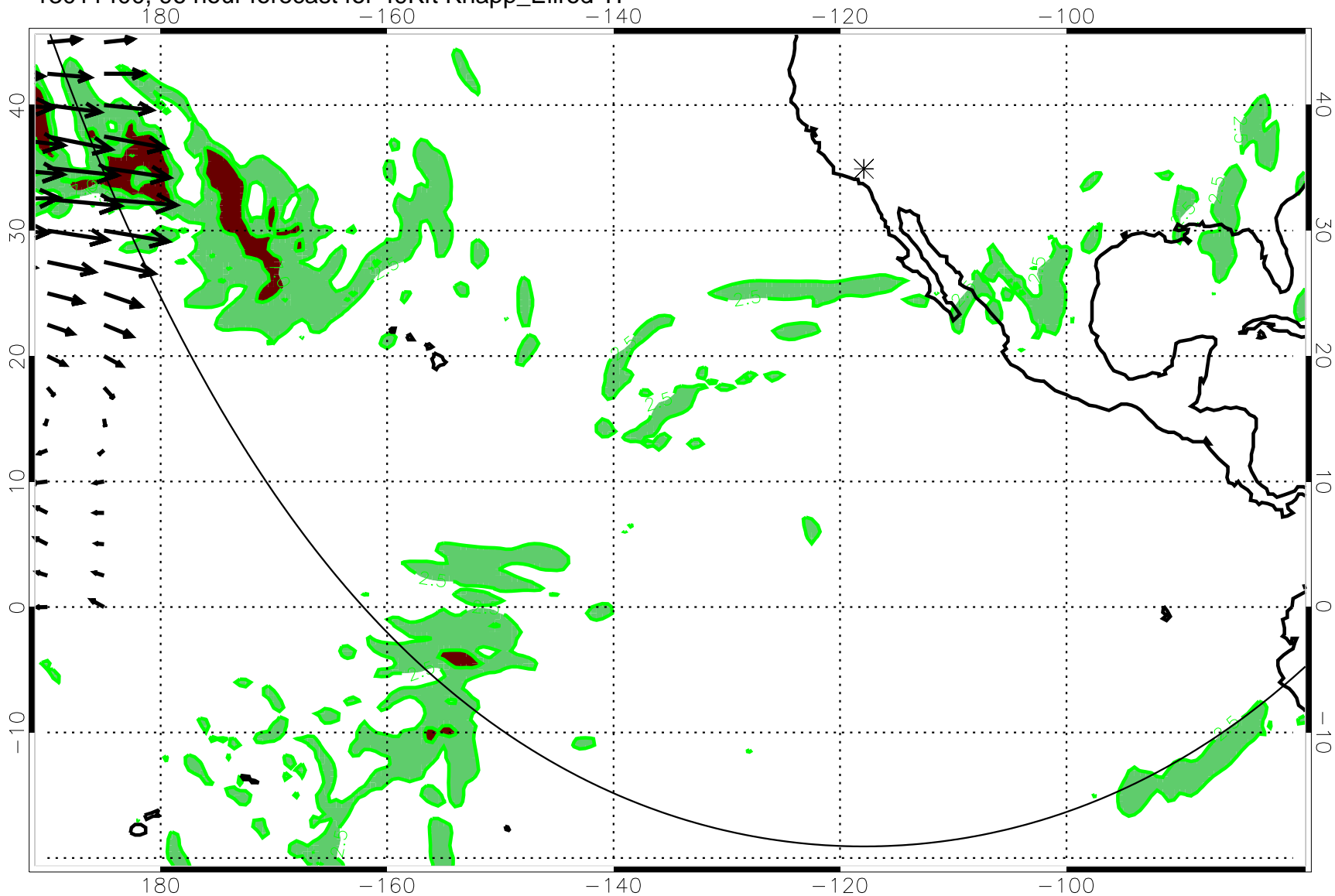
13011400, 96 hour forecast for 49Kft Knapp_Ellrod TI
