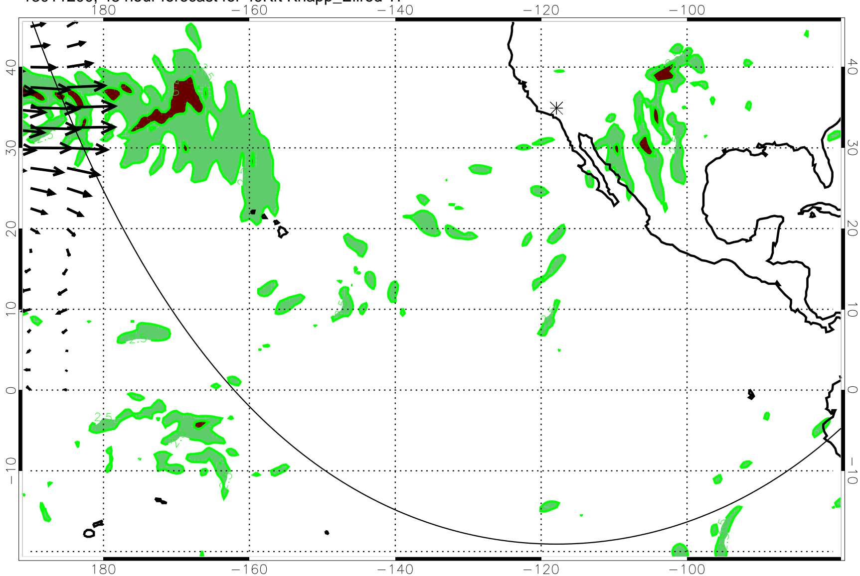
13011200, 48 hour forecast for 49Kft Knapp_Ellrod TI
