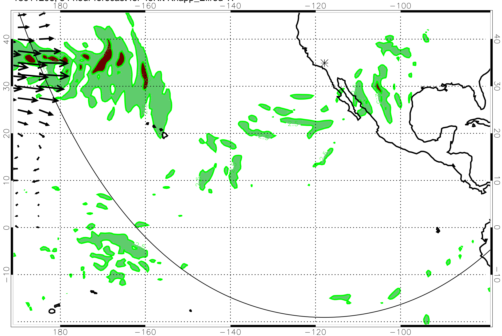
13011206, 54 hour forecast for 49Kft Knapp_Ellrod TI
