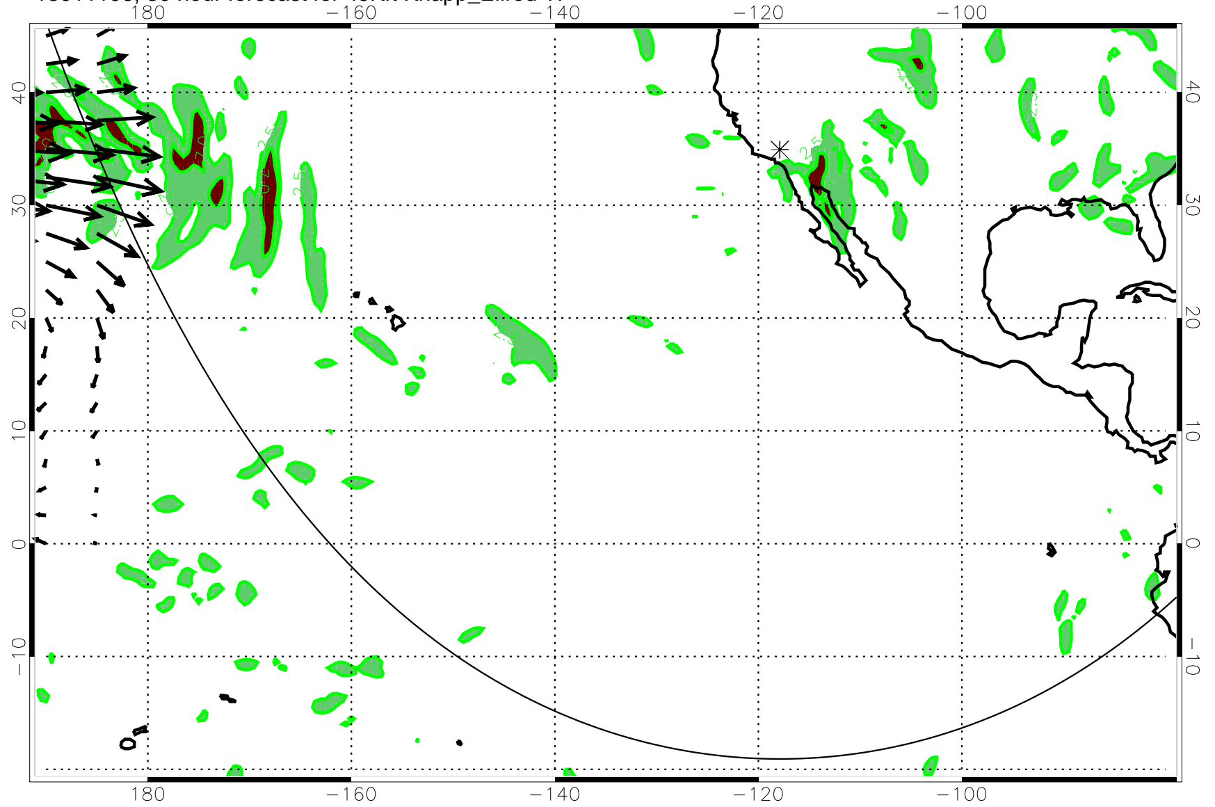
13011106, 30 hour forecast for 49Kft Knapp_Ellrod TI
