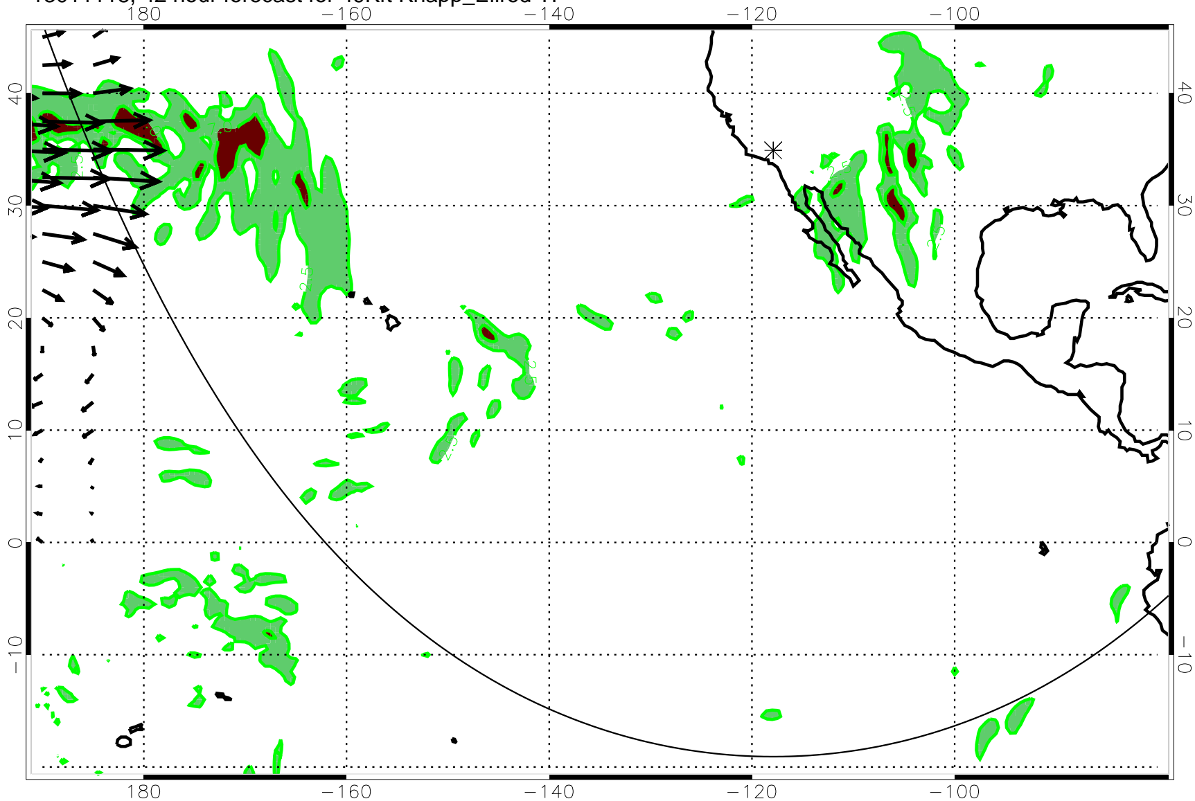
13011118, 42 hour forecast for 49Kft Knapp_Ellrod TI
