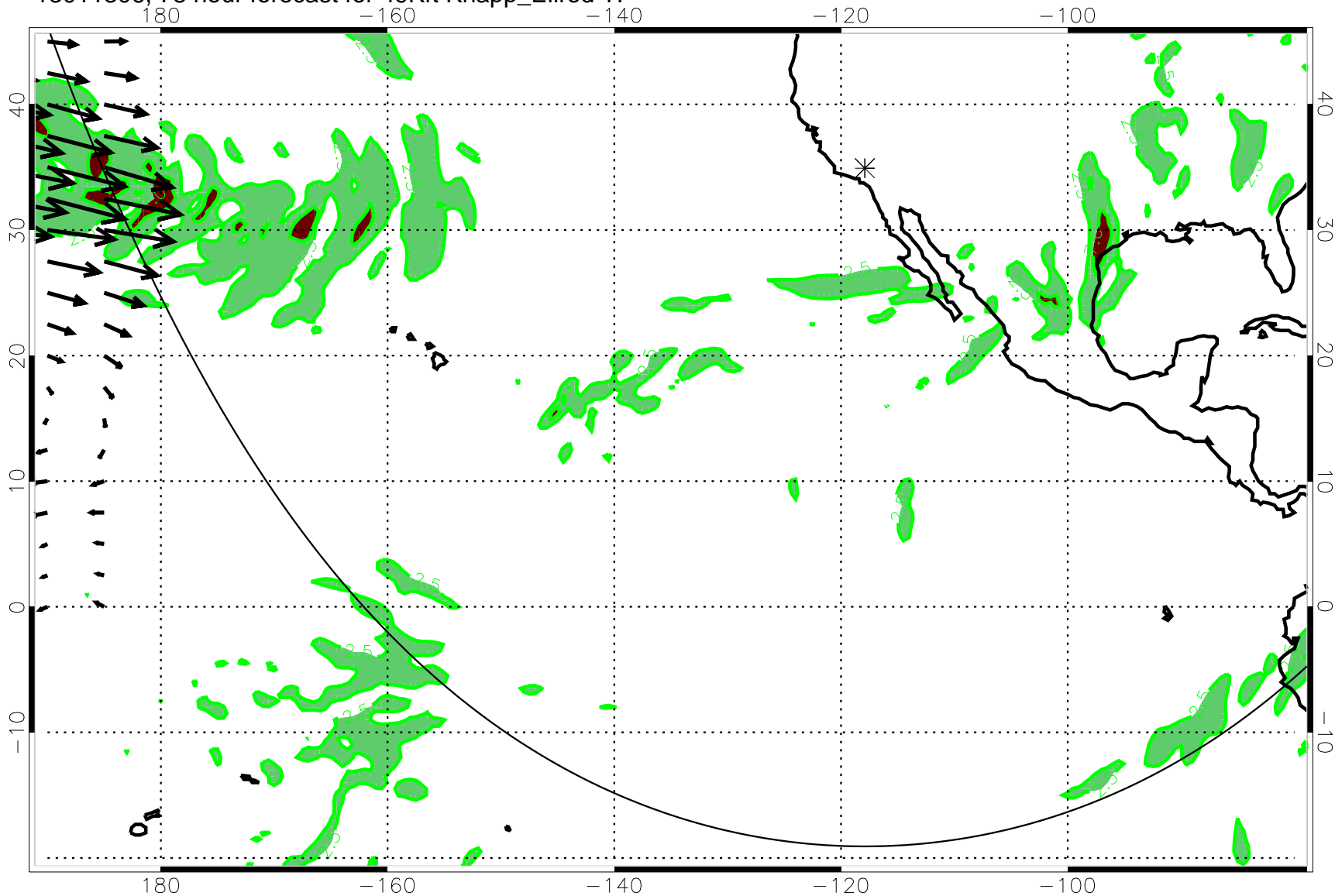
13011306, 78 hour forecast for 49Kft Knapp_Ellrod TI
