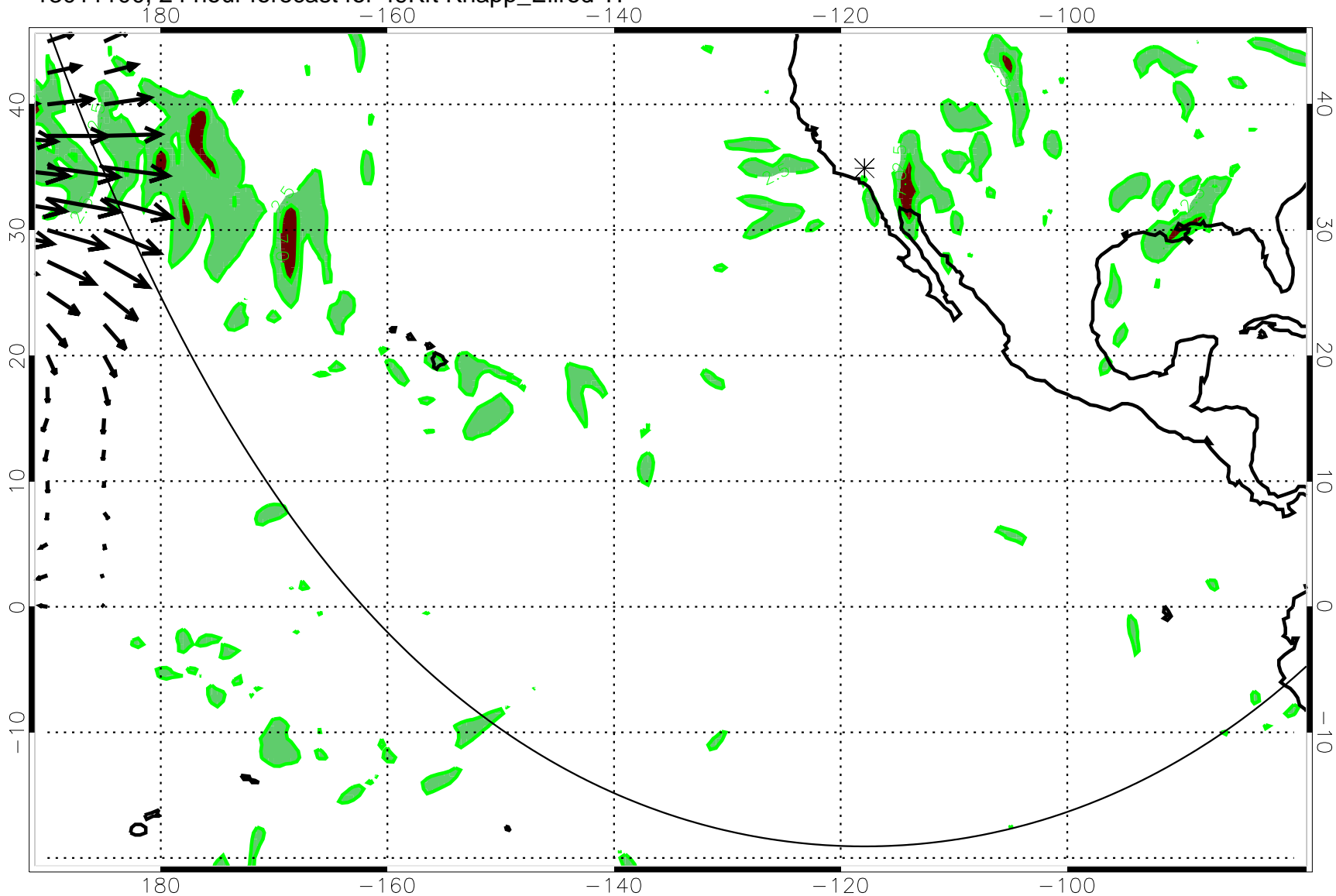
13011100, 24 hour forecast for 49Kft Knapp_Ellrod TI
