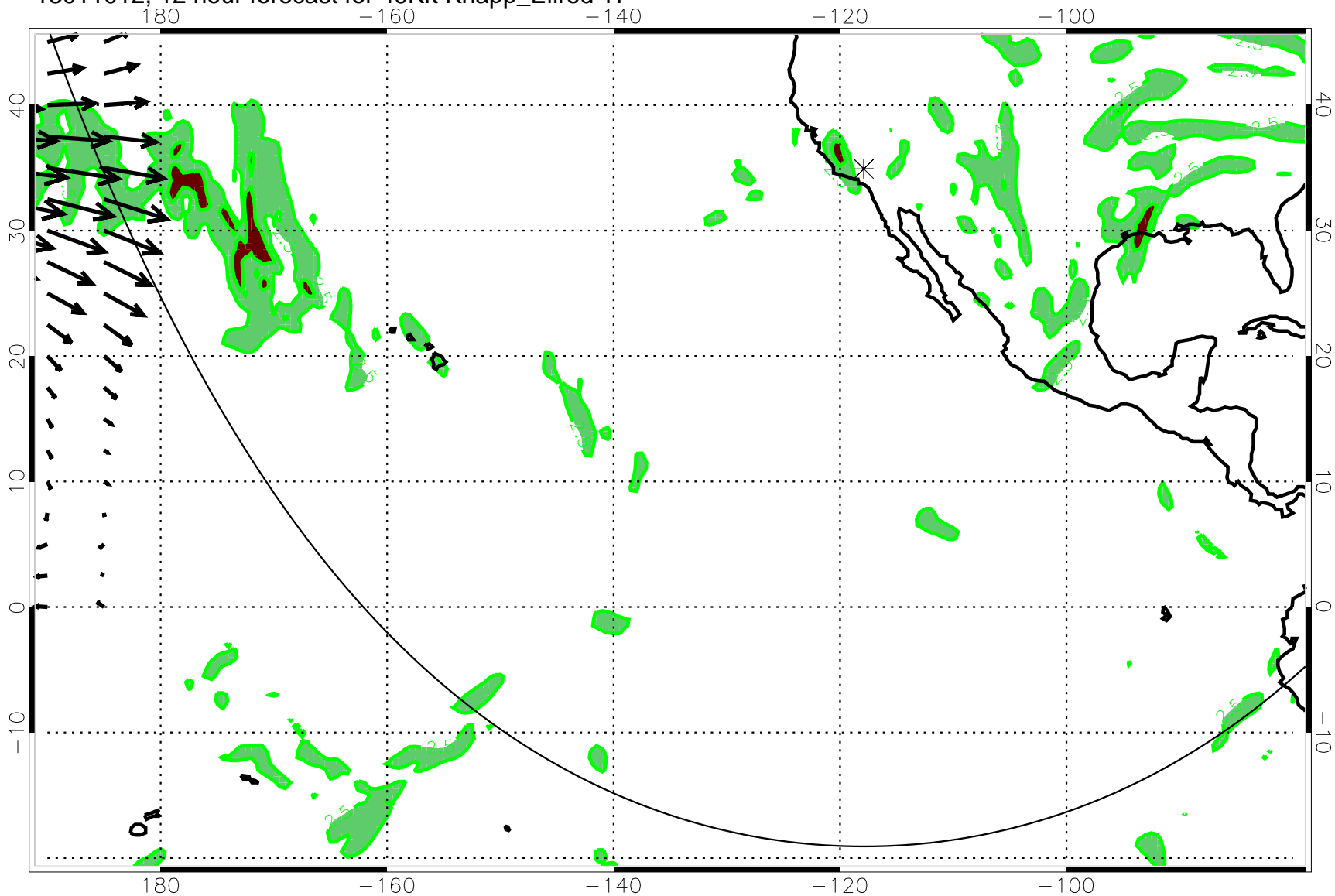
13011012, 12 hour forecast for 49Kft Knapp_Ellrod TI
