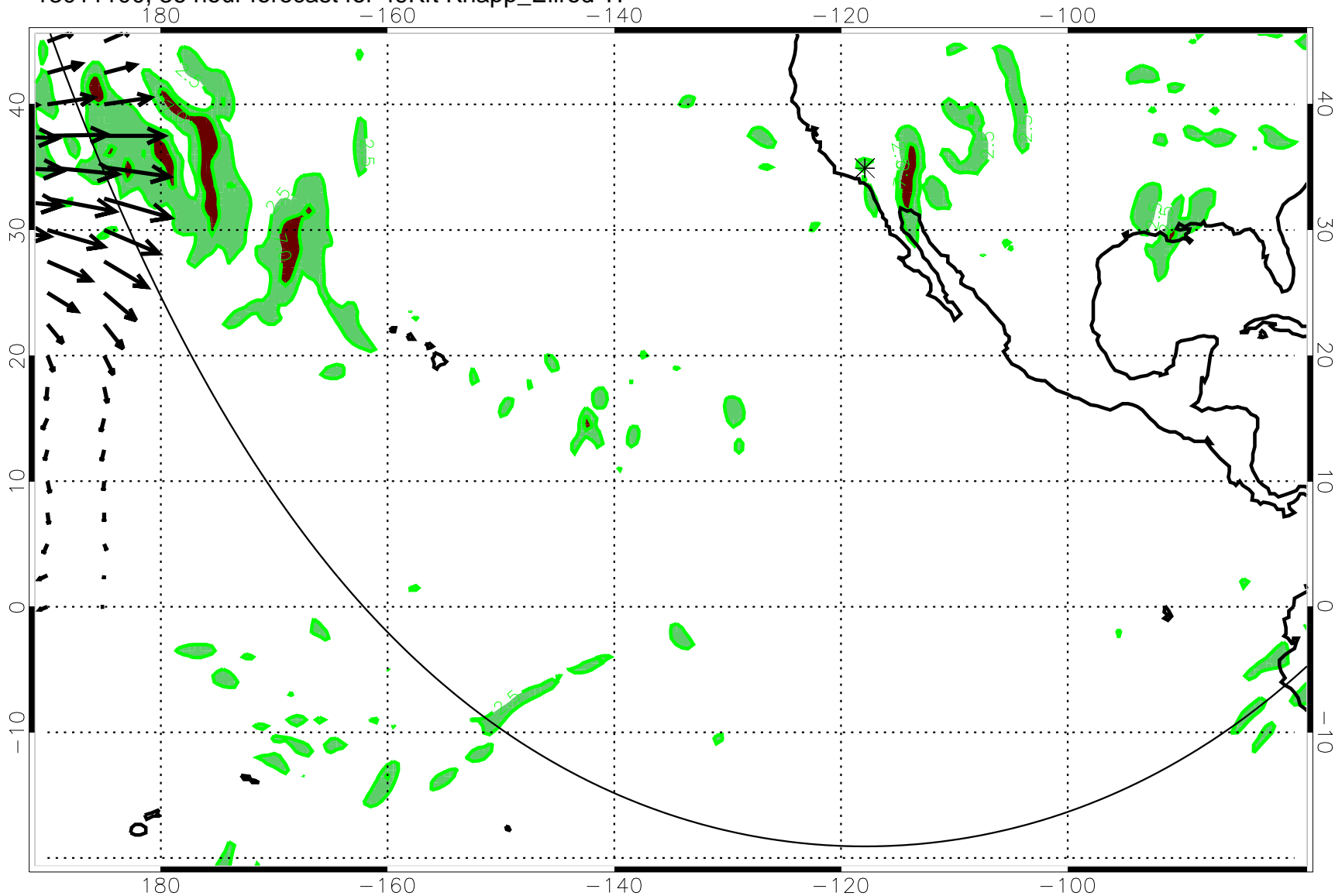
13011100, 36 hour forecast for 49Kft Knapp_Ellrod TI
