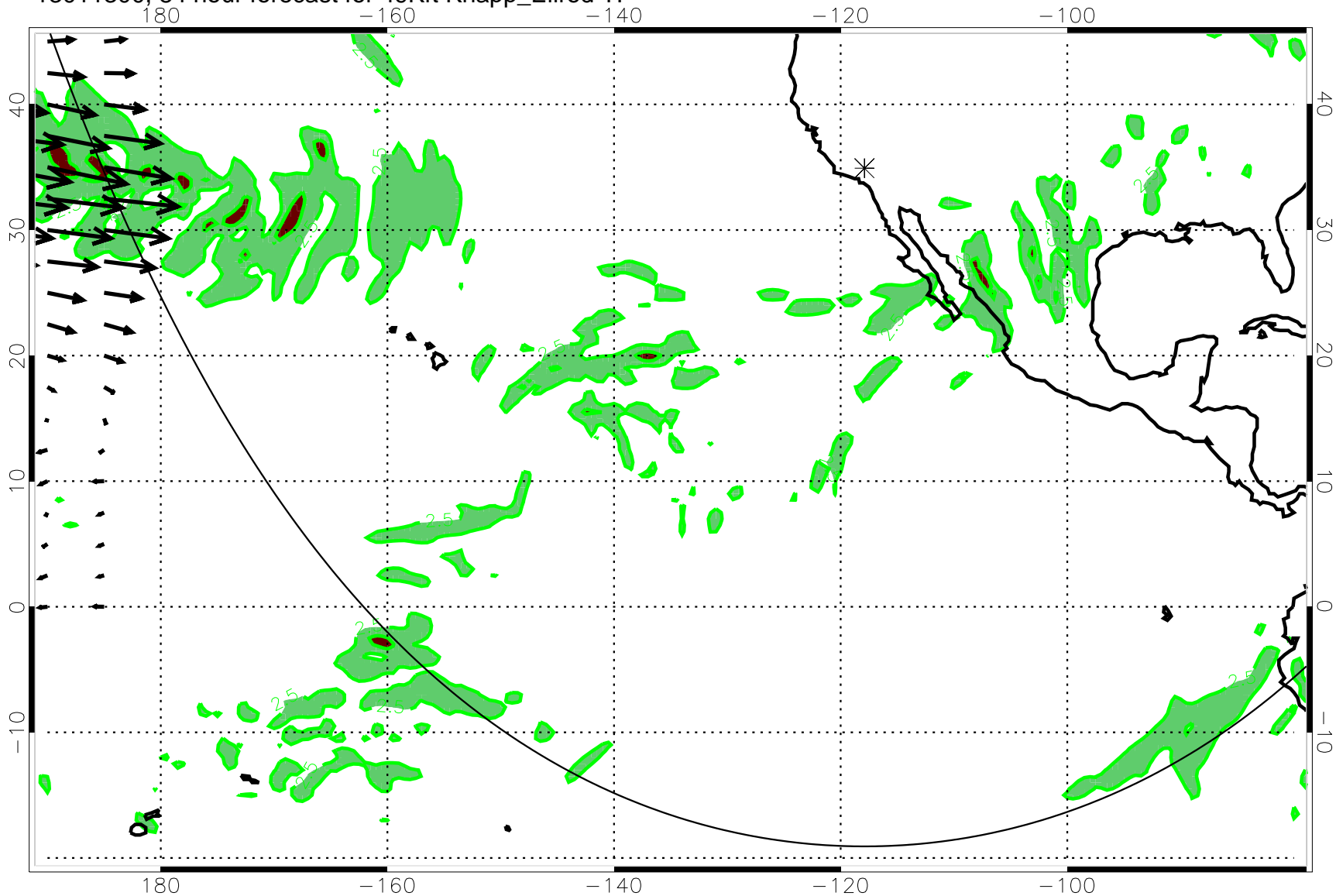
13011300, 84 hour forecast for 49Kft Knapp_Ellrod TI
