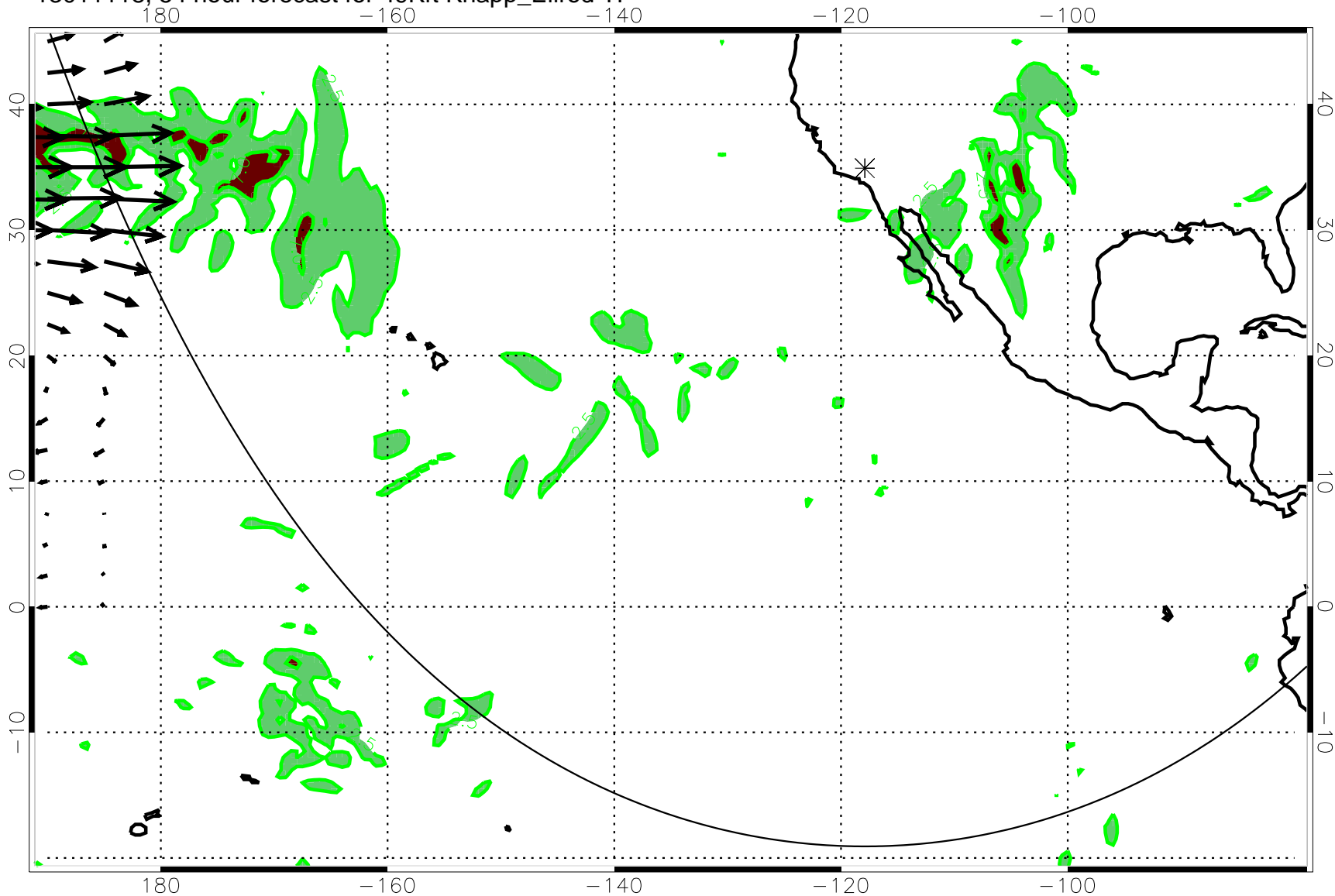
13011118, 54 hour forecast for 49Kft Knapp_Ellrod TI
