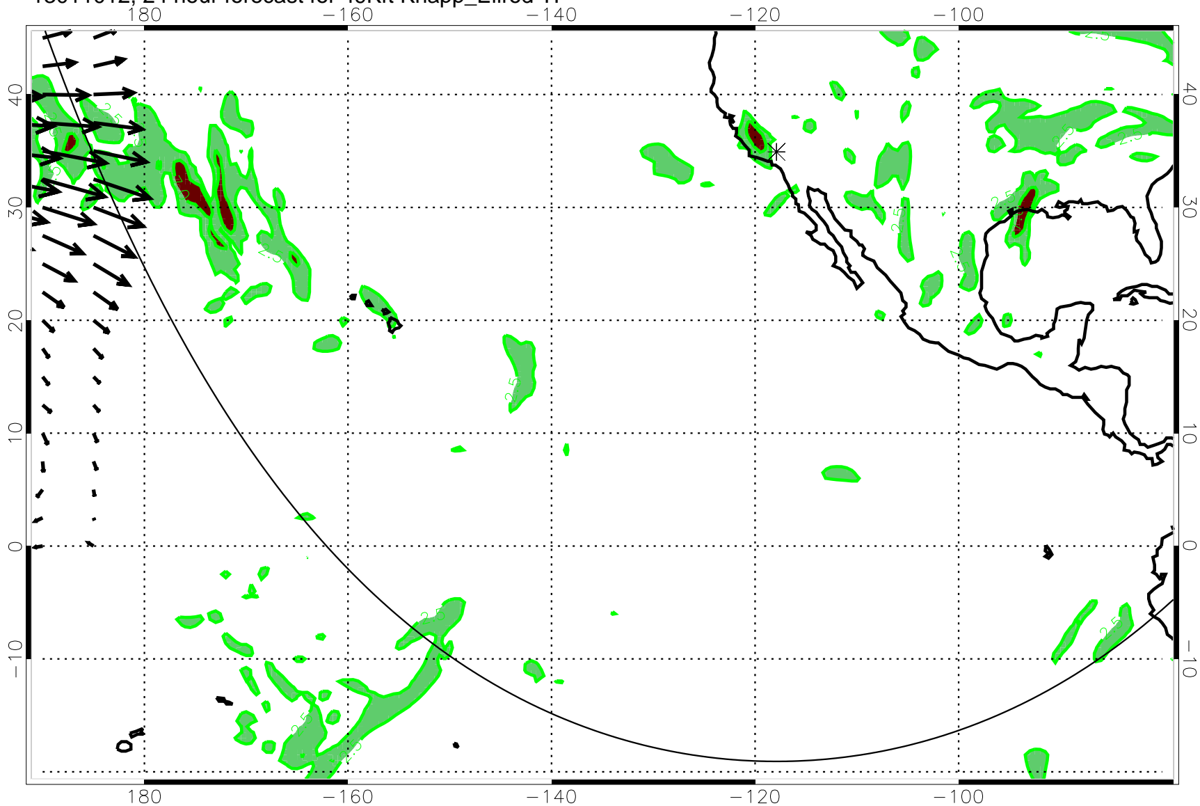
13011012, 24 hour forecast for 49Kft Knapp_Ellrod TI
