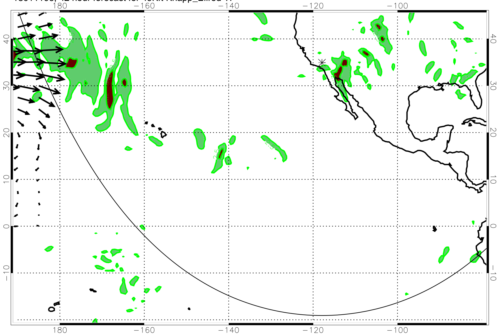
13011106, 42 hour forecast for 49Kft Knapp_Ellrod TI
