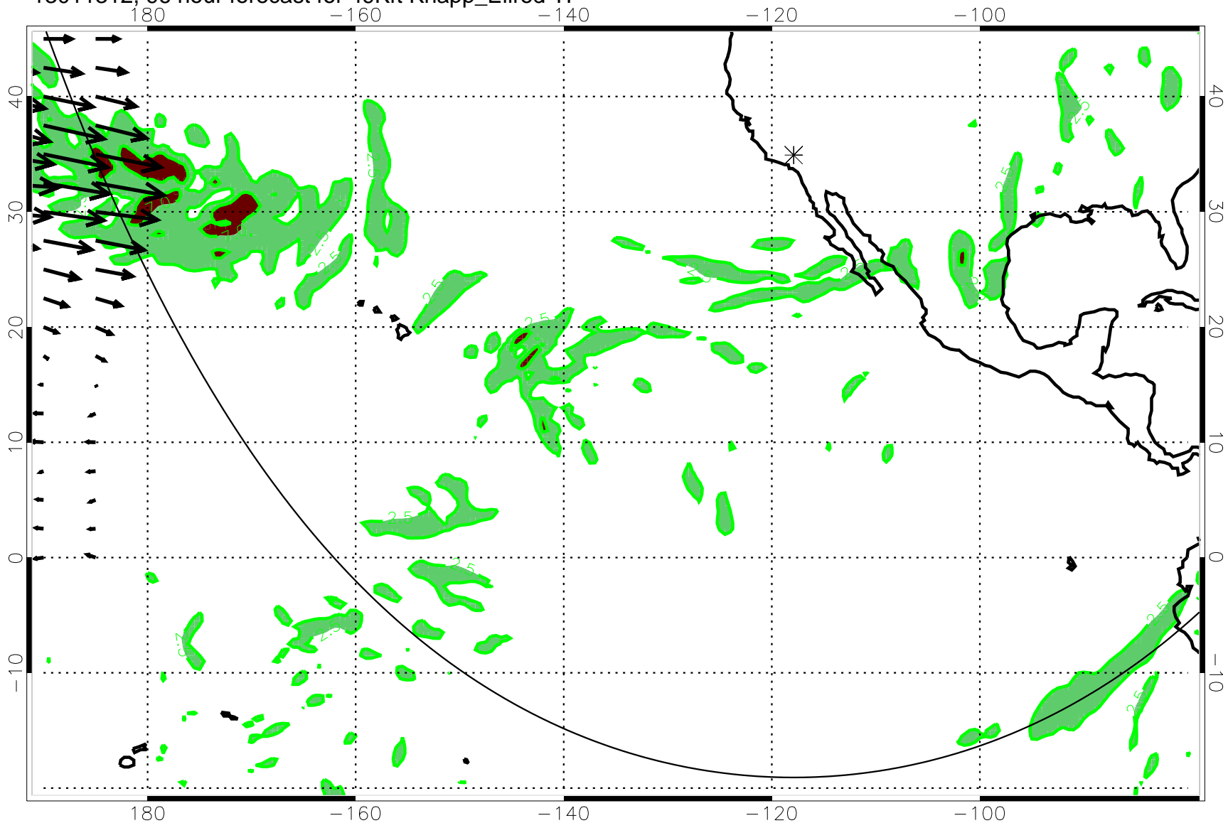
13011312, 96 hour forecast for 49Kft Knapp_Ellrod TI
