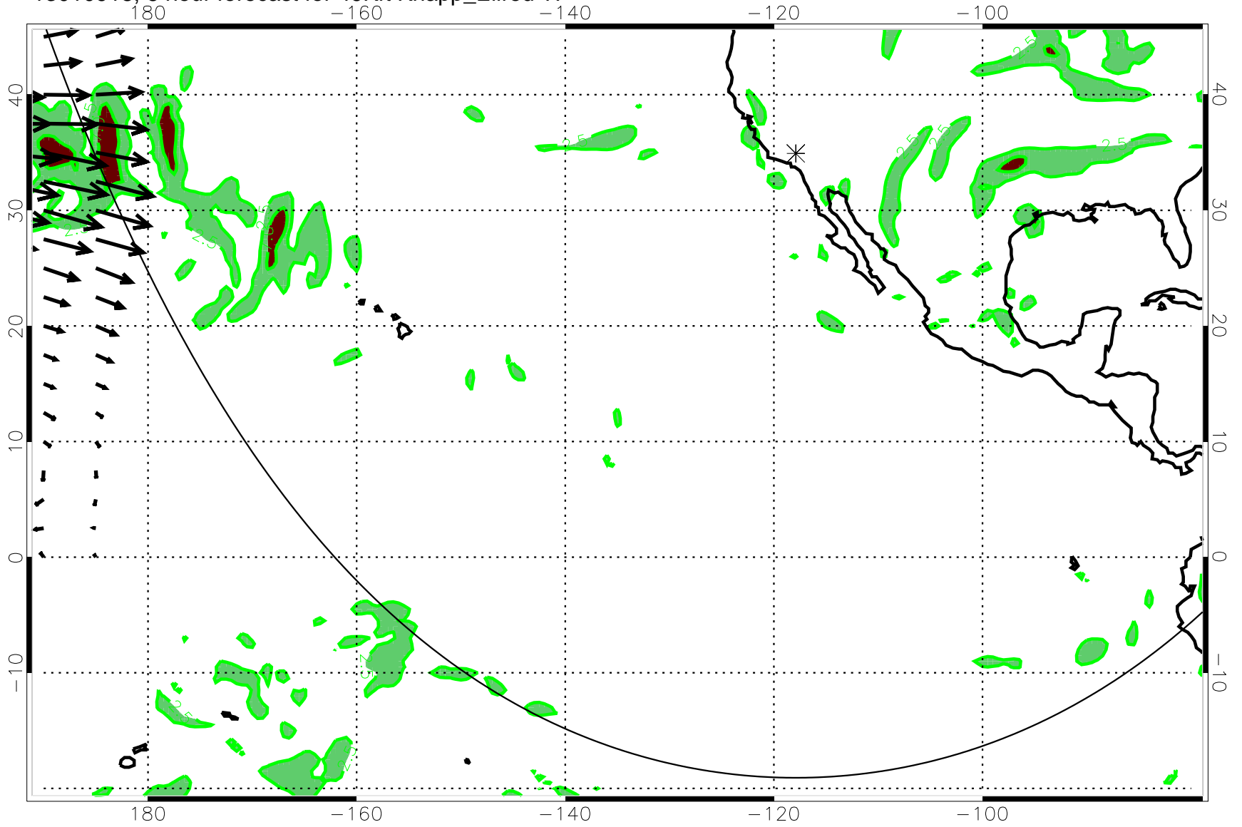
13010918, 6 hour forecast for 49Kft Knapp_Ellrod TI
