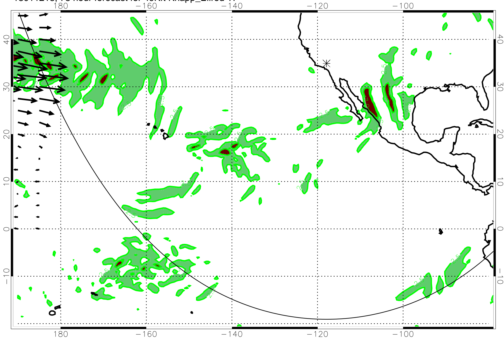
13011218, 78 hour forecast for 49Kft Knapp_Ellrod TI
