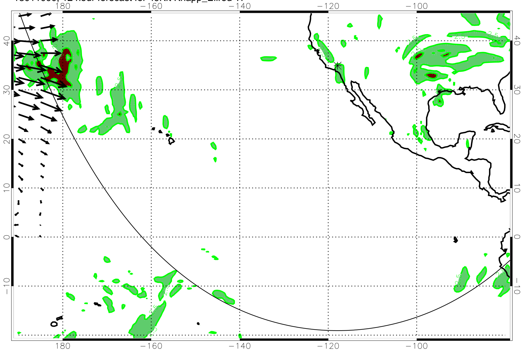
13011000, 12 hour forecast for 49Kft Knapp_Ellrod TI
