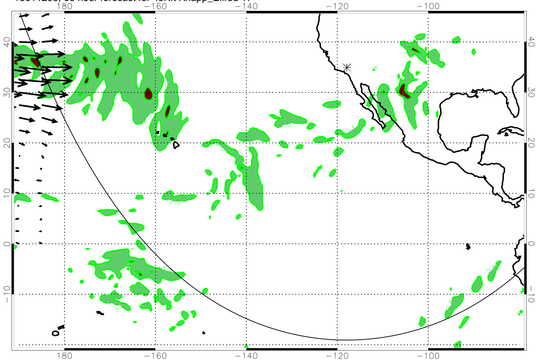
13011206, 66 hour forecast for 49Kft Knapp_Ellrod TI
