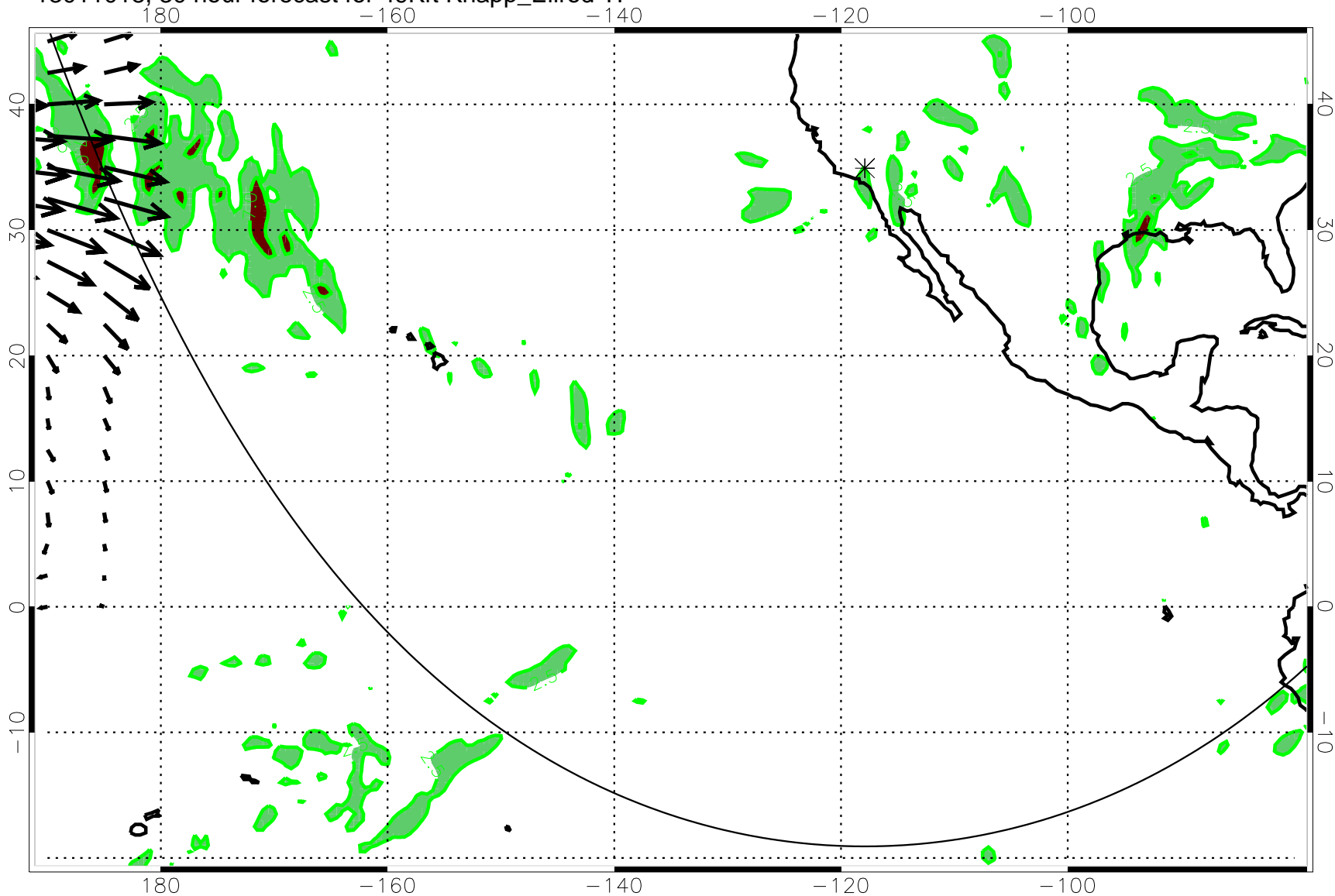
13011018, 30 hour forecast for 49Kft Knapp_Ellrod TI
