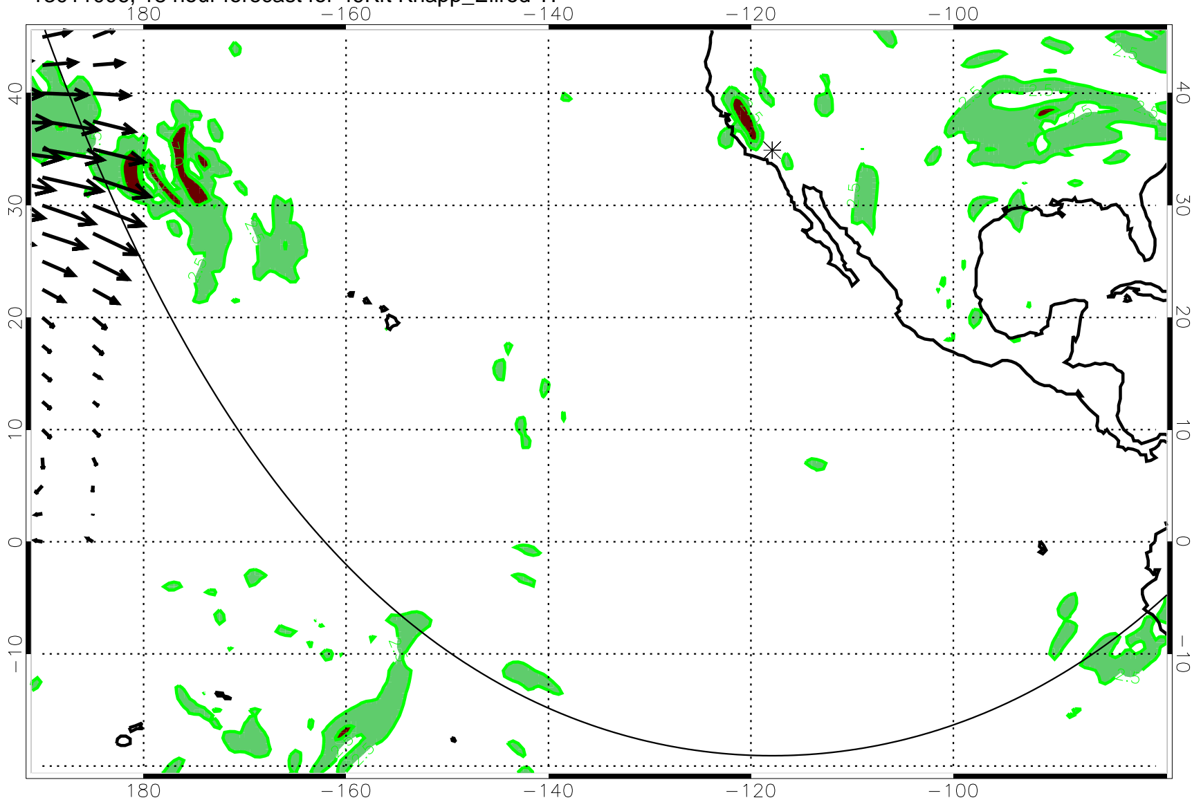
13011006, 18 hour forecast for 49Kft Knapp_Ellrod TI
