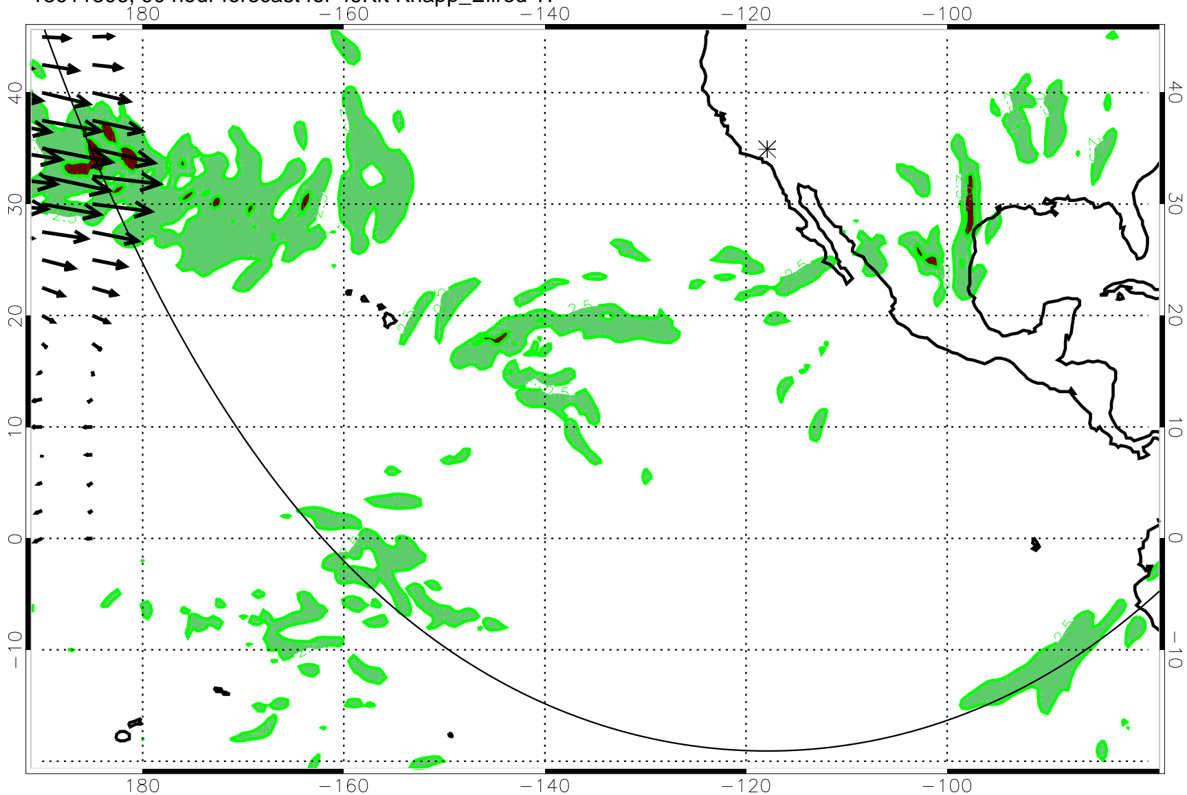
13011306, 90 hour forecast for 49Kft Knapp_Ellrod TI
