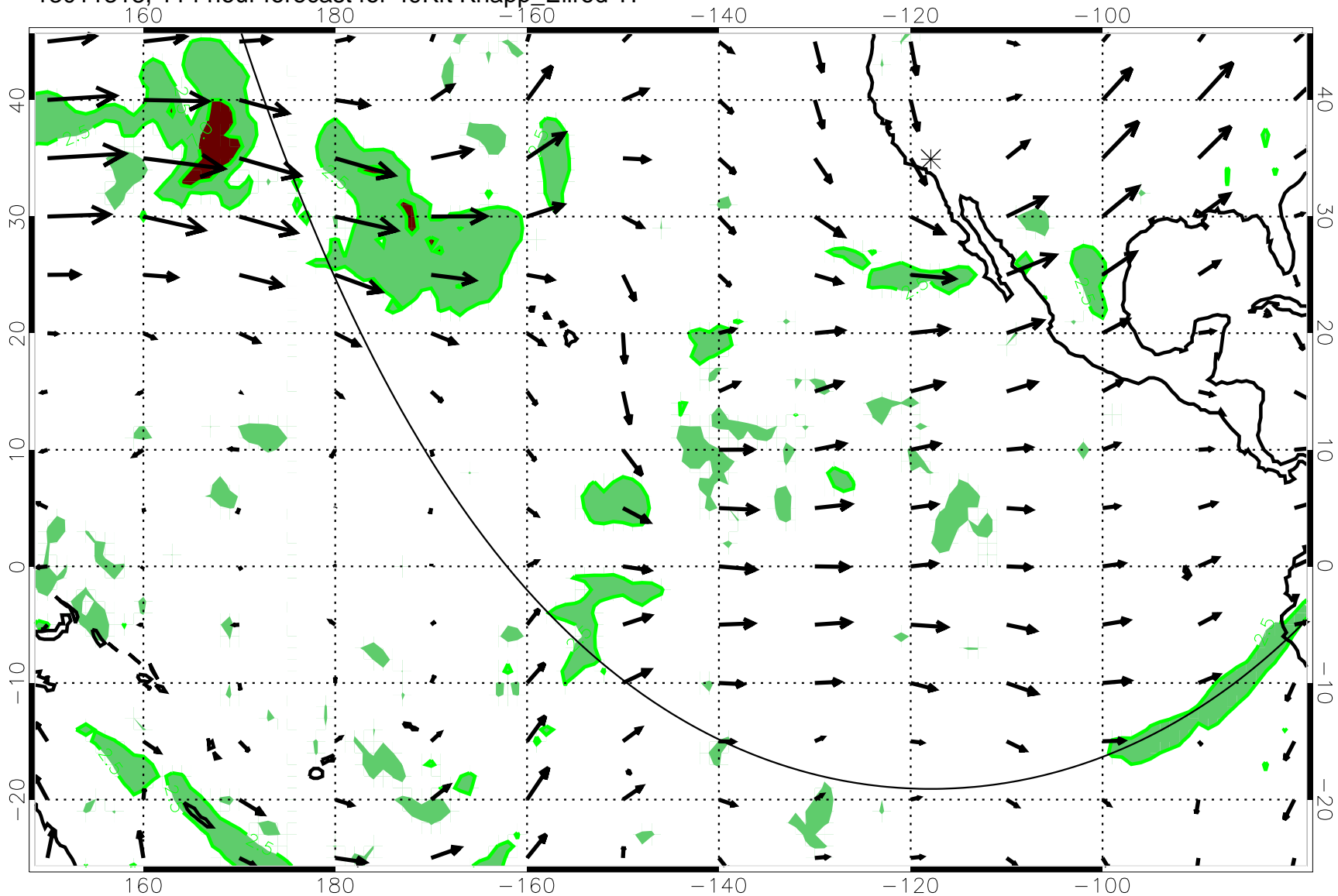
13011318, 114 hour forecast for 49Kft Knapp_Ellrod T1
