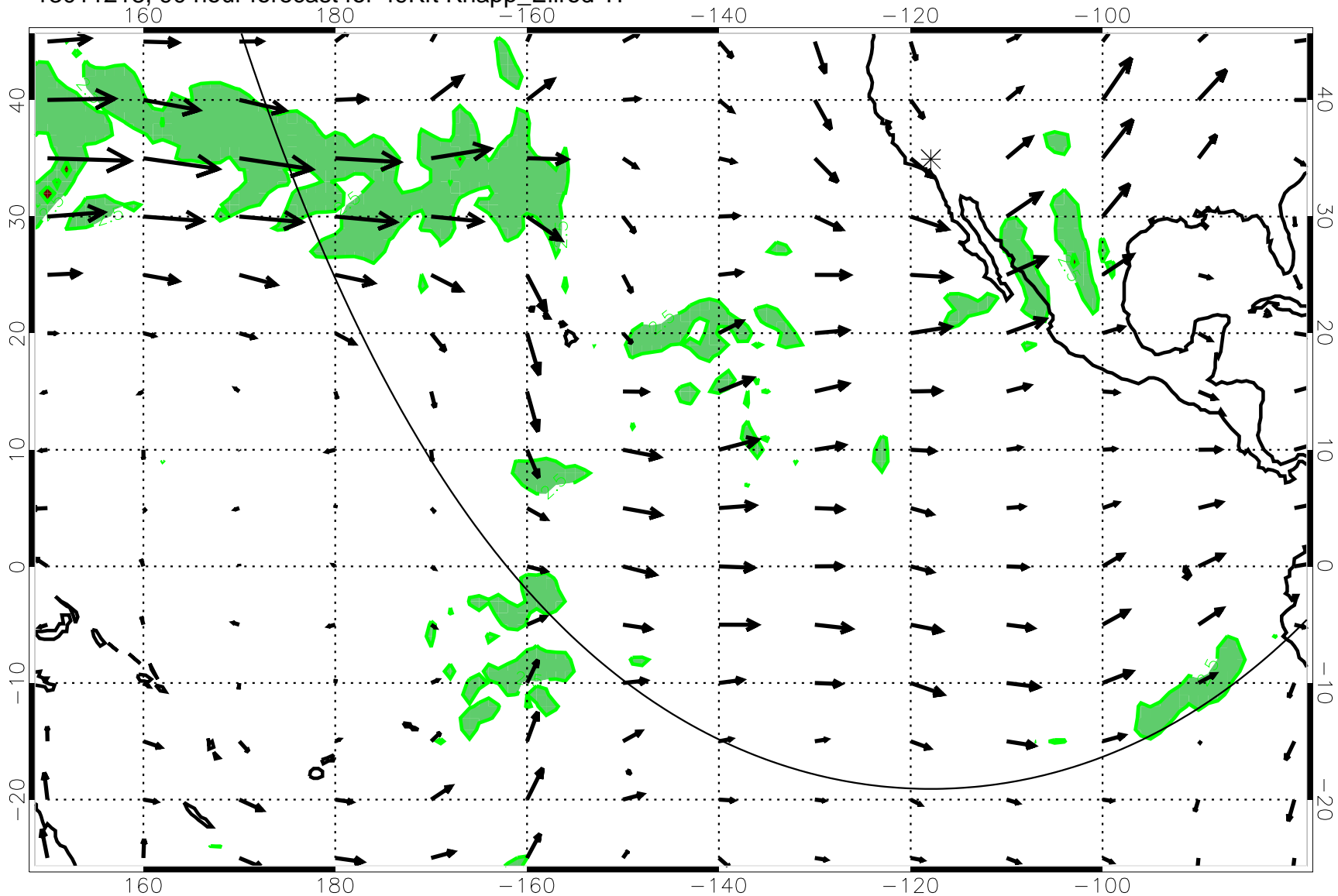
13011218, 90 hour forecast for 49Kft Knapp_Ellrod T1
