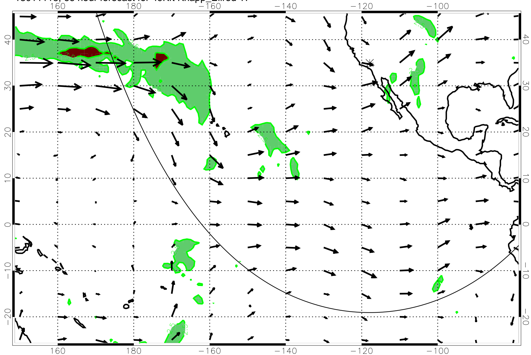
13011118, 66 hour forecast for 49Kft Knapp_Ellrod T1
