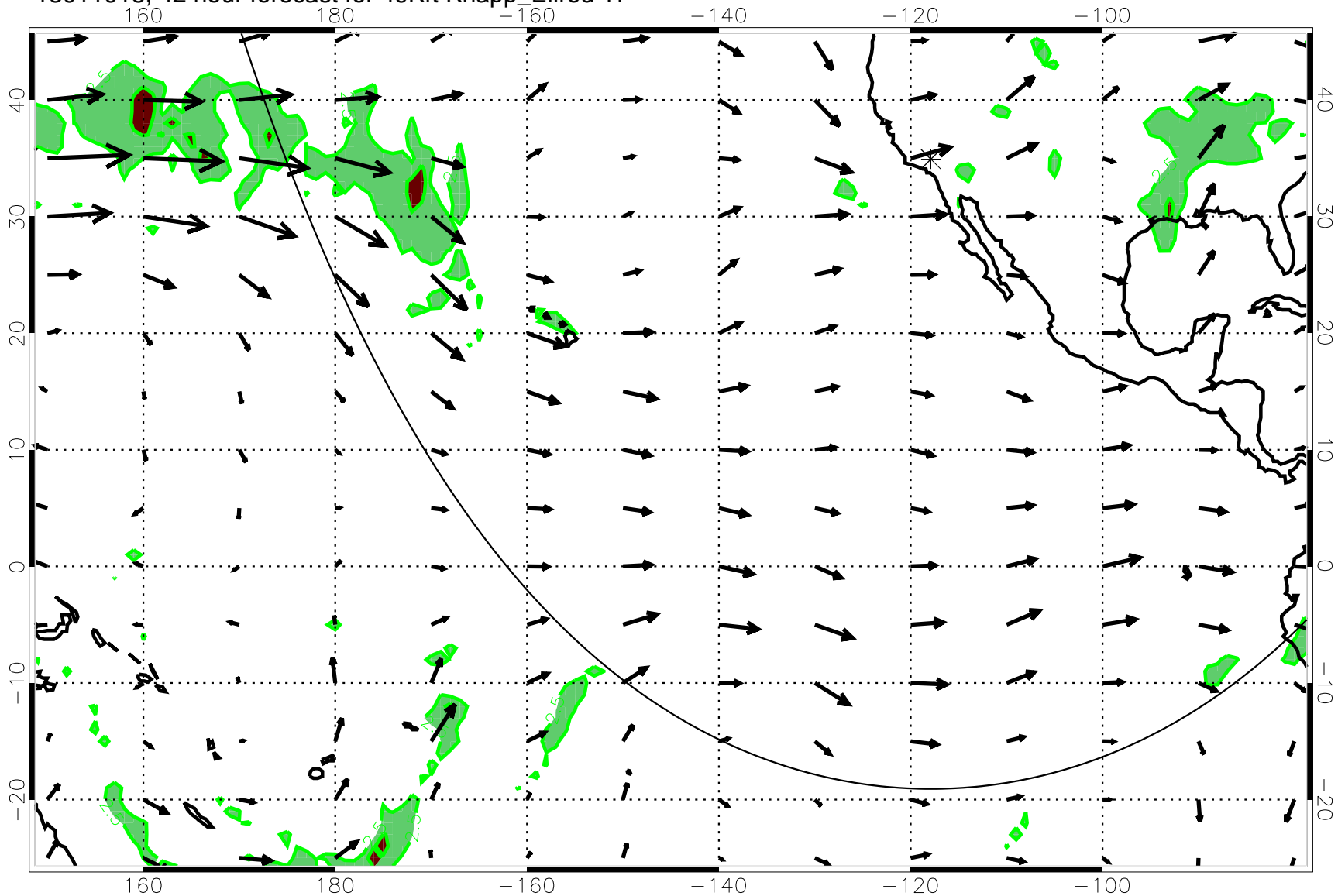
13011018, 42 hour forecast for 49Kft Knapp_Ellrod T1
