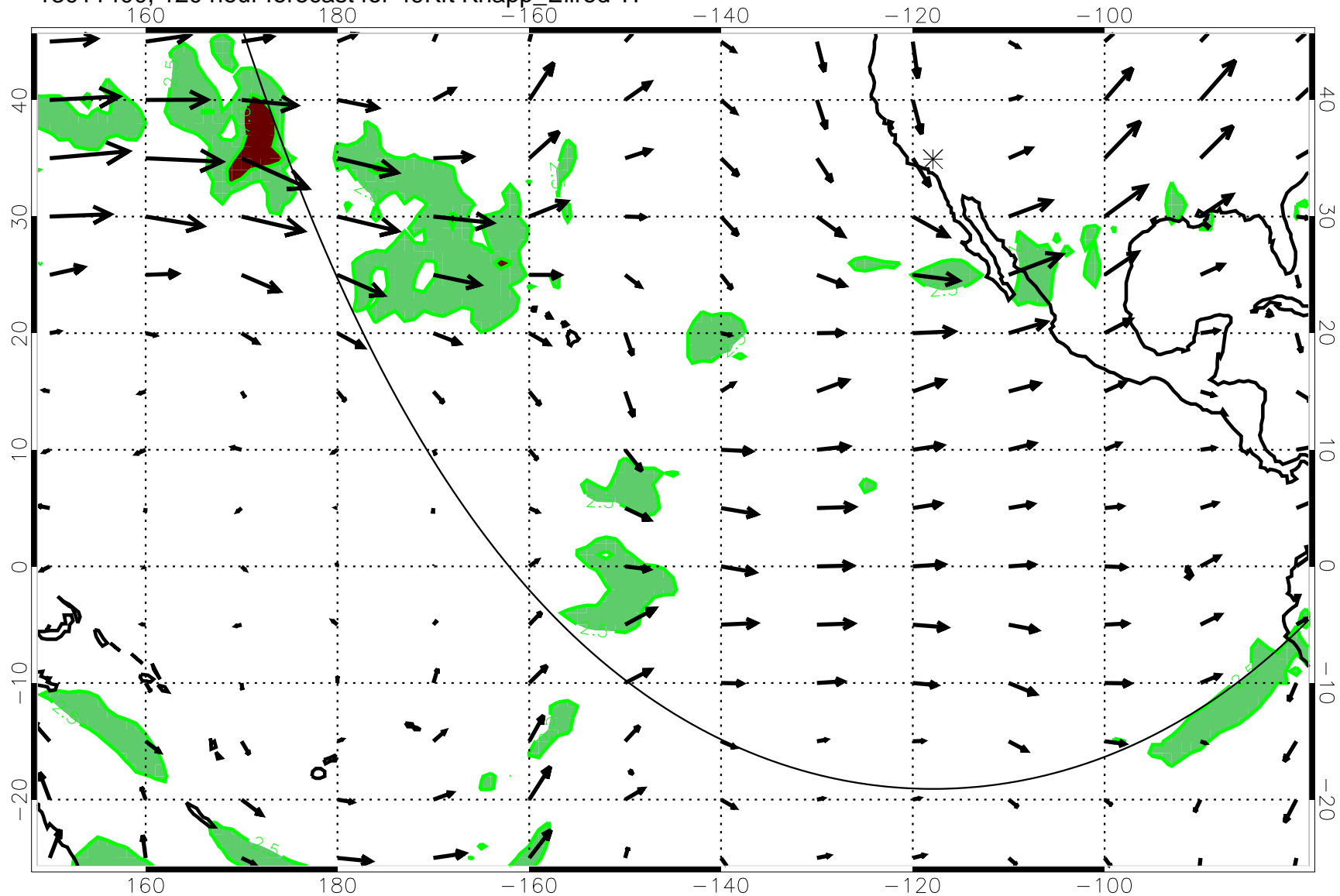
13011400, 120 hour forecast for 49Kft Knapp_Ellrod T1
