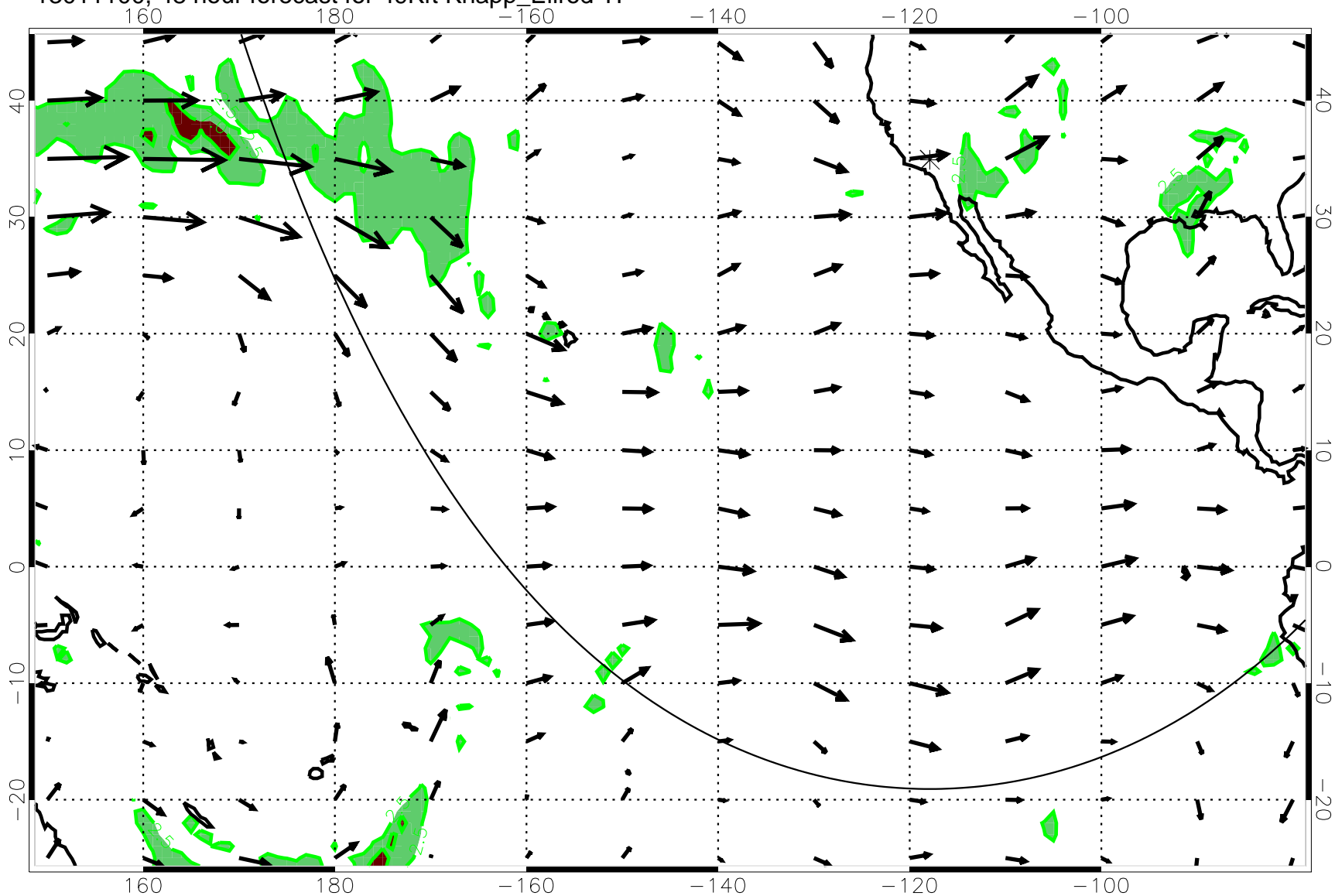
13011100, 48 hour forecast for 49Kft Knapp_Ellrod T1
