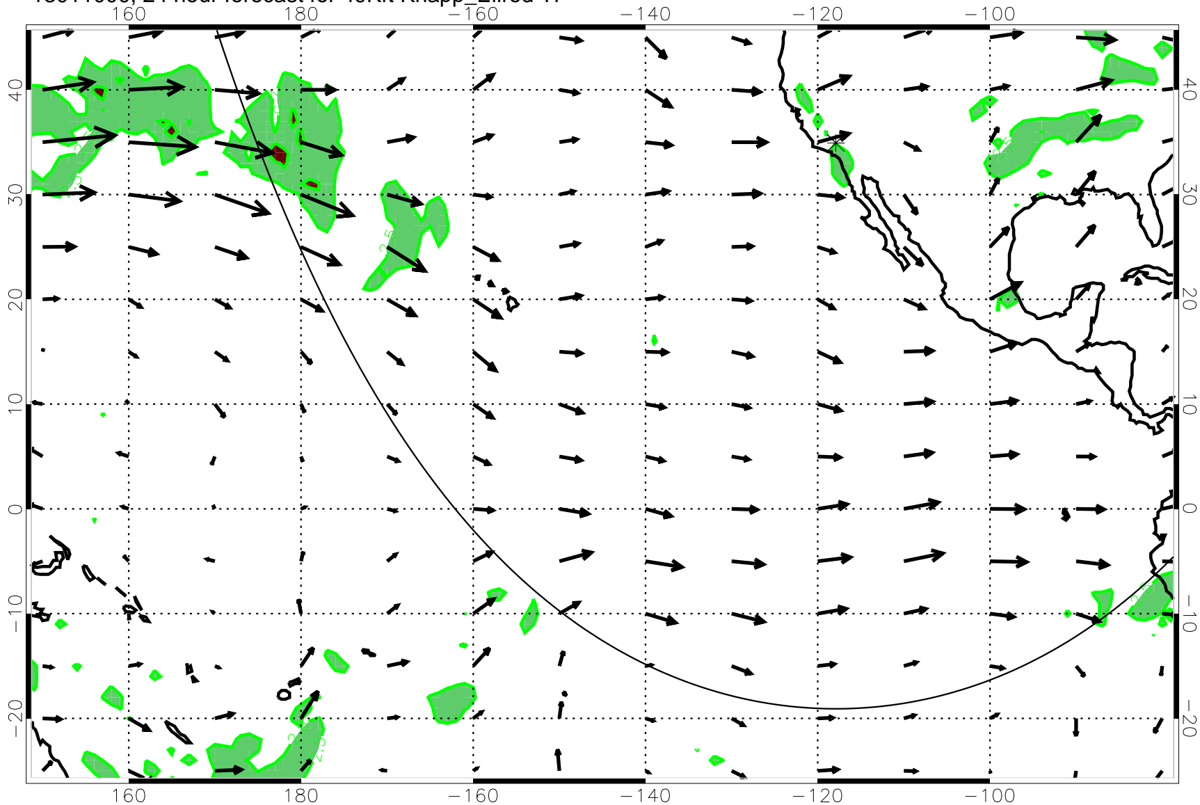
13011000, 24 hour forecast for 49Kft Knapp_Ellrod T1
