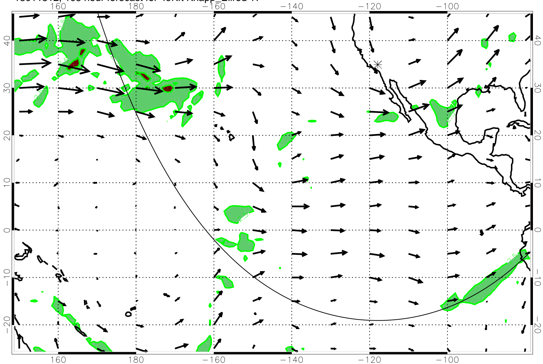
13011312, 108 hour forecast for 49Kft Knapp_Ellrod T1
