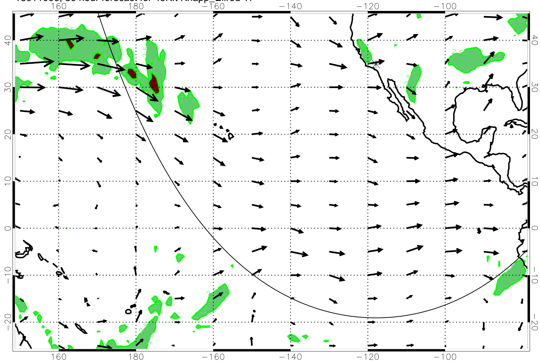
13011006, 30 hour forecast for 49Kft Knapp_Ellrod T1
