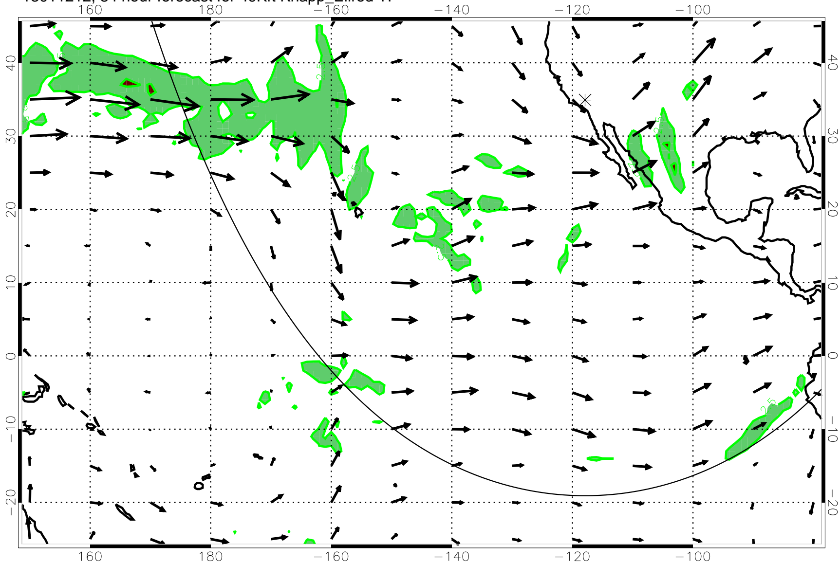
13011212, 84 hour forecast for 49Kft Knapp_Ellrod TI
