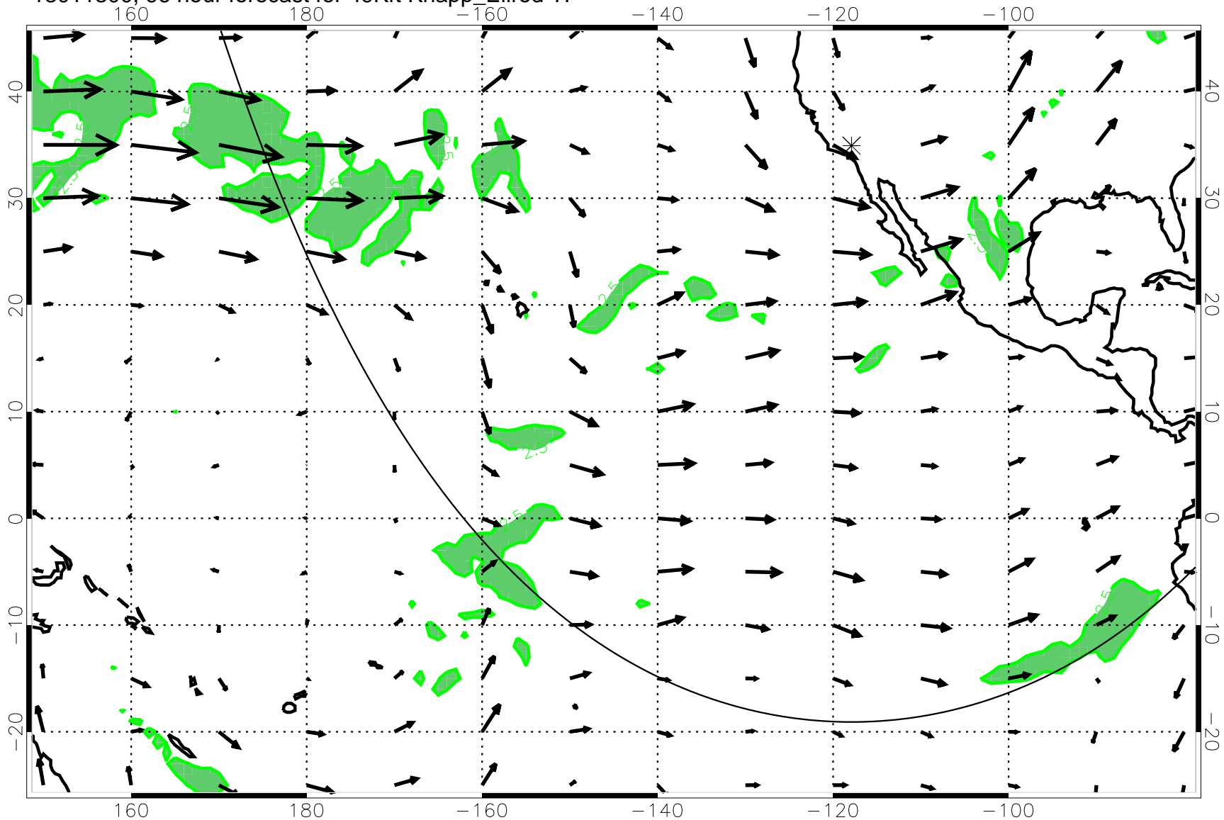
13011300, 96 hour forecast for 49Kft Knapp_Ellrod TI
