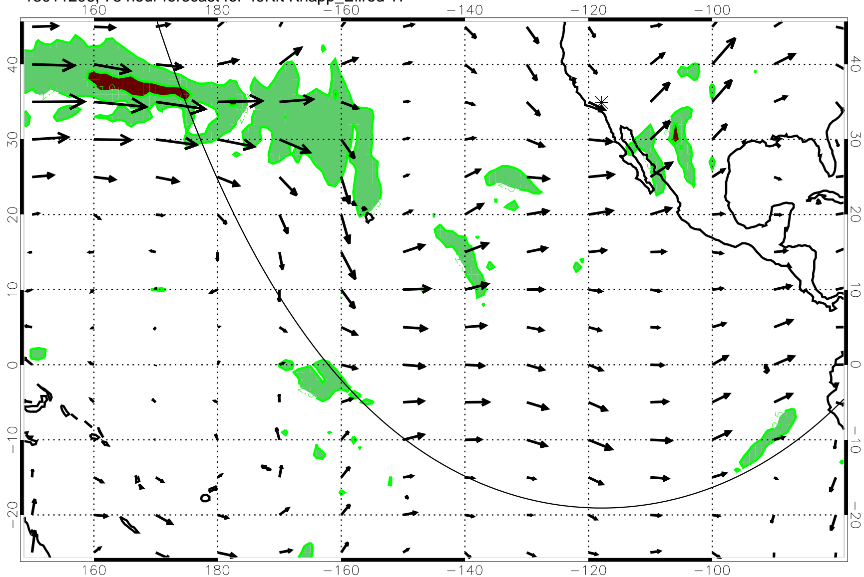
13011206, 78 hour forecast for 49Kft Knapp_Ellrod T1
