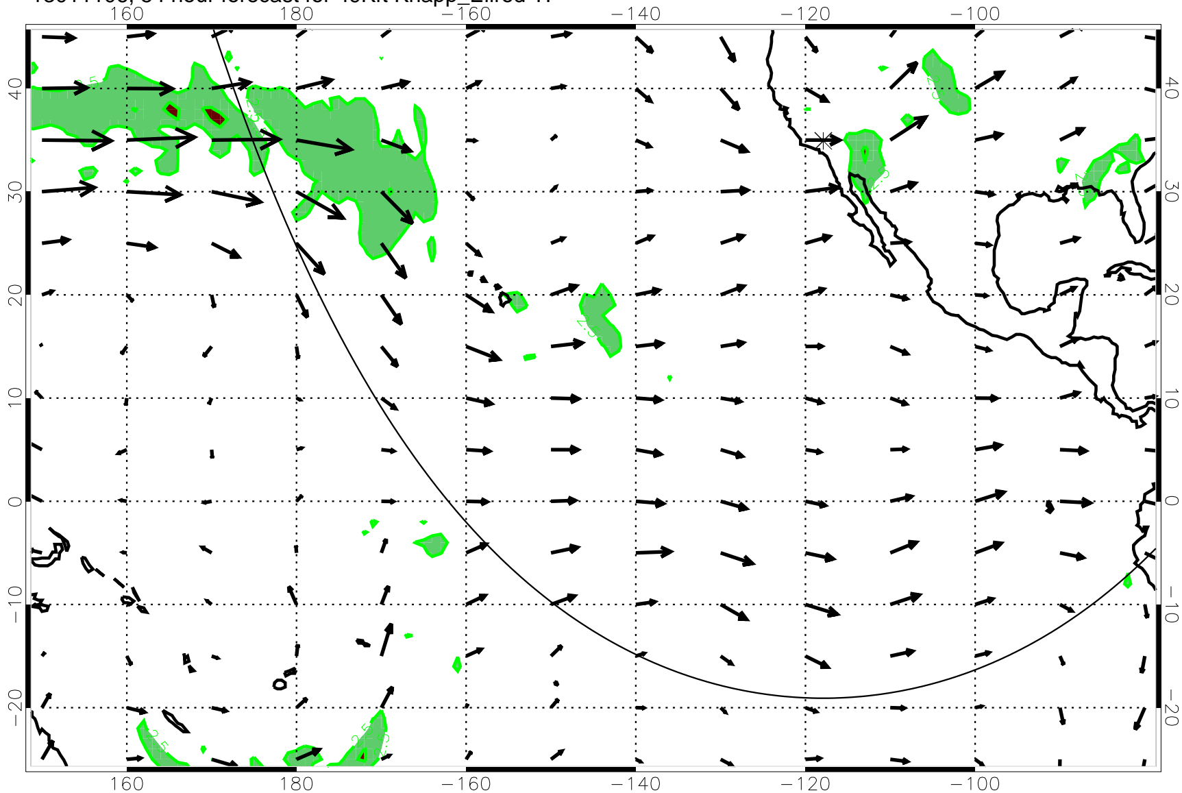
13011106, 54 hour forecast for 49Kft Knapp_Ellrod T1
