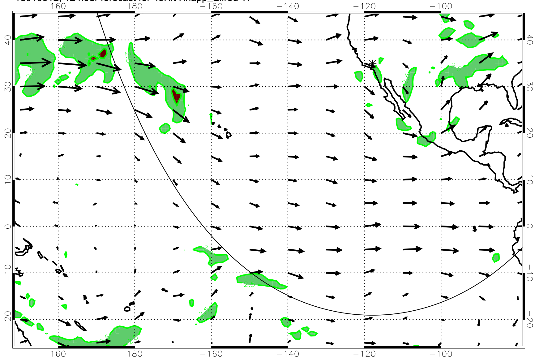
13010912, 12 hour forecast for 49Kft Knapp_Ellrod T1
