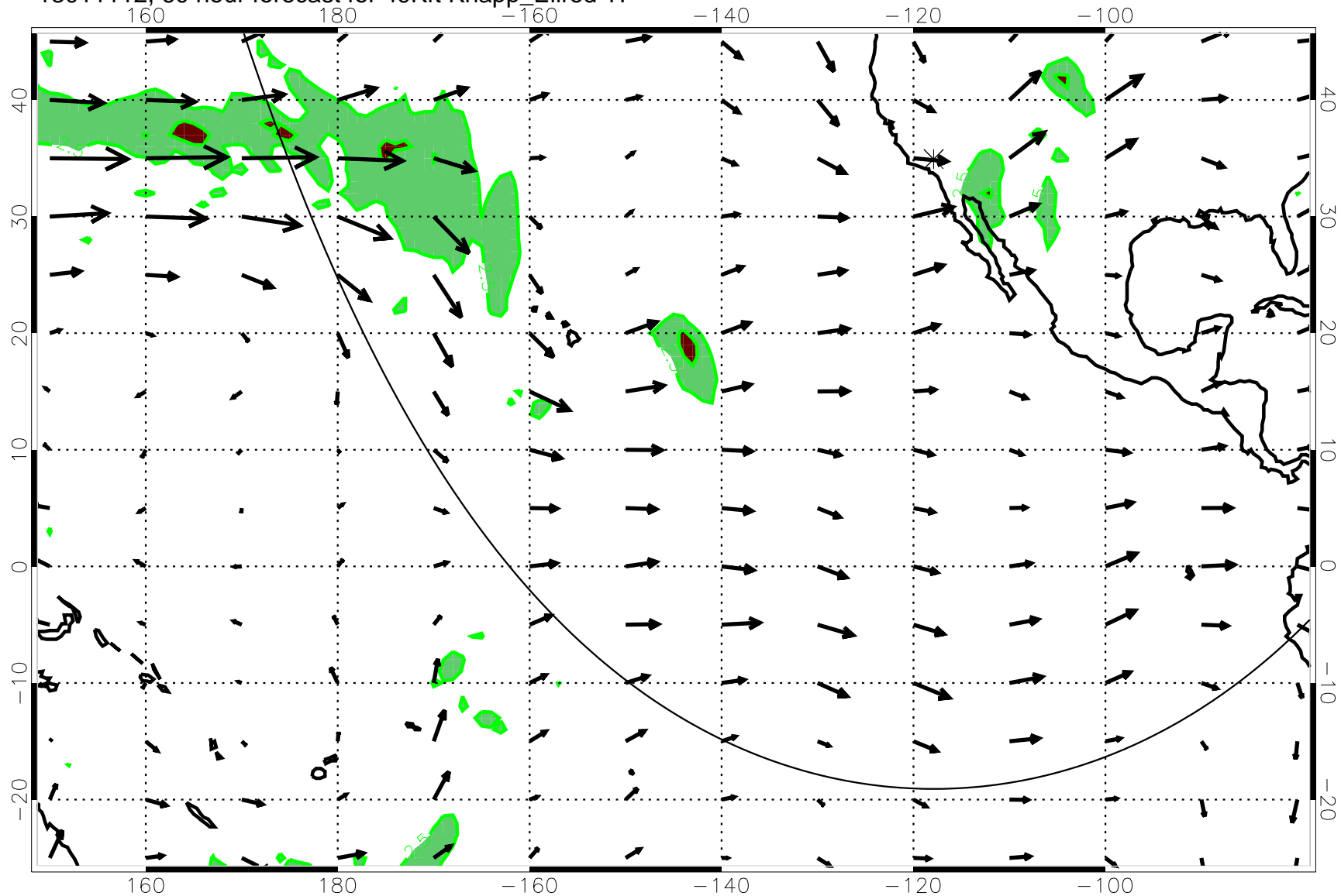
13011112, 60 hour forecast for 49Kft Knapp_Ellrod T1
