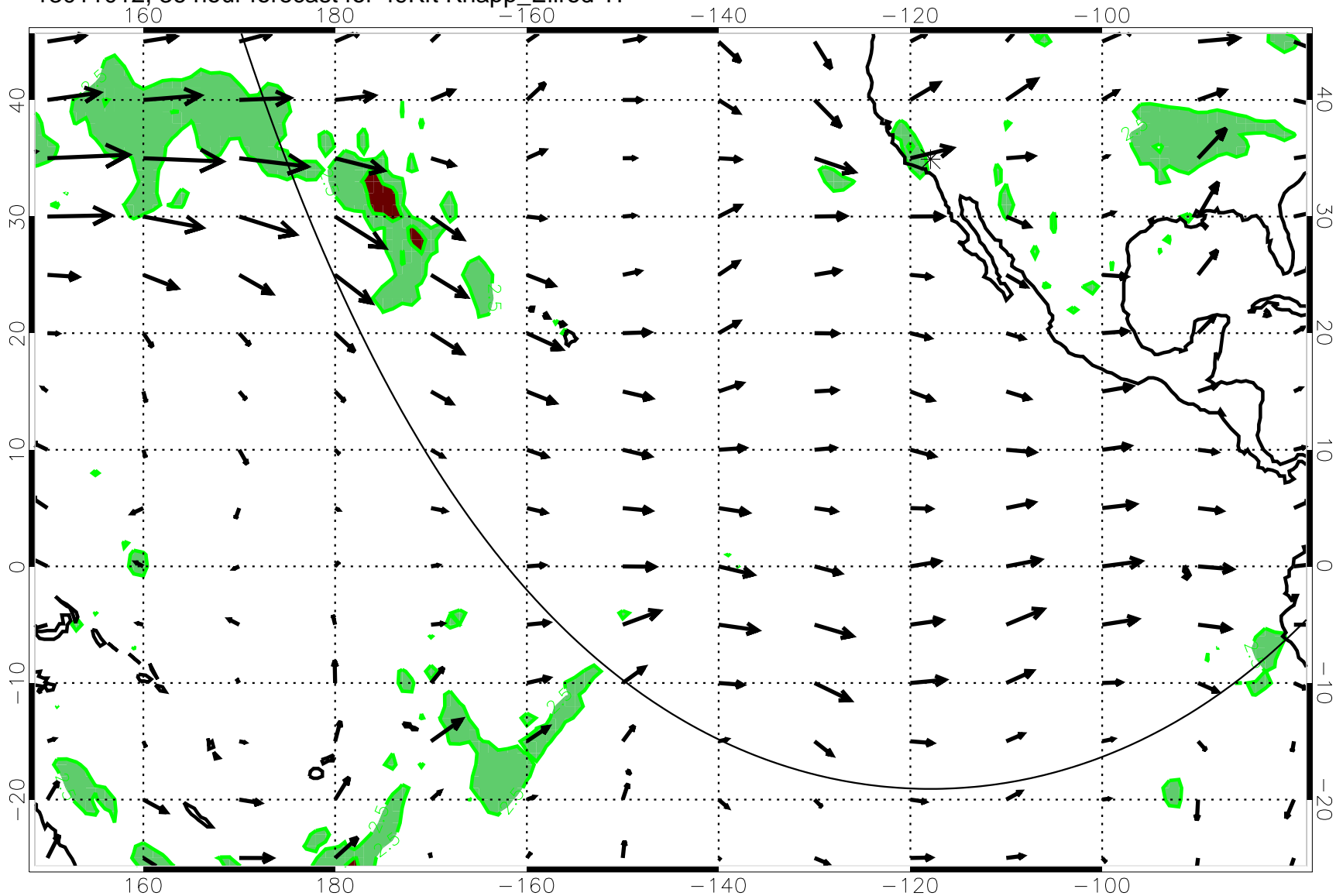
13011012, 36 hour forecast for 49Kft Knapp_Ellrod T1
