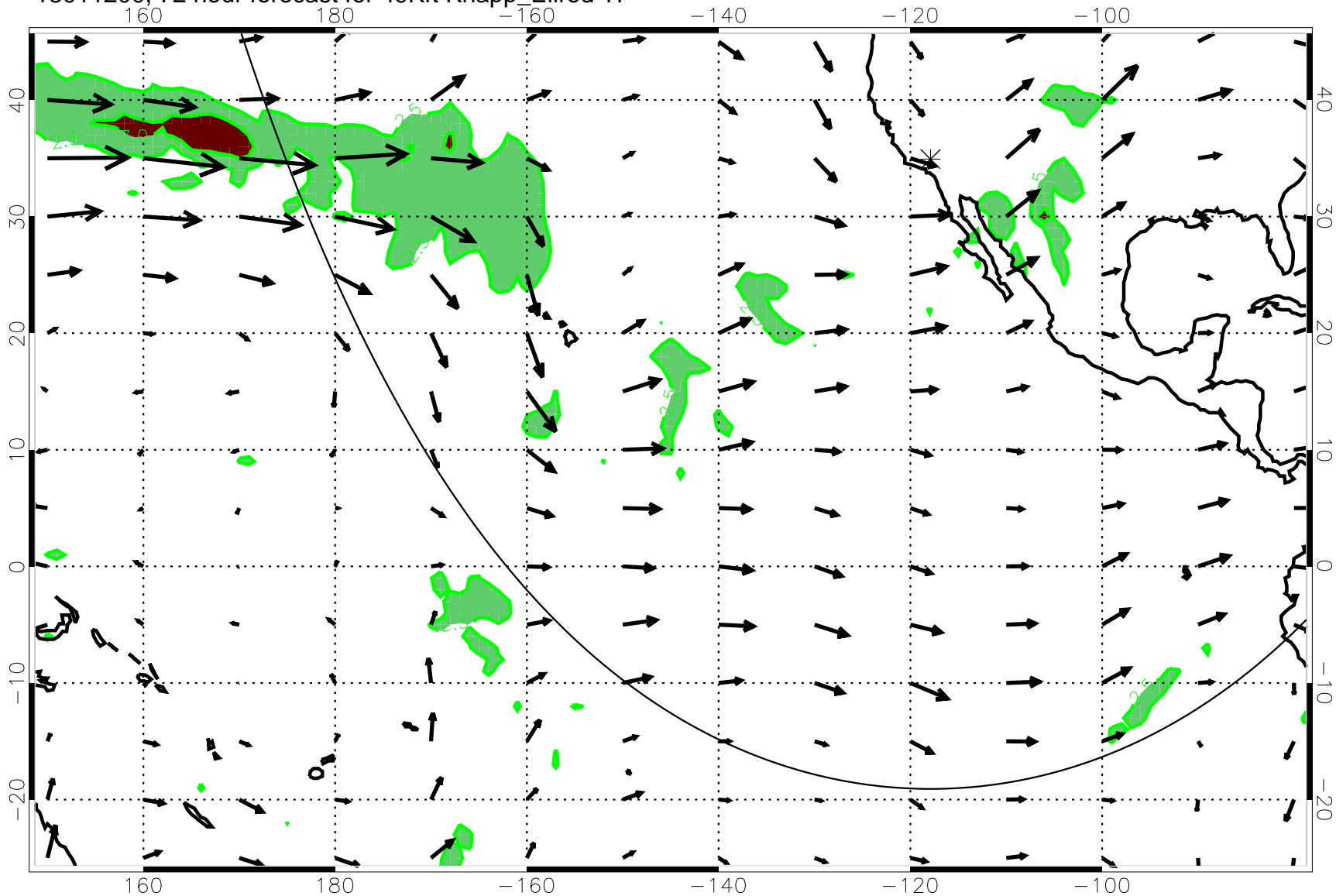
13011200, 72 hour forecast for 49Kft Knapp_Ellrod T1
