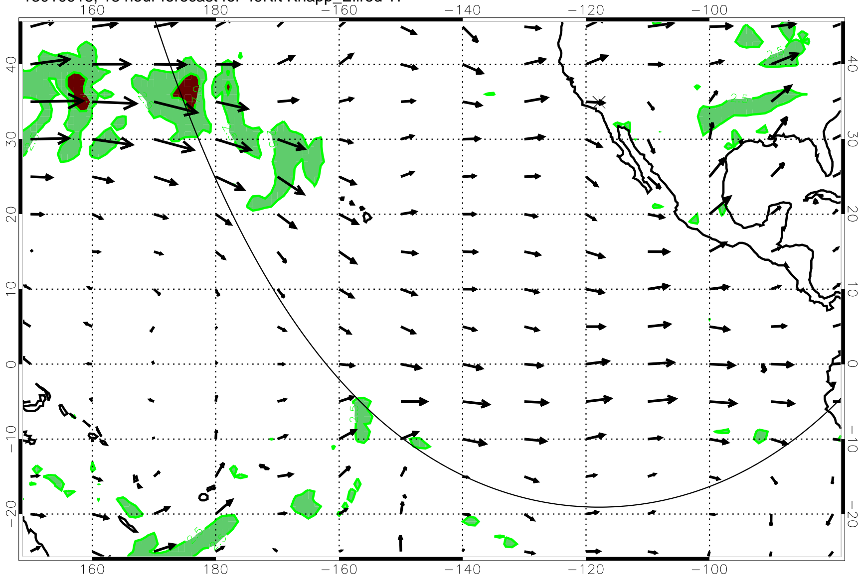
13010918, 18 hour forecast for 49Kft Knapp_Ellrod Tl
