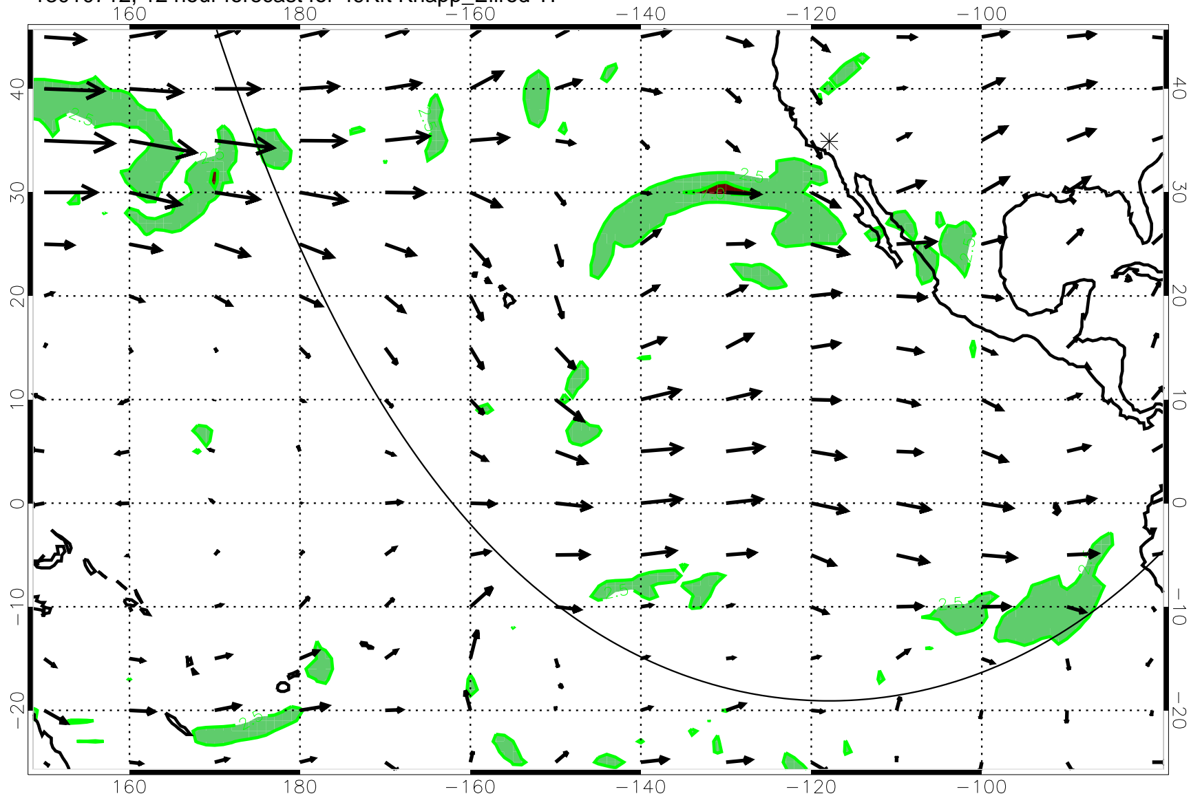
13010712, 12 hour forecast for 49Kft Knapp_Ellrod T1
