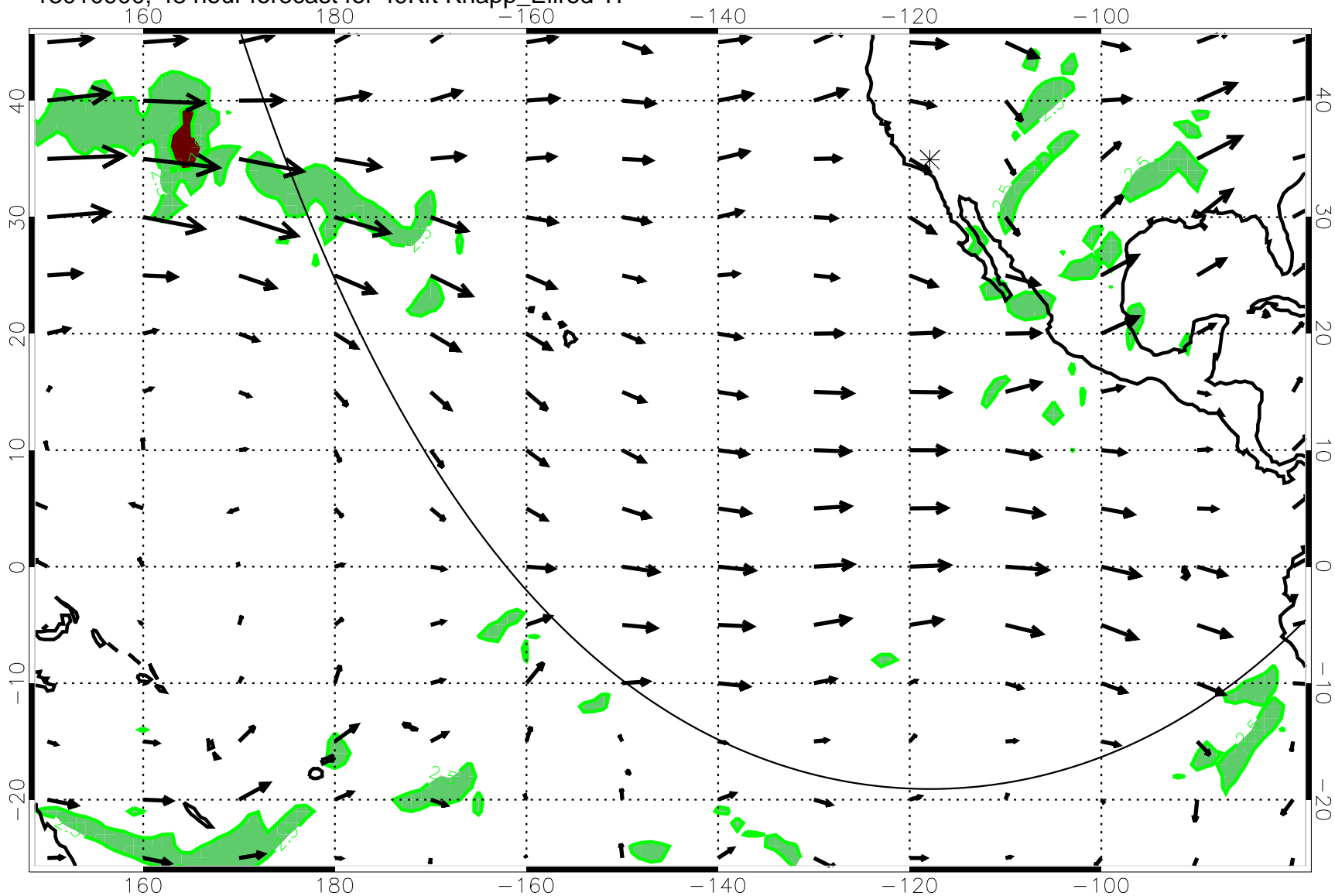
13010900, 48 hour forecast for 49Kft Knapp_Ellrod Tl
