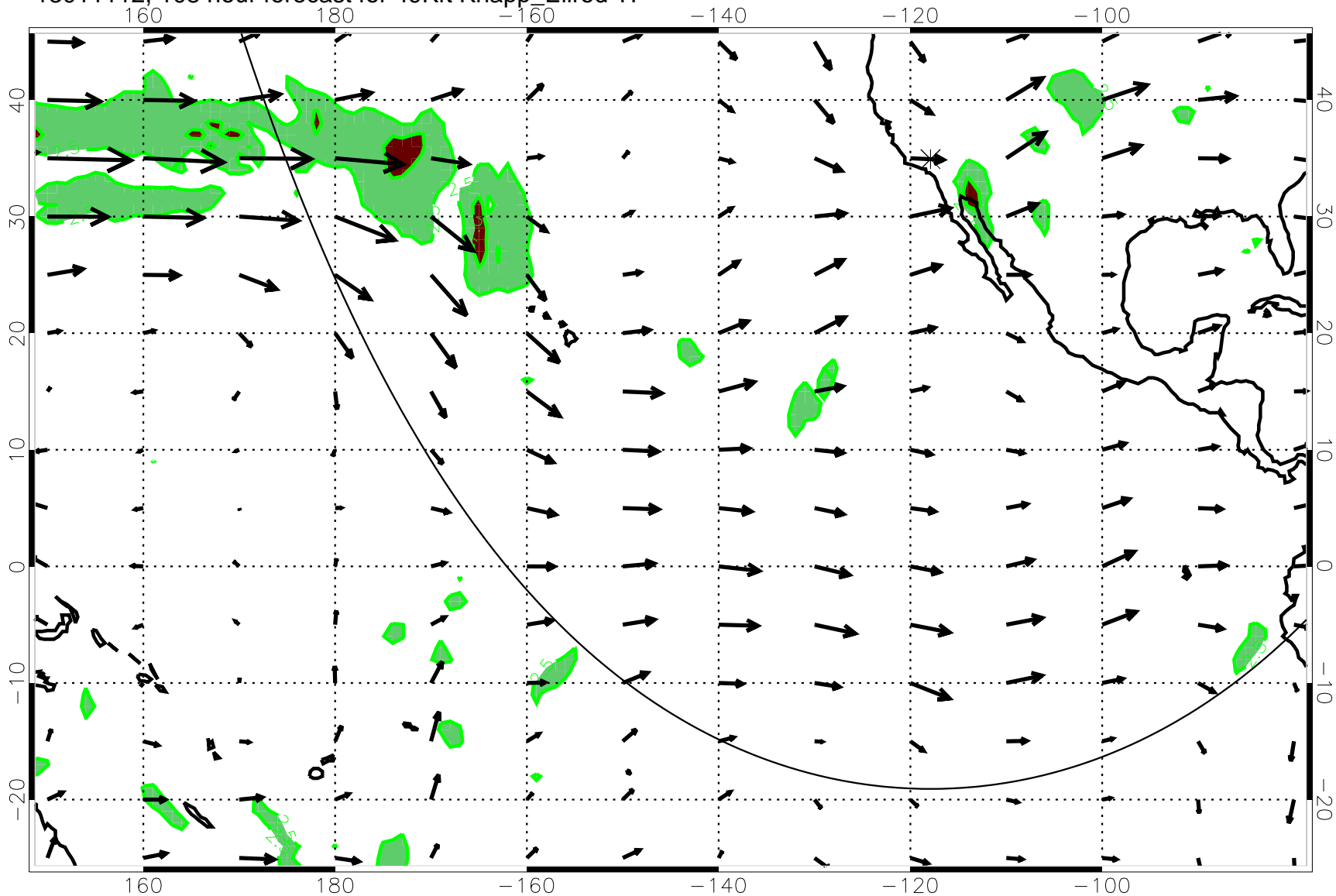
13011112, 108 hour forecast for 49Kft Knapp_Ellrod T1
