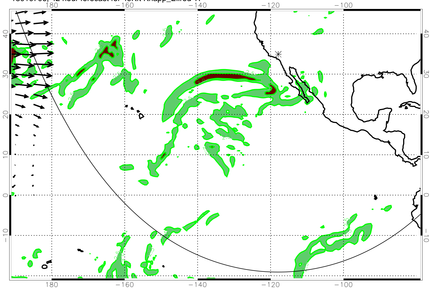
13010706, 42 hour forecast for 49Kft Knapp_Ellrod TI
