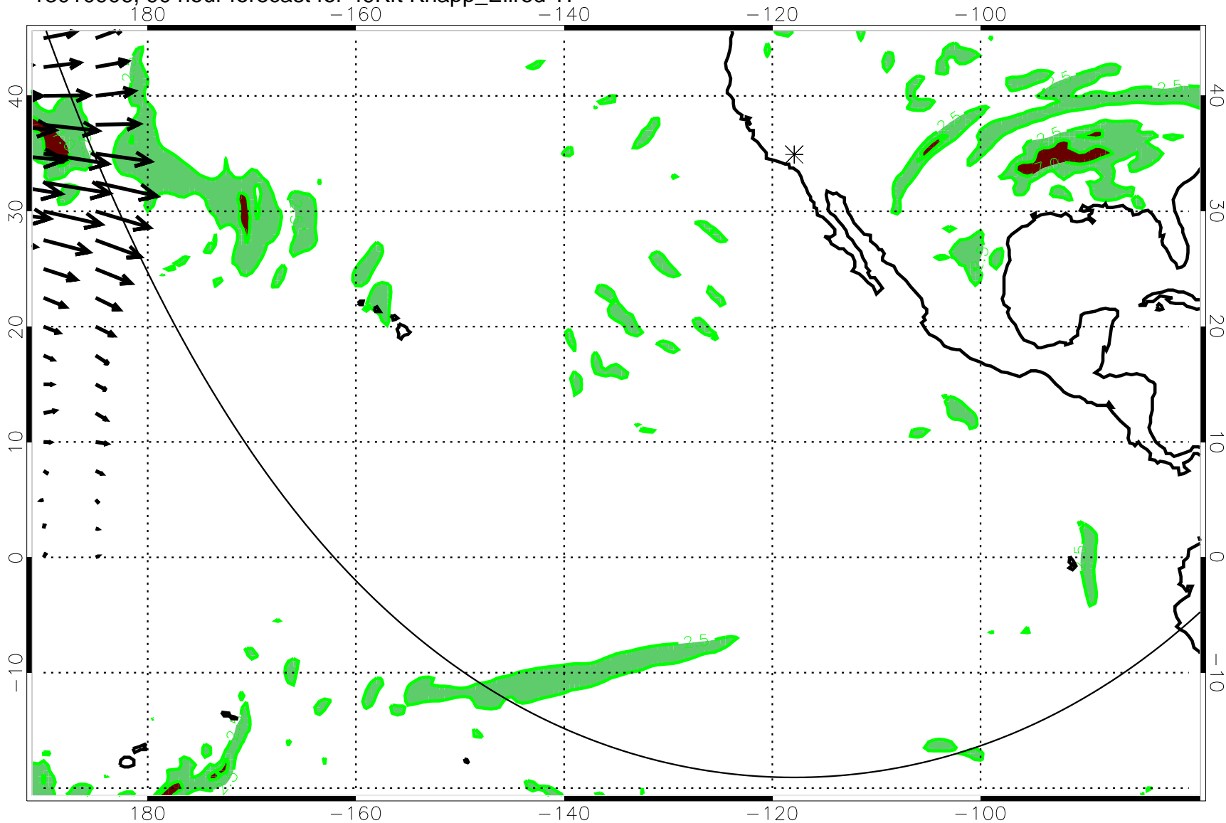
13010906, 90 hour forecast for 49Kft Knapp_Ellrod TI
