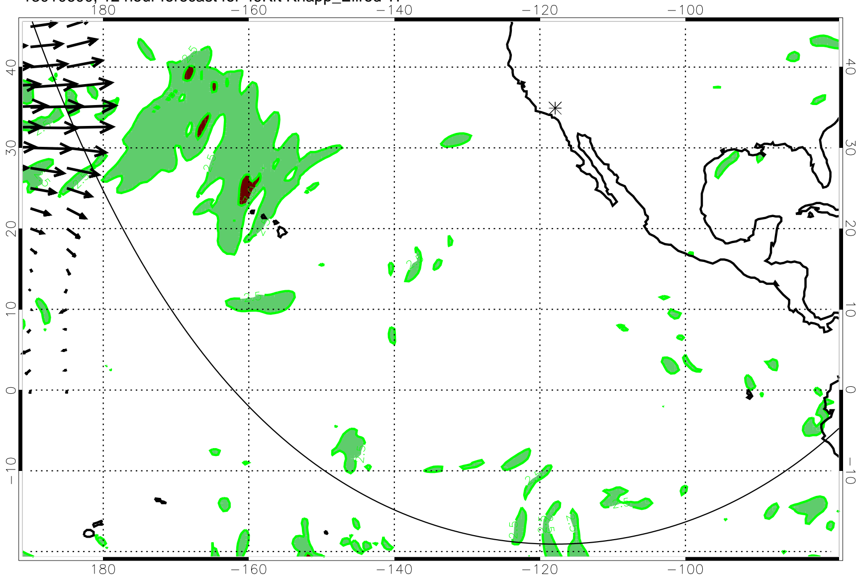
13010600, 12 hour forecast for 49Kft Knapp_Ellrod TI
