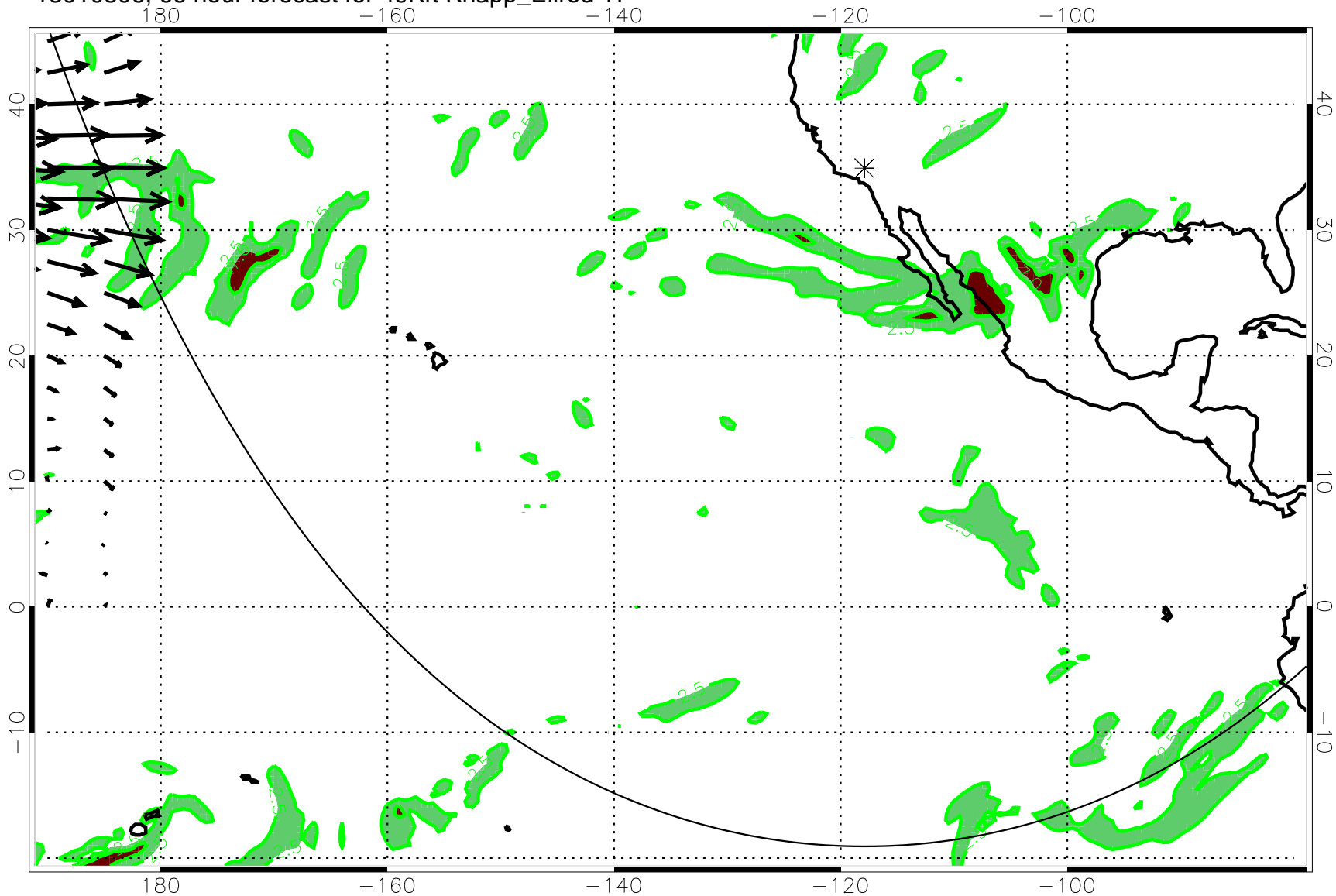
13010806, 66 hour forecast for 49Kft Knapp_Ellrod TI
