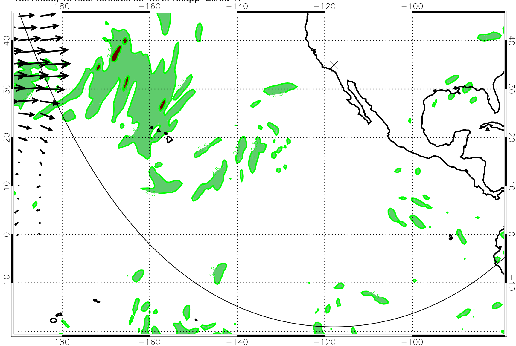
13010606, 18 hour forecast for 49Kft Knapp_Ellrod TI
