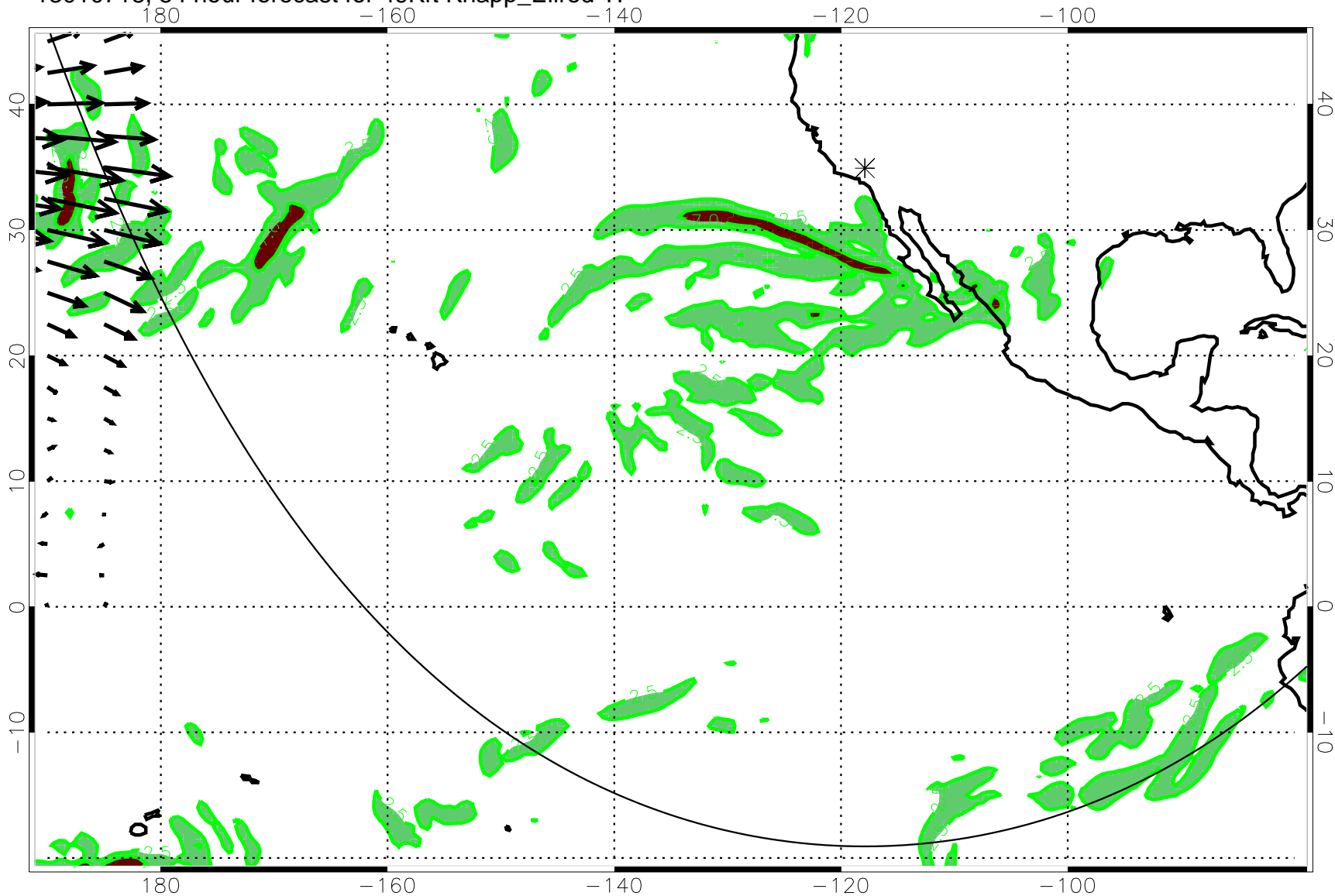
13010718, 54 hour forecast for 49Kft Knapp_Ellrod TI
