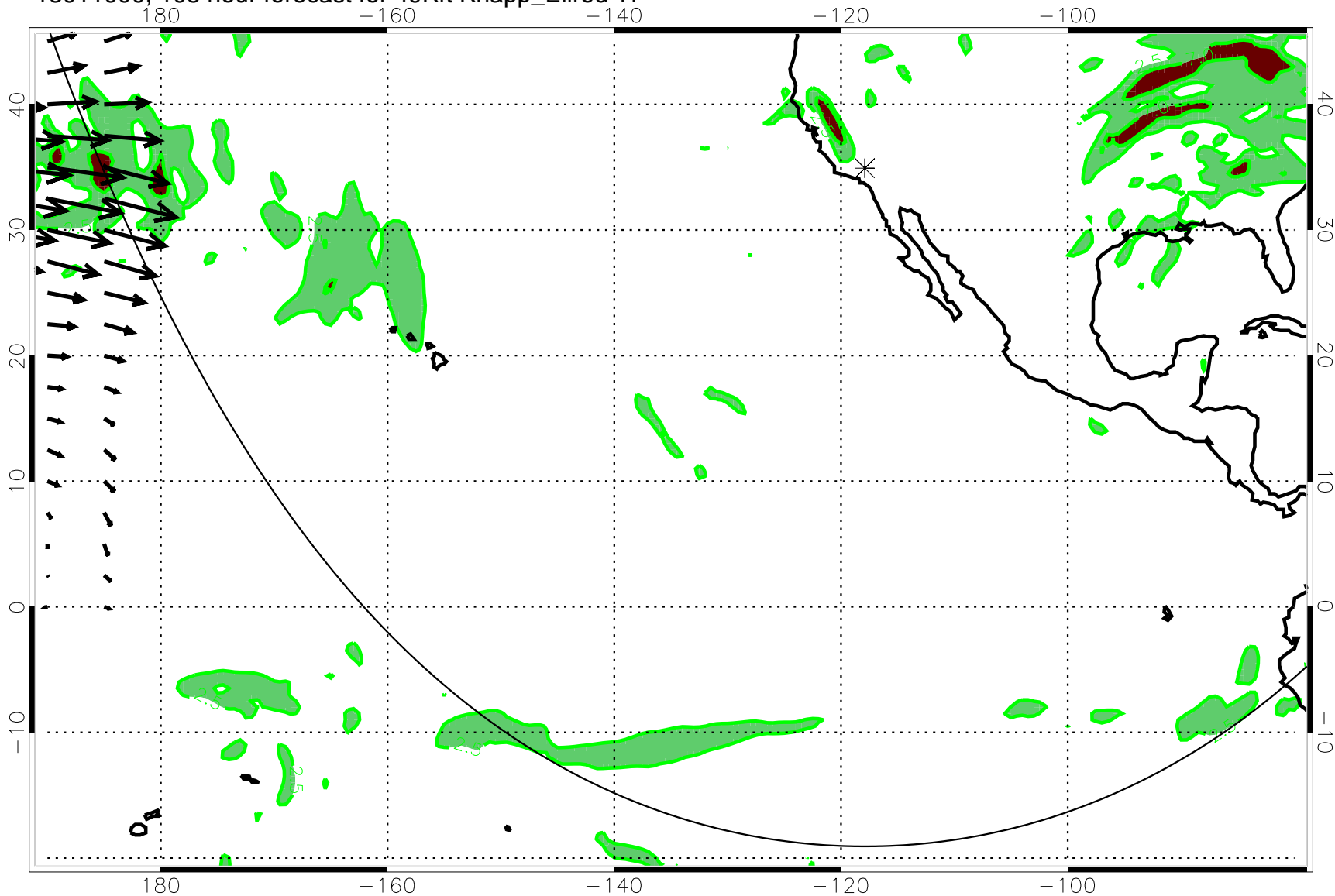
13011000, 108 hour forecast for 49Kft Knapp_Ellrod T1
