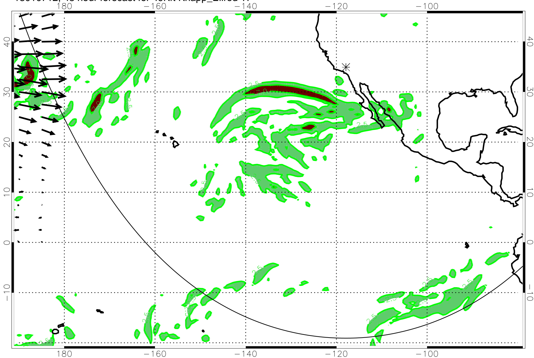
13010712, 48 hour forecast for 49Kft Knapp_Ellrod TI
