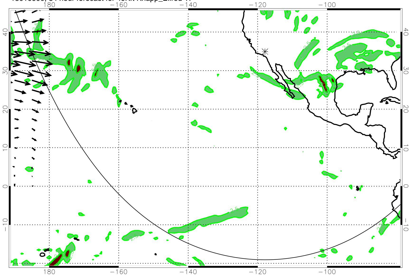
13010900, 84 hour forecast for 49Kft Knapp_Ellrod TI
