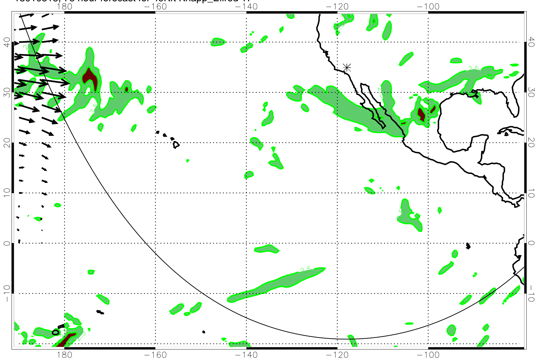
13010818, 78 hour forecast for 49Kft Knapp_Ellrod TI
