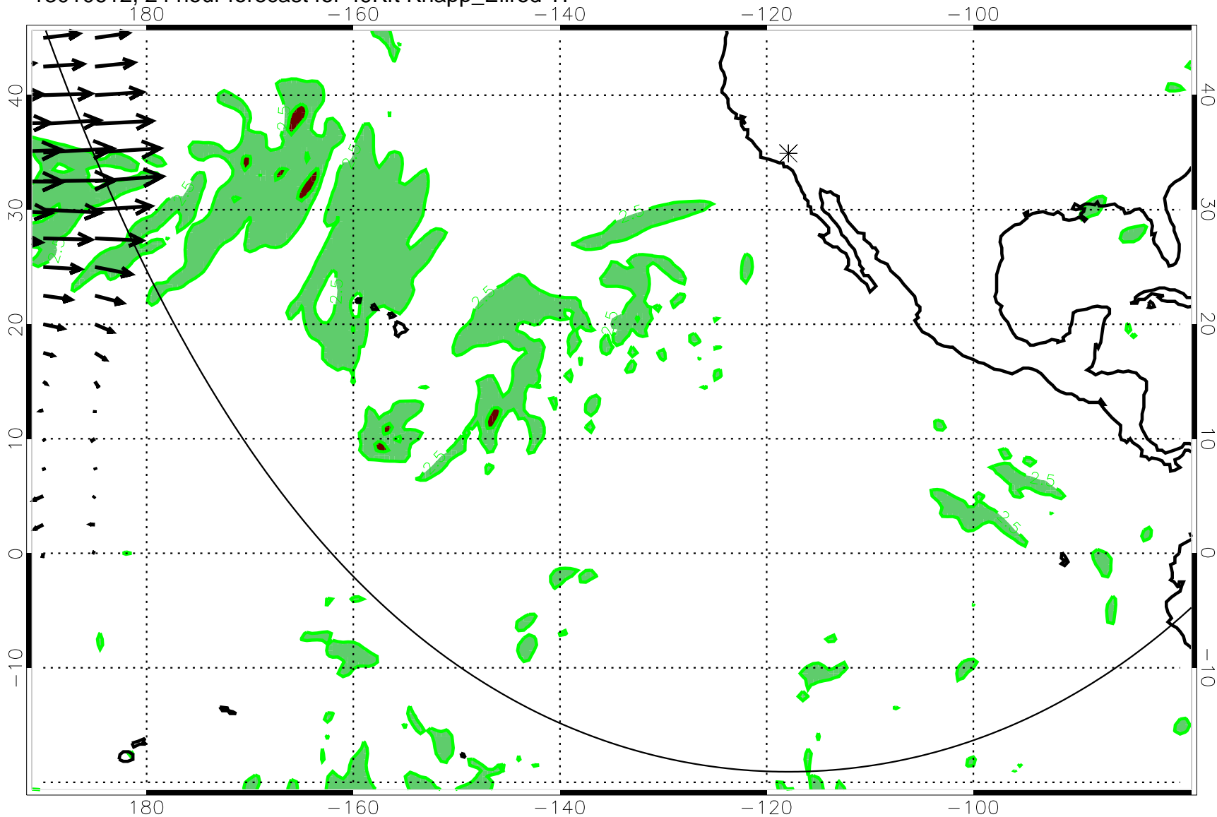
13010612, 24 hour forecast for 49Kft Knapp_Ellrod TI
