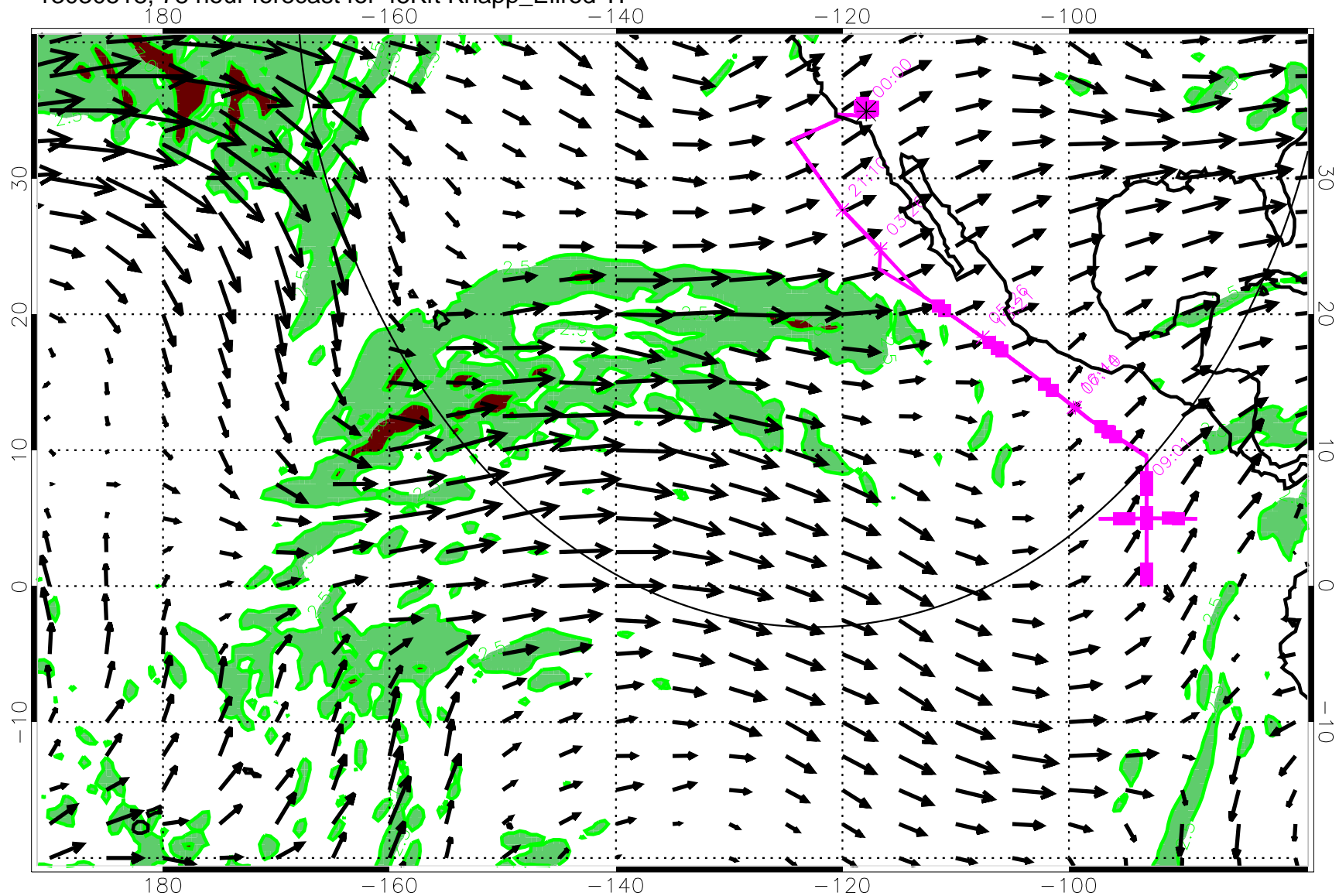
13030518, 78 hour forecast for 45Kft Knapp_Ellrod TI
