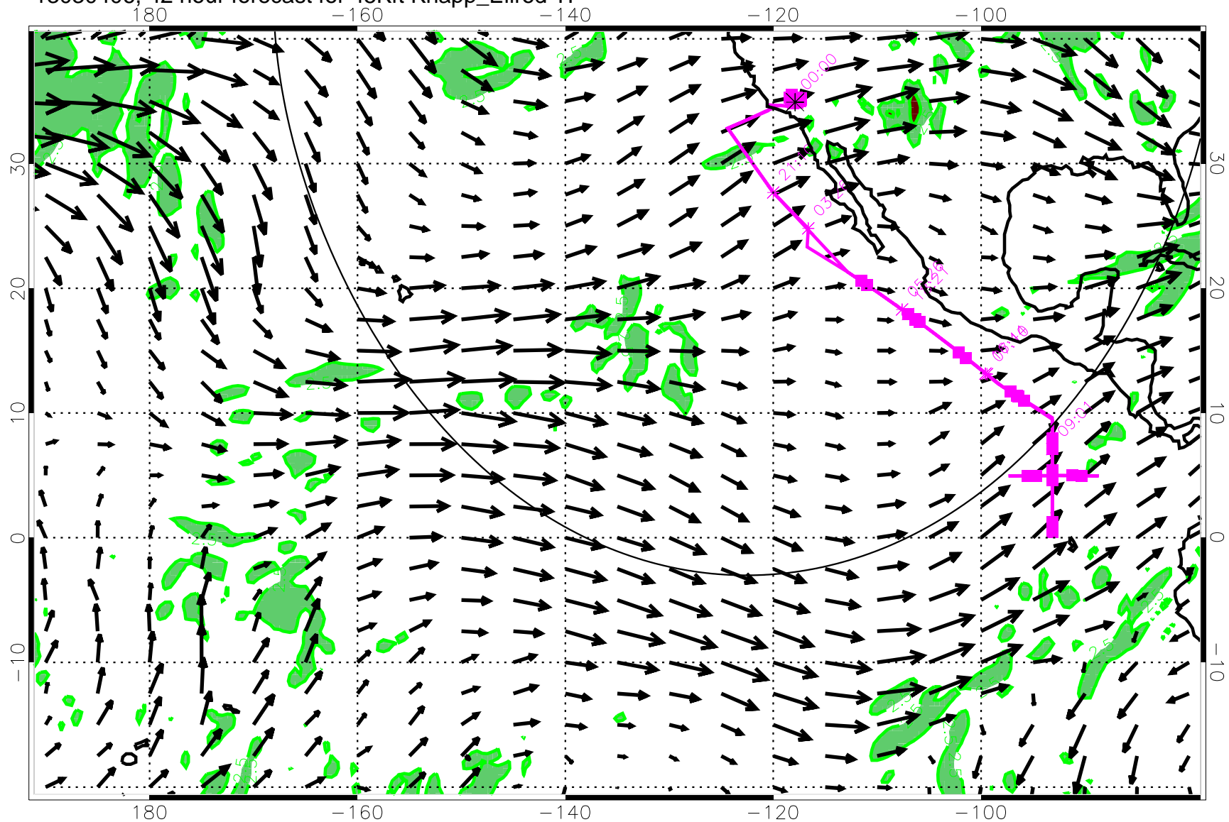
13030406, 42 hour forecast for 45Kft Knapp_Ellrod TI
