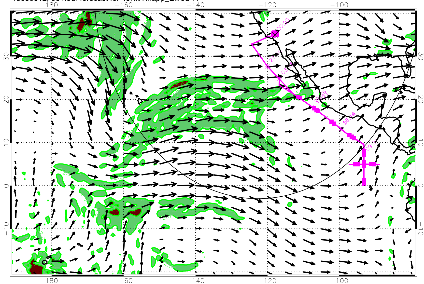
13030612, 96 hour forecast for 45Kft Knapp_Ellrod TI
