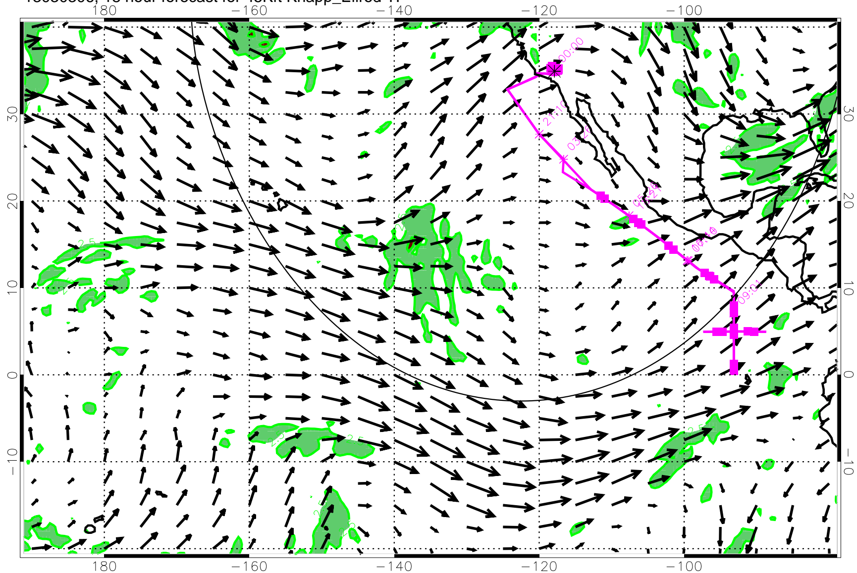
13030306, 18 hour forecast for 45Kft Knapp_Ellrod TI
