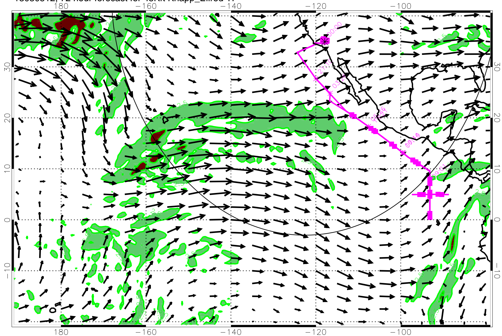
13030512, 72 hour forecast for 45Kft Knapp_Ellrod TI
