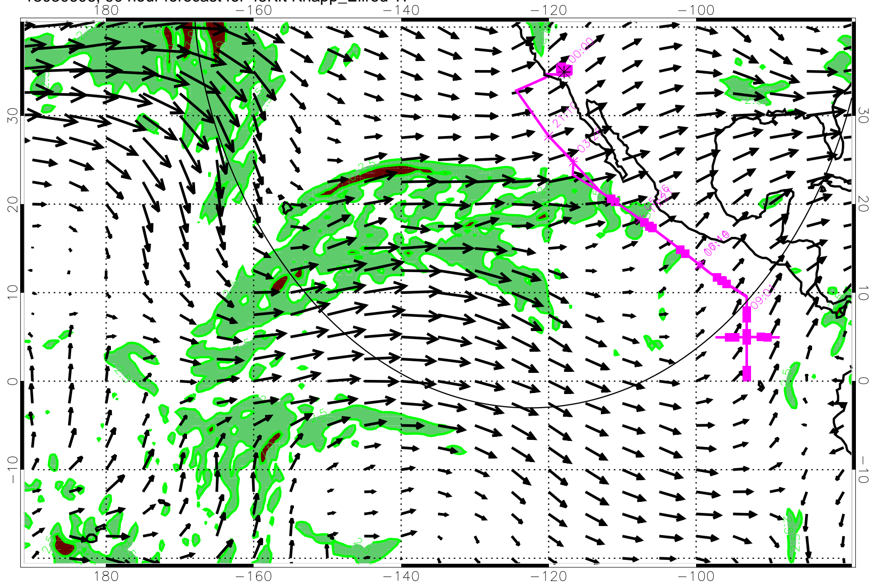
13030606, 90 hour forecast for 45Kft Knapp_Ellrod TI
