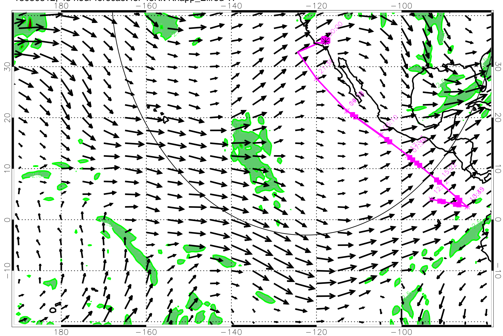
13030312, 48 hour forecast for 45Kft Knapp_Ellrod TI
