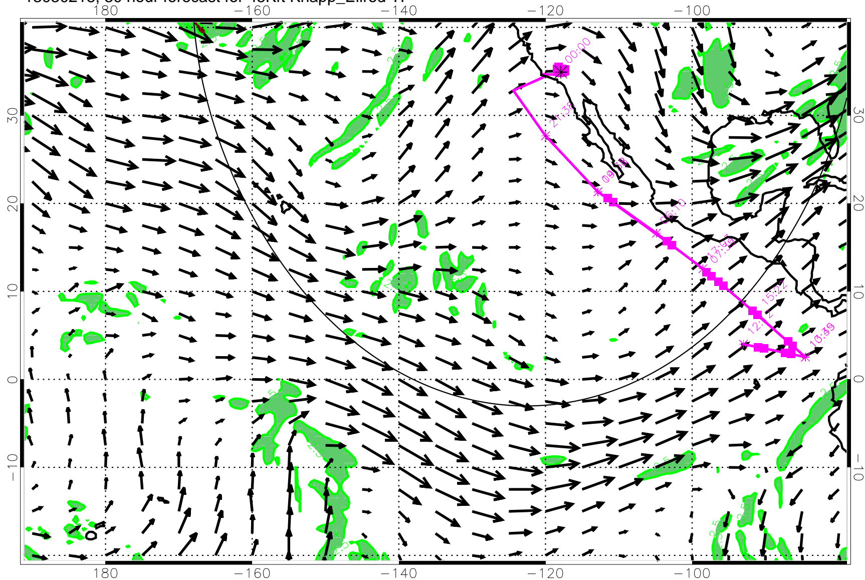
13030218, 30 hour forecast for 45Kft Knapp_Ellrod TI
