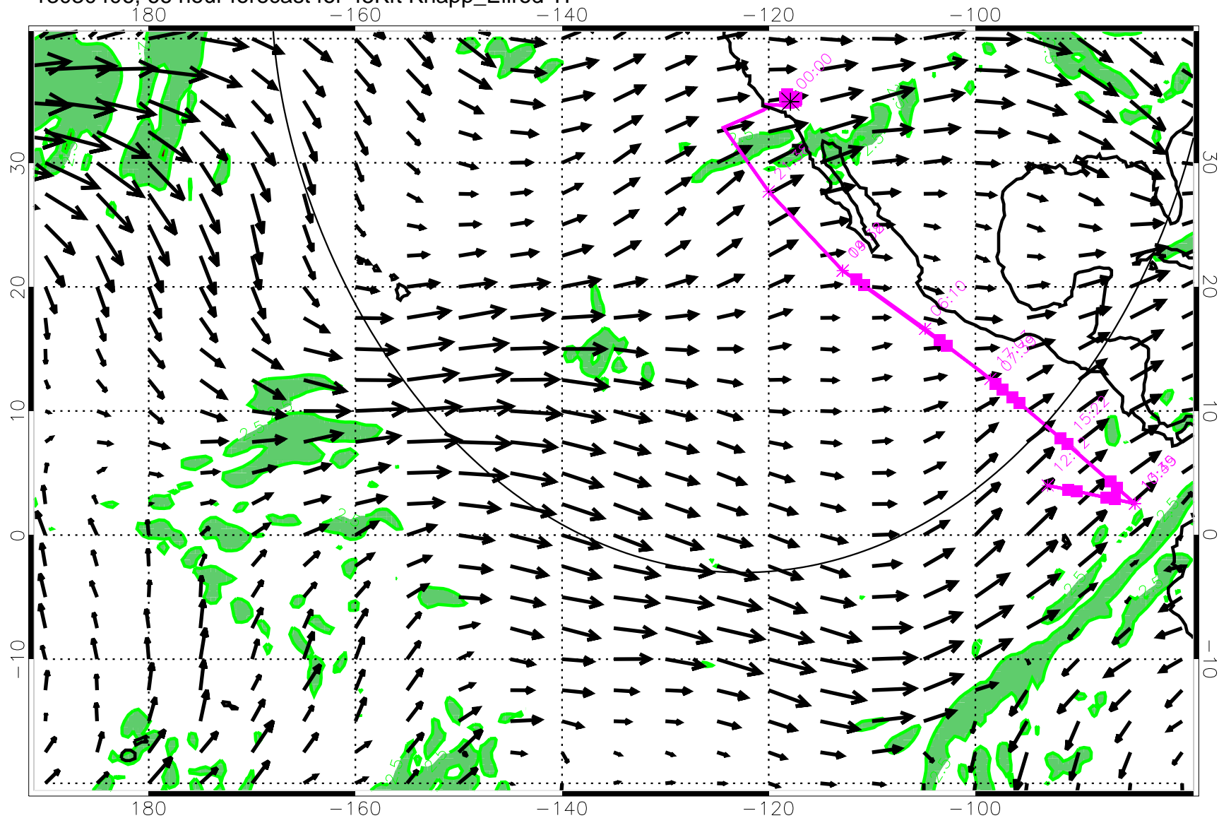
13030406, 66 hour forecast for 45Kft Knapp_Ellrod TI
