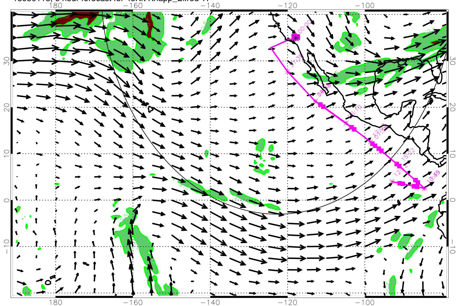
13030118, 6 hour forecast for 45Kft Knapp_Ellrod TI
