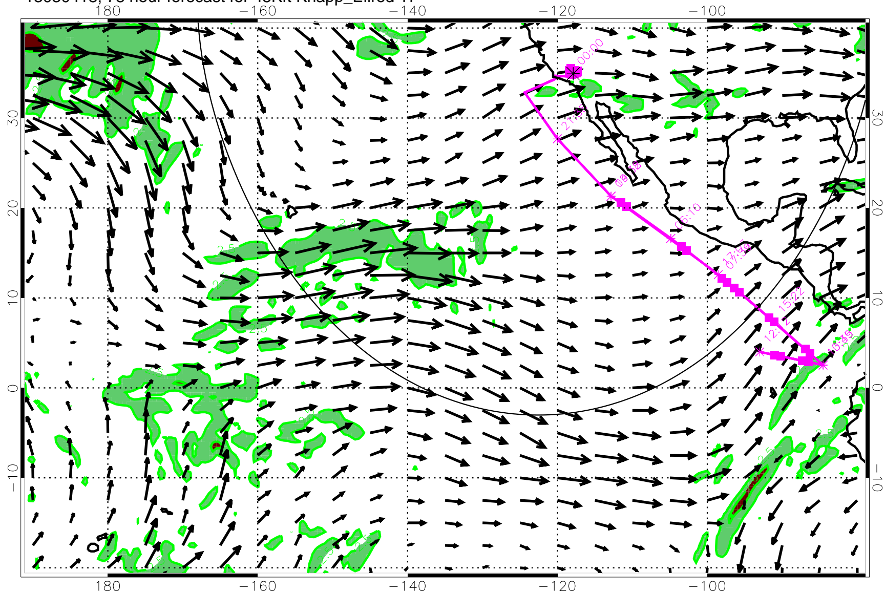
13030418, 78 hour forecast for 45Kft Knapp_Ellrod TI
