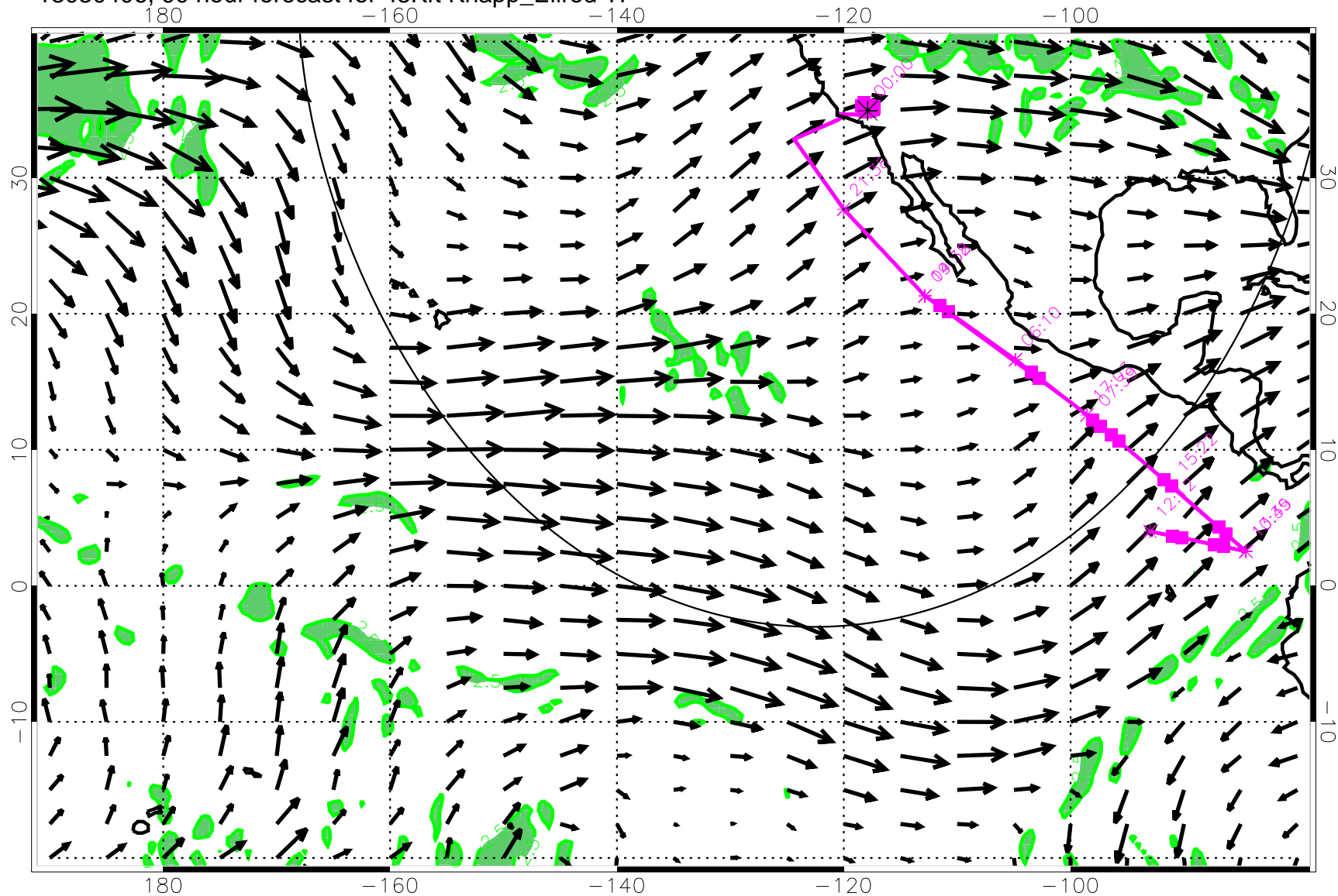
13030406, 90 hour forecast for 45Kft Knapp_Ellrod TI
