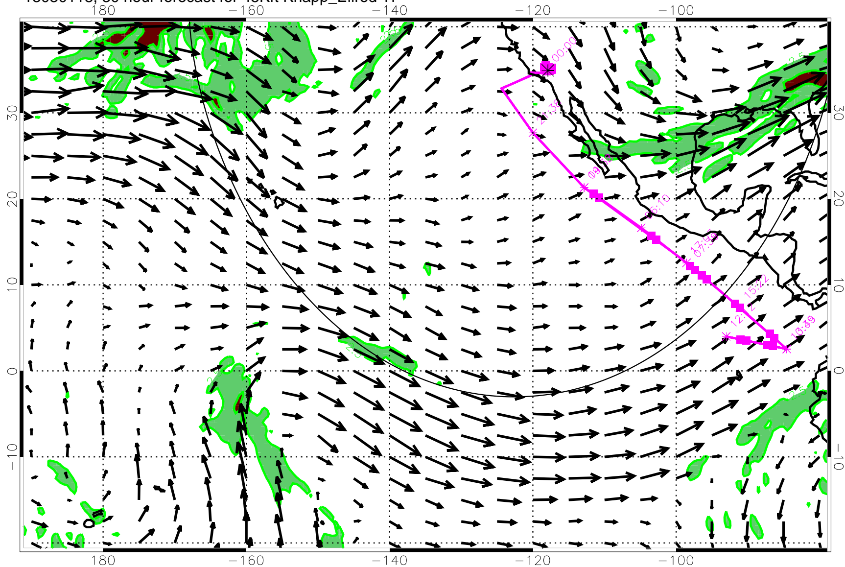
13030118, 30 hour forecast for 45Kft Knapp_Ellrod TI
