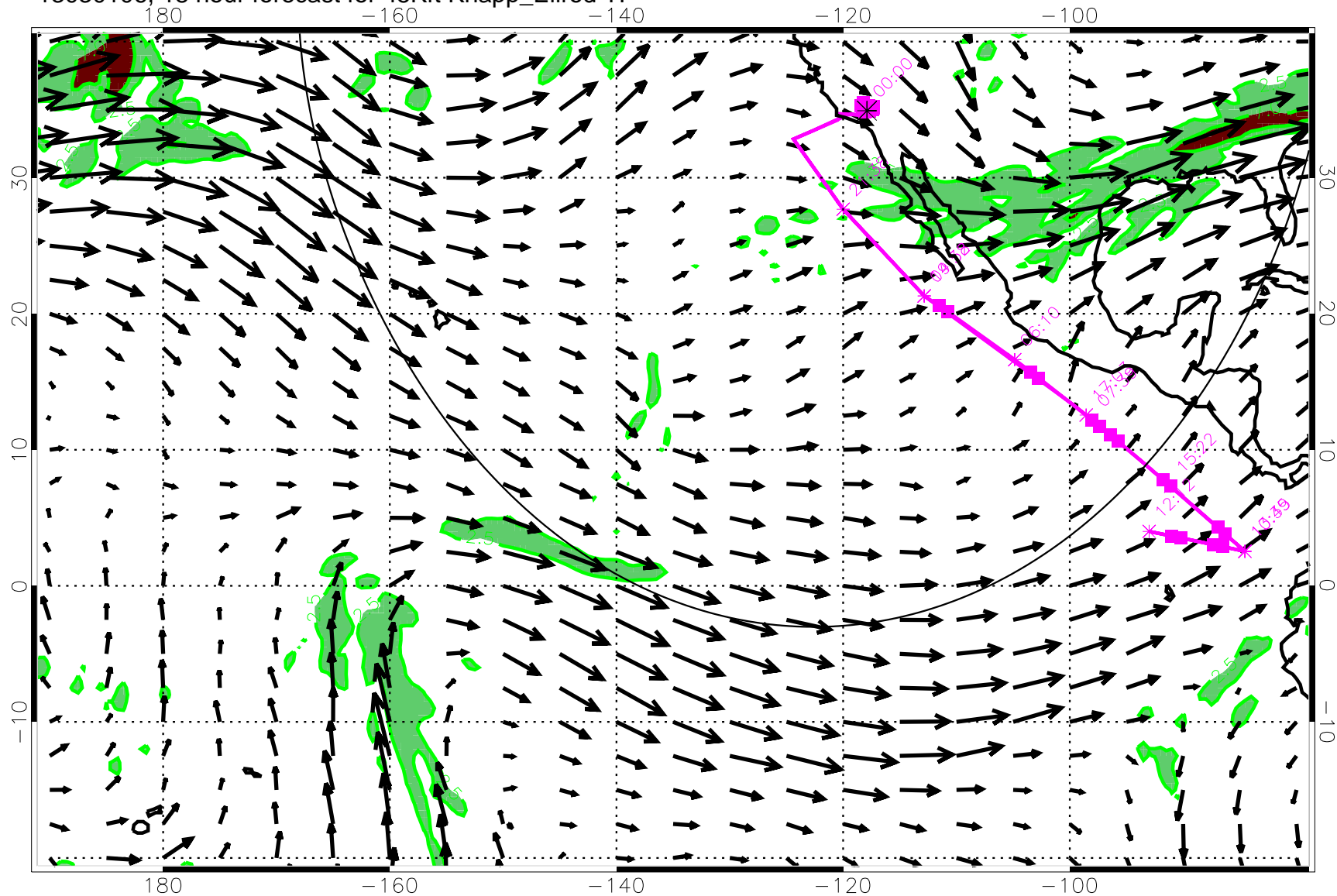
13030106, 18 hour forecast for 45Kft Knapp_Ellrod TI
