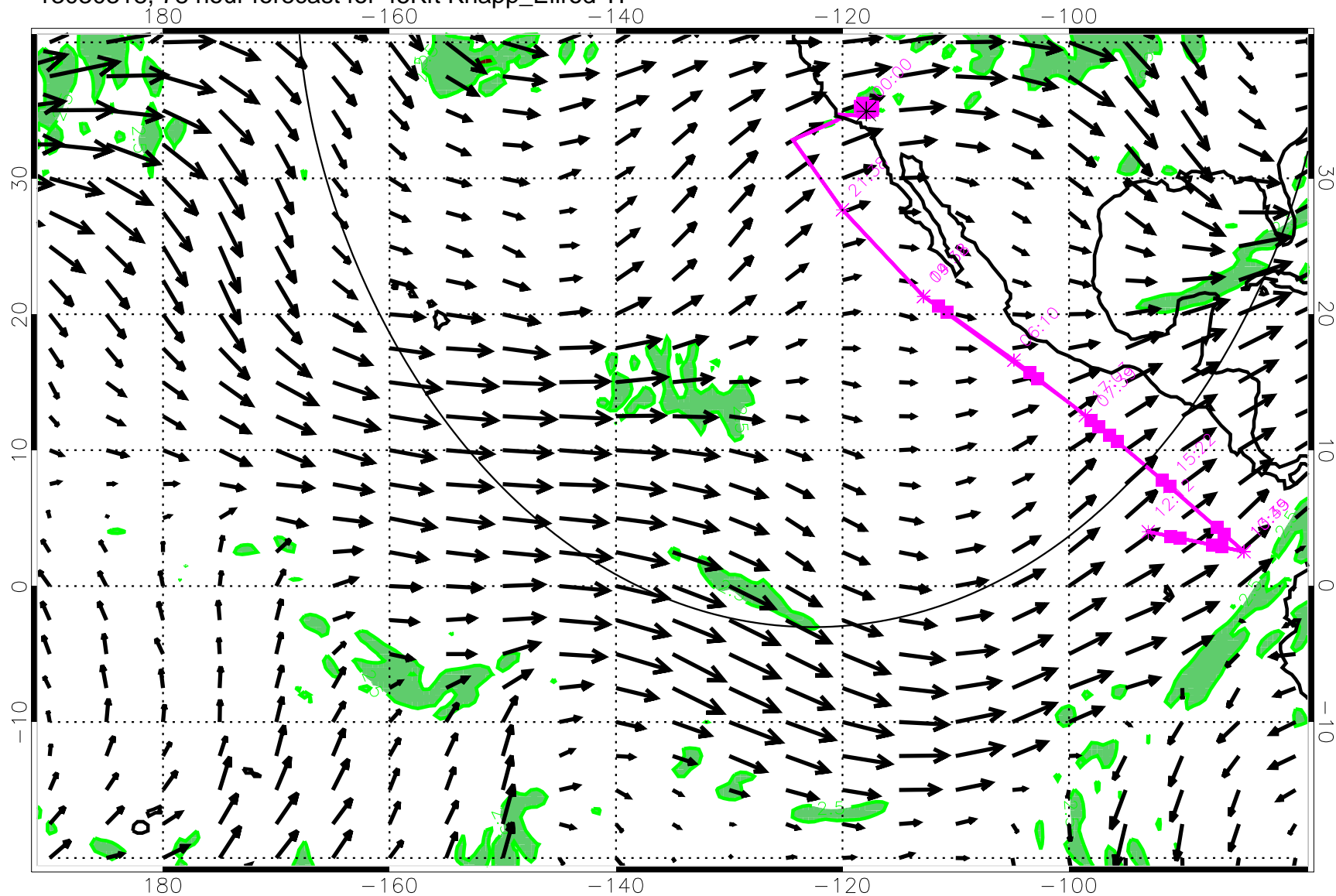
13030318, 78 hour forecast for 45Kft Knapp_Ellrod TI
