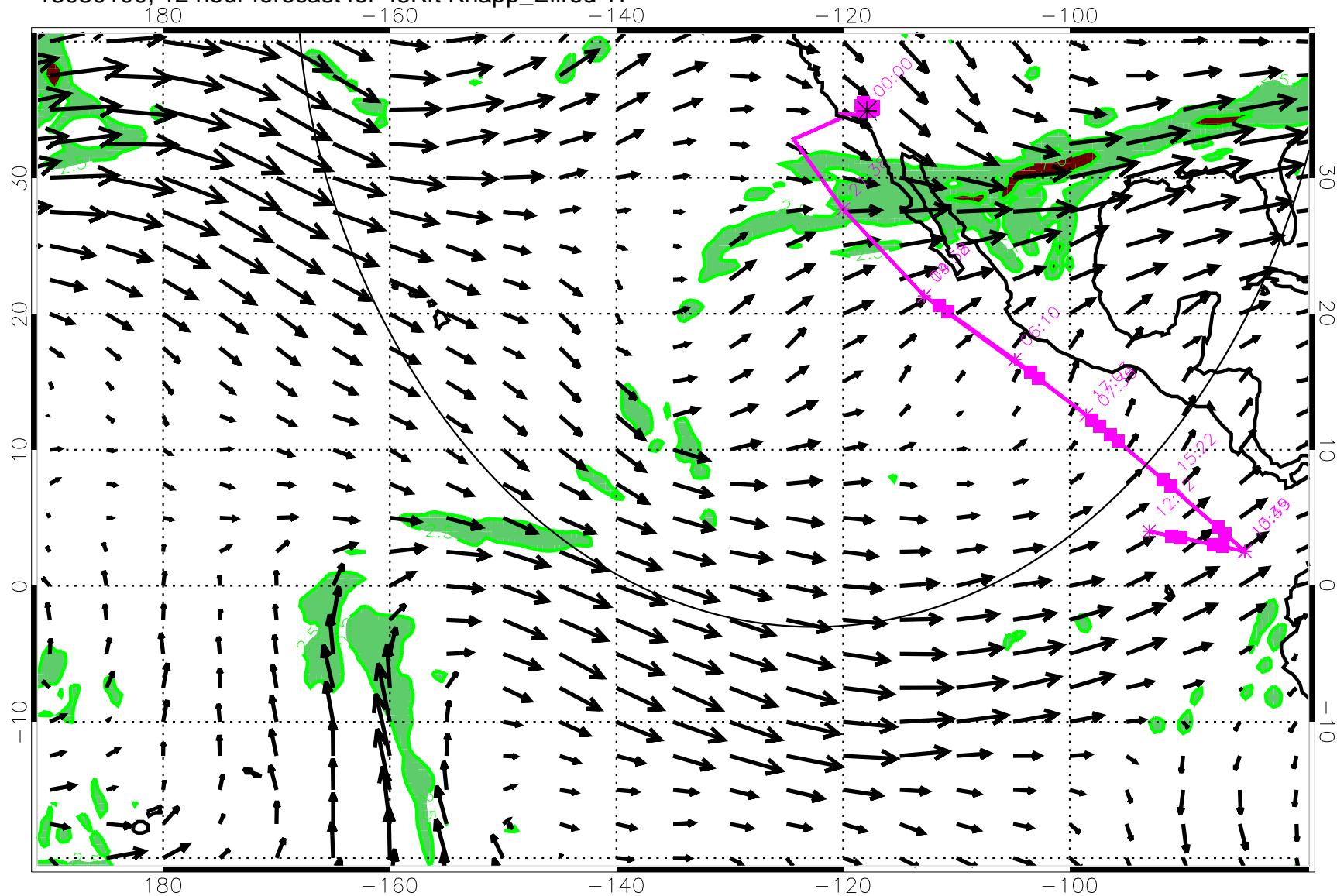
13030100, 12 hour forecast for 45Kft Knapp_Ellrod TI
