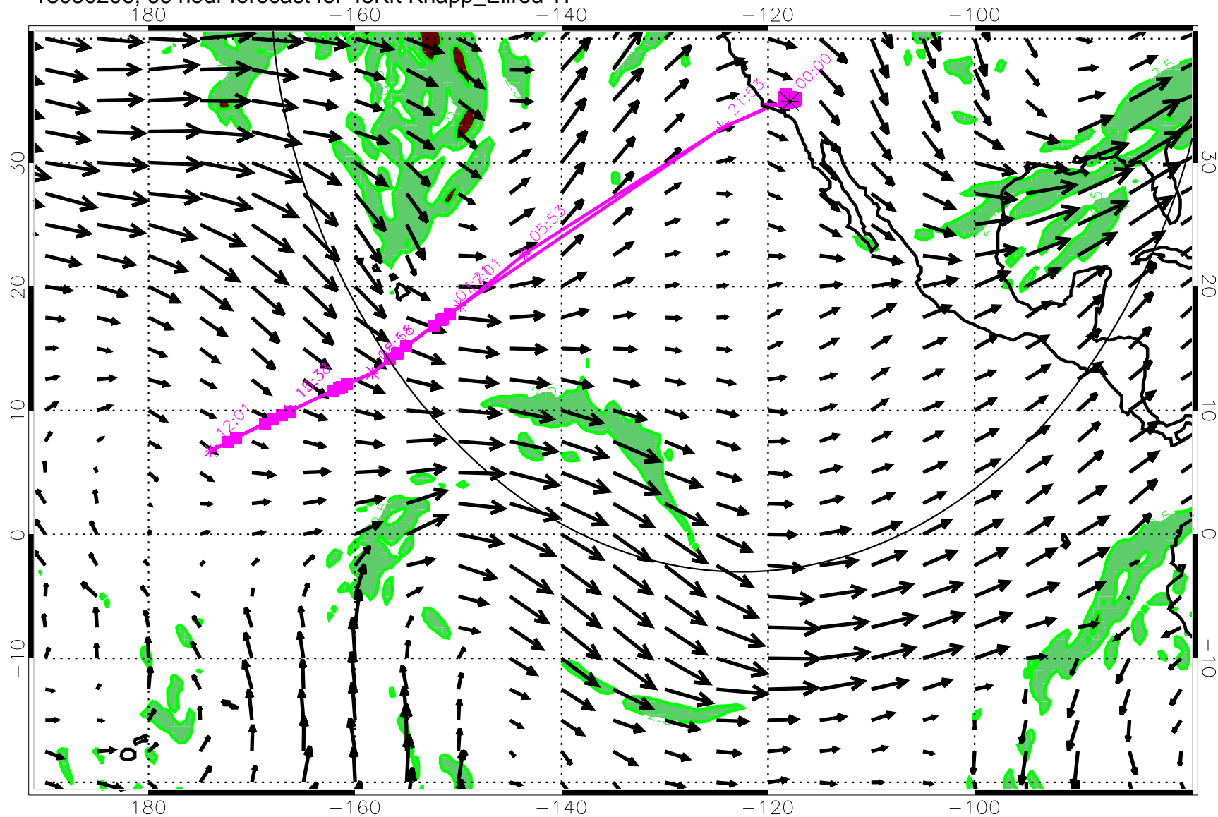
13030206, 66 hour forecast for 45Kft Knapp_Ellrod TI
