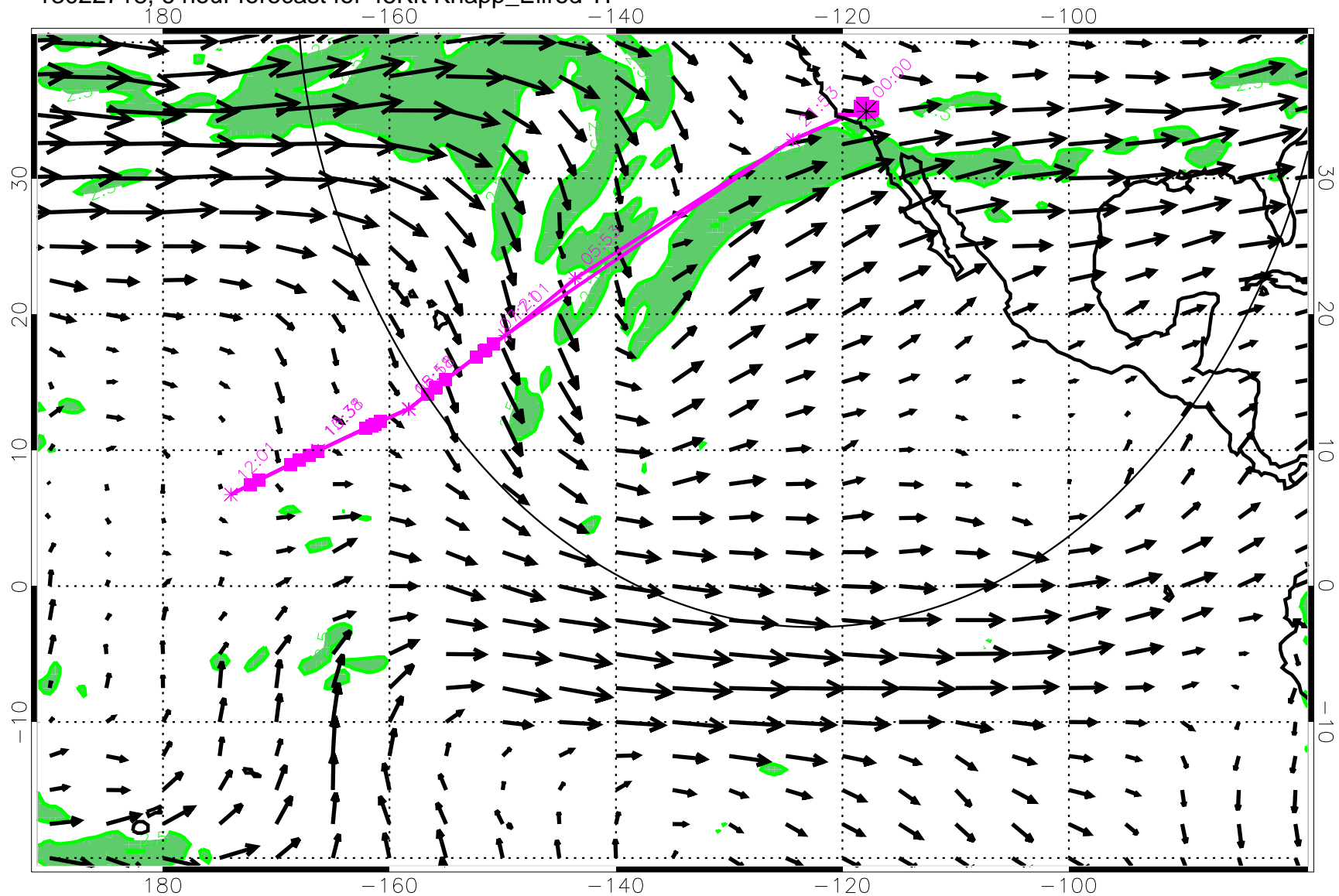
13022718, 6 hour forecast for 45Kft Knapp_Ellrod TI
