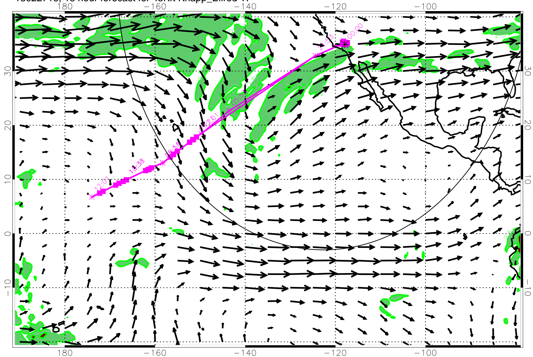
13022718, 18 hour forecast for 45Kft Knapp_Ellrod TI
