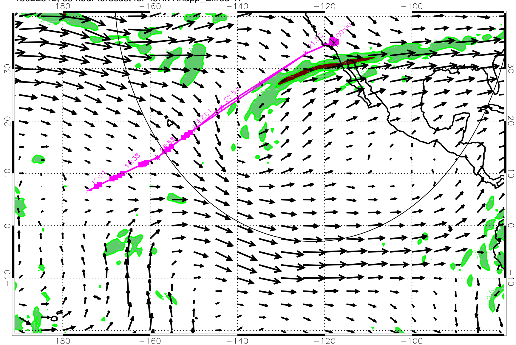
13022812, 36 hour forecast for 45Kft Knapp_Ellrod TI
