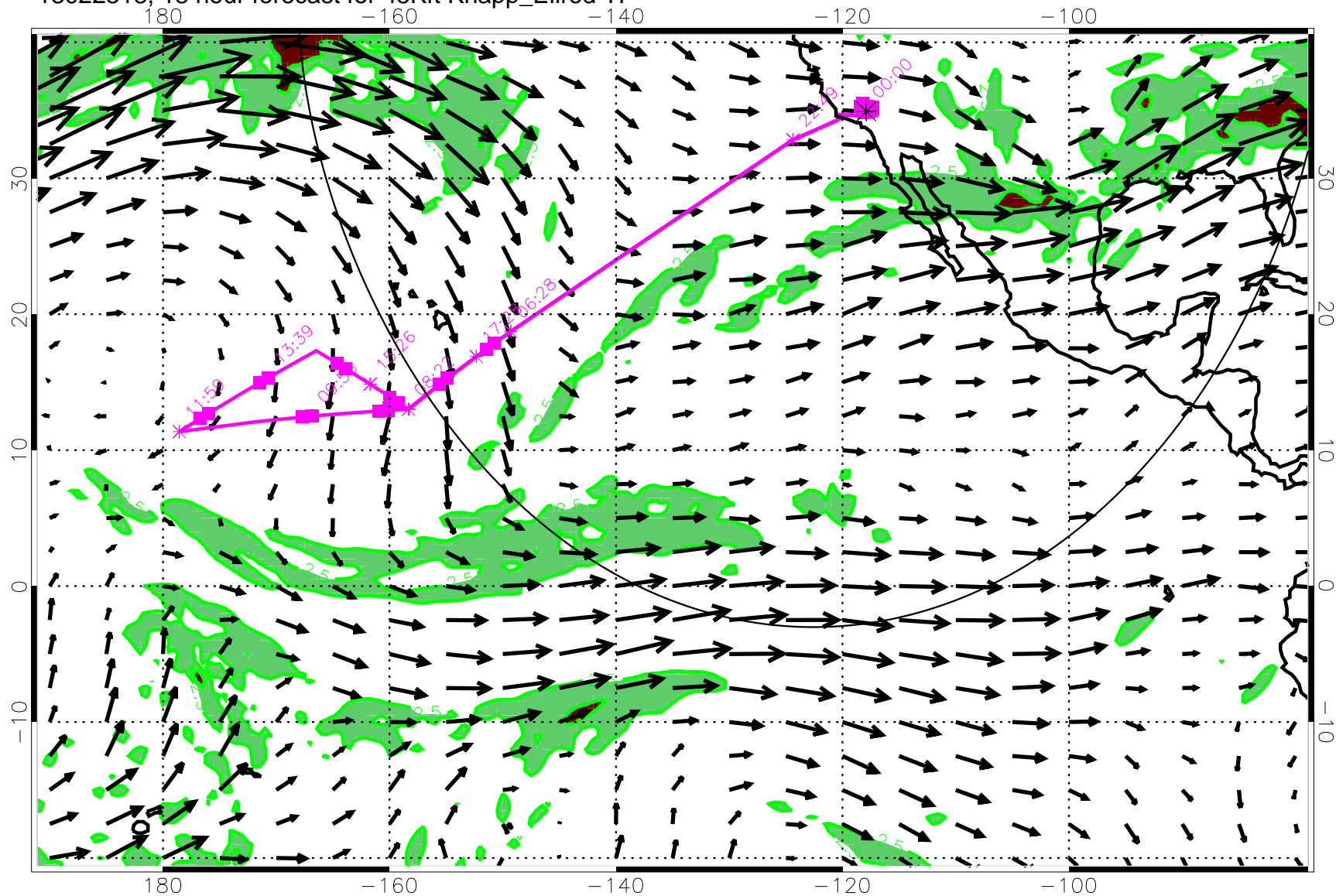
13022518, 18 hour forecast for 45Kft Knapp_Ellrod TI
