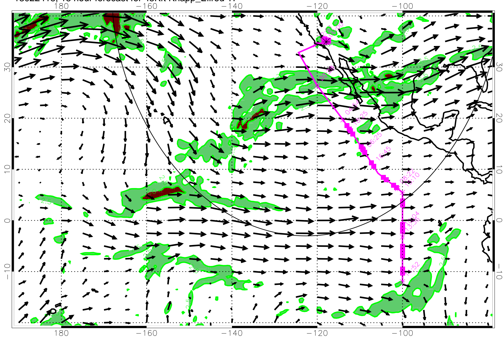
13022418, 18 hour forecast for 45Kft Knapp_Ellrod TI
