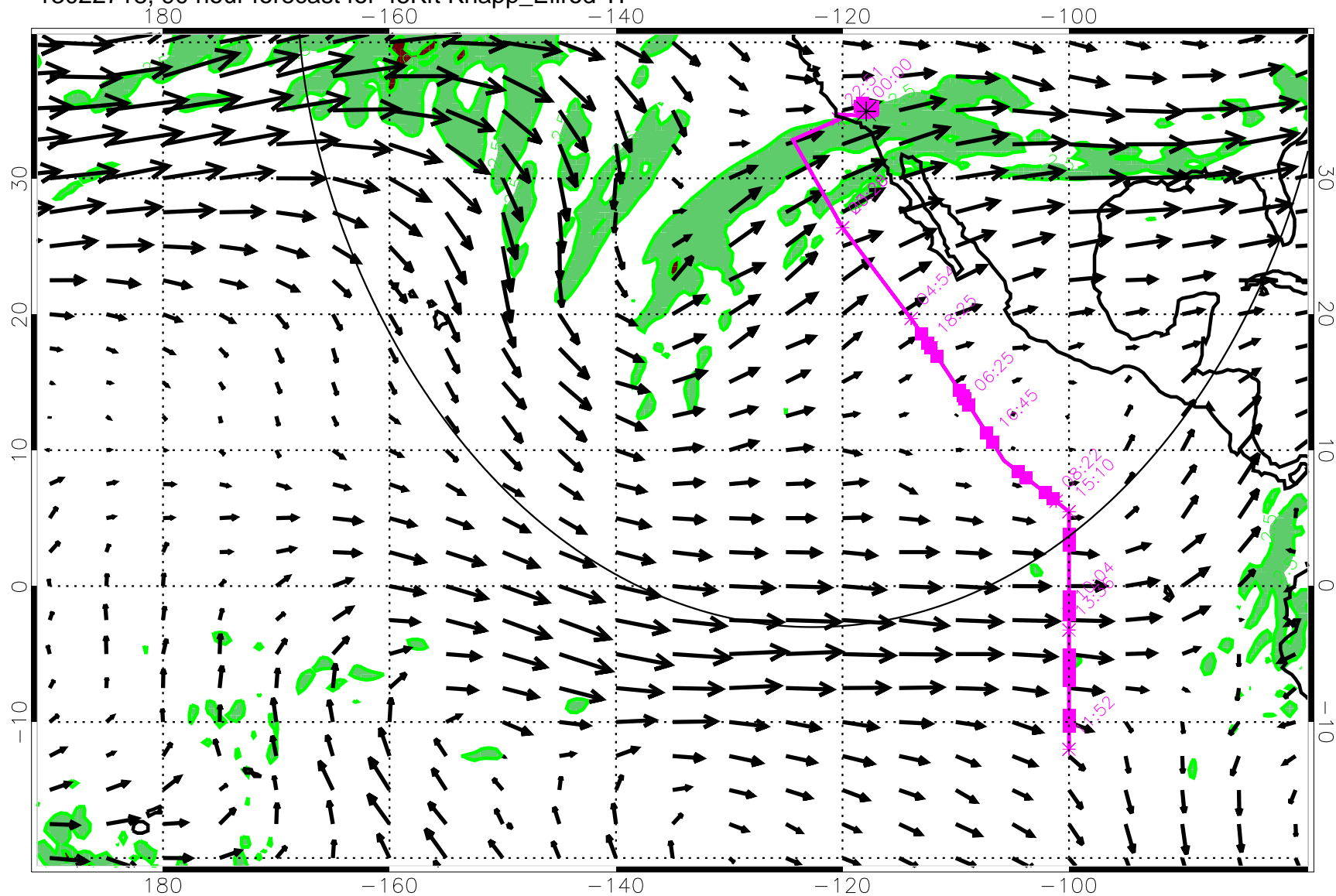
13022718, 90 hour forecast for 45Kft Knapp_Ellrod TI
