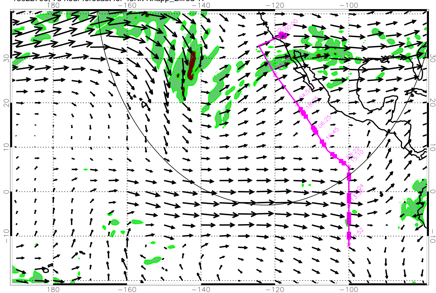
13022706, 78 hour forecast for 45Kft Knapp_Ellrod TI
