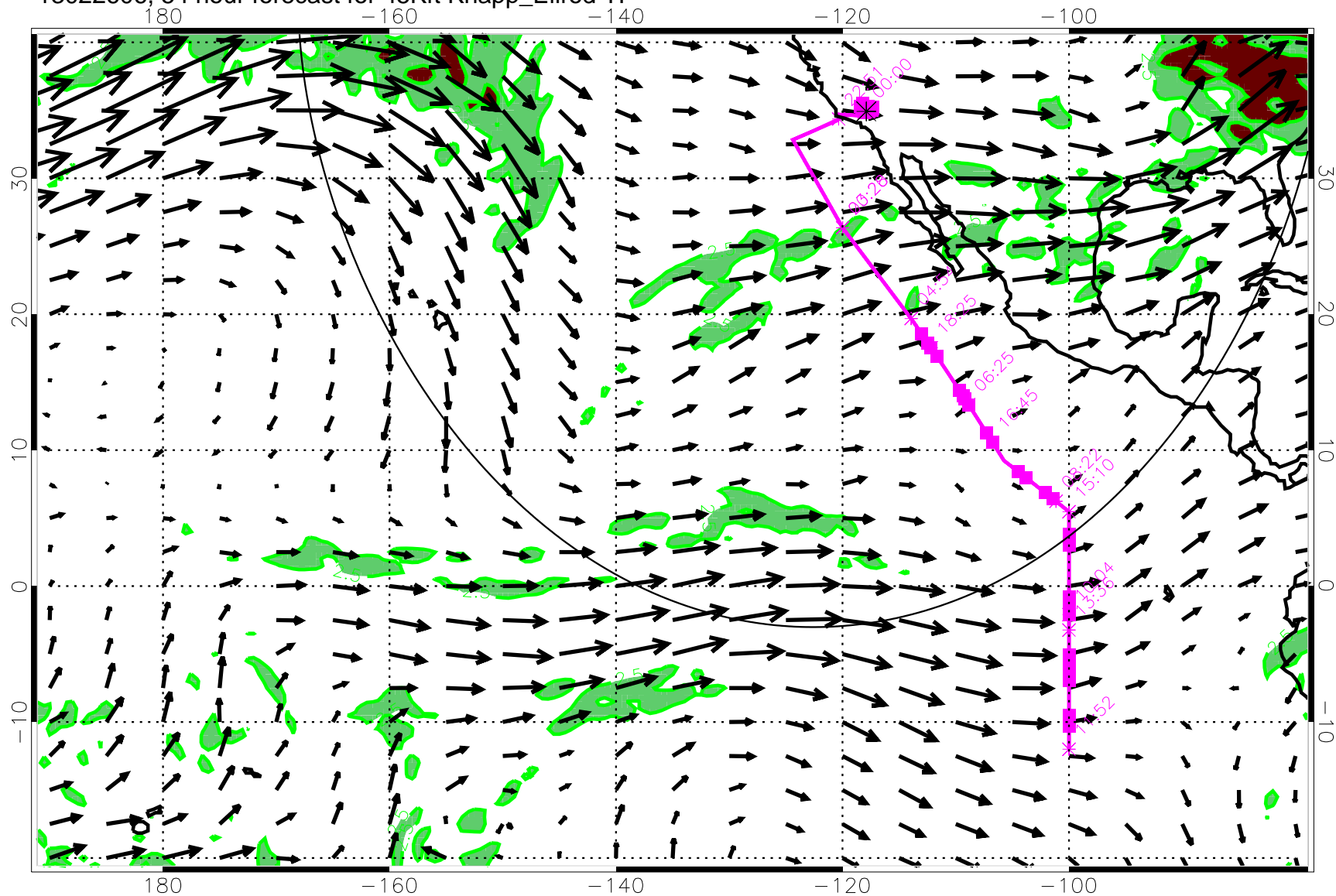
13022606, 54 hour forecast for 45Kft Knapp_Ellrod TI
