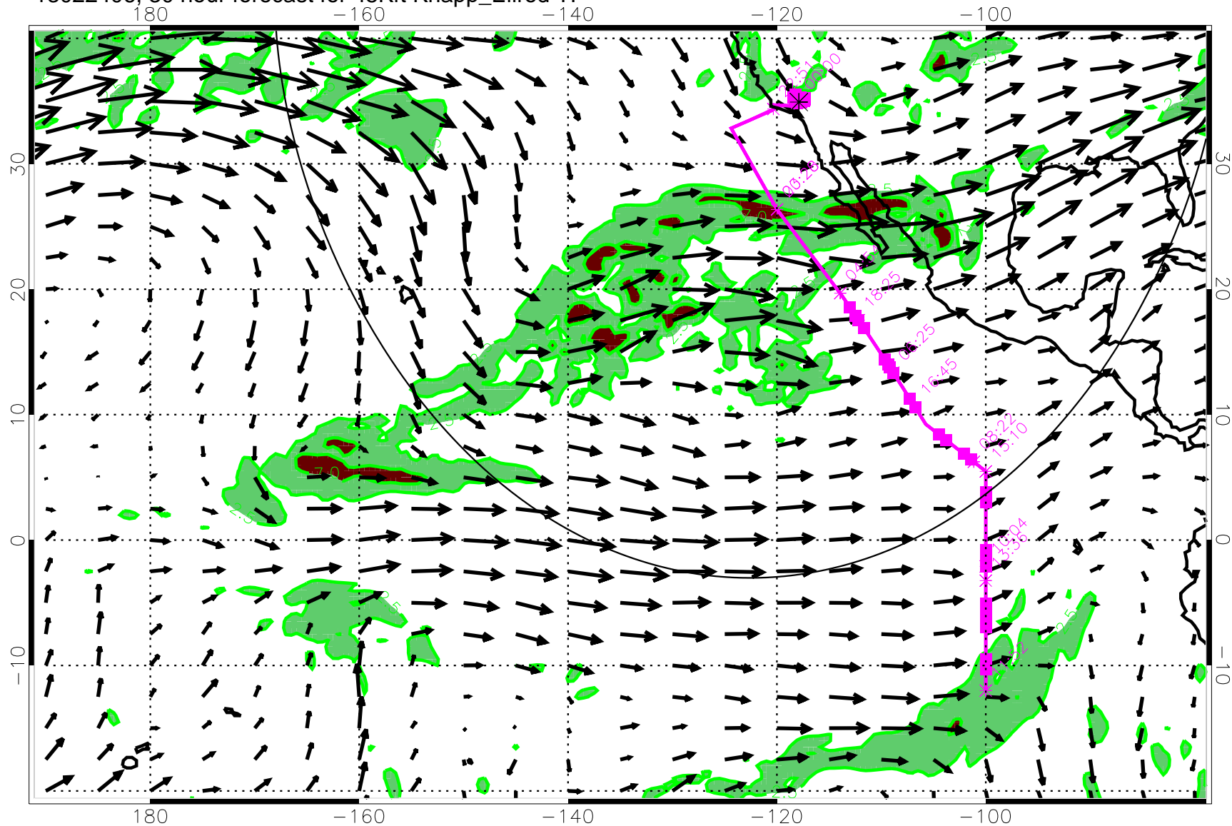
13022406, 30 hour forecast for 45Kft Knapp_Ellrod TI
