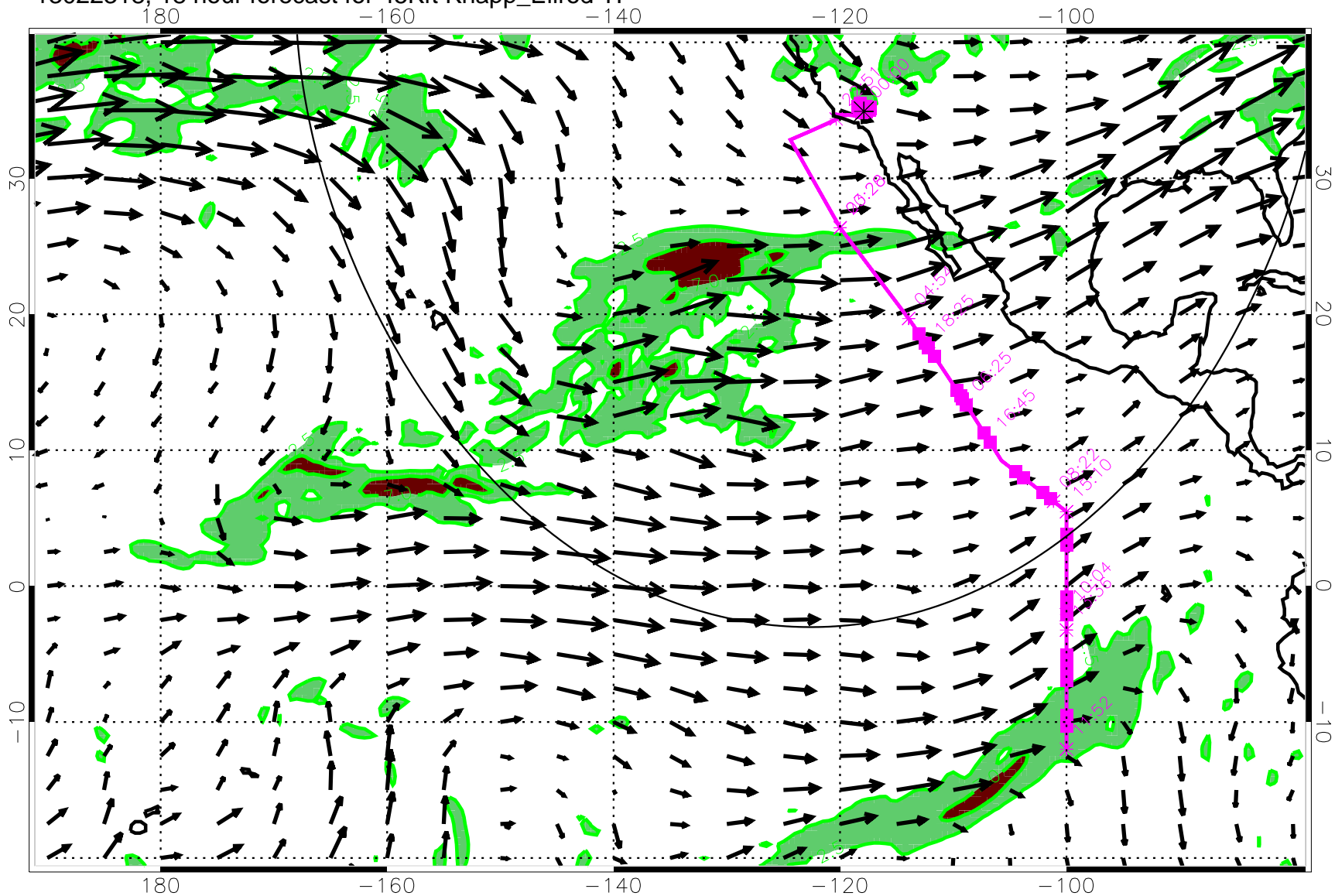
13022318, 18 hour forecast for 45Kft Knapp_Ellrod TI
