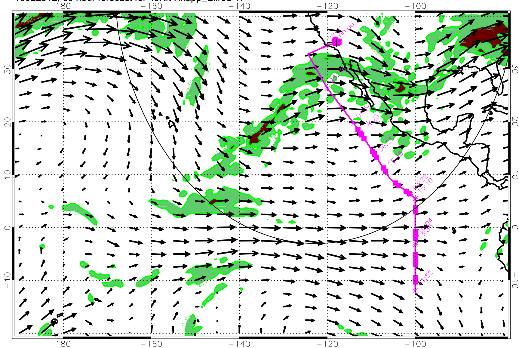
13022512, 60 hour forecast for 45Kft Knapp_Ellrod TI
