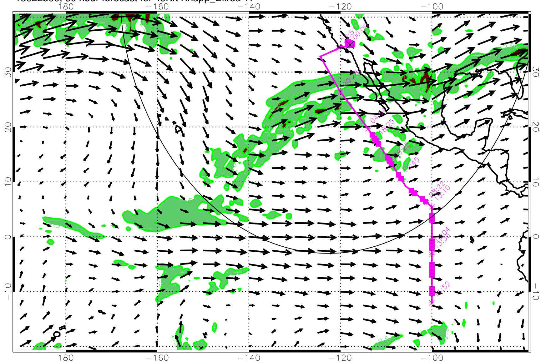
13022500, 60 hour forecast for 45Kft Knapp_Ellrod TI
