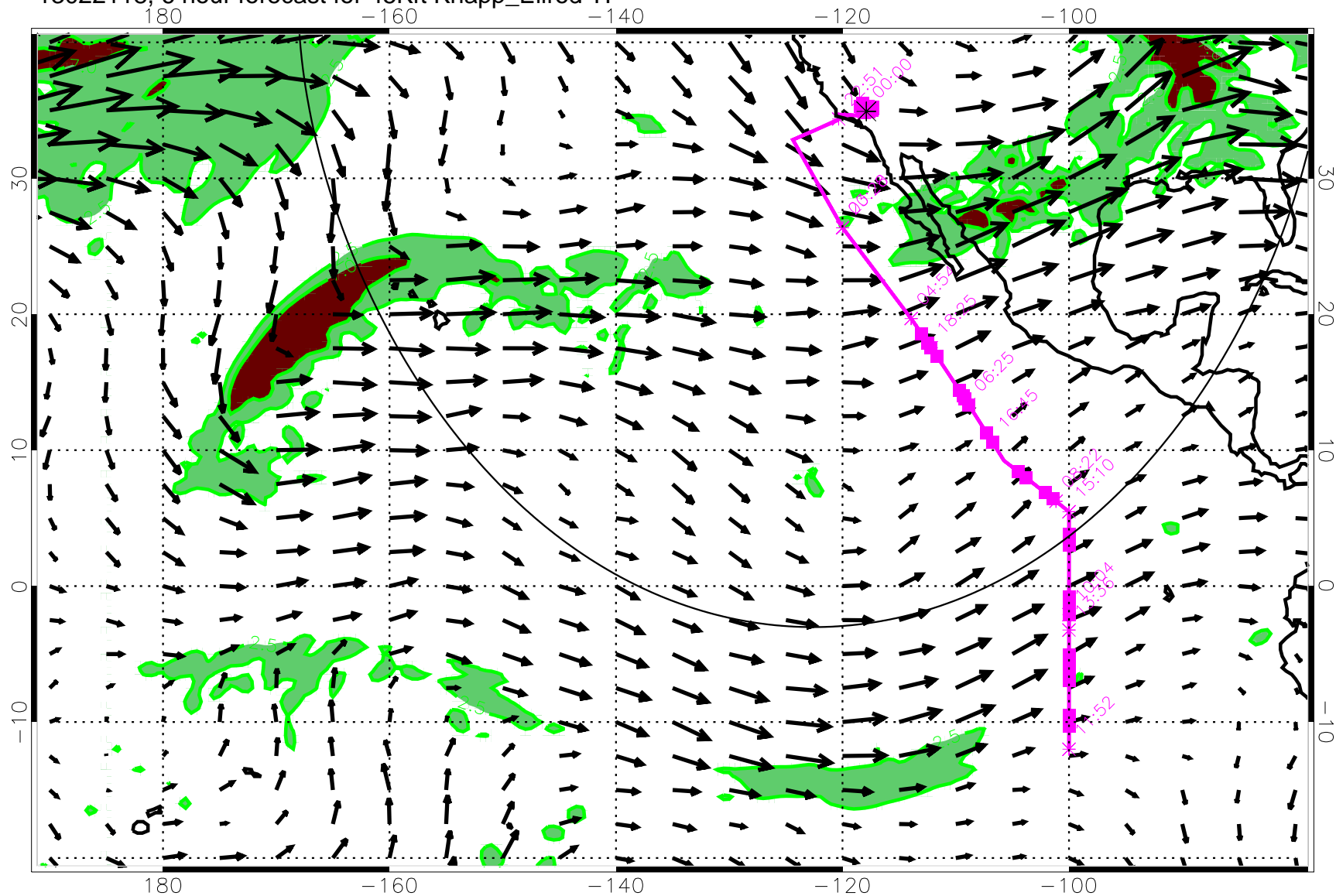
13022118, 6 hour forecast for 45Kft Knapp_Ellrod TI
