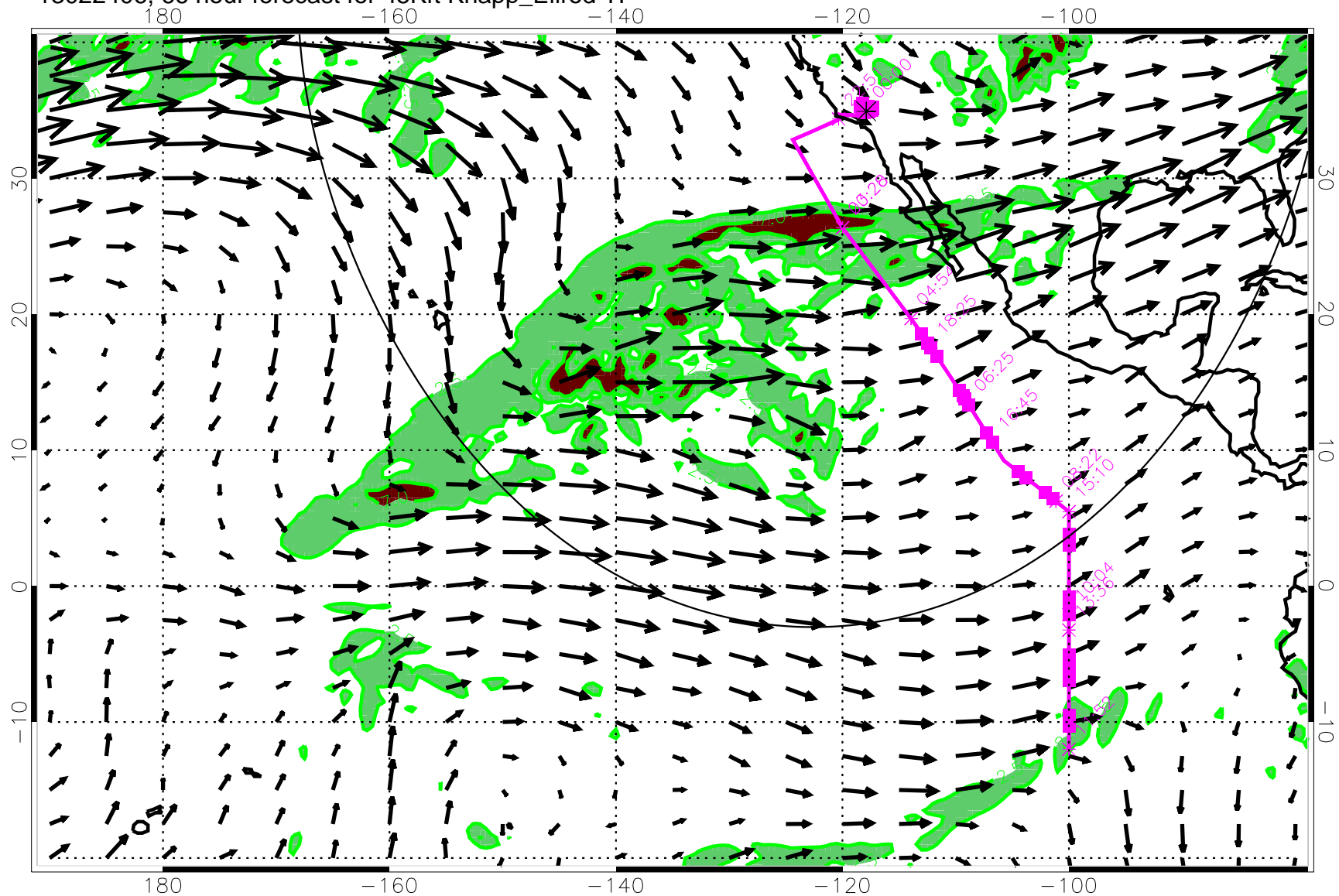
13022406, 66 hour forecast for 45Kft Knapp_Ellrod TI
