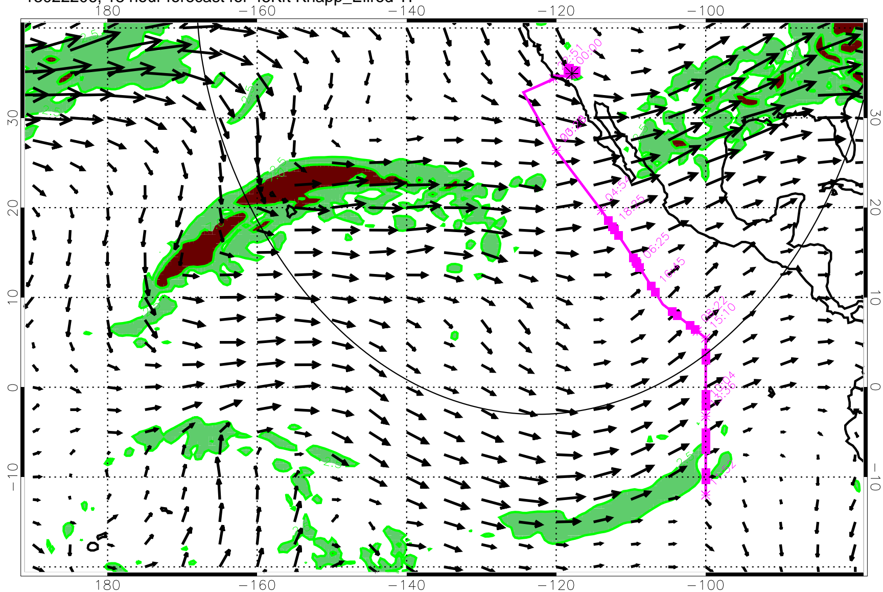
13022206, 18 hour forecast for 45Kft Knapp_Ellrod TI
