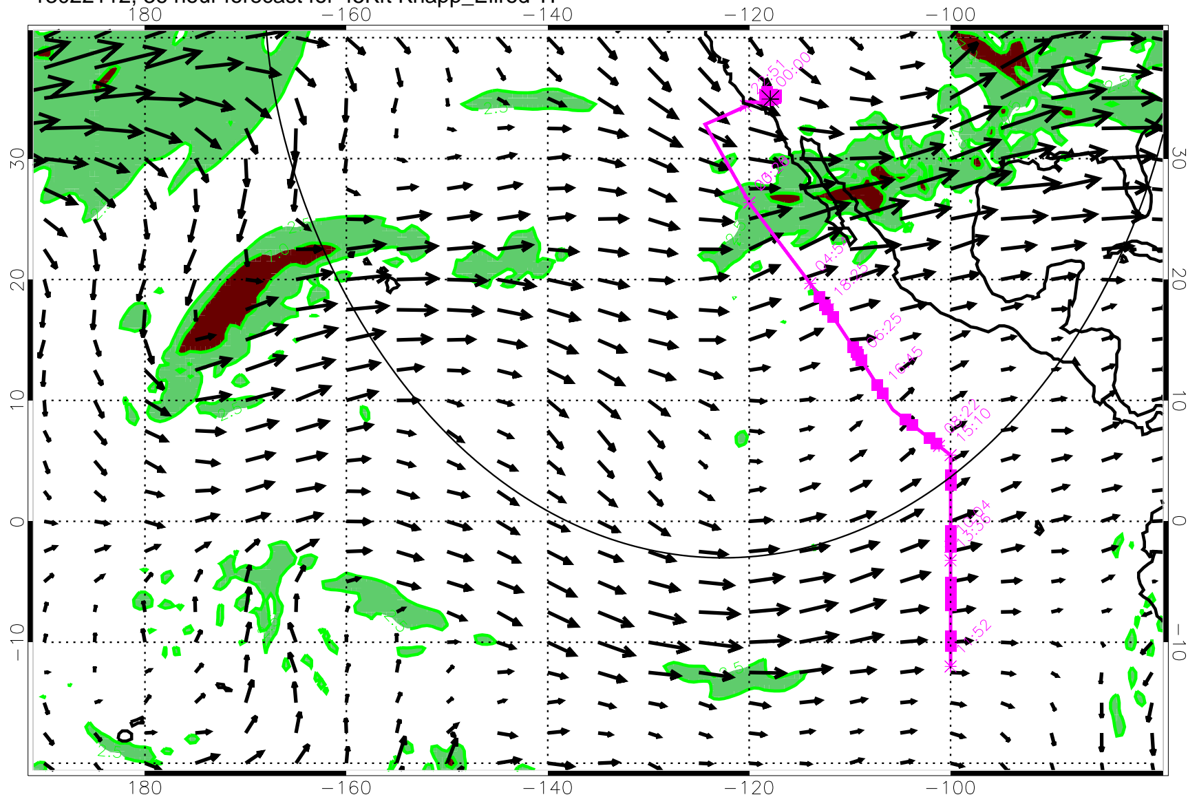
13022112, 36 hour forecast for 45Kft Knapp_Ellrod TI
