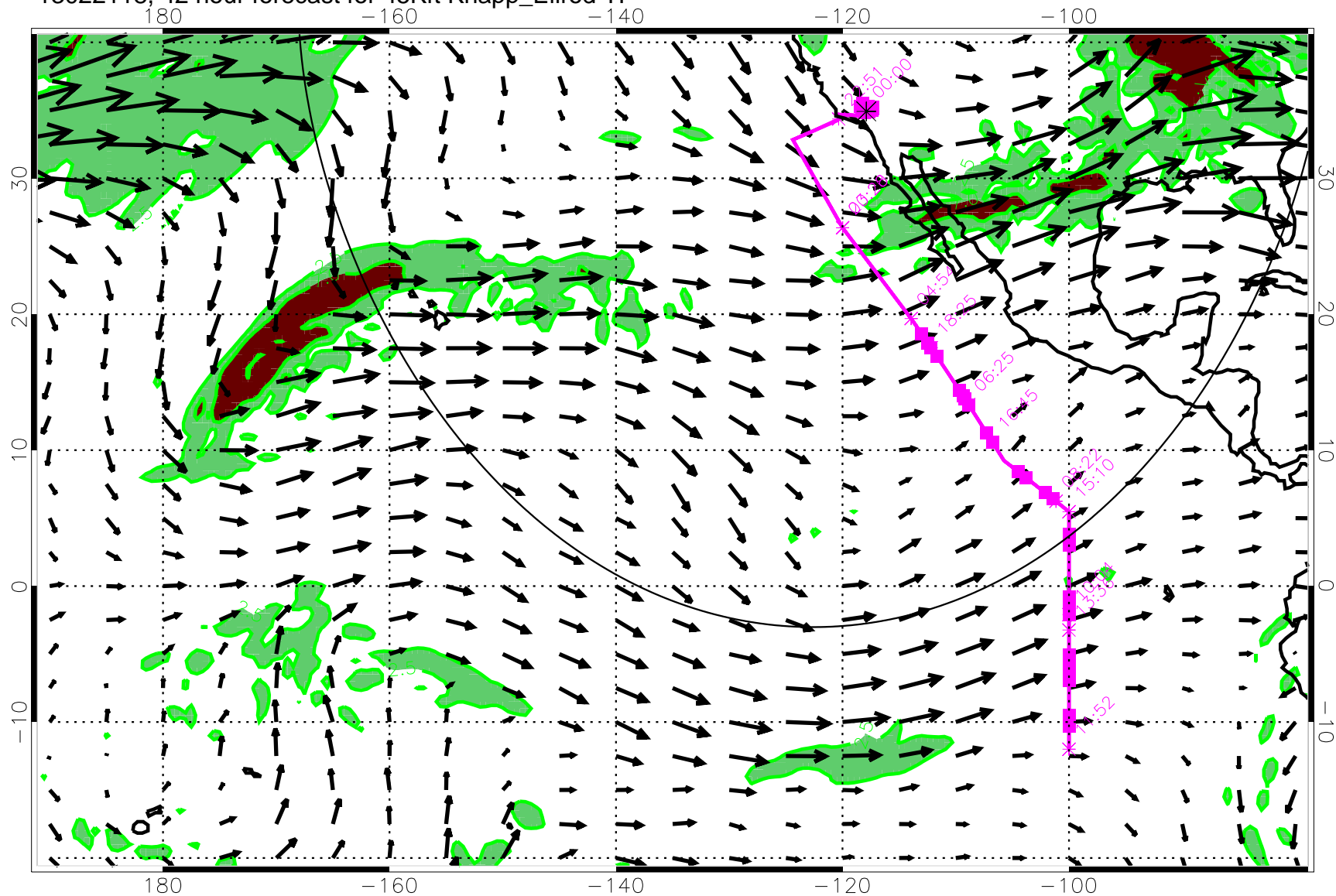
13022118, 42 hour forecast for 45Kft Knapp_Ellrod TI
