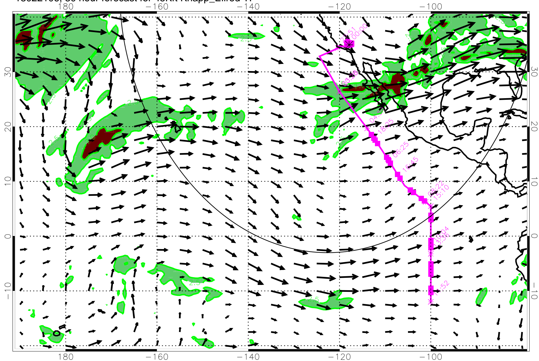
13022106, 30 hour forecast for 45Kft Knapp_Ellrod TI
