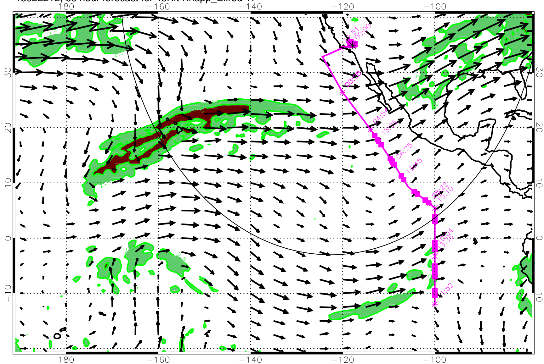
13022212, 60 hour forecast for 45Kft Knapp_Ellrod TI
