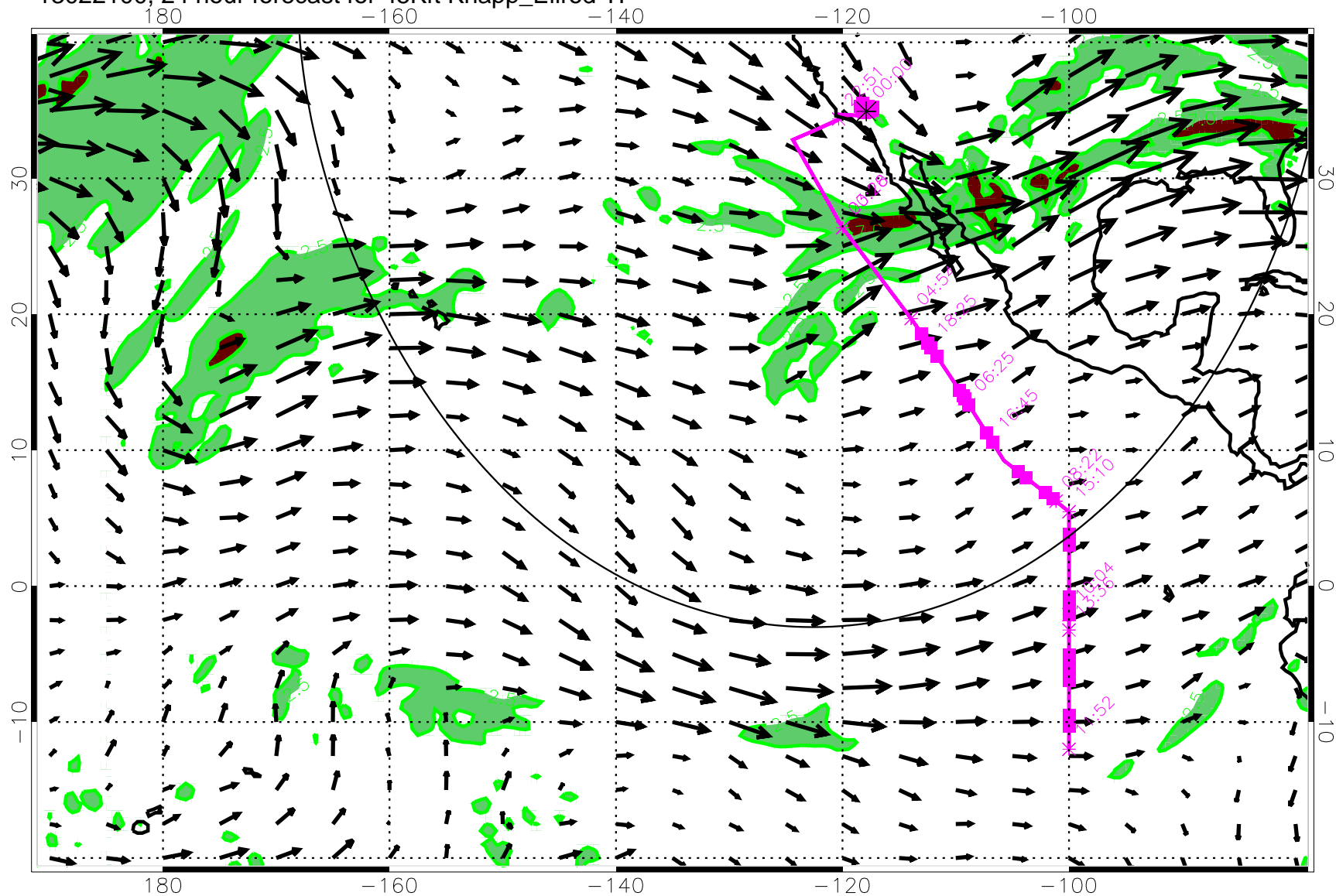
13022100, 24 hour forecast for 45Kft Knapp_Ellrod TI
