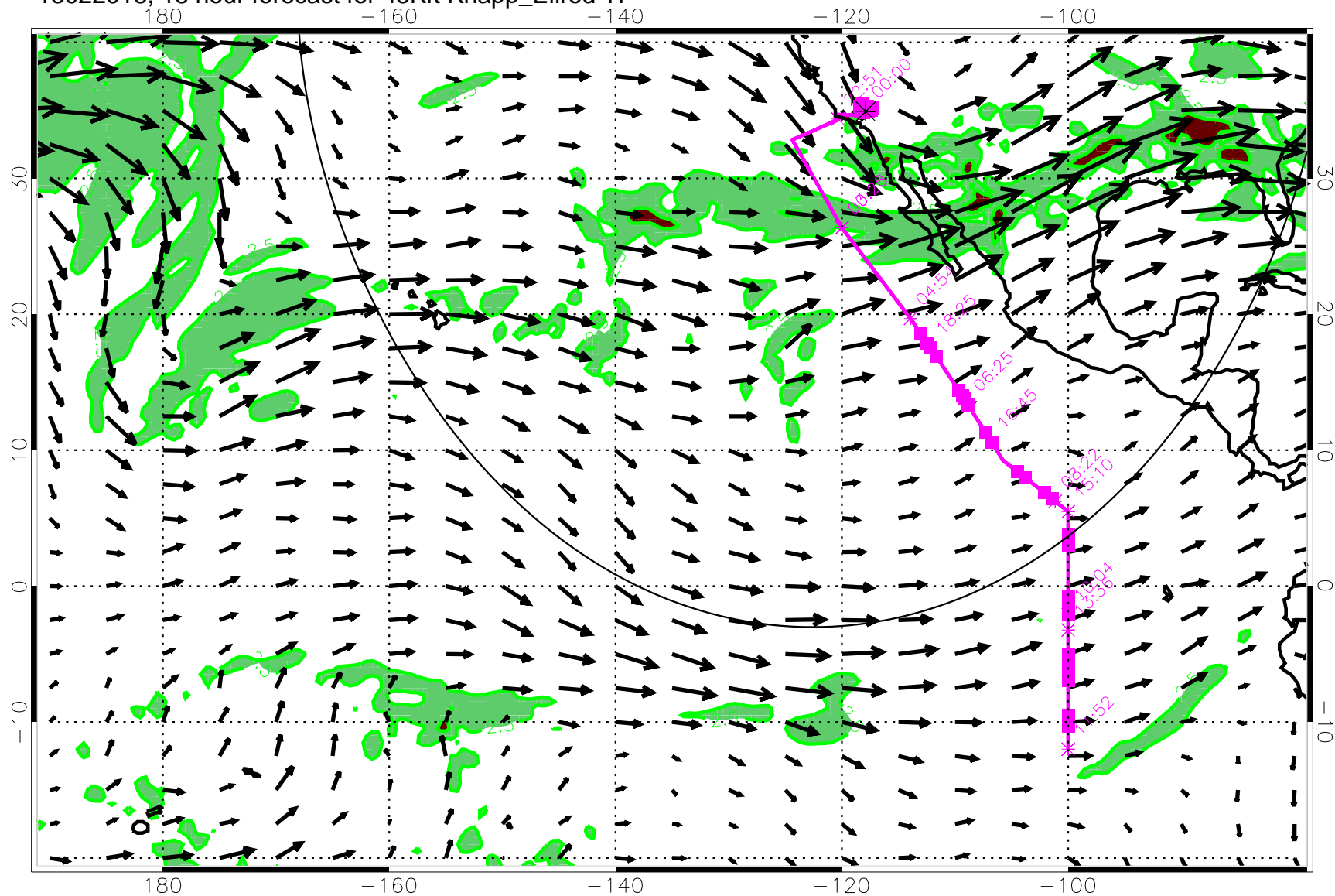
13022018, 18 hour forecast for 45Kft Knapp_Ellrod TI
