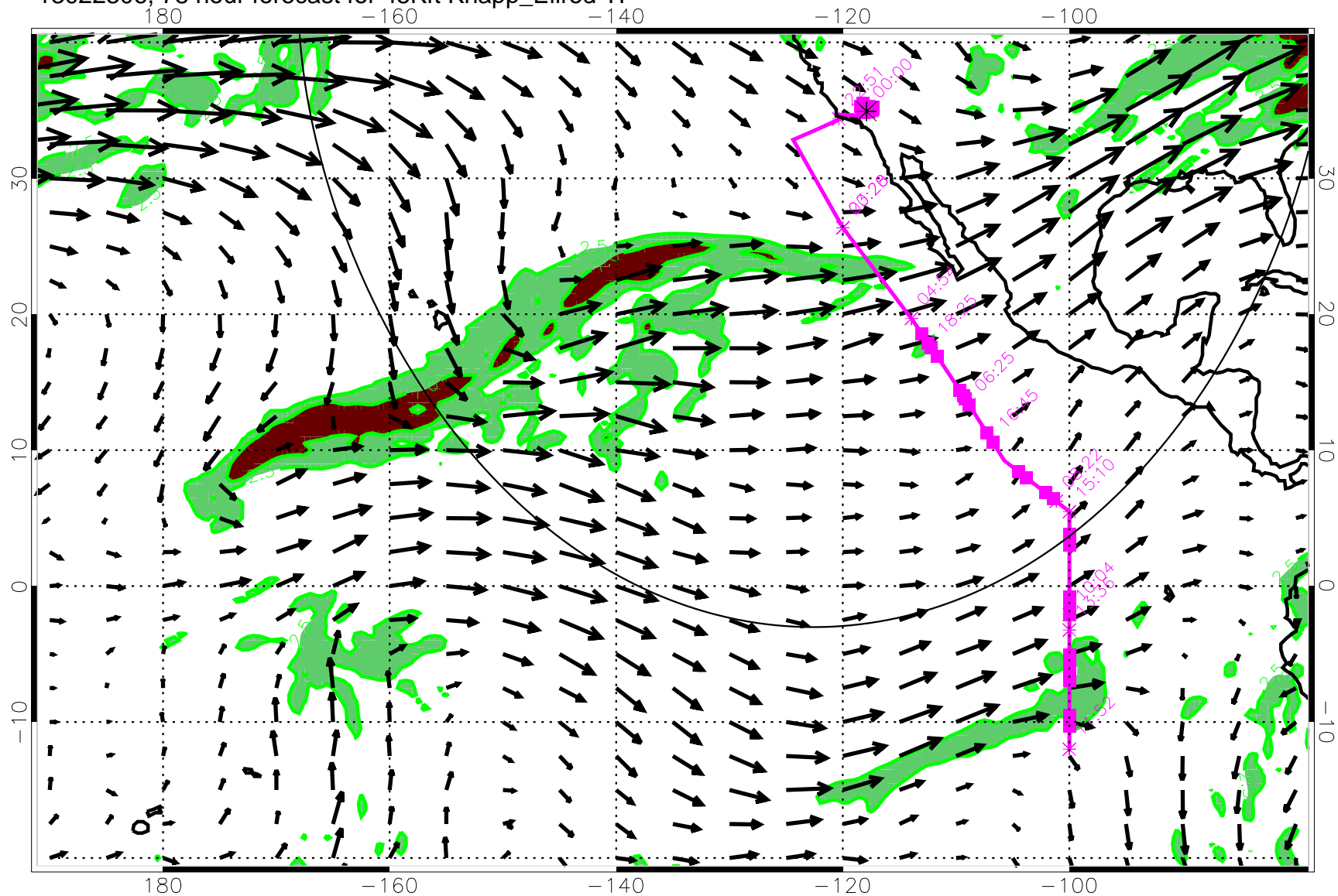
13022306, 78 hour forecast for 45Kft Knapp_Ellrod TI
