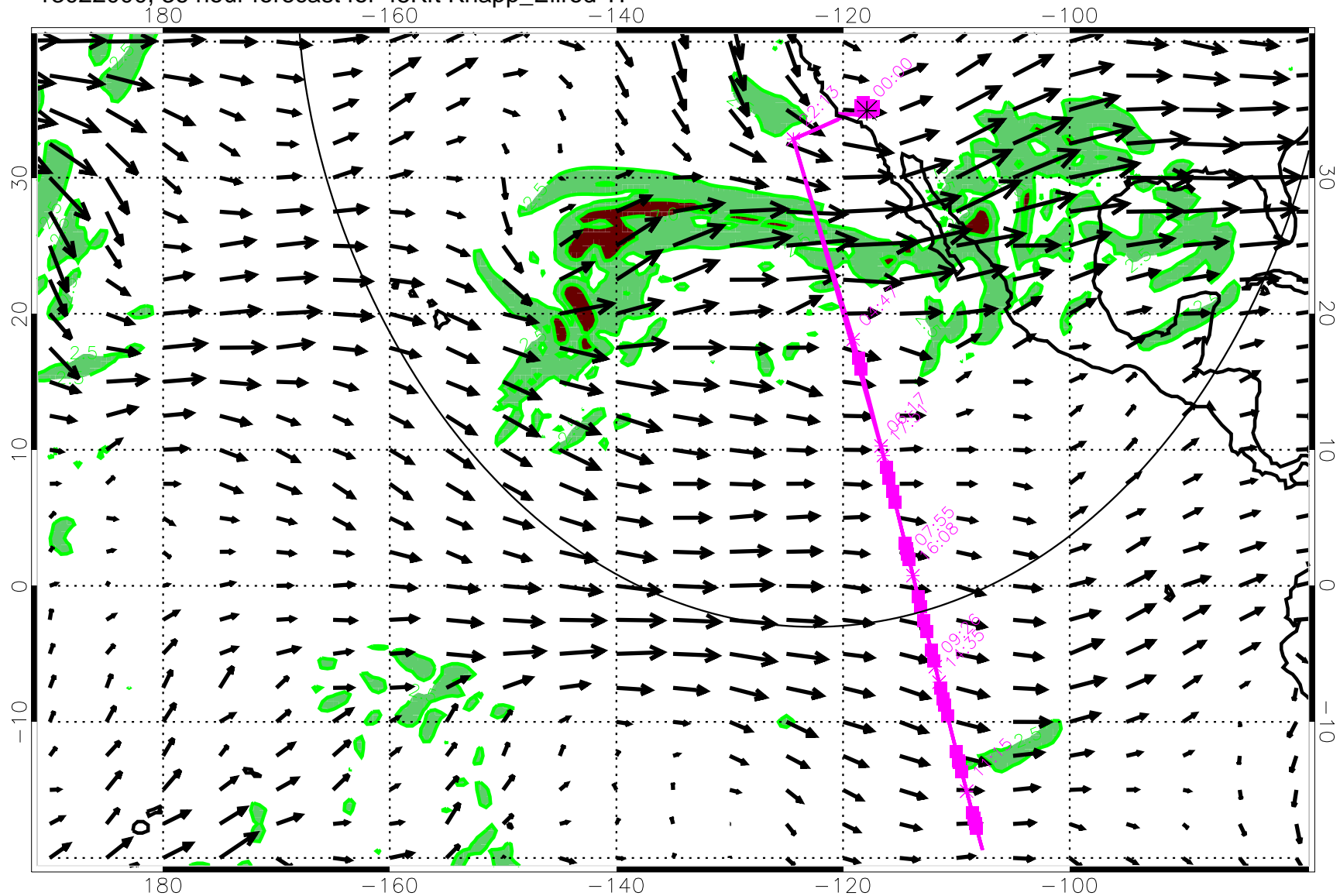
13022000, 36 hour forecast for 45Kft Knapp_Ellrod TI
