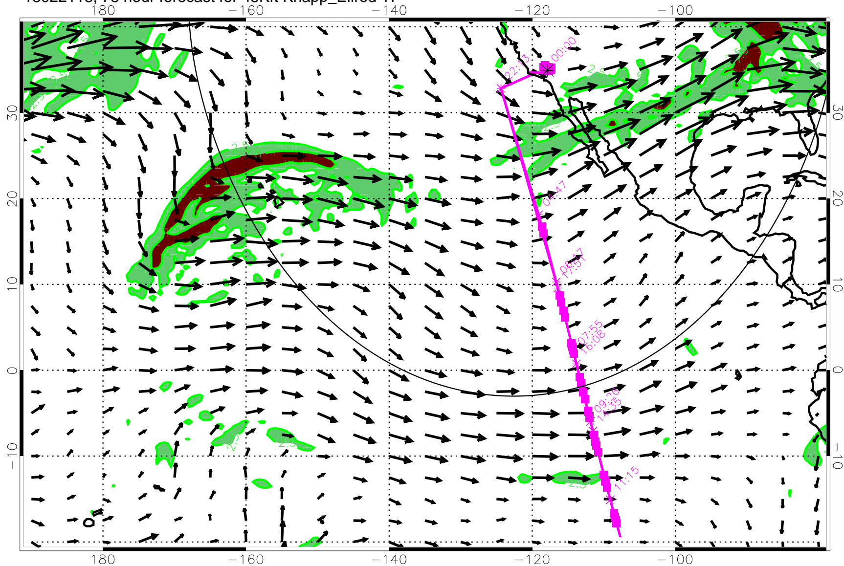
13022118, 78 hour forecast for 45Kft Knapp_Ellrod TI
