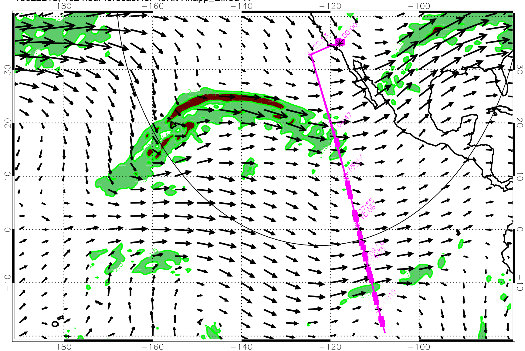
13022218, 102 hour forecast for 45Kft Knapp_Ellrod T1
