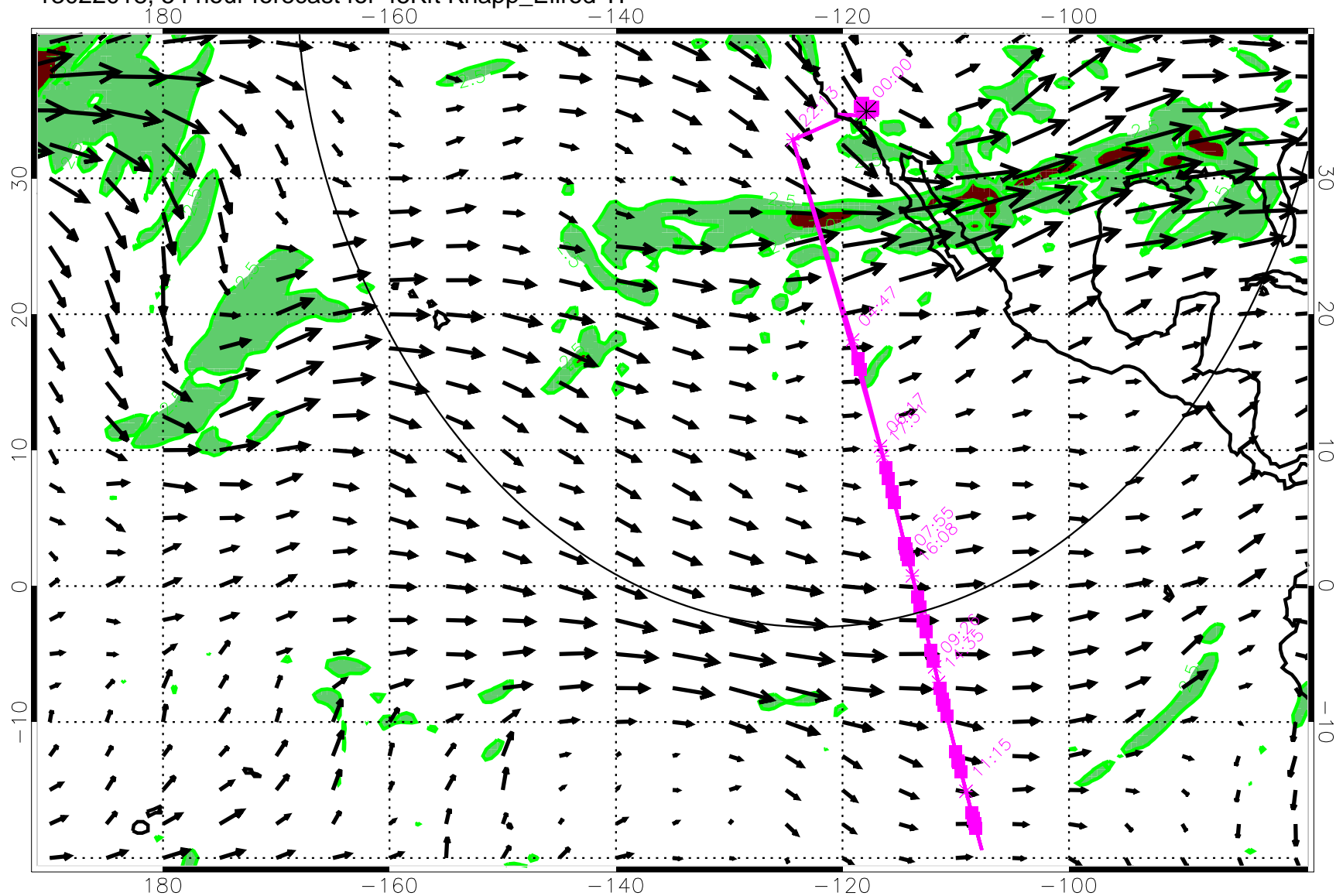
13022018, 54 hour forecast for 45Kft Knapp_Ellrod TI
