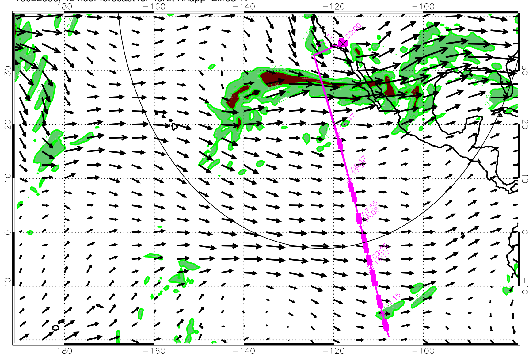
13022006, 42 hour forecast for 45Kft Knapp_Ellrod TI
