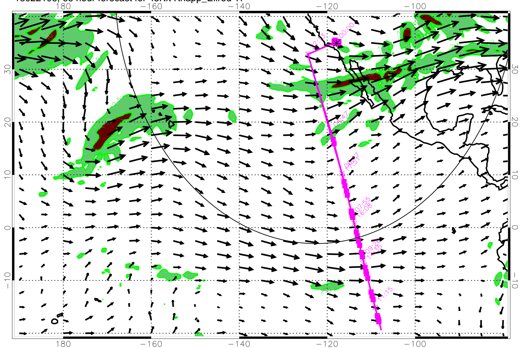
13022106, 66 hour forecast for 45Kft Knapp_Ellrod TI
