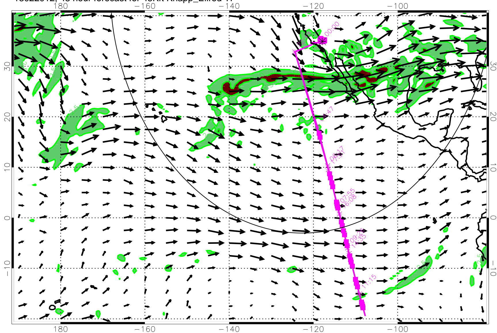
13022012, 48 hour forecast for 45Kft Knapp_Ellrod TI
