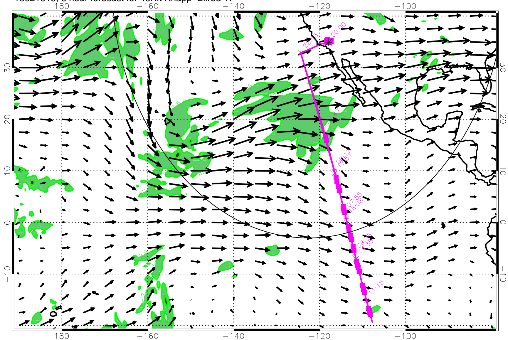
13021818, 6 hour forecast for 45Kft Knapp_Ellrod TI
