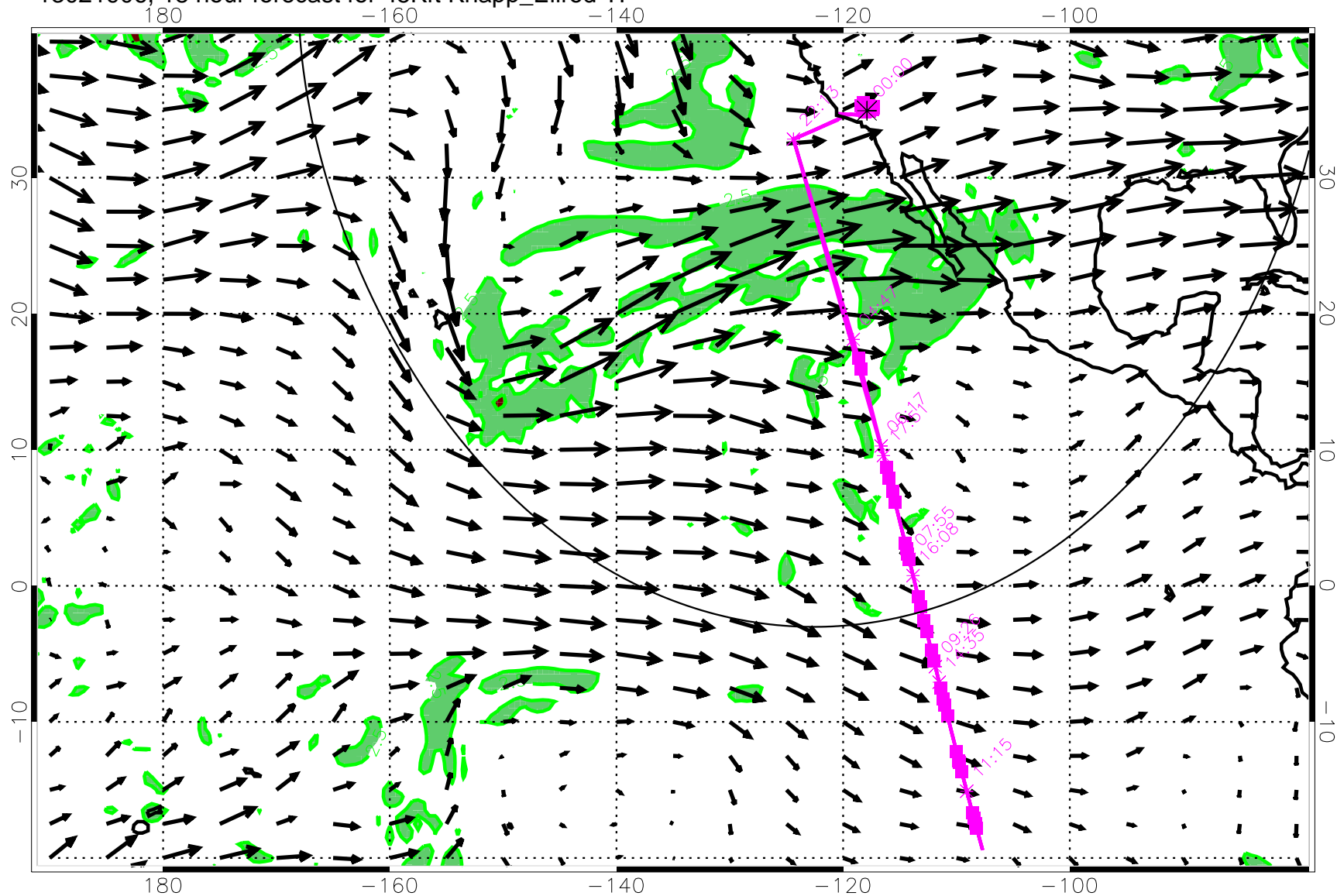
13021906, 18 hour forecast for 45Kft Knapp_Ellrod TI
