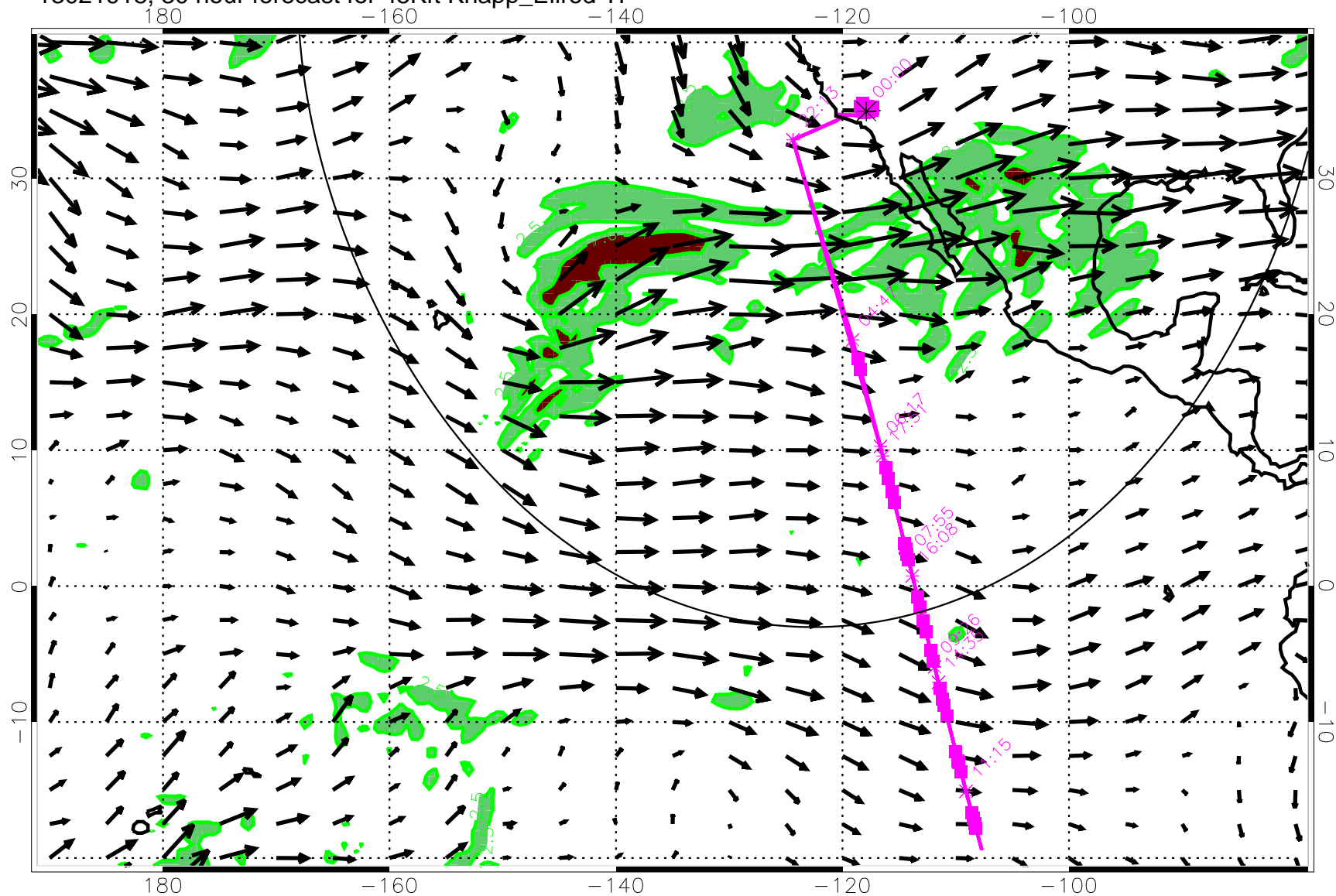
13021918, 30 hour forecast for 45Kft Knapp_Ellrod TI
