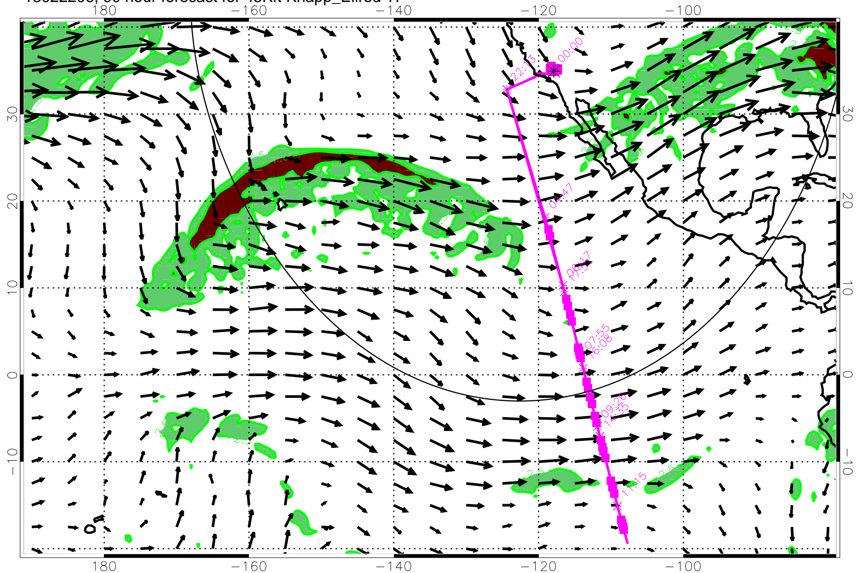
13022206, 90 hour forecast for 45Kft Knapp_Ellrod TI
