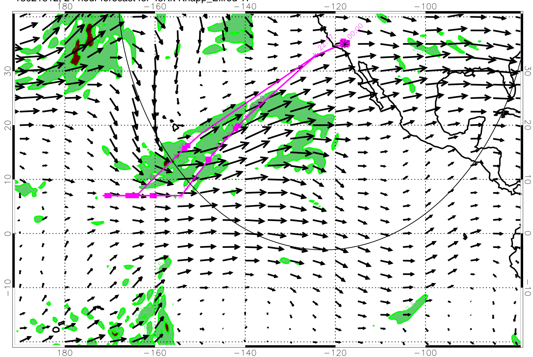
13021812, 24 hour forecast for 45Kft Knapp_Ellrod TI
