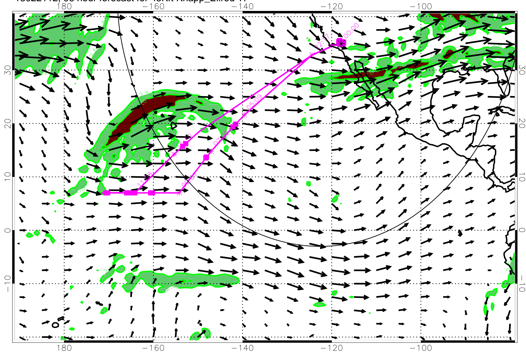
13022112, 96 hour forecast for 45Kft Knapp_Ellrod TI
