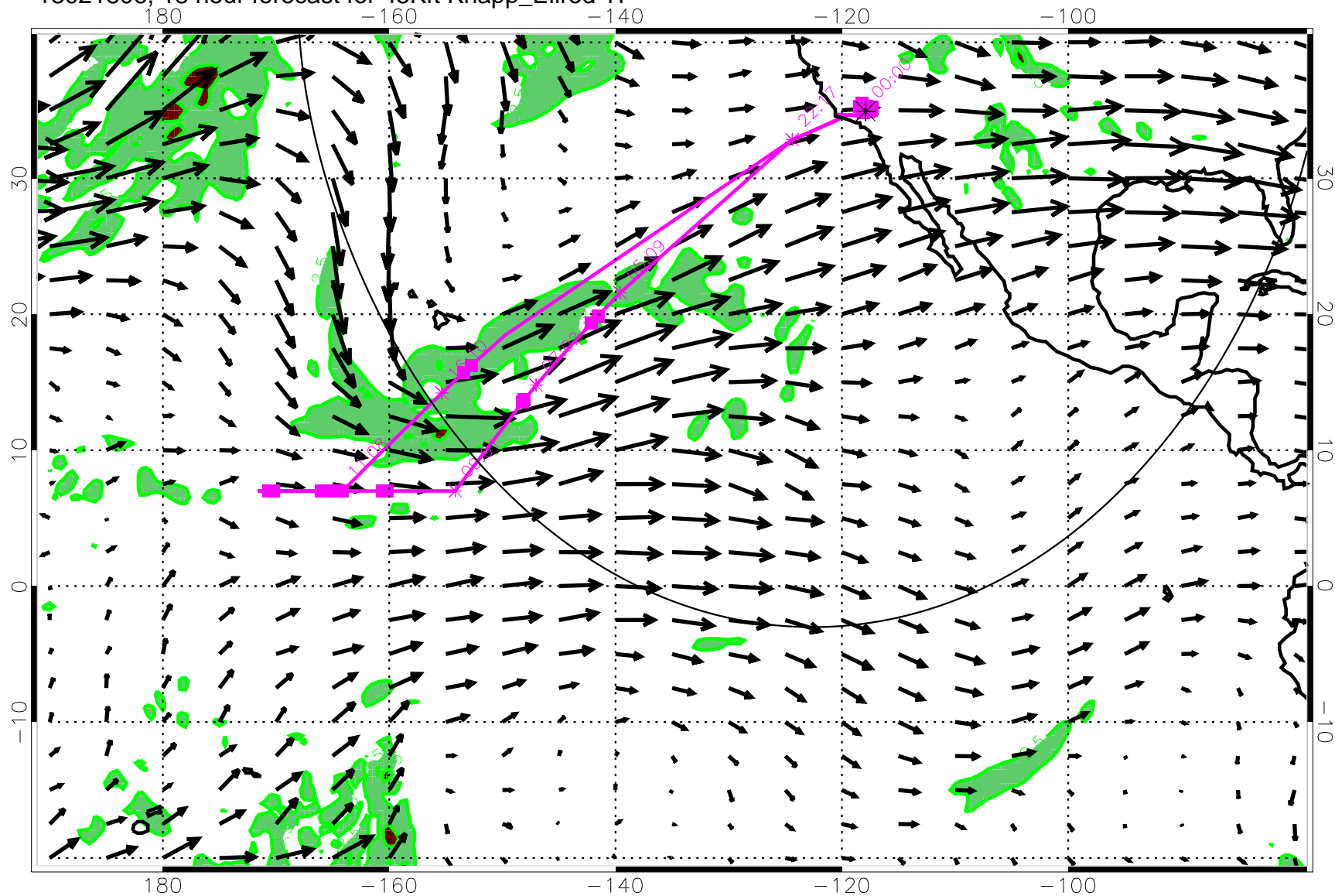
13021806, 18 hour forecast for 45Kft Knapp_Ellrod TI
