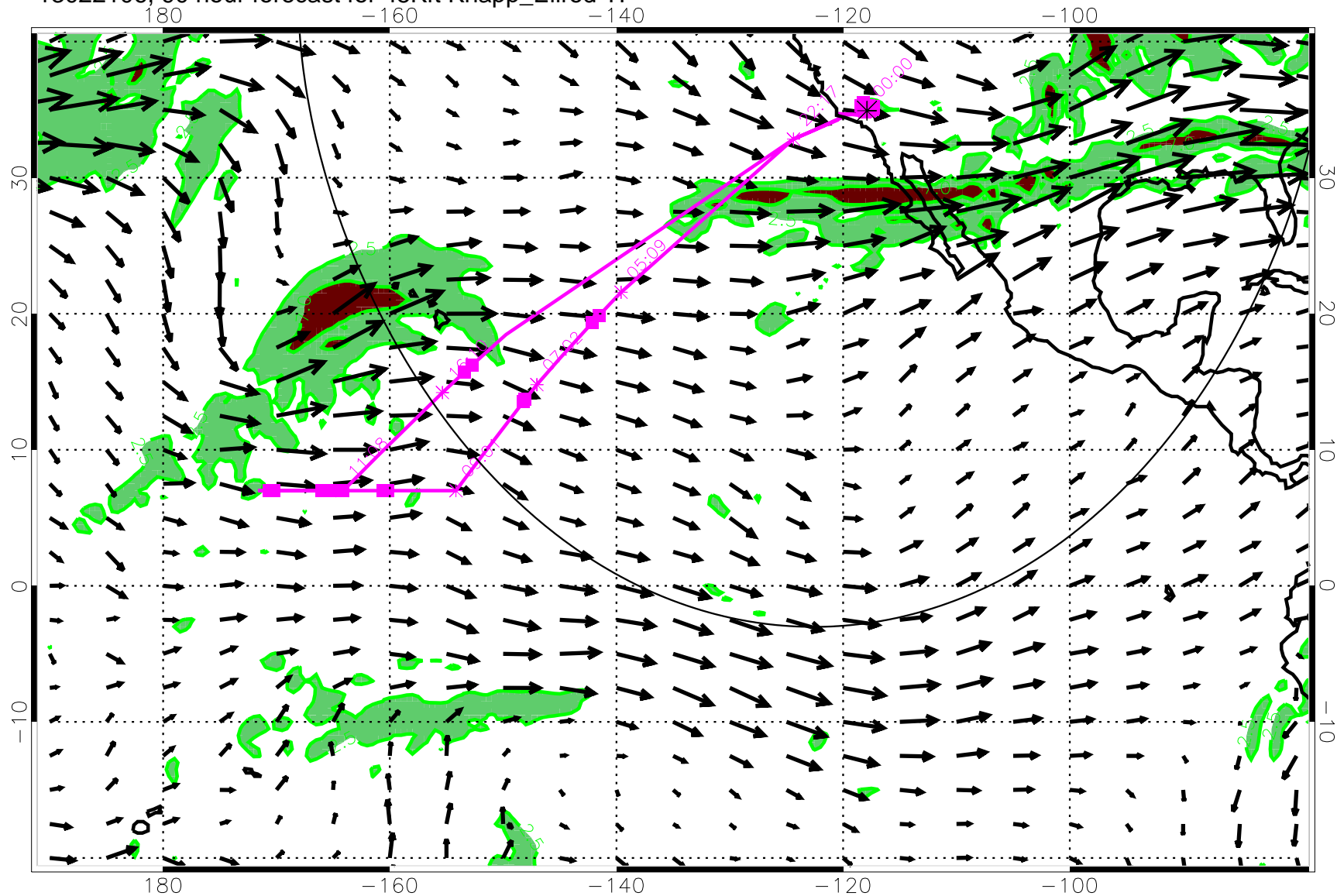
13022106, 90 hour forecast for 45Kft Knapp_Ellrod TI
