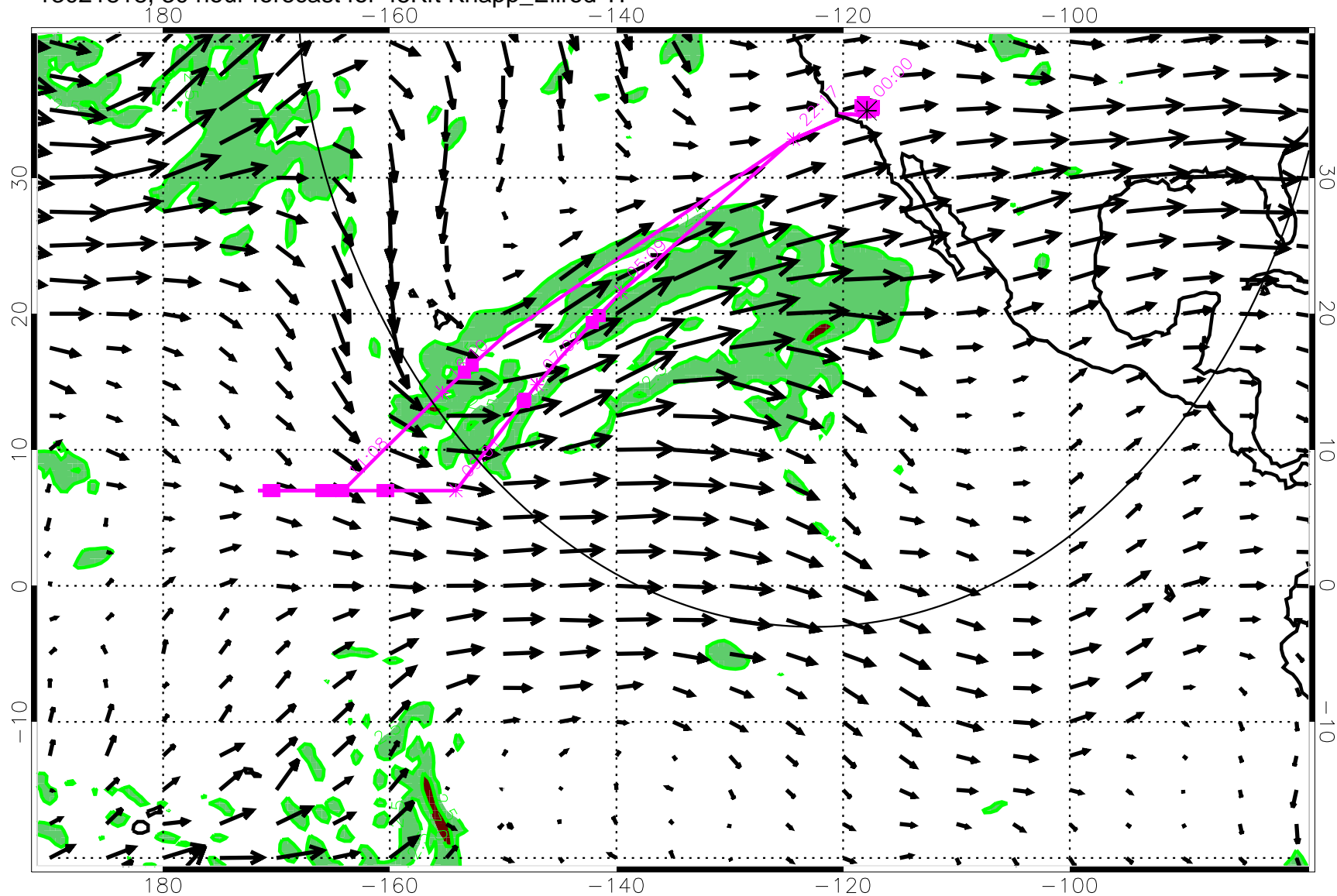
13021818, 30 hour forecast for 45Kft Knapp_Ellrod TI
