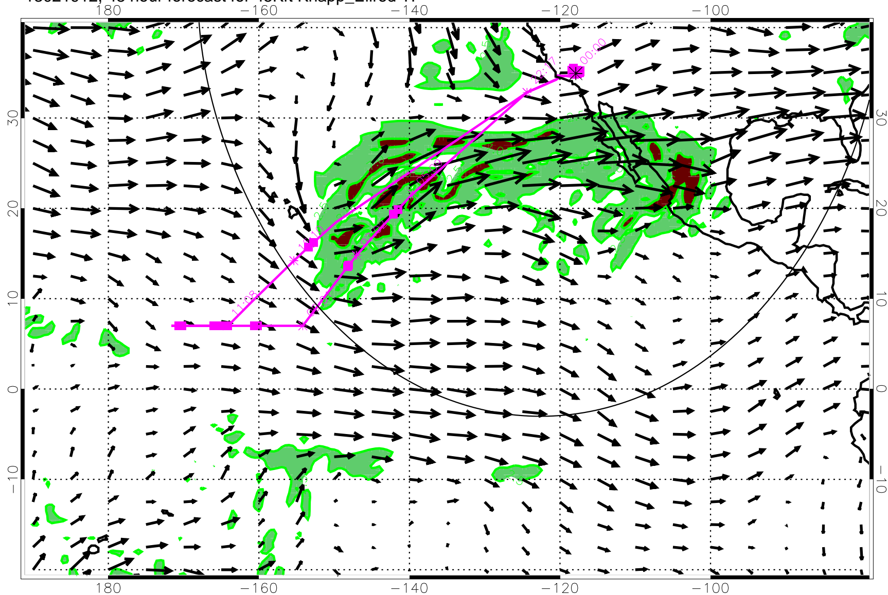
13021912, 48 hour forecast for 45Kft Knapp_Ellrod TI
