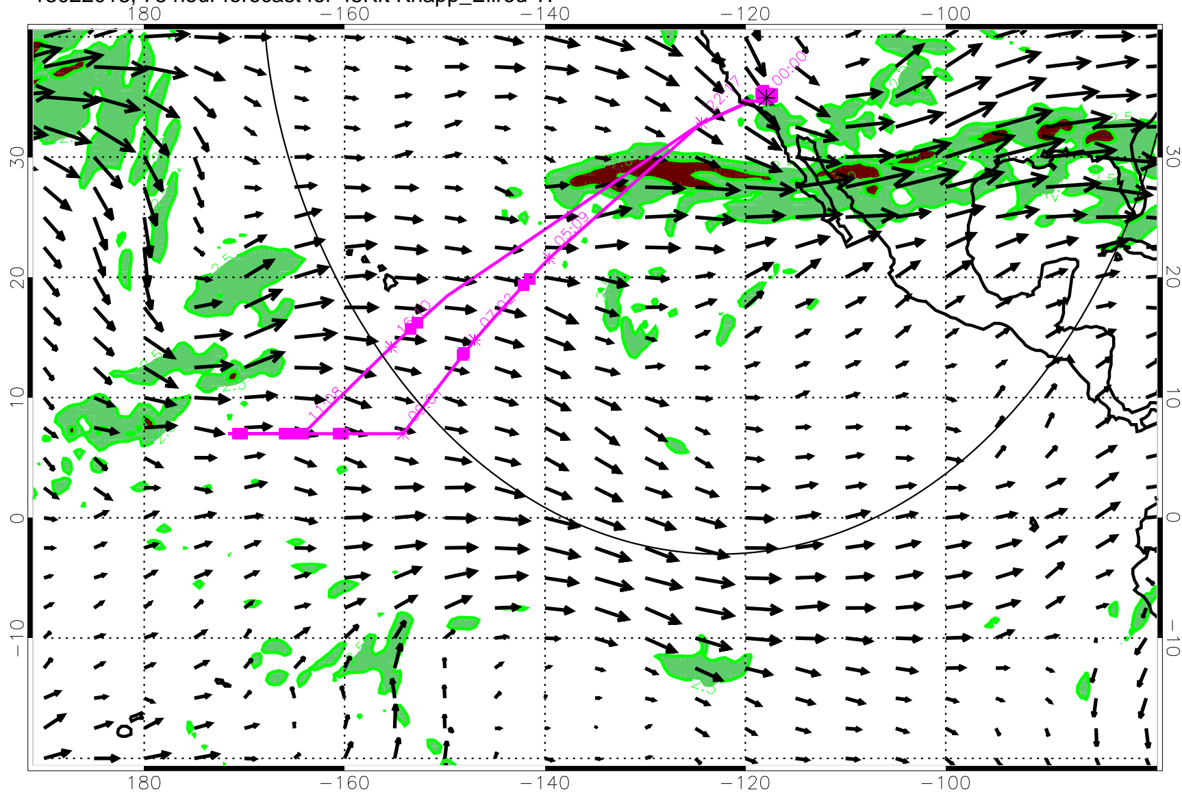
13022018, 78 hour forecast for 45Kft Knapp_Ellrod TI
