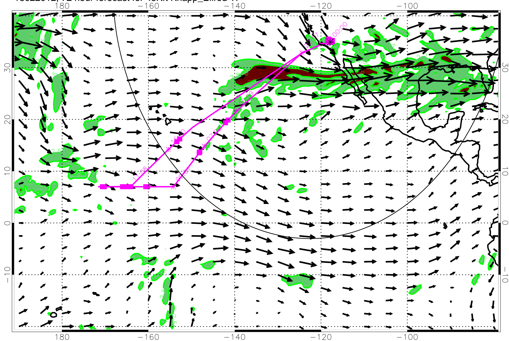
13022012, 72 hour forecast for 45Kft Knapp_Ellrod TI
