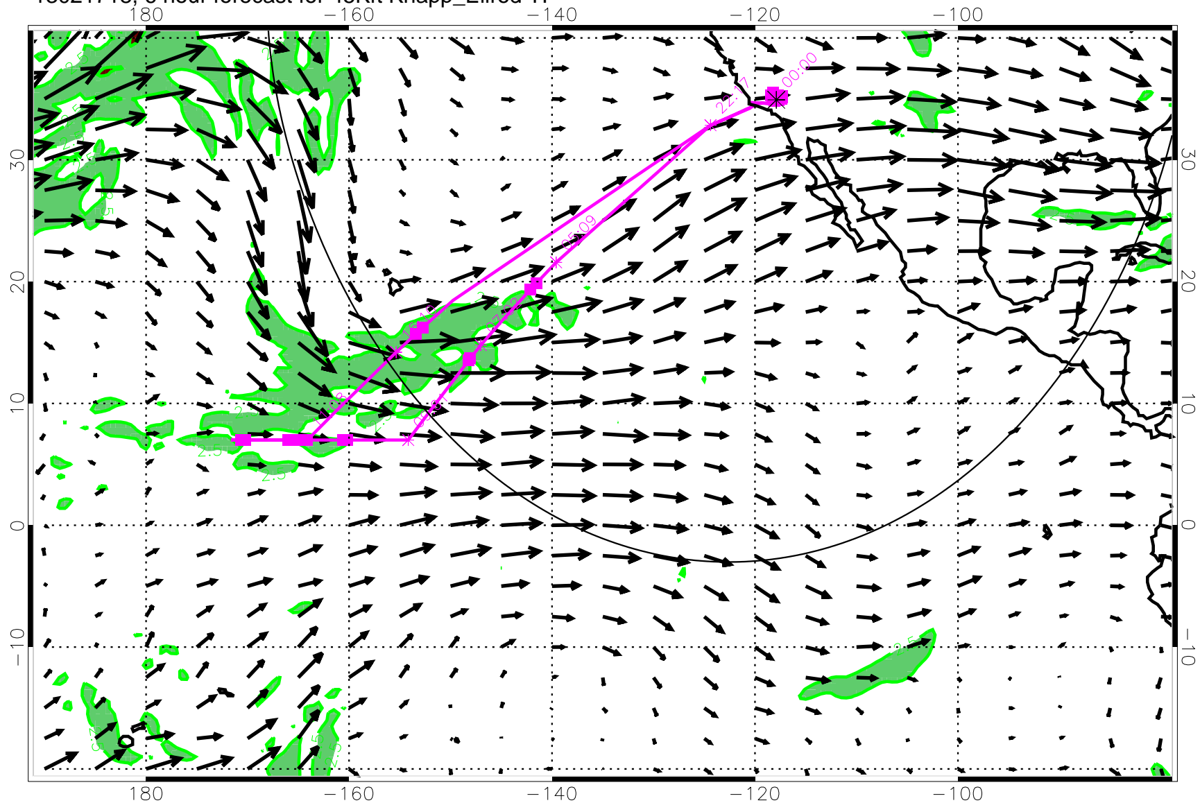
13021718, 6 hour forecast for 45Kft Knapp_Ellrod TI
