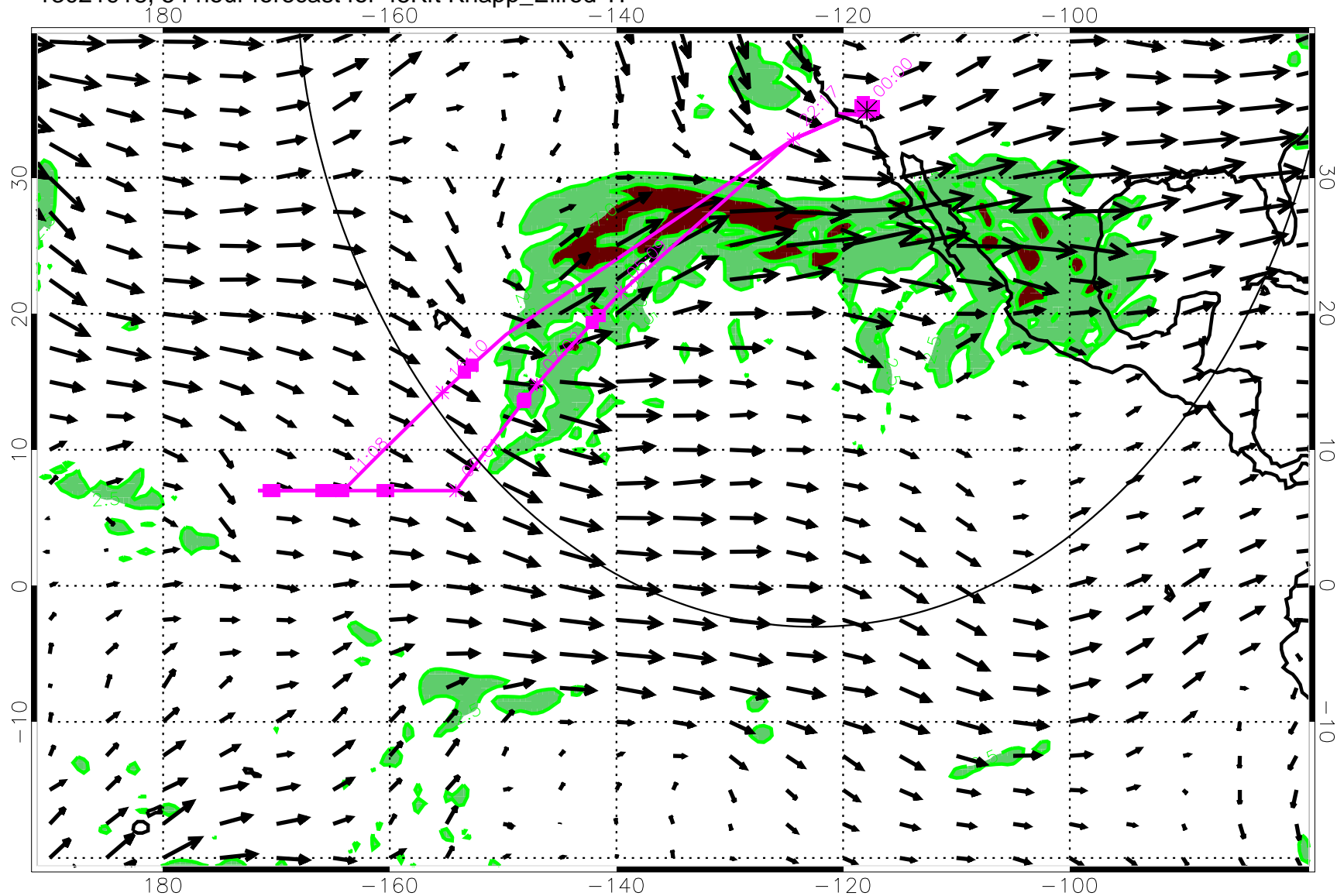
13021918, 54 hour forecast for 45Kft Knapp_Ellrod TI
