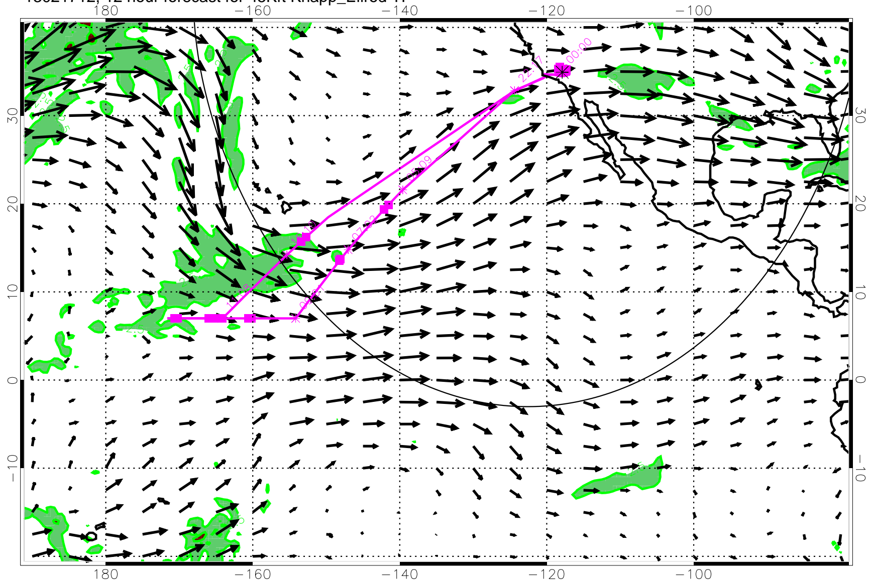
13021712, 12 hour forecast for 45Kft Knapp_Ellrod TI
