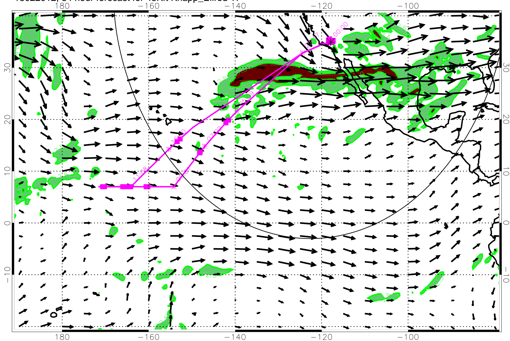
13022012, 84 hour forecast for 45Kft Knapp_Ellrod TI
