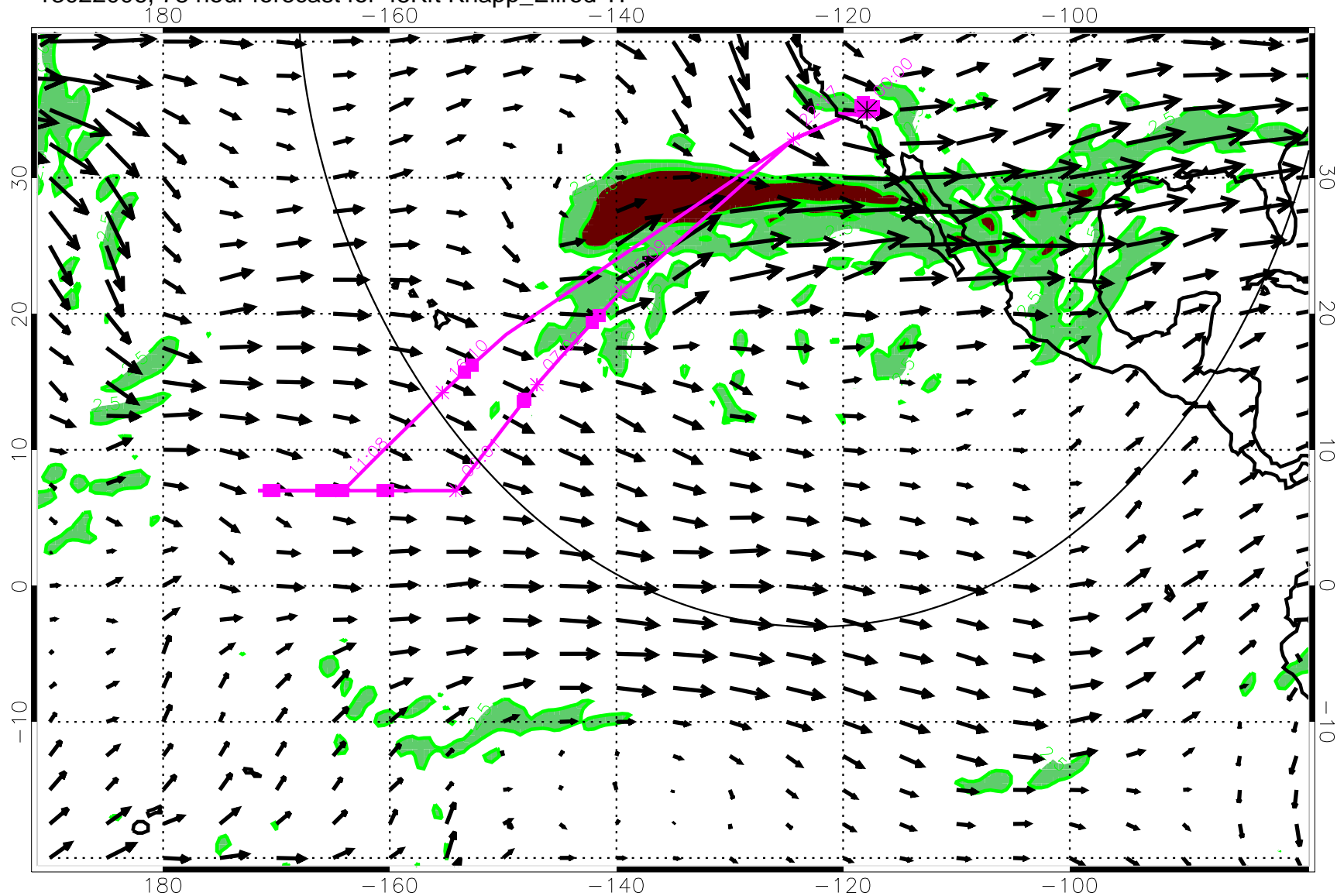
13022006, 78 hour forecast for 45Kft Knapp_Ellrod TI
