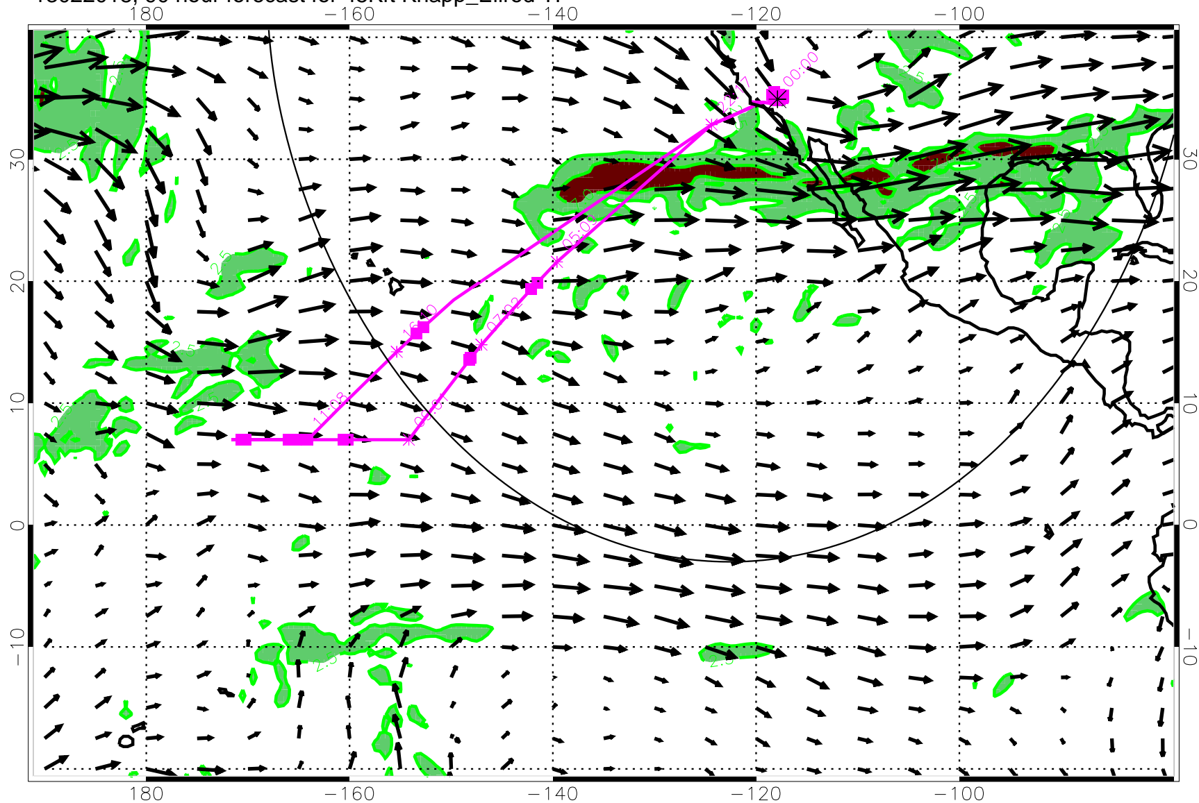
13022018, 90 hour forecast for 45Kft Knapp_Ellrod TI
