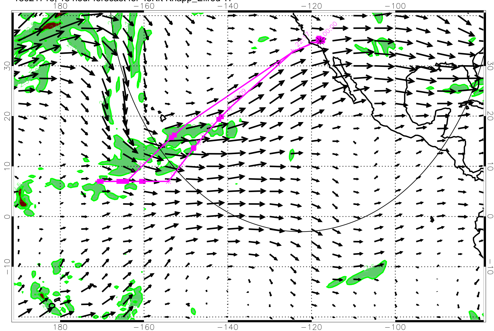
13021718, 18 hour forecast for 45Kft Knapp_Ellrod TI
