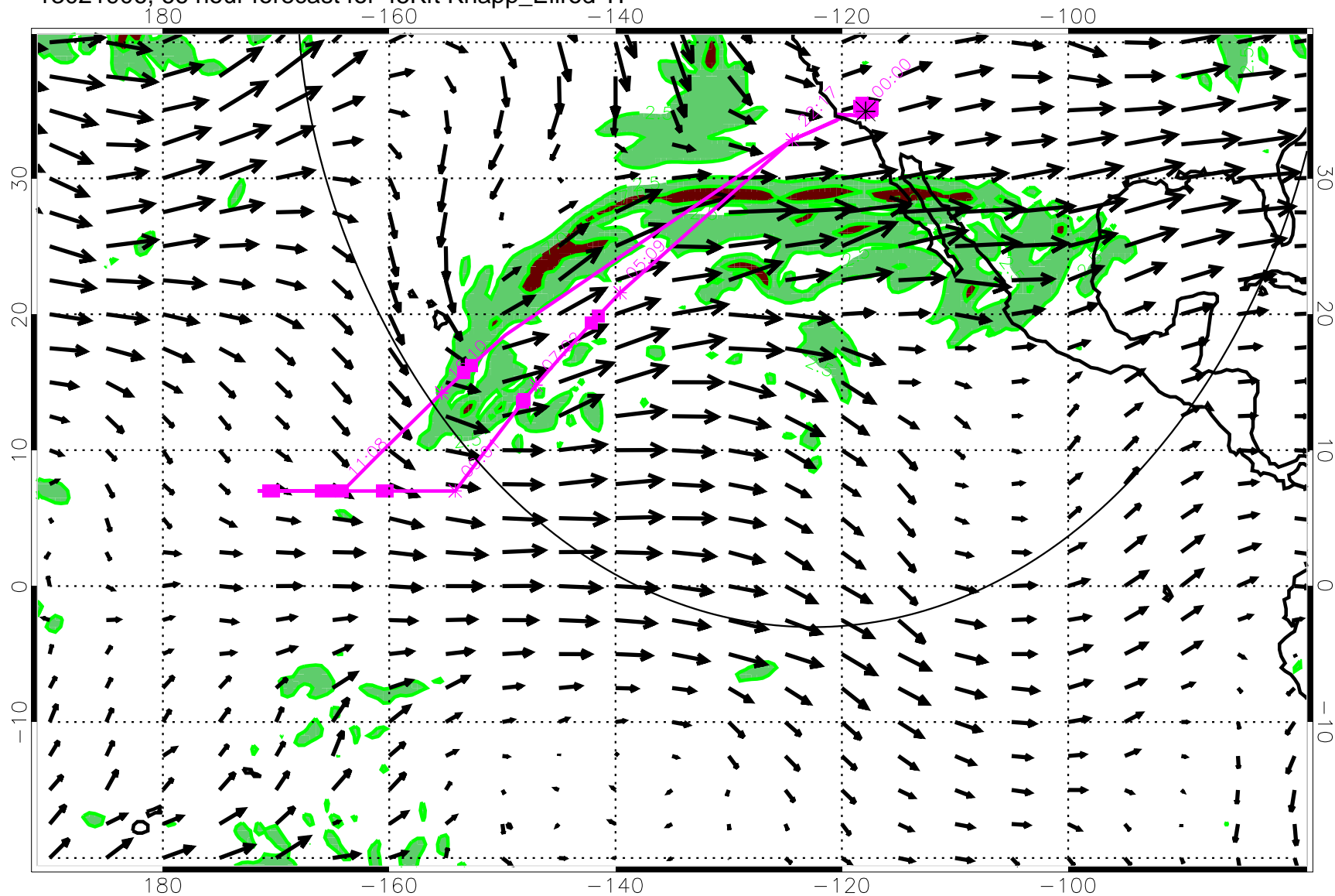
13021906, 66 hour forecast for 45Kft Knapp_Ellrod TI
