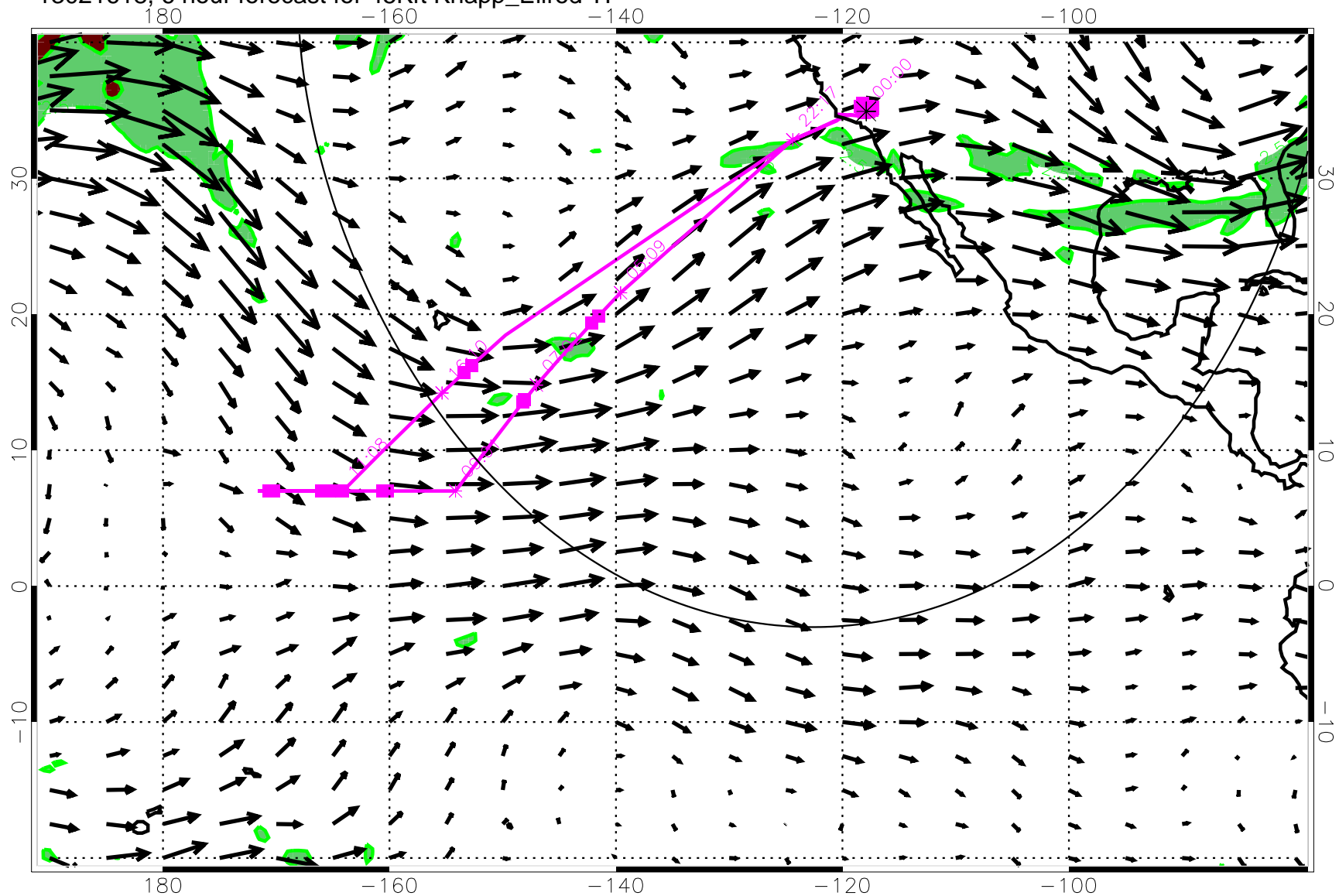
13021618, 6 hour forecast for 45Kft Knapp_Ellrod TI
