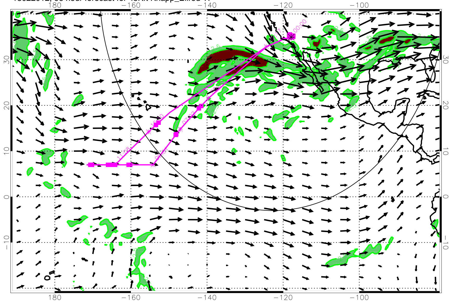
13022012, 96 hour forecast for 45Kft Knapp_Ellrod TI
