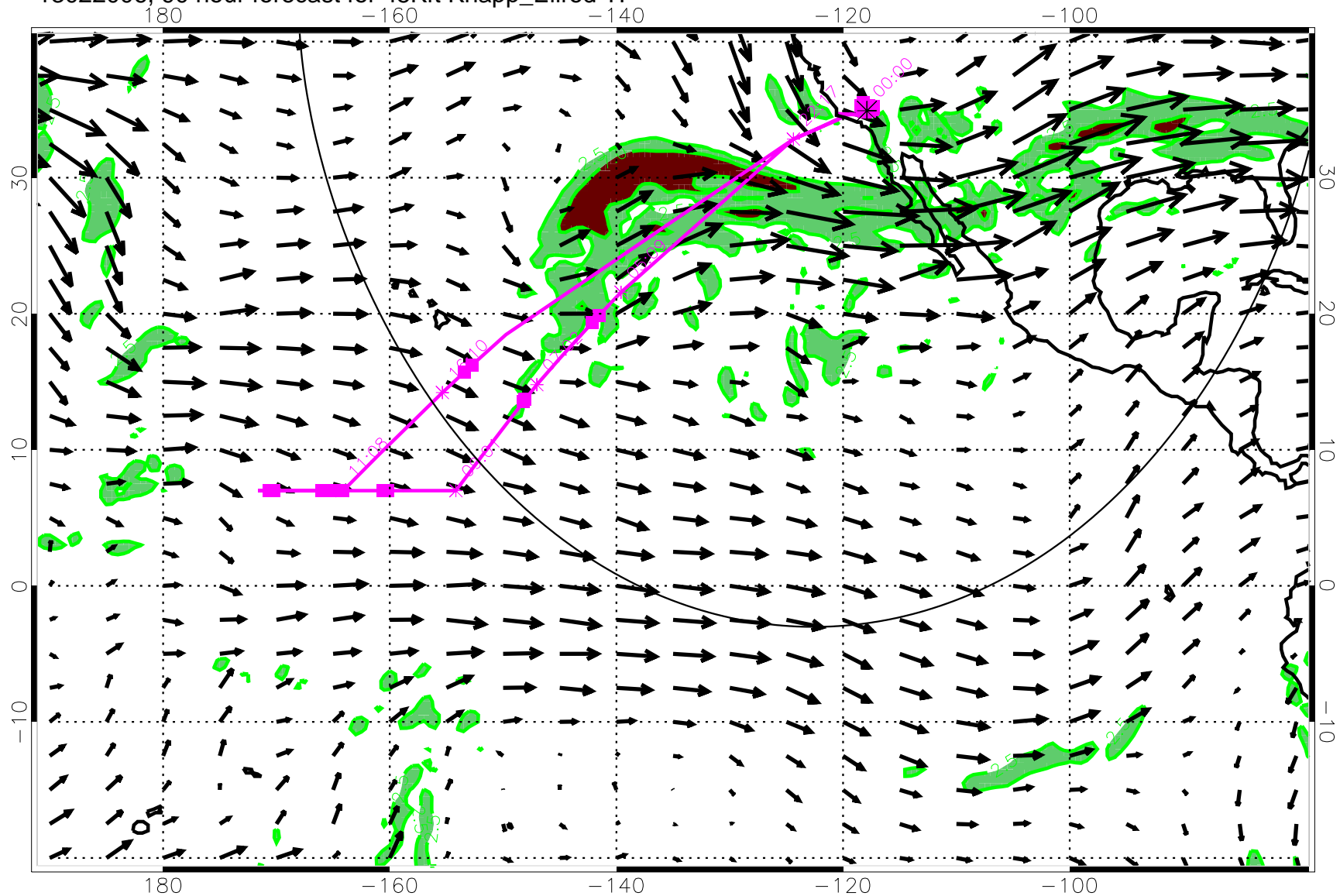
13022006, 90 hour forecast for 45Kft Knapp_Ellrod TI
