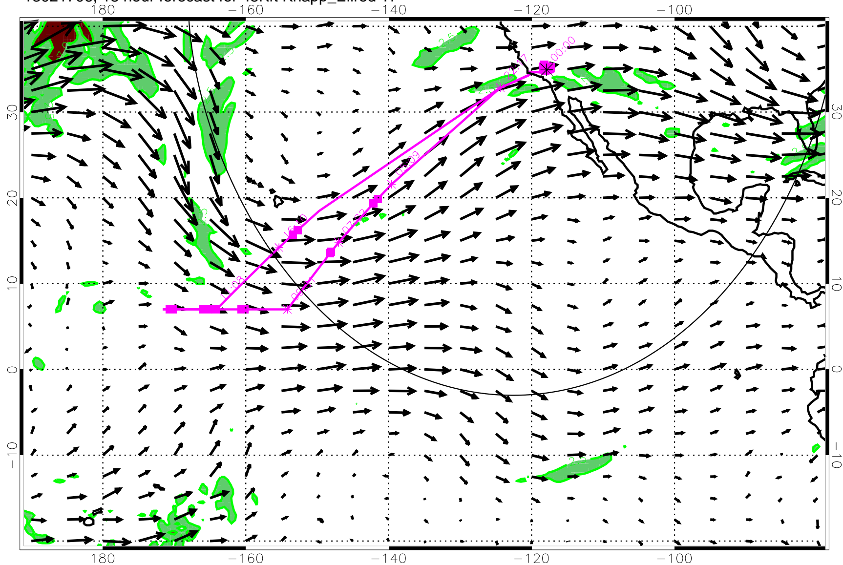
13021706, 18 hour forecast for 45Kft Knapp_Ellrod TI
