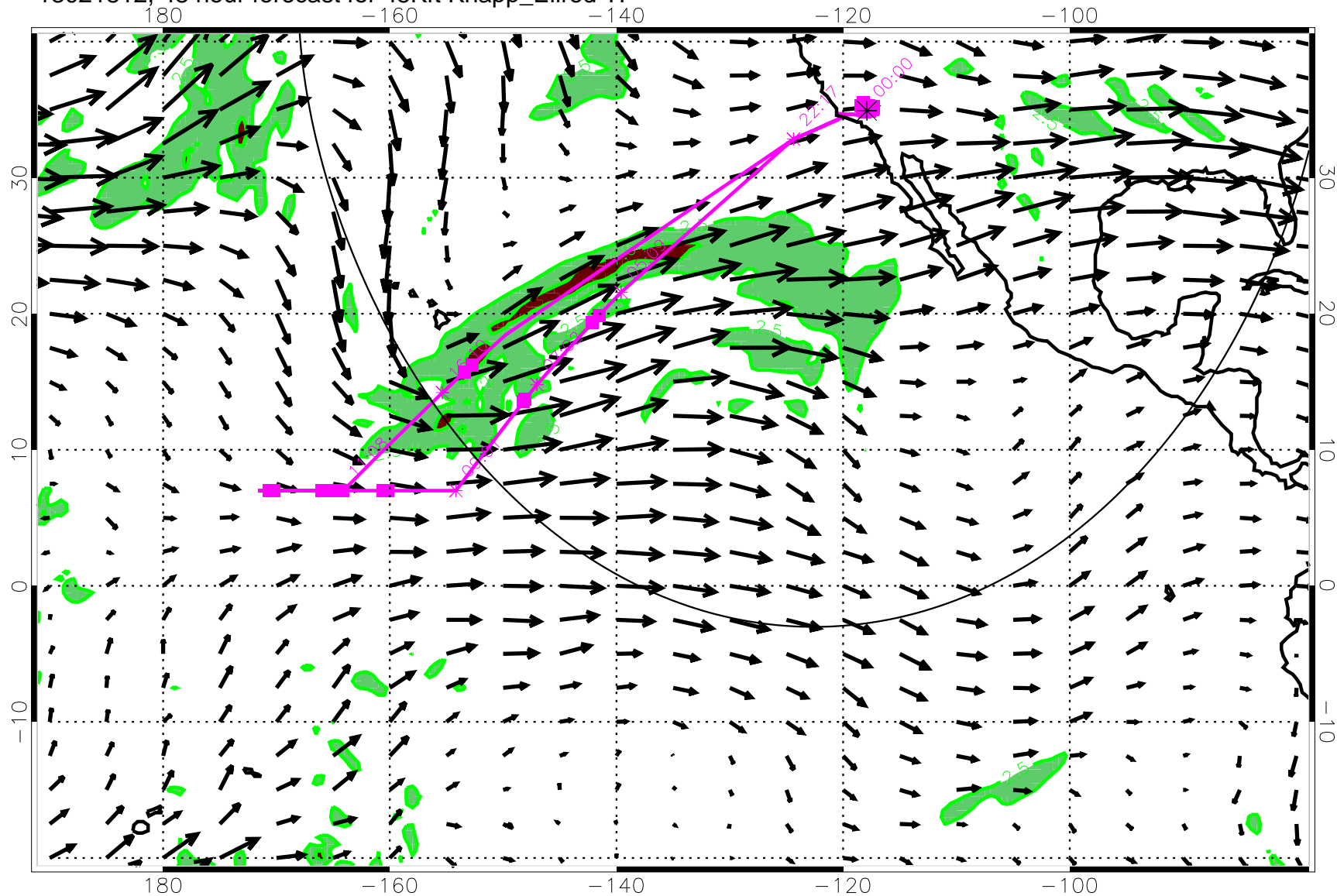
13021812, 48 hour forecast for 45Kft Knapp_Ellrod TI
