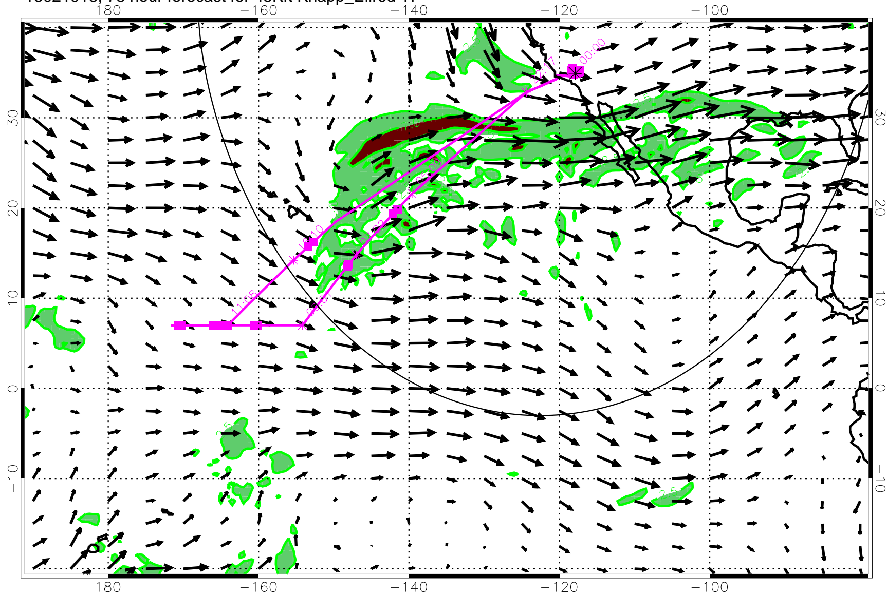
13021918, 78 hour forecast for 45Kft Knapp_Ellrod TI
