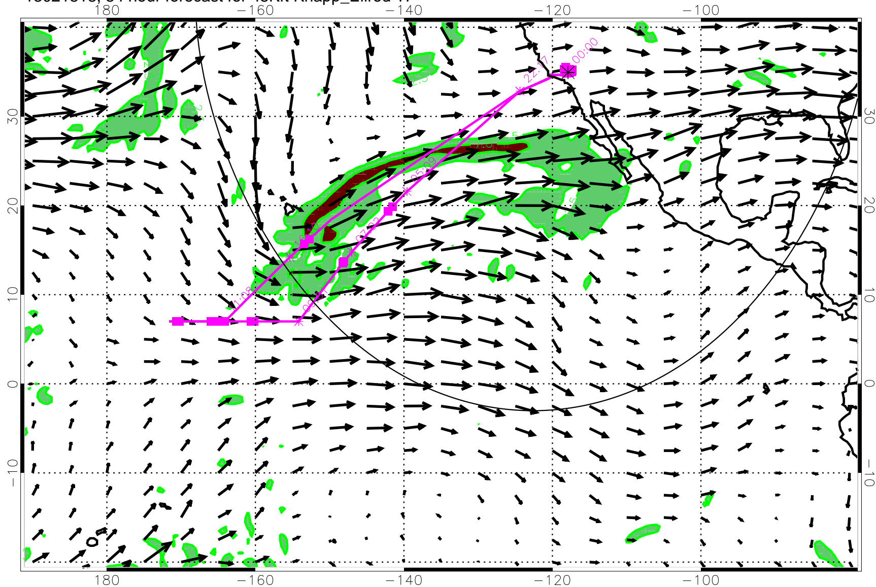
13021818, 54 hour forecast for 45Kft Knapp_Ellrod TI
