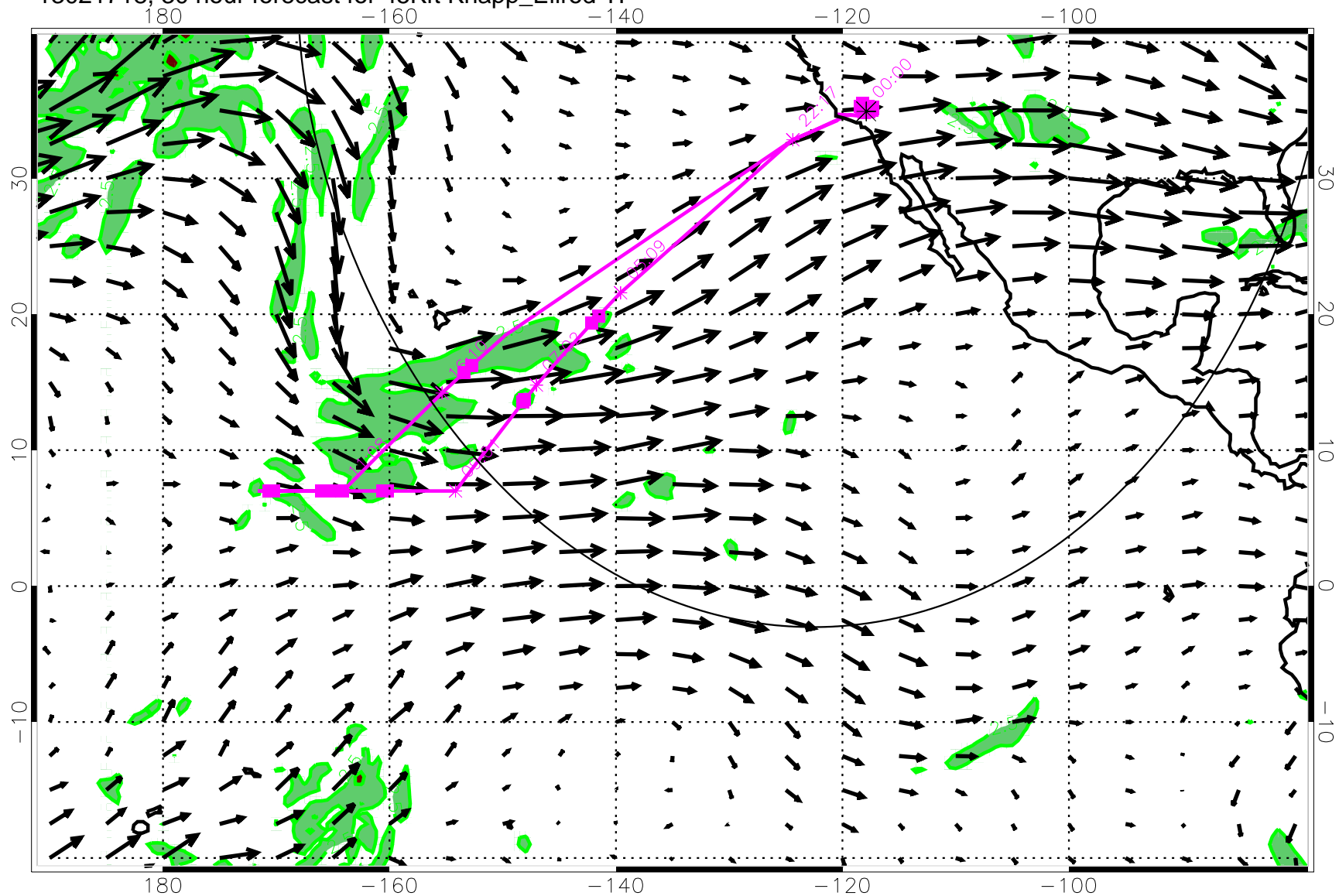
13021718, 30 hour forecast for 45Kft Knapp_Ellrod TI
