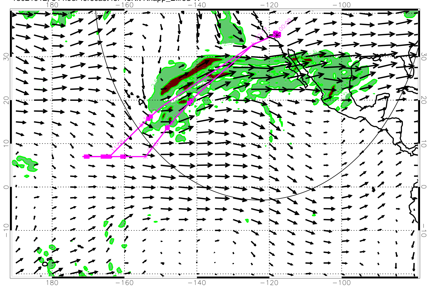
13021912, 84 hour forecast for 45Kft Knapp_Ellrod TI
