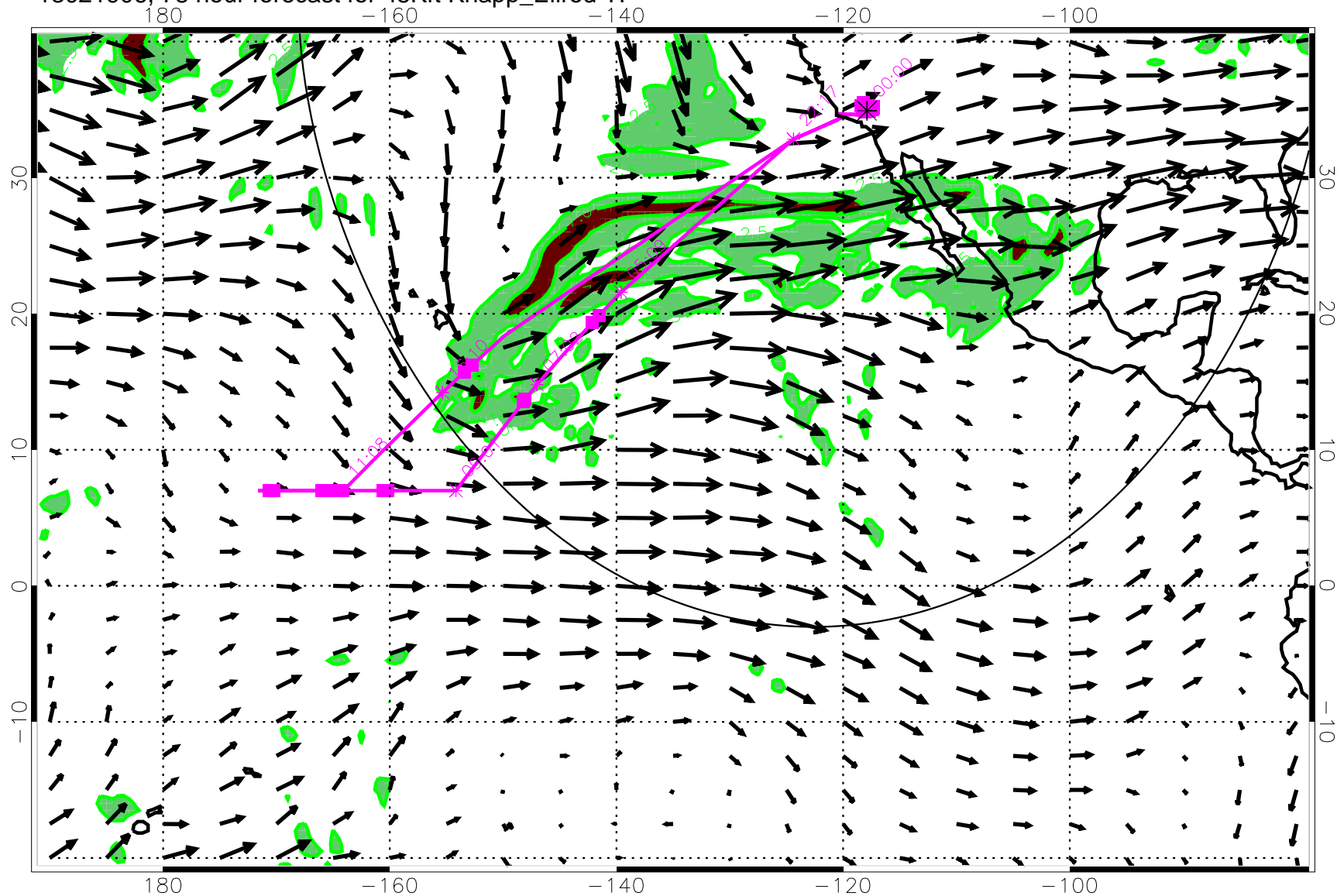
13021906, 78 hour forecast for 45Kft Knapp_Ellrod TI
