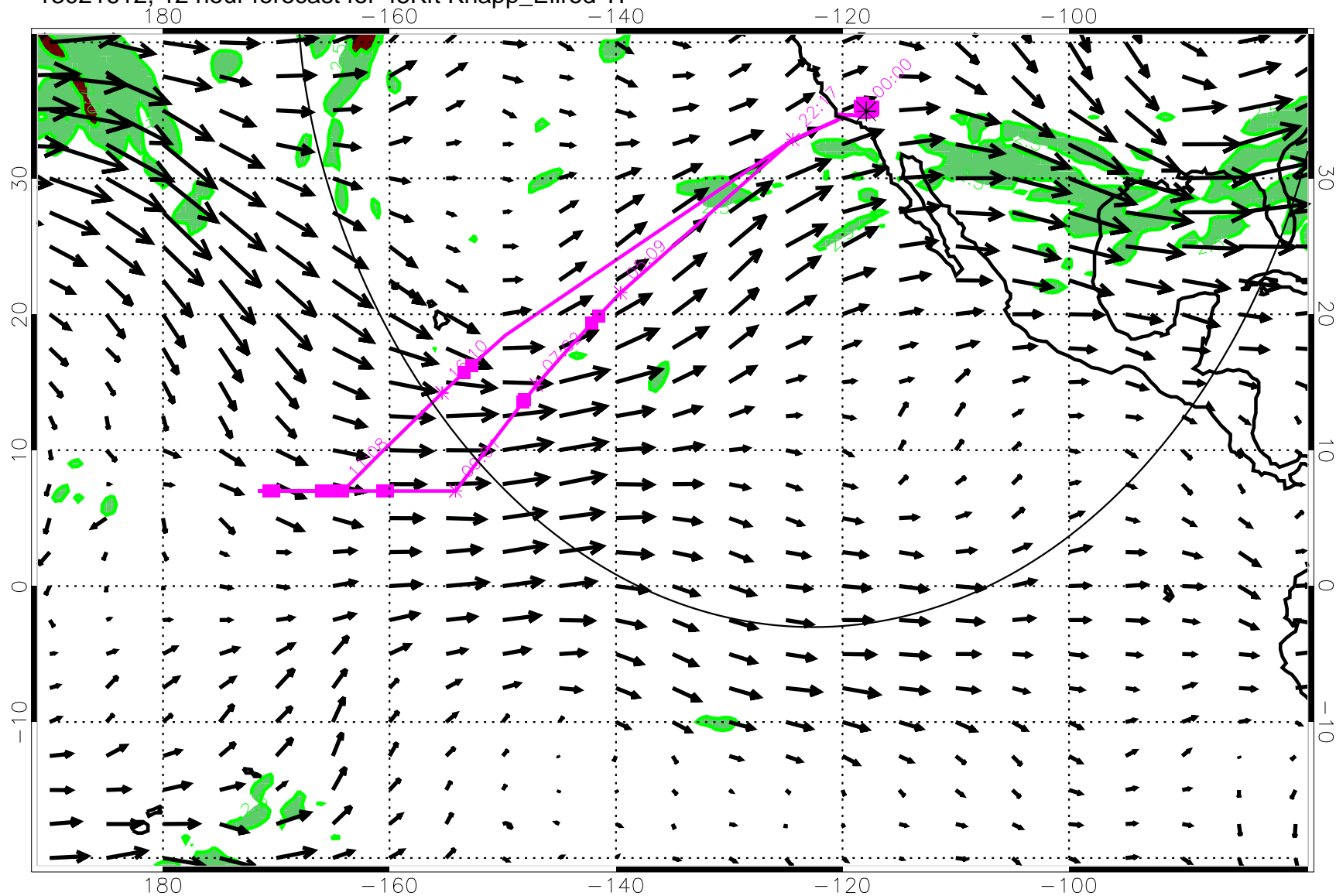
13021612, 12 hour forecast for 45Kft Knapp_Ellrod TI
