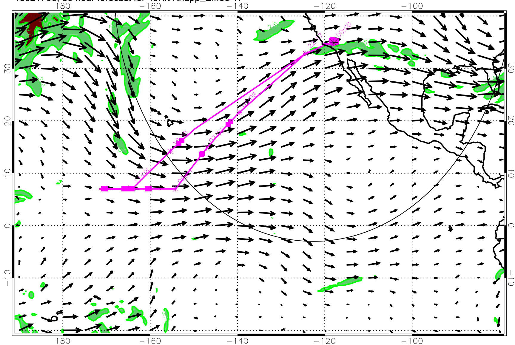
13021706, 30 hour forecast for 45Kft Knapp_Ellrod TI
