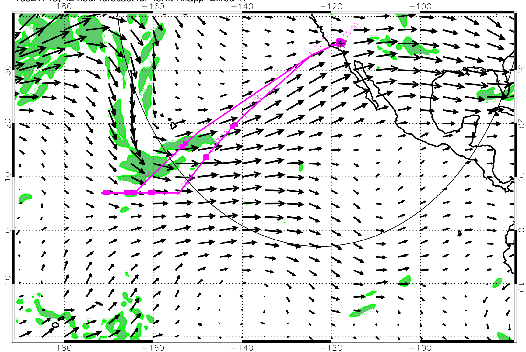
13021718, 42 hour forecast for 45Kft Knapp_Ellrod TI
