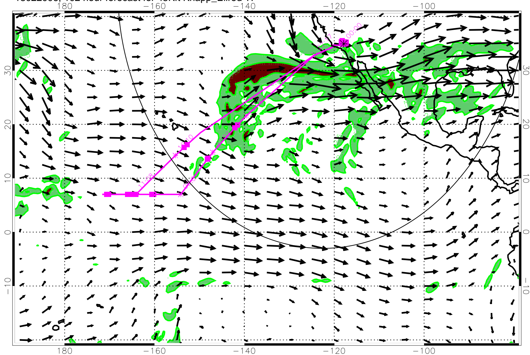
13022006, 102 hour forecast for 45Kft Knapp_Ellrod TI
