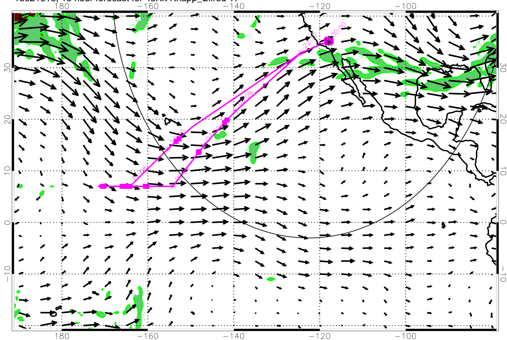
13021618, 18 hour forecast for 45Kft Knapp_Ellrod TI
