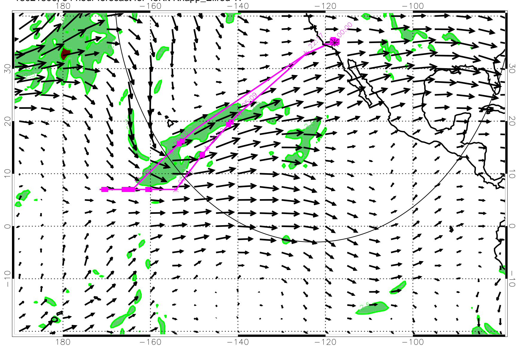
13021806, 54 hour forecast for 45Kft Knapp_Ellrod TI
