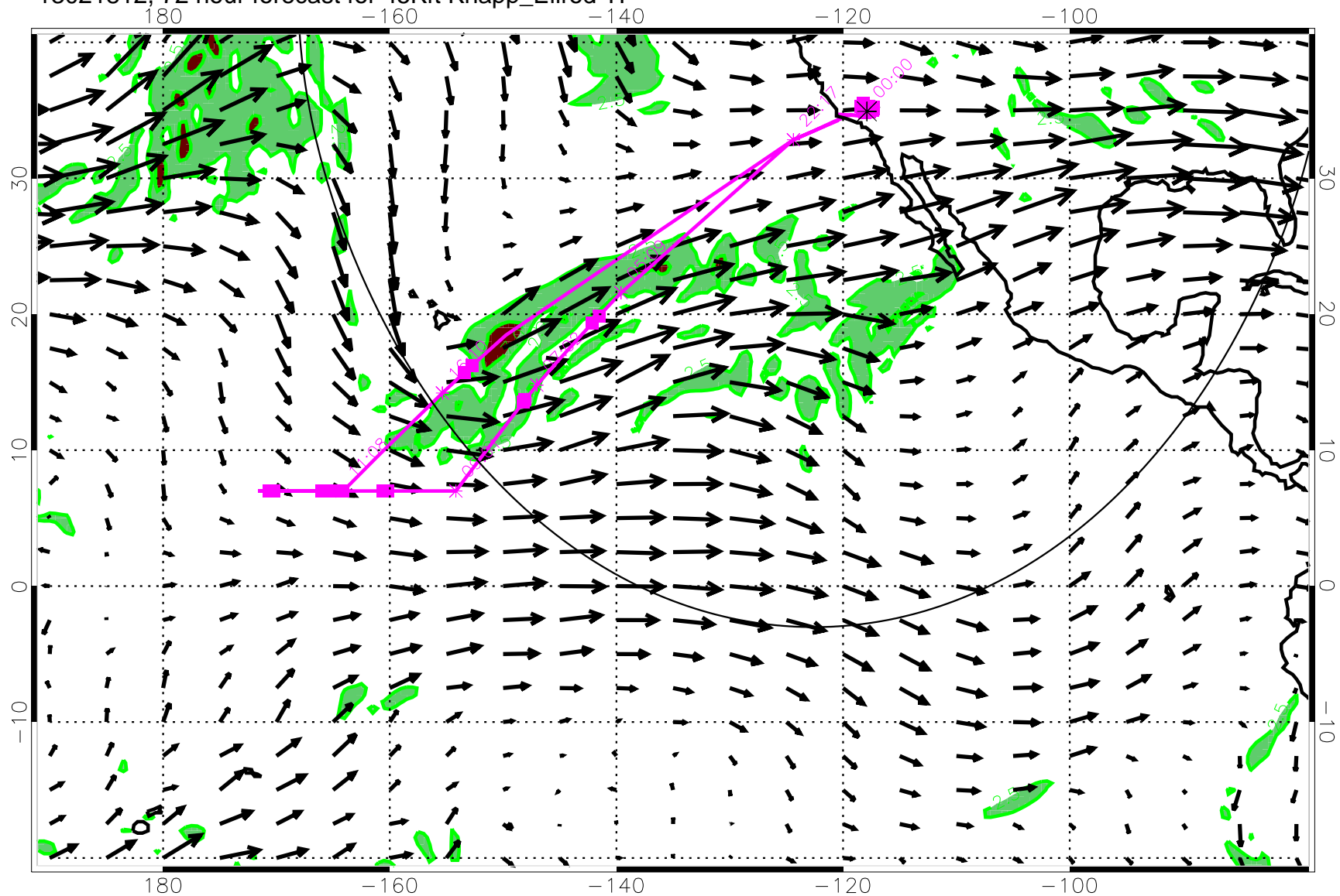
13021812, 72 hour forecast for 45Kft Knapp_Ellrod TI
