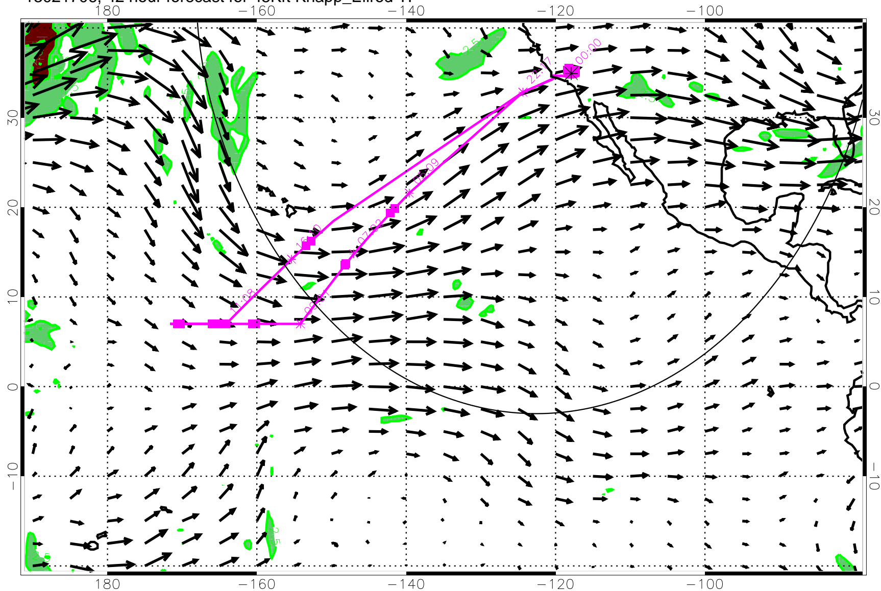
13021706, 42 hour forecast for 45Kft Knapp_Ellrod TI
