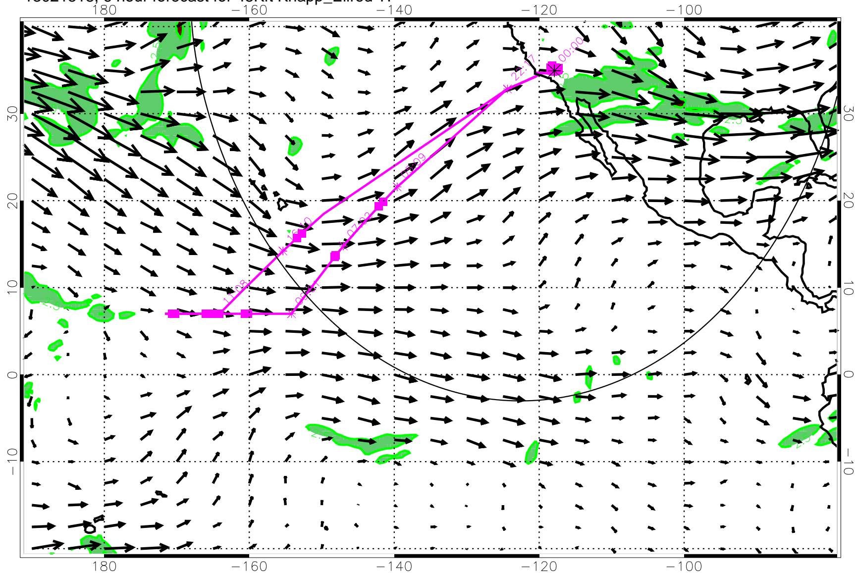
13021518, 6 hour forecast for 45Kft Knapp_Ellrod TI
