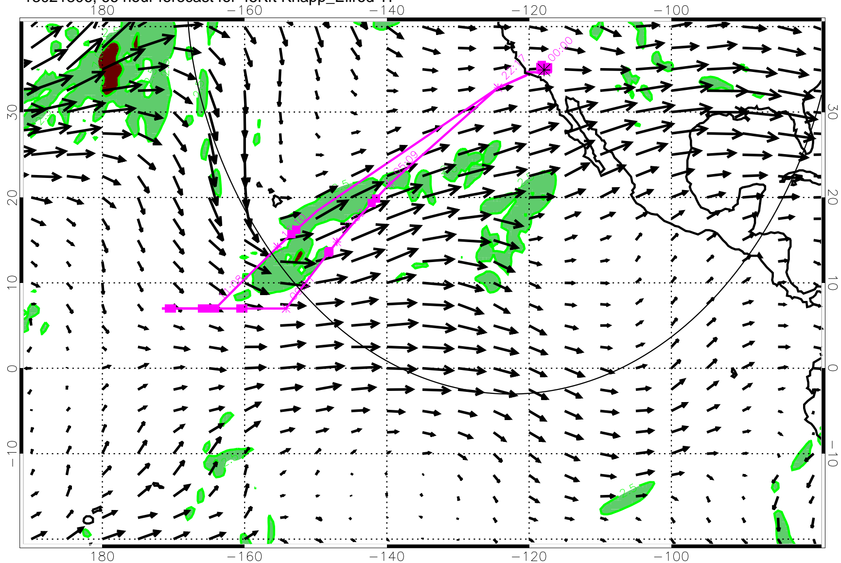
13021806, 66 hour forecast for 45Kft Knapp_Ellrod TI
