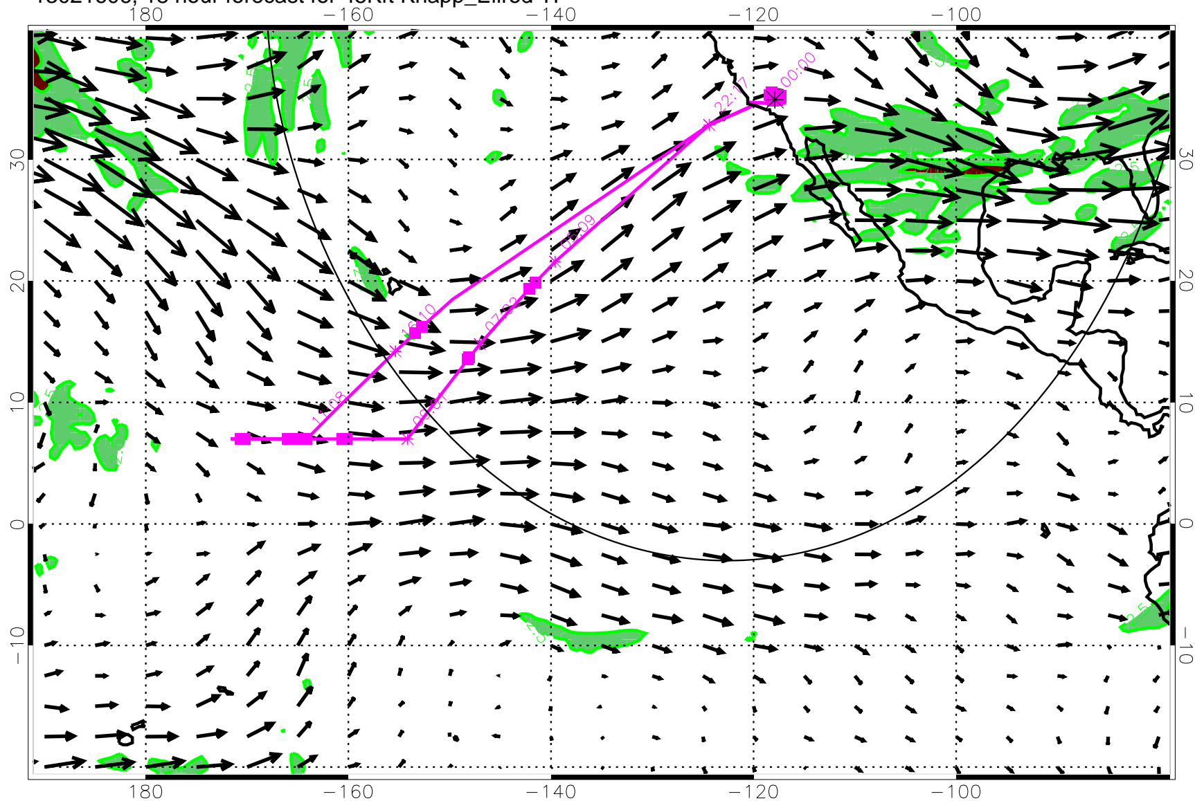
13021606, 18 hour forecast for 45Kft Knapp_Ellrod TI
