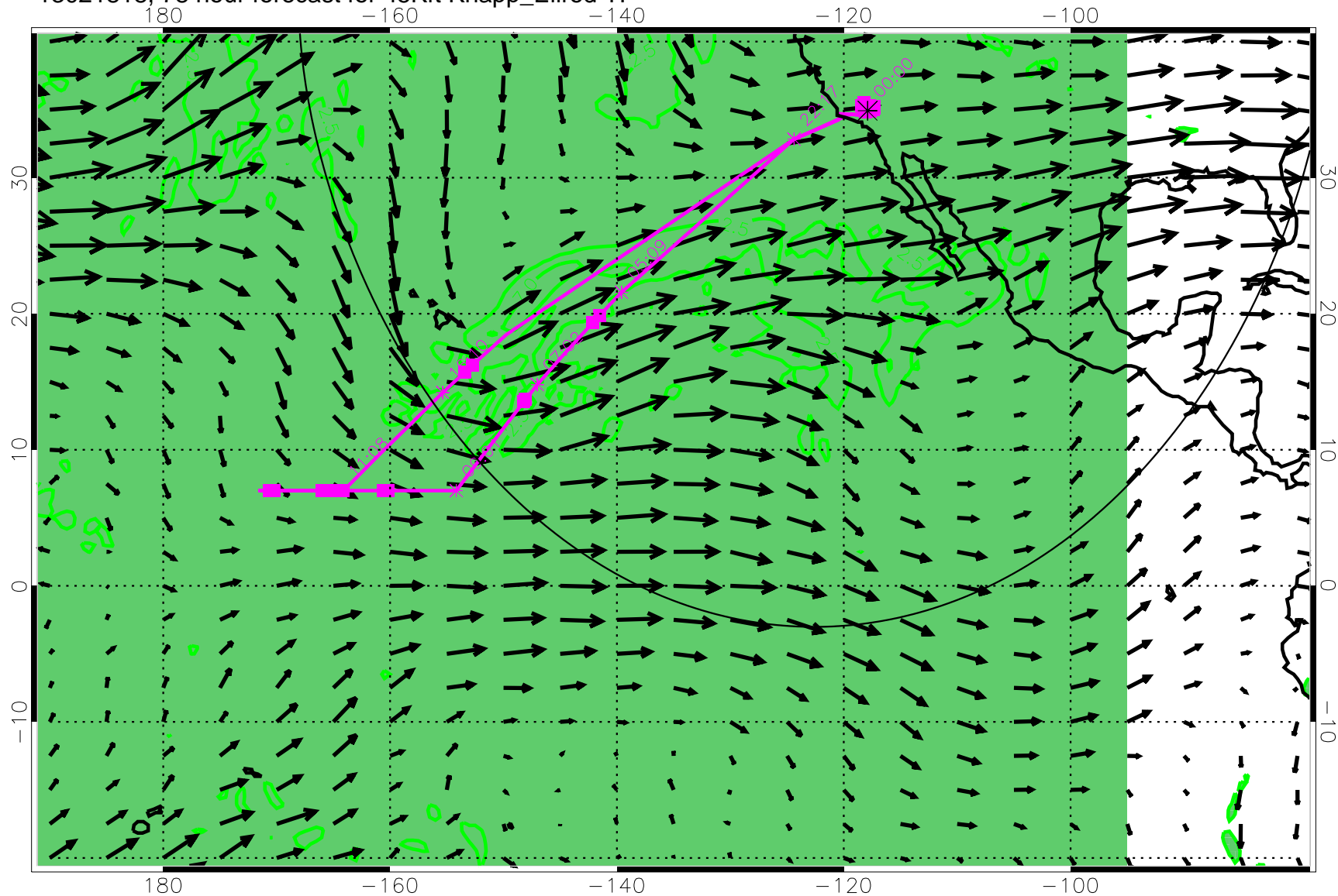
13021818, 78 hour forecast for 45Kft Knapp_Ellrod TI
