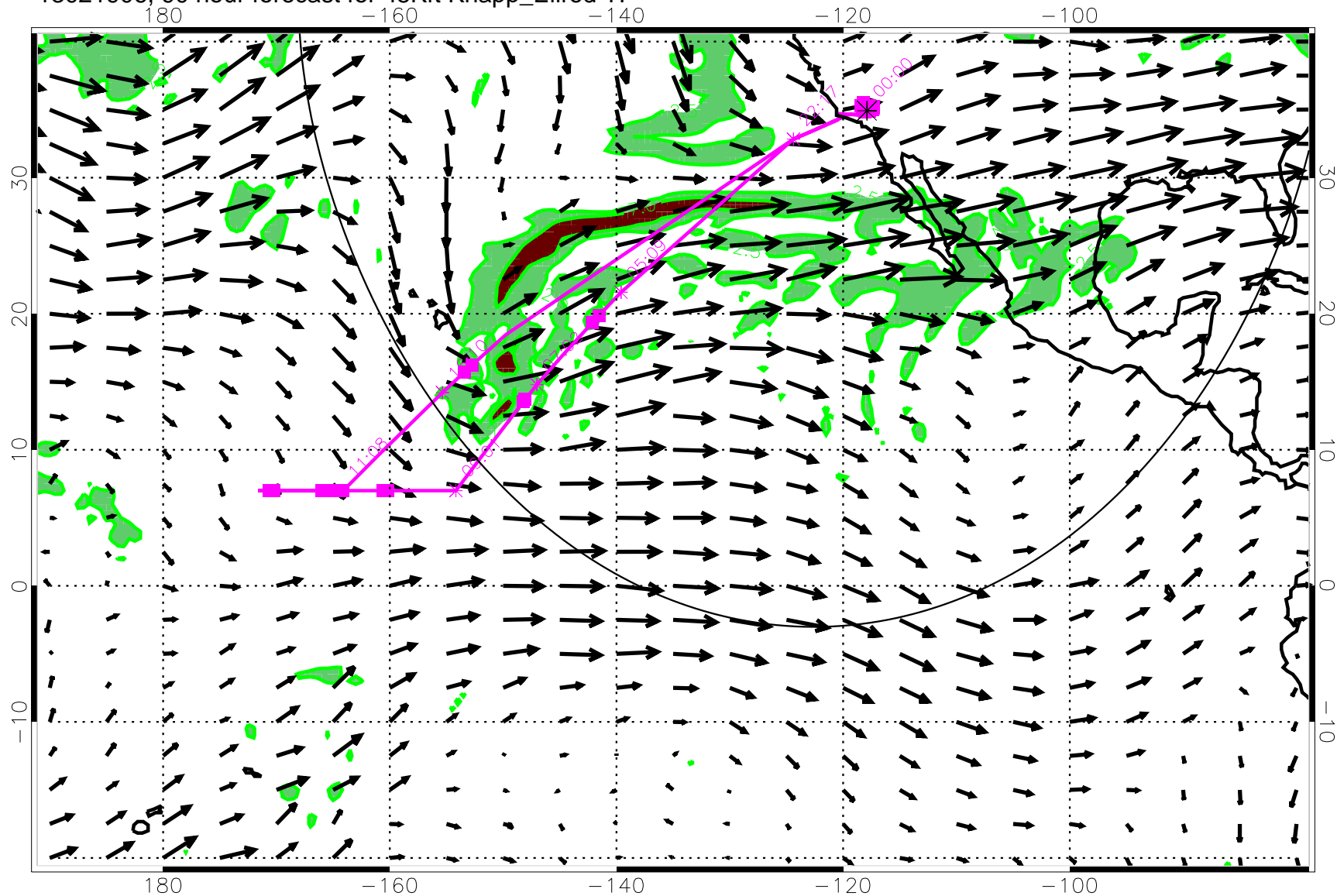
13021906, 90 hour forecast for 45Kft Knapp_Ellrod TI
