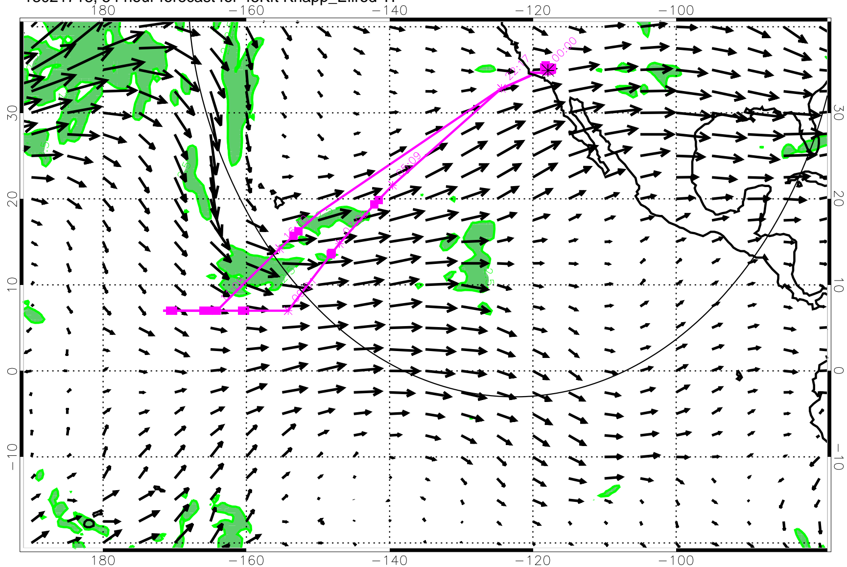
13021718, 54 hour forecast for 45Kft Knapp_Ellrod TI
