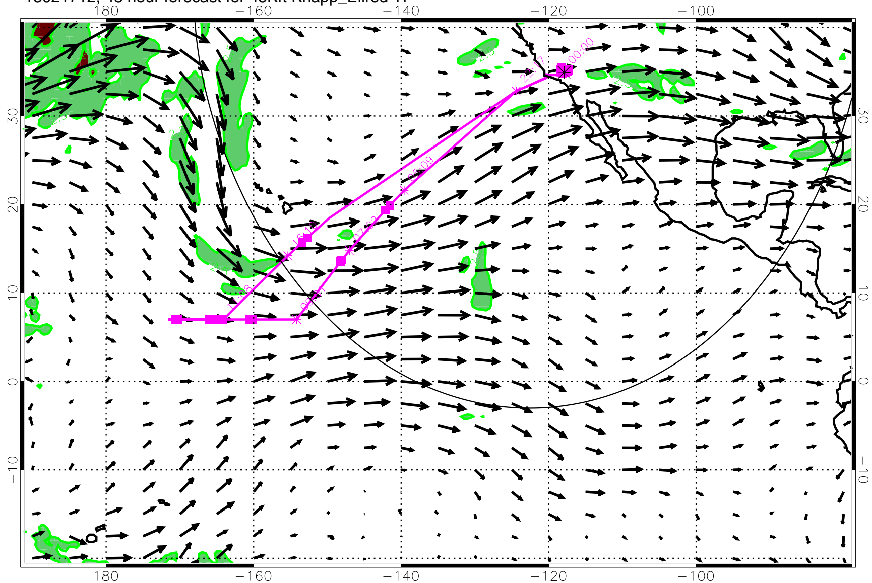
13021712, 48 hour forecast for 45Kft Knapp_Ellrod TI
