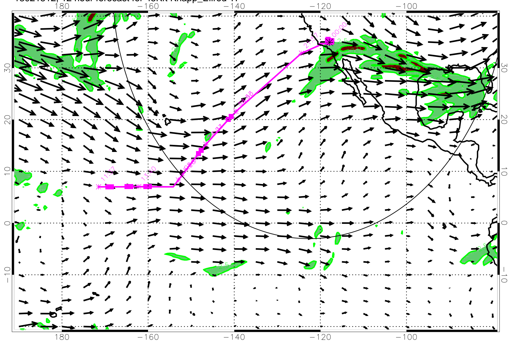
13021512, 12 hour forecast for 45Kft Knapp_Ellrod TI
