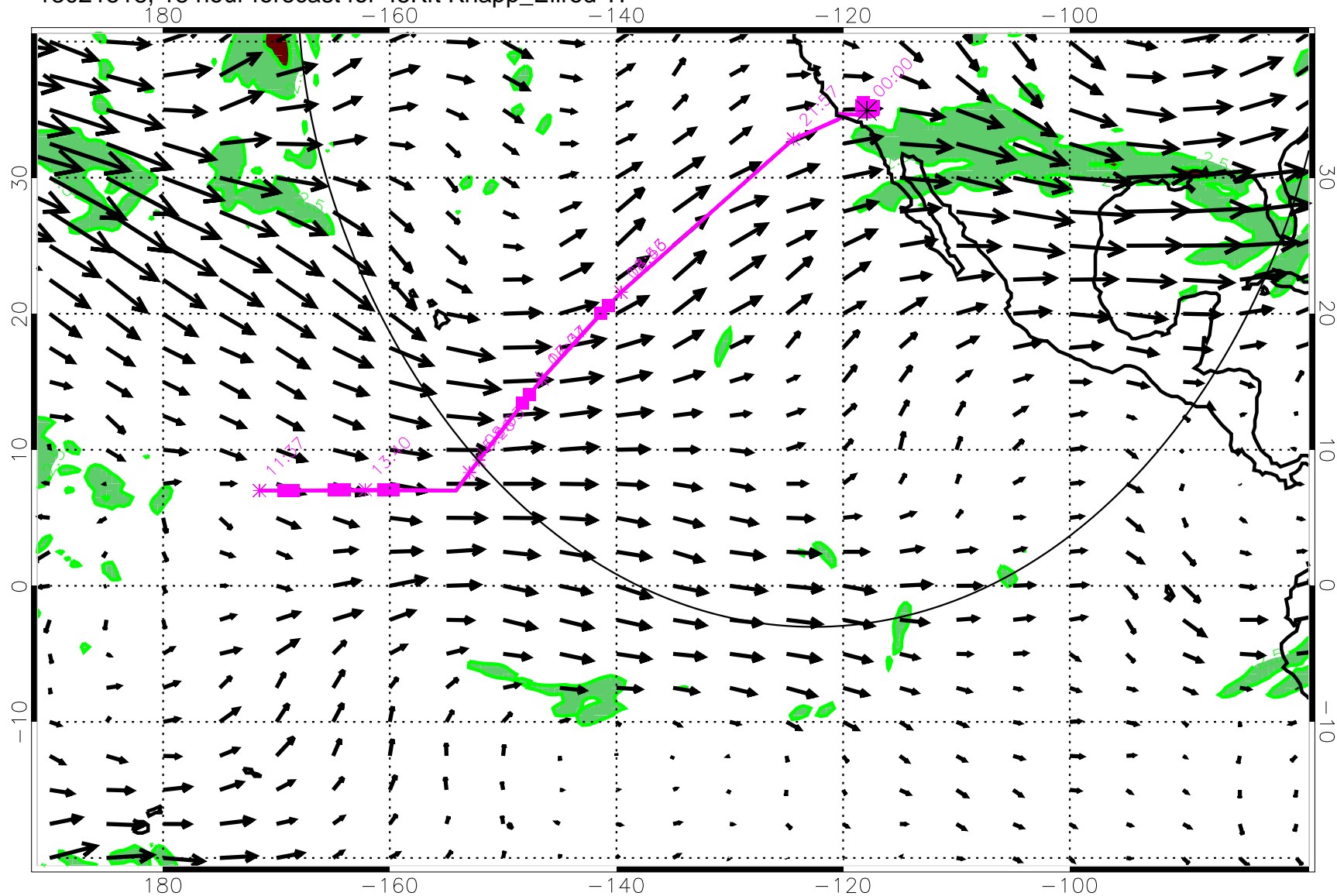
13021518, 18 hour forecast for 45Kft Knapp_Ellrod TI
