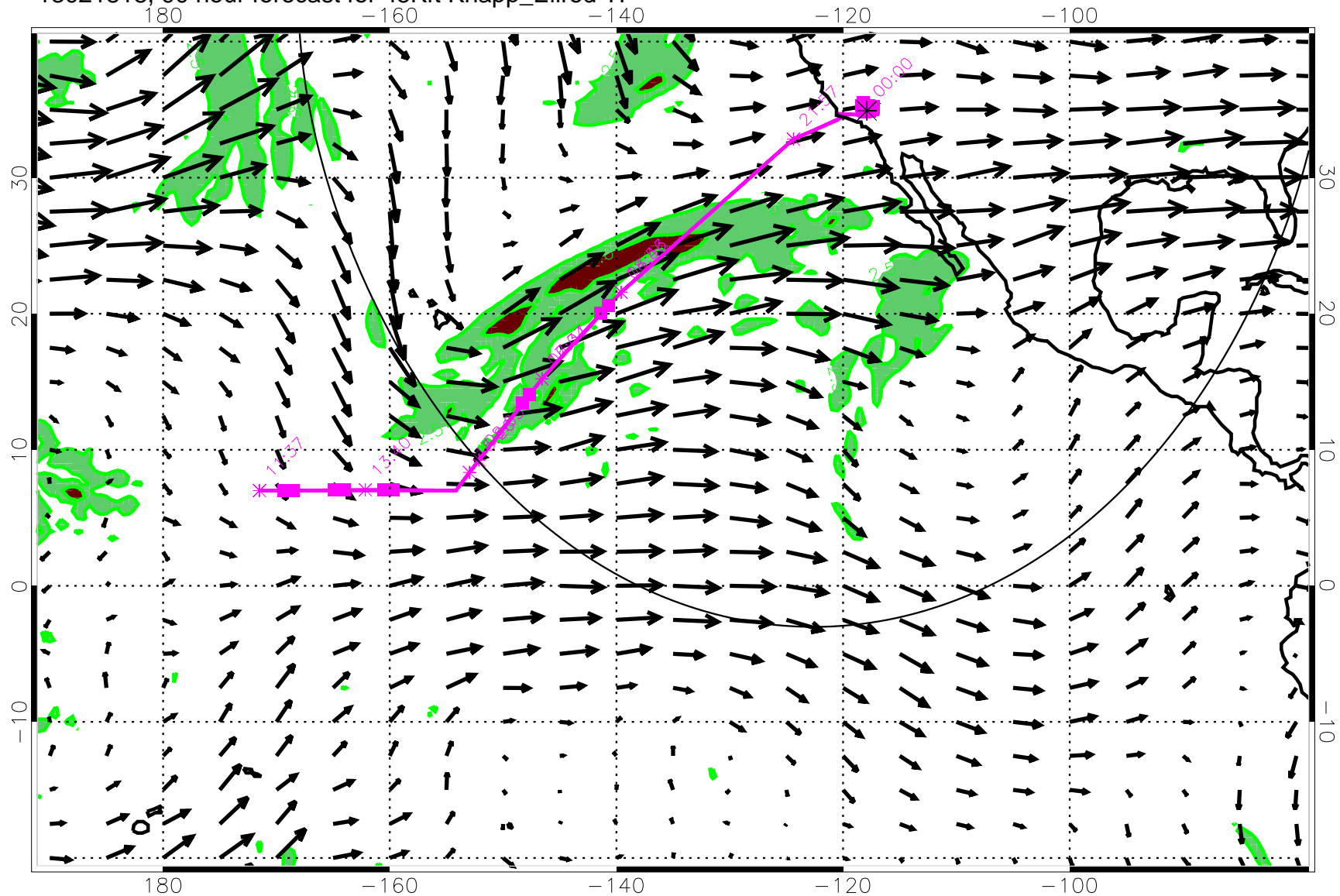
13021818, 90 hour forecast for 45Kft Knapp_Ellrod TI
