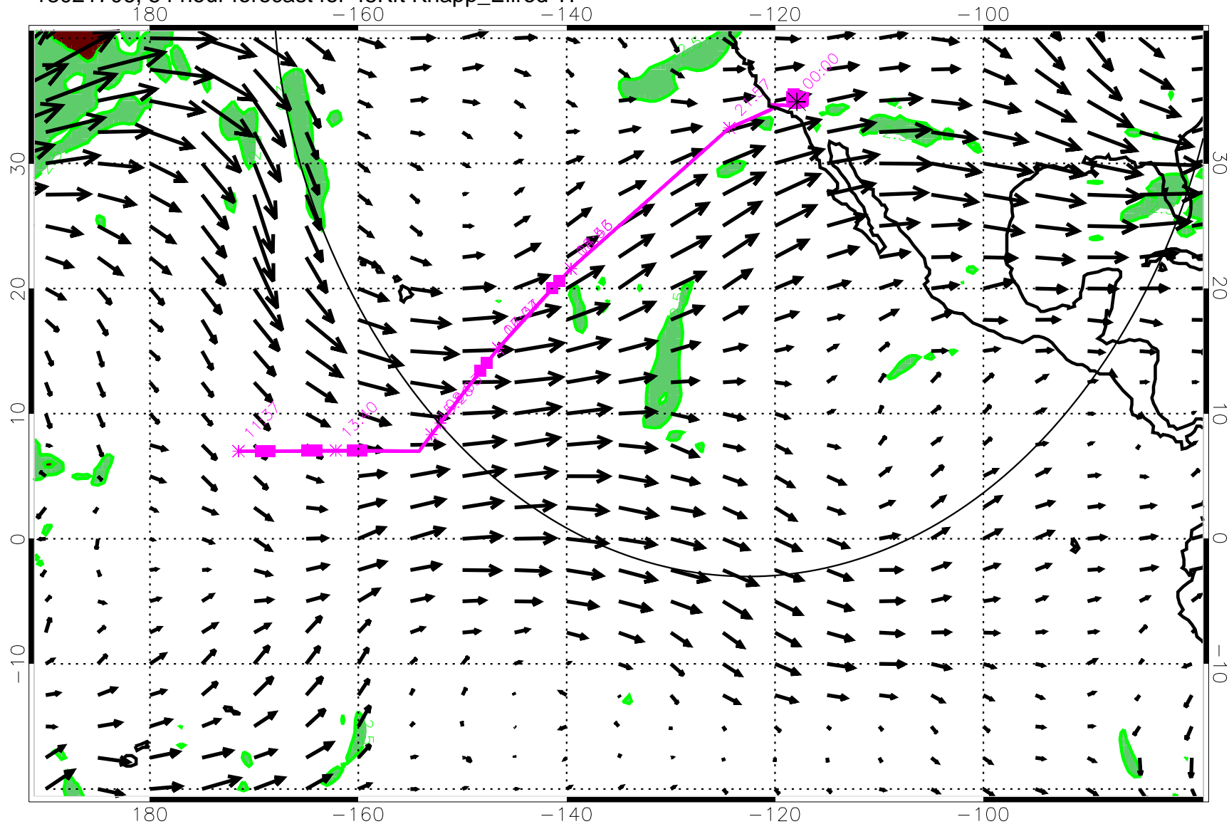
13021706, 54 hour forecast for 45Kft Knapp_Ellrod TI
