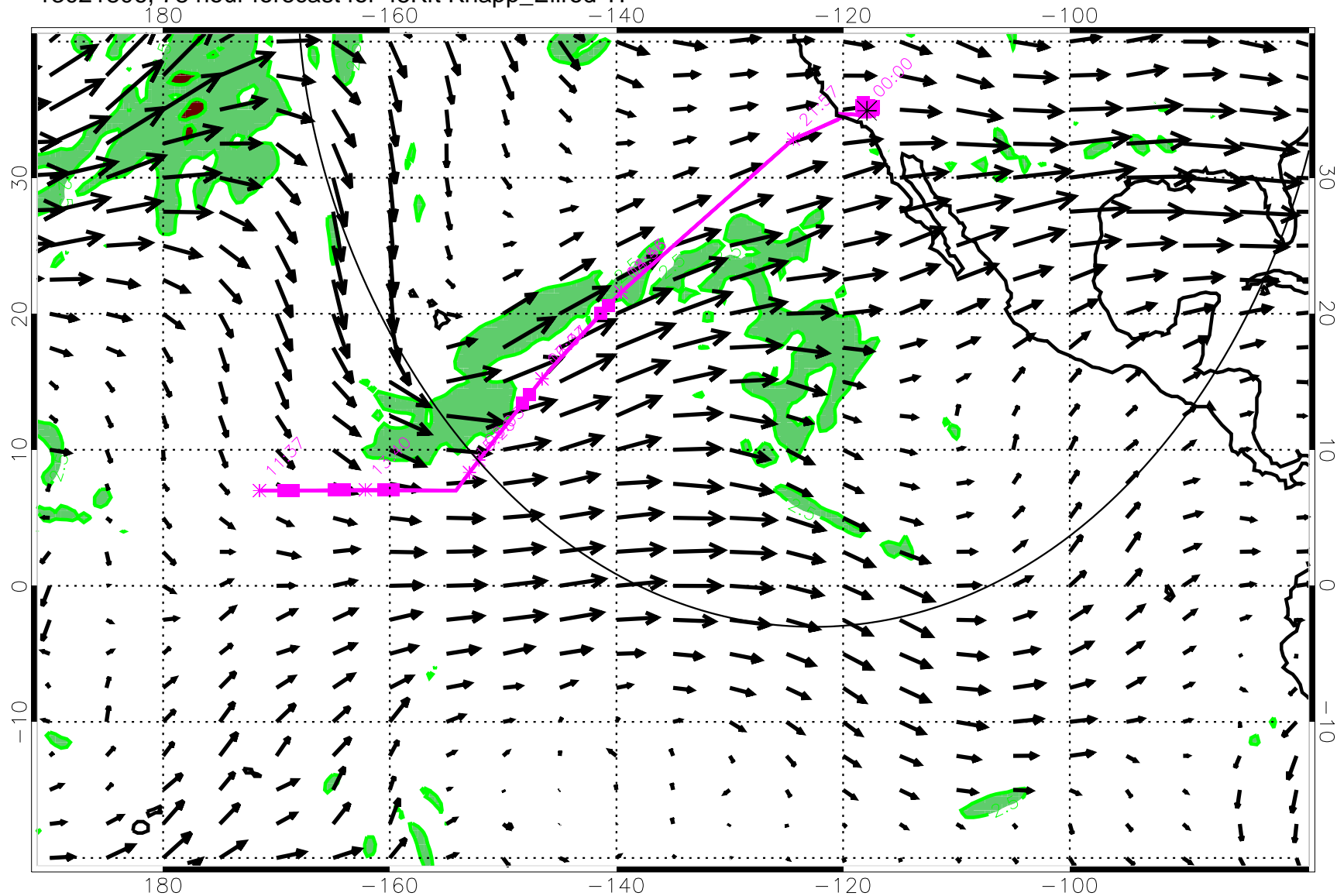
13021806, 78 hour forecast for 45Kft Knapp_Ellrod TI
