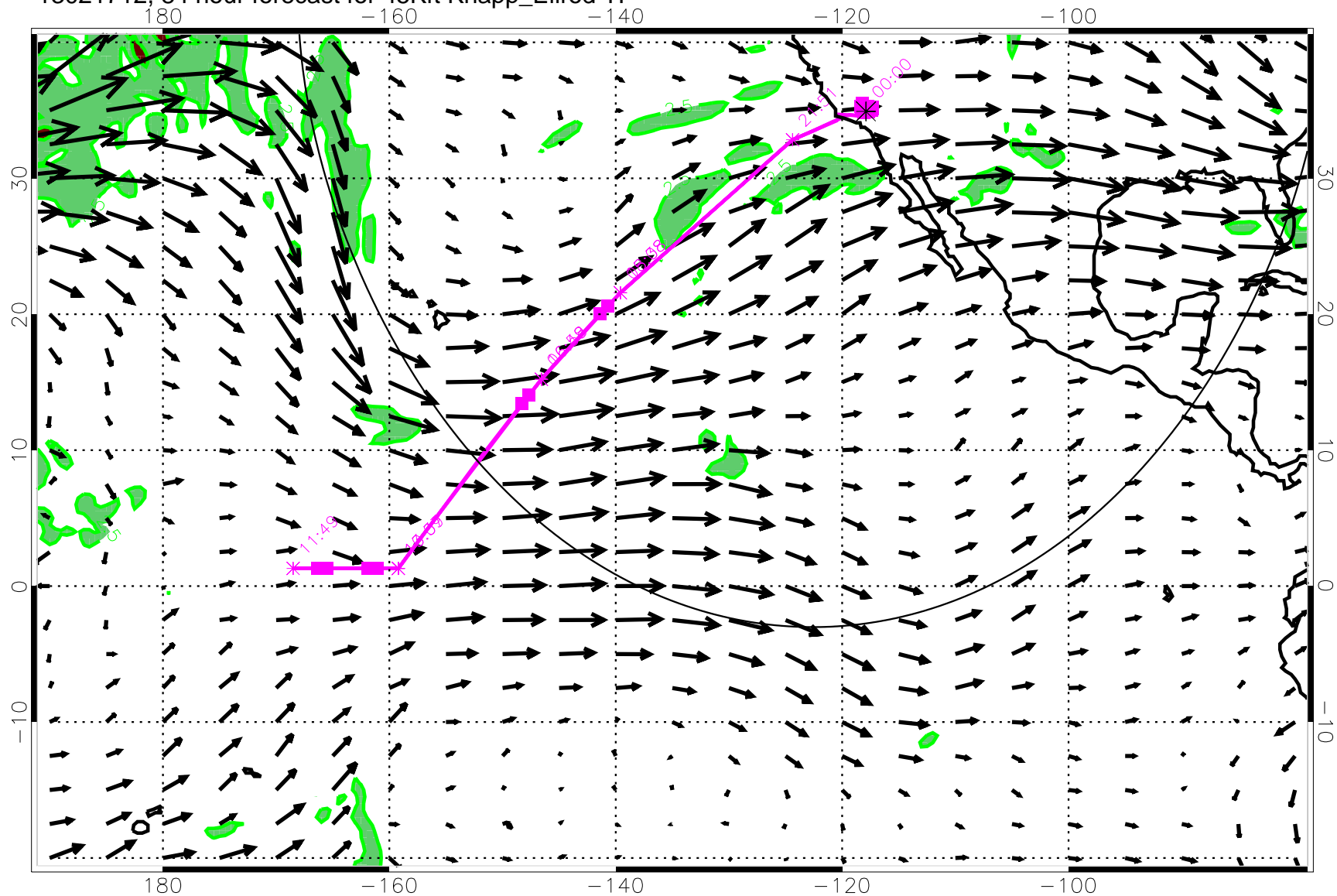
13021712, 84 hour forecast for 45Kft Knapp_Ellrod TI
