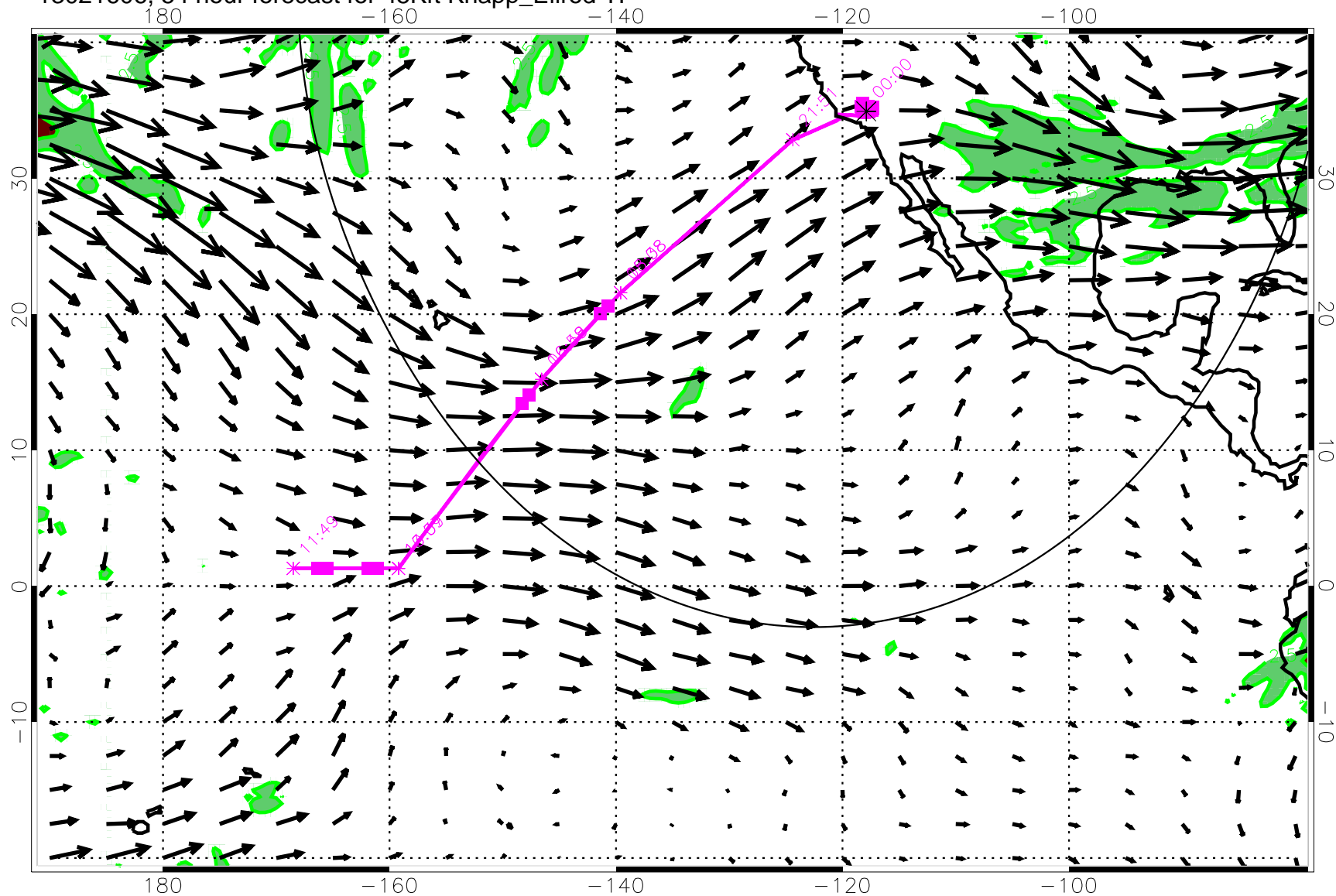
13021606, 54 hour forecast for 45Kft Knapp_Ellrod TI
