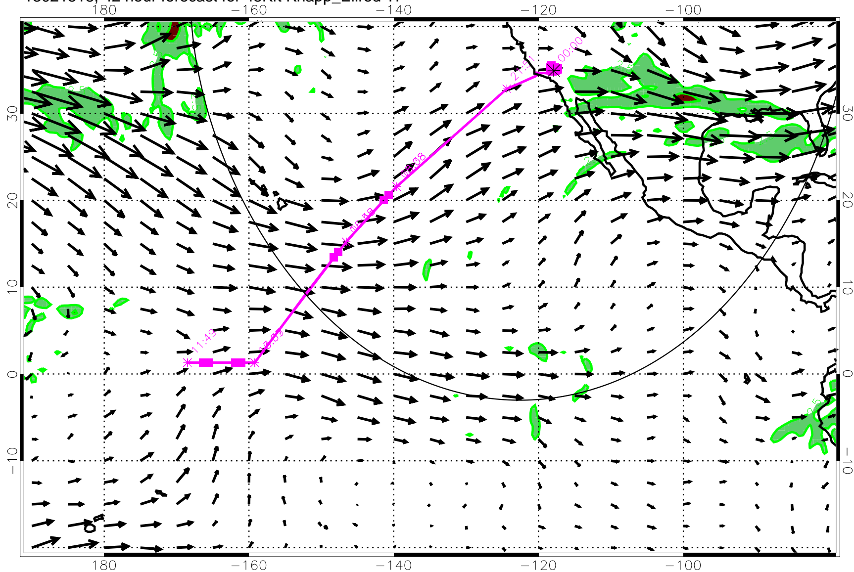
13021518, 42 hour forecast for 45Kft Knapp_Ellrod TI
