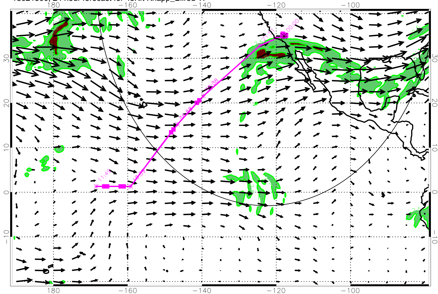
13021500, 24 hour forecast for 45Kft Knapp_Ellrod TI
