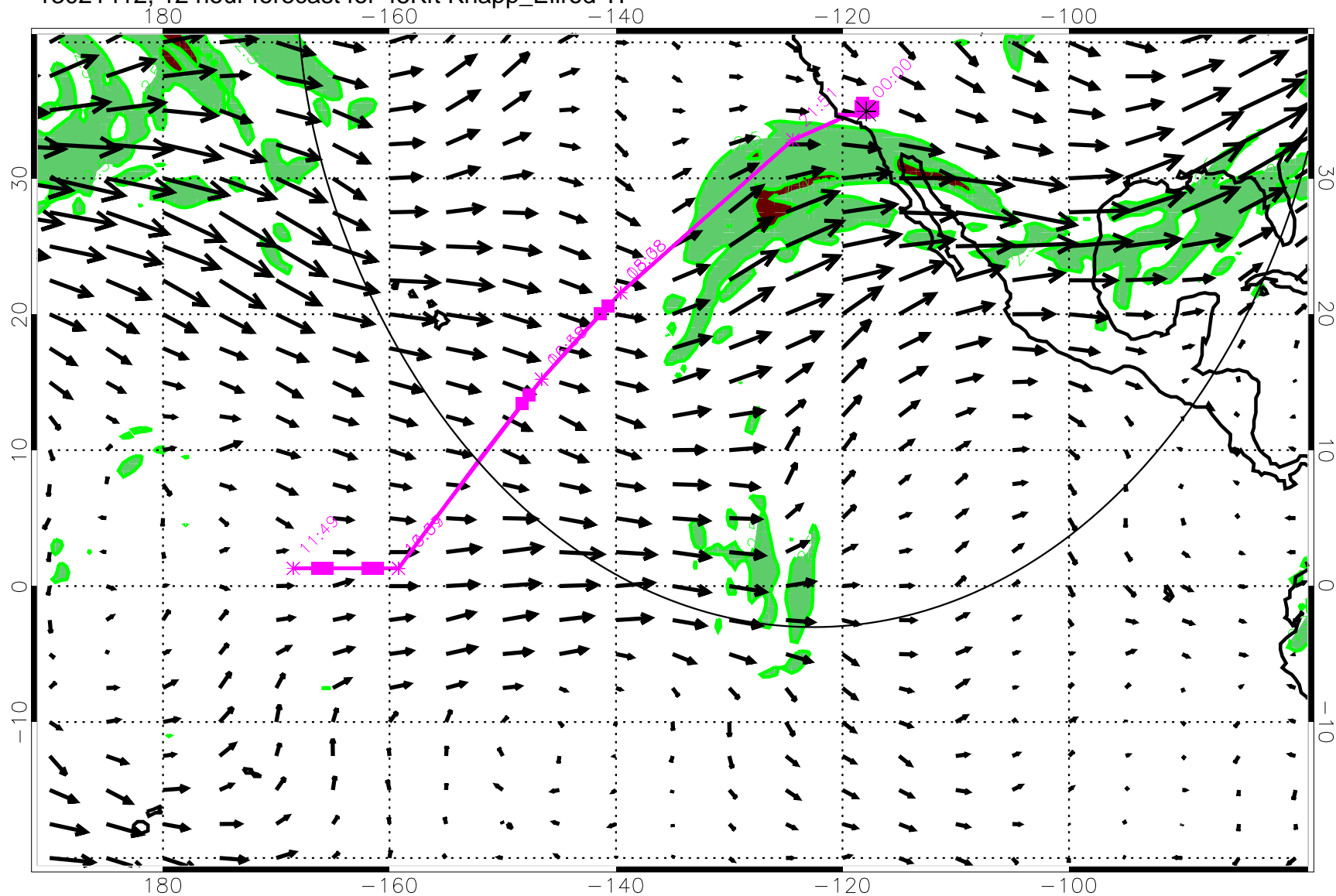
13021412, 12 hour forecast for 45Kft Knapp_Ellrod TI
