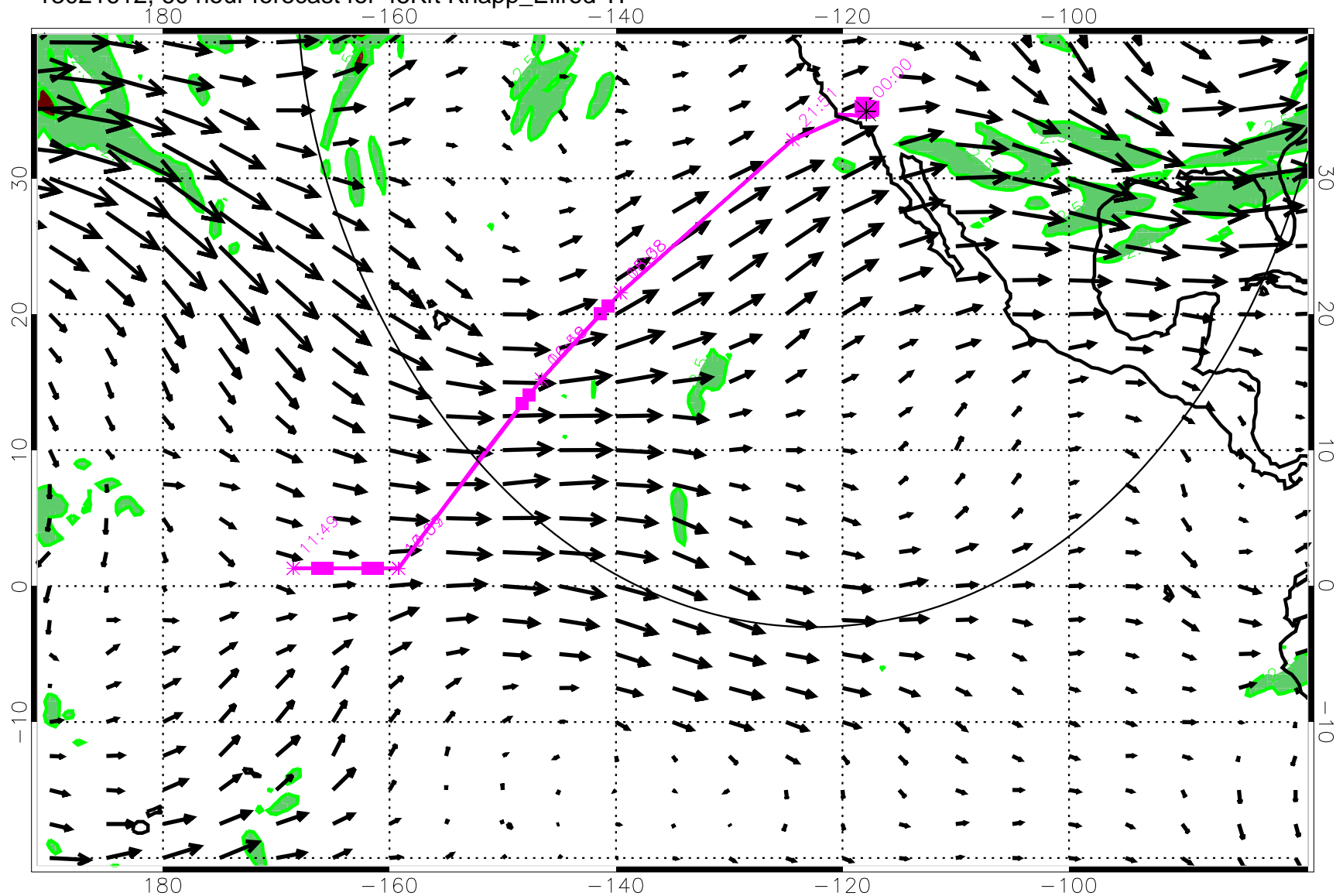
13021612, 60 hour forecast for 45Kft Knapp_Ellrod TI
