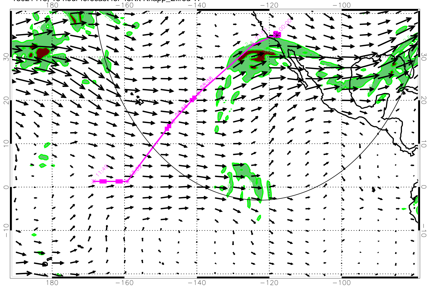
13021418, 18 hour forecast for 45Kft Knapp_Ellrod TI
