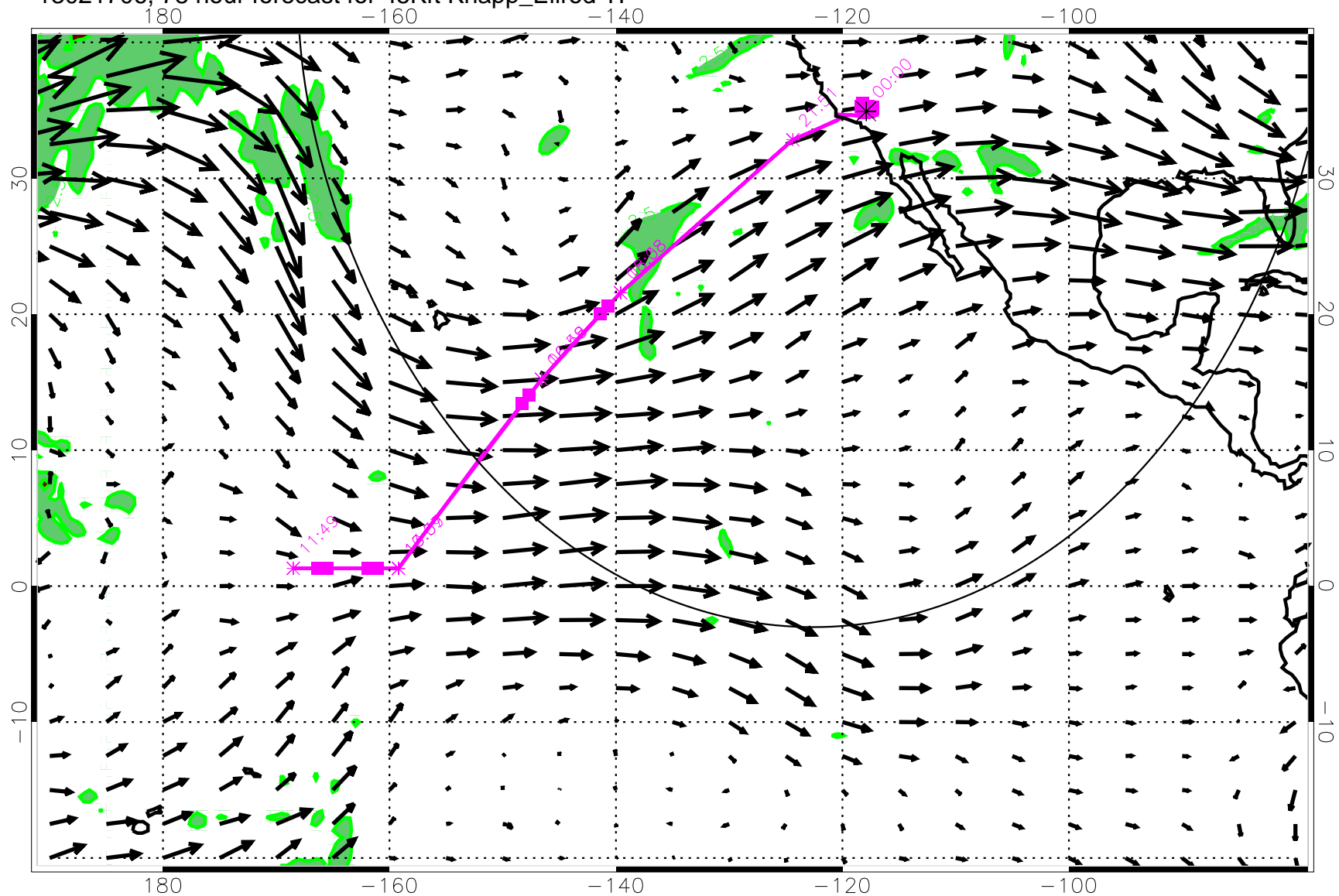
13021706, 78 hour forecast for 45Kft Knapp_Ellrod TI
