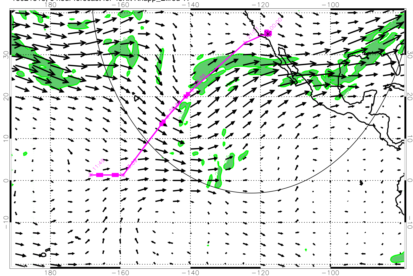
13021318, 6 hour forecast for 45Kft Knapp_Ellrod TI
