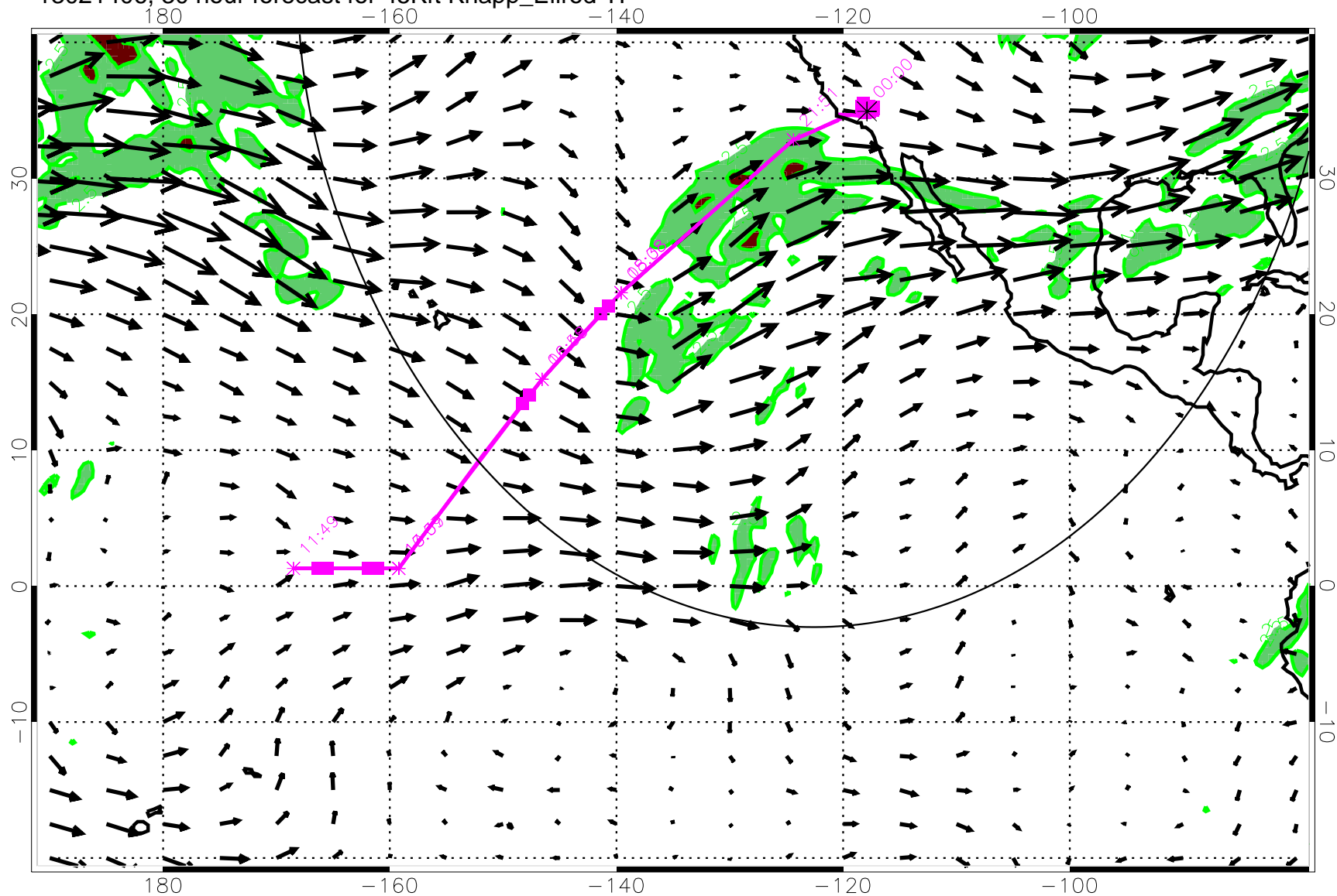
13021406, 30 hour forecast for 45Kft Knapp_Ellrod TI
