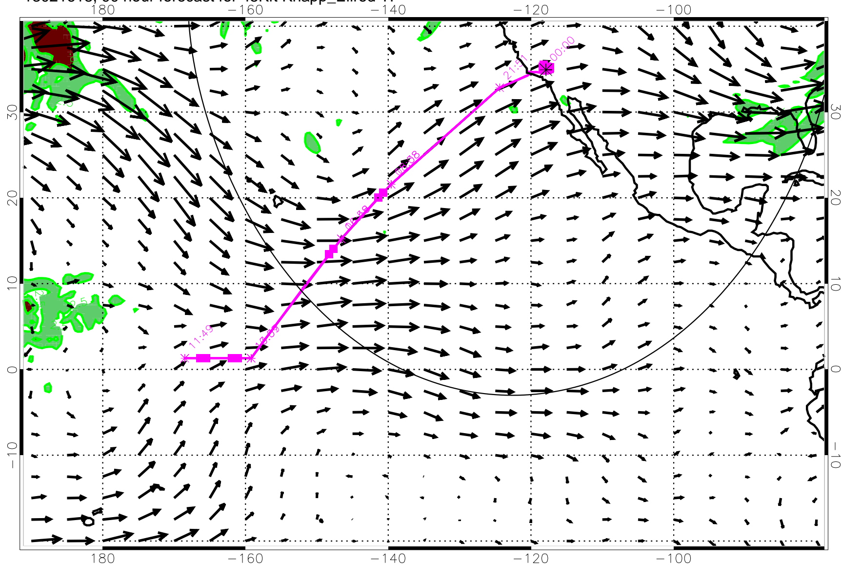
13021618, 90 hour forecast for 45Kft Knapp_Ellrod TI
