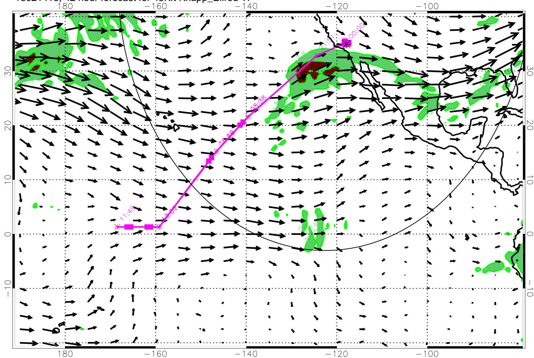
13021418, 42 hour forecast for 45Kft Knapp_Ellrod TI
