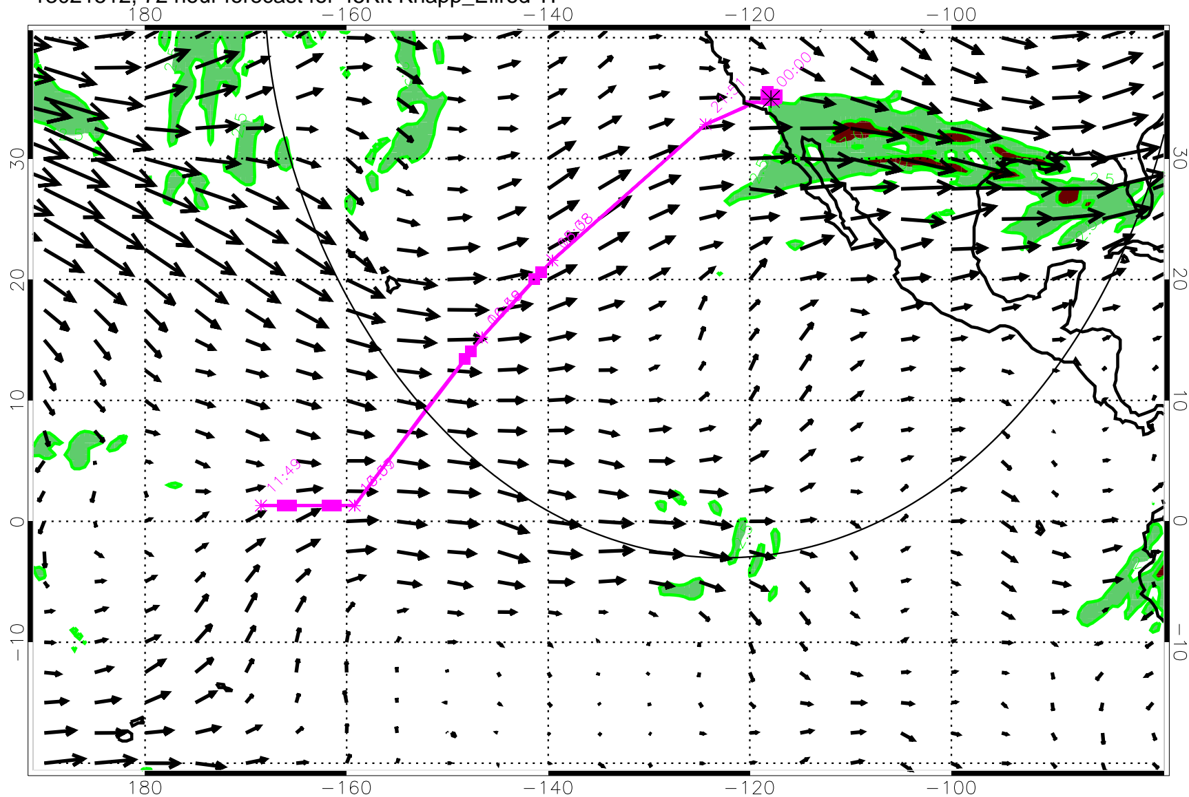
13021512, 72 hour forecast for 45Kft Knapp_Ellrod TI
