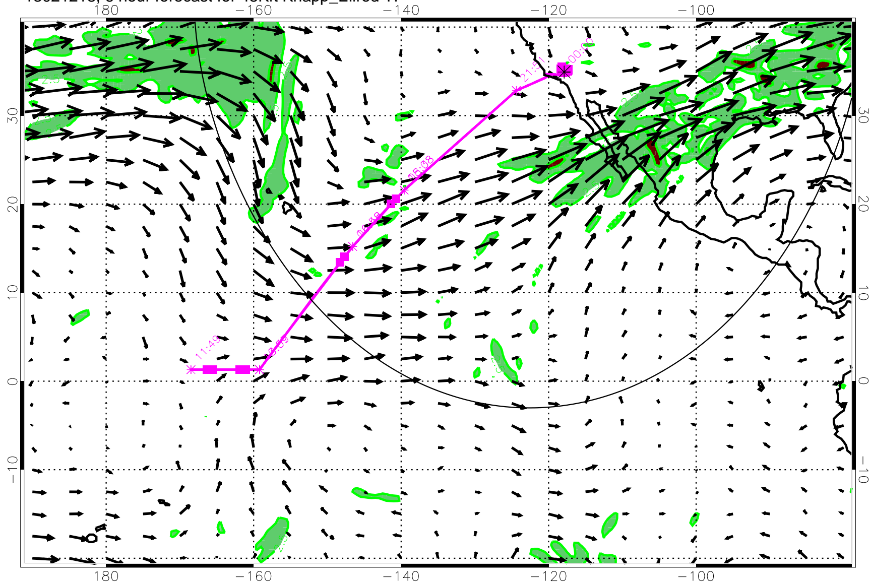
13021218, 6 hour forecast for 45Kft Knapp_Ellrod TI
