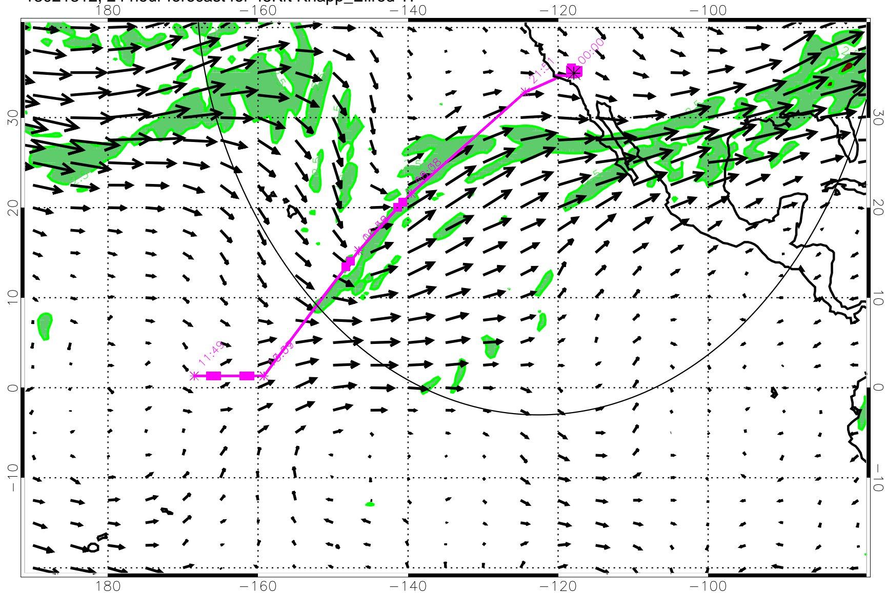
13021312, 24 hour forecast for 45Kft Knapp_Ellrod TI
