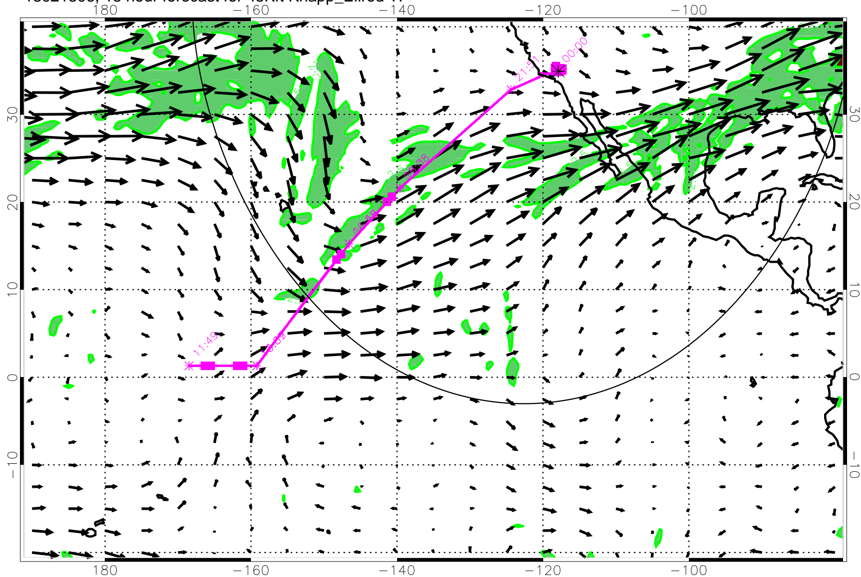
13021306, 18 hour forecast for 45Kft Knapp_Ellrod TI
