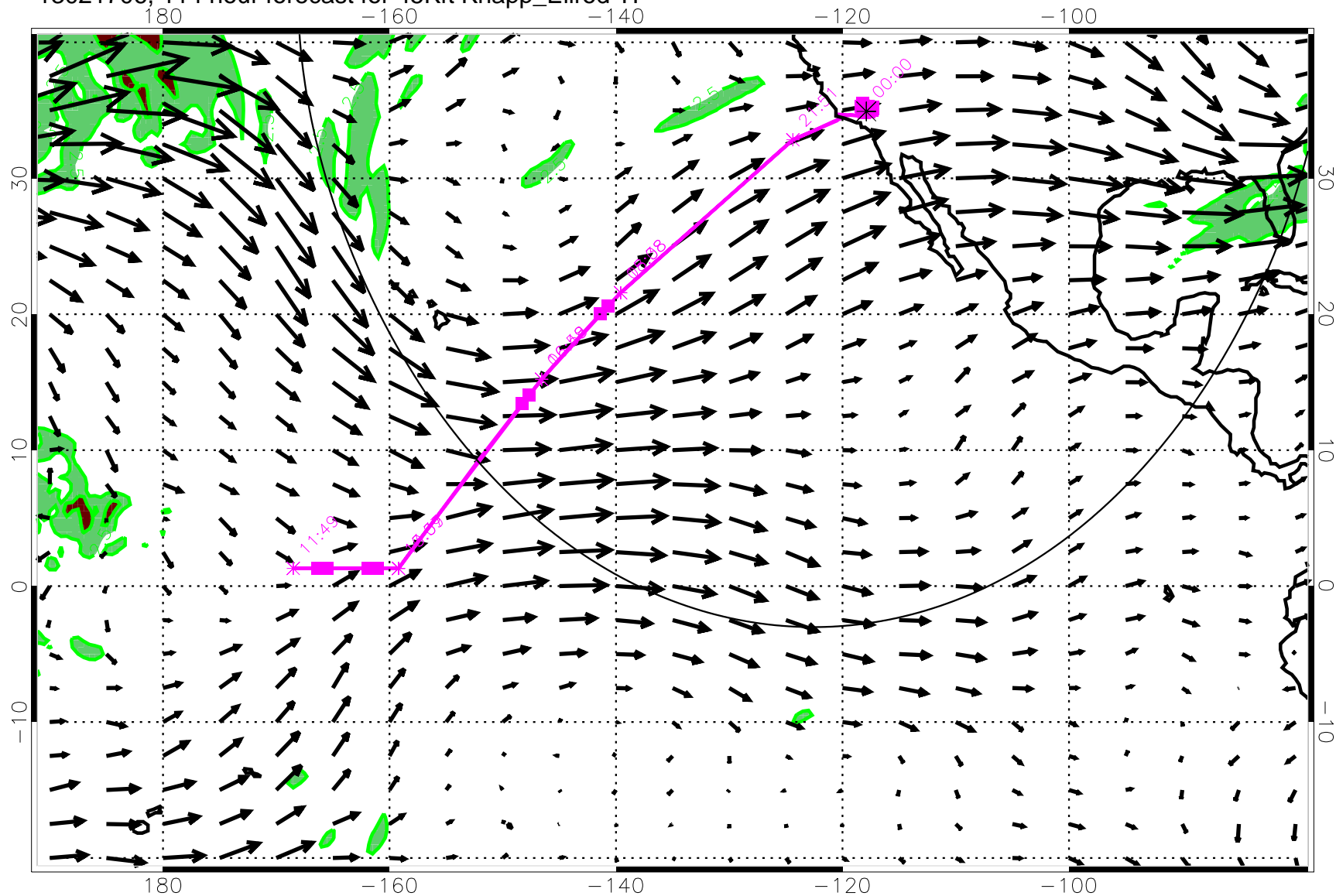
13021706, 114 hour forecast for 45Kft Knapp_Ellrod T1
