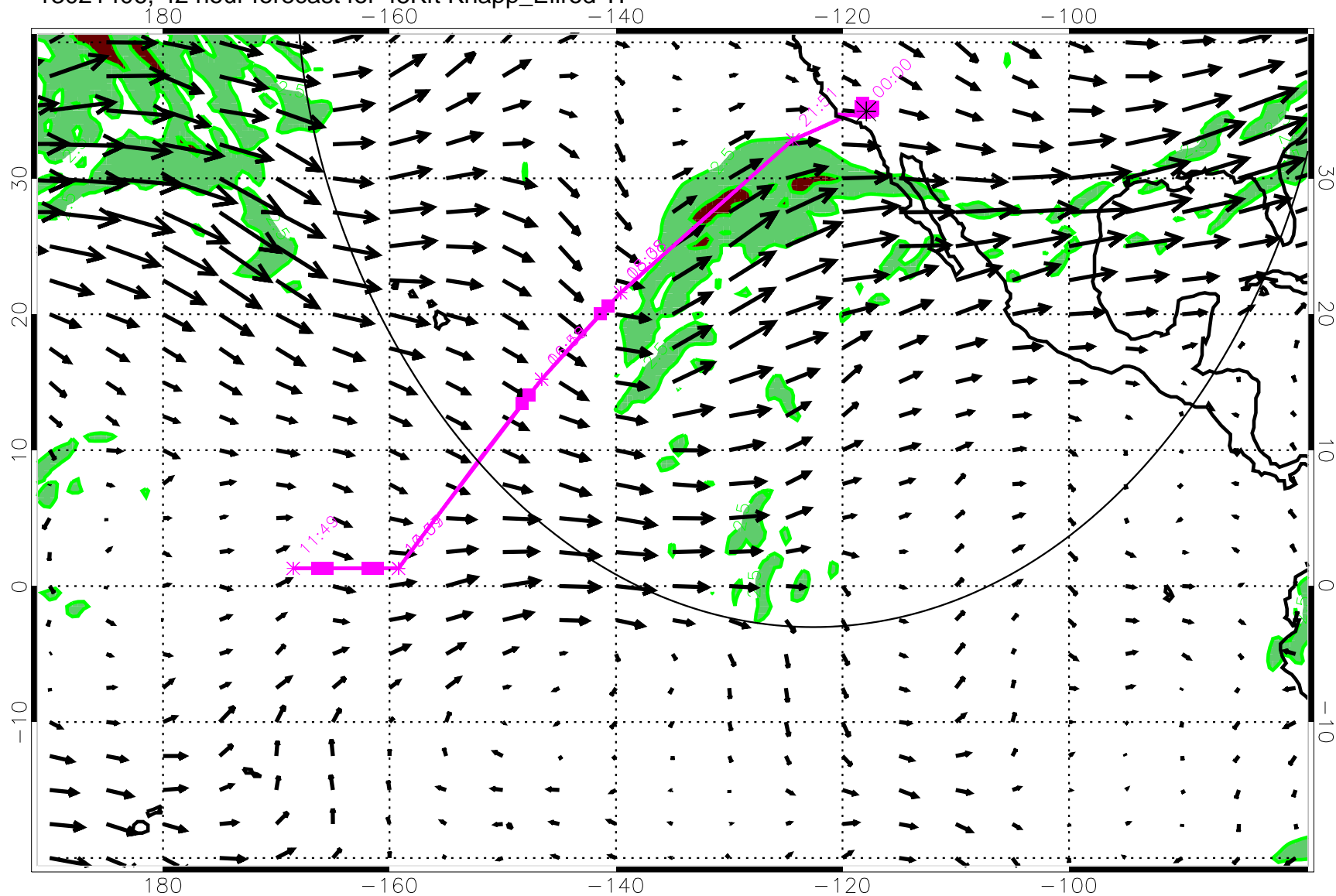
13021406, 42 hour forecast for 45Kft Knapp_Ellrod TI
