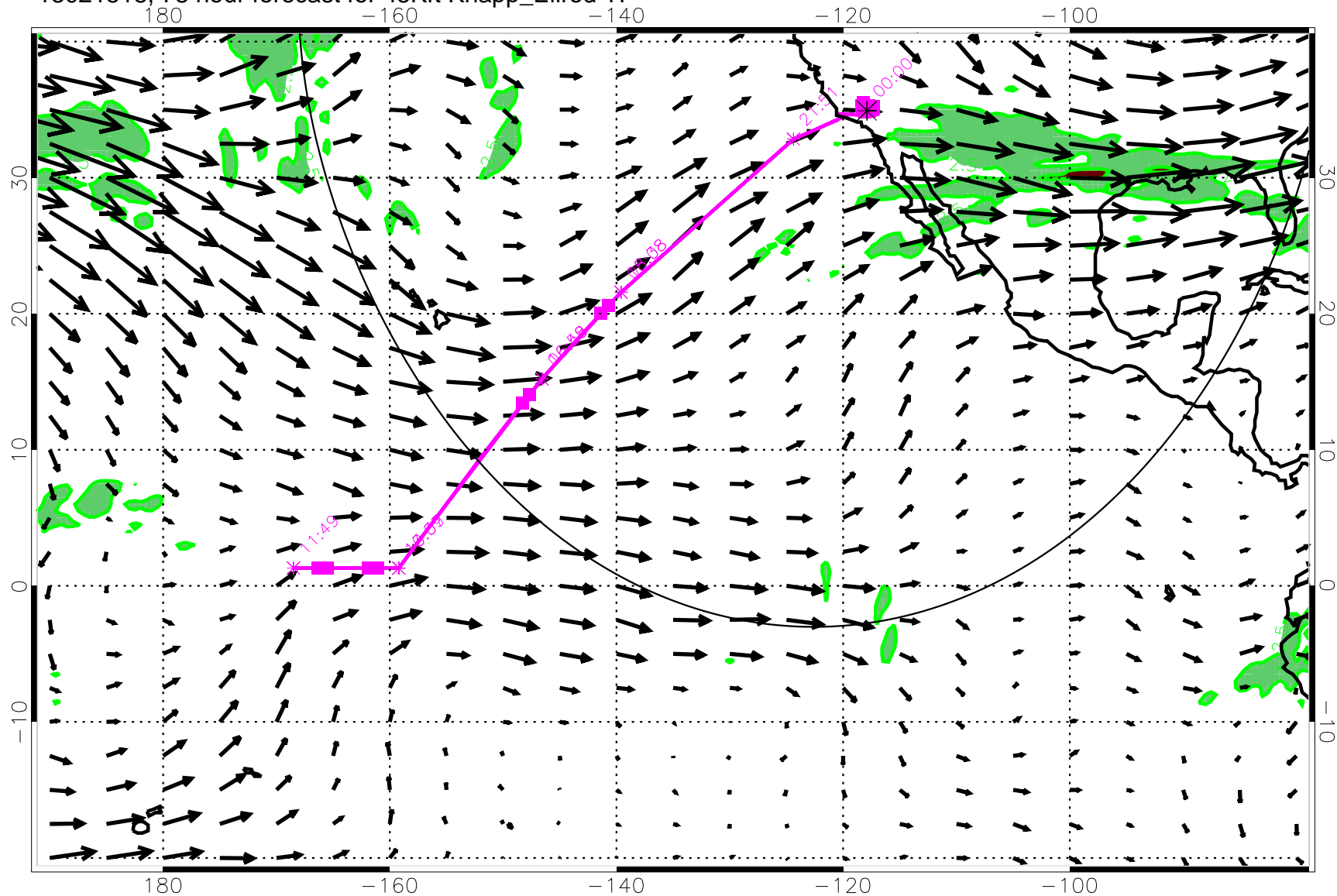
13021518, 78 hour forecast for 45Kft Knapp_Ellrod TI
