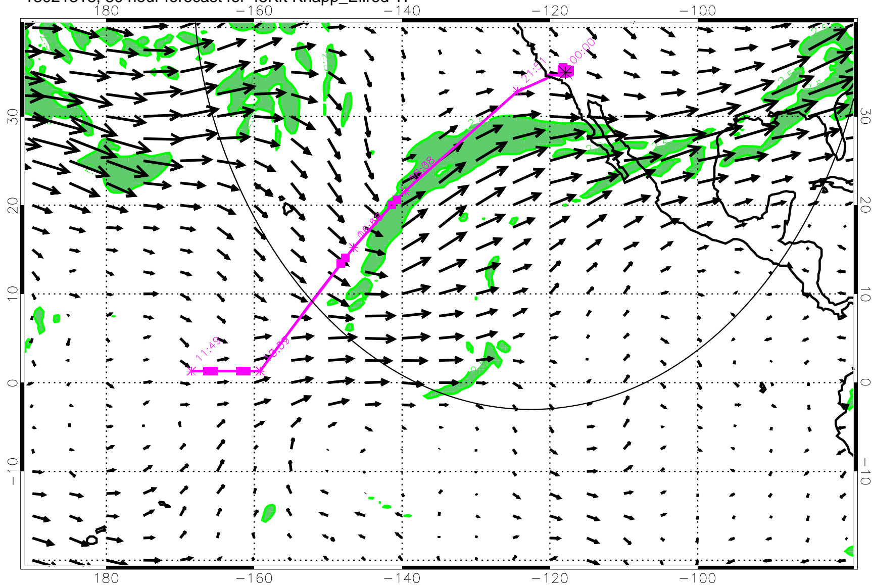
13021318, 30 hour forecast for 45Kft Knapp_Ellrod TI
