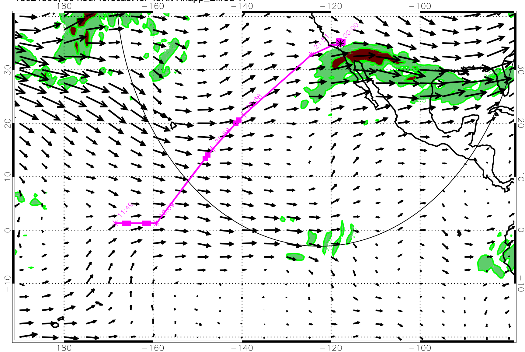
13021506, 66 hour forecast for 45Kft Knapp_Ellrod TI
