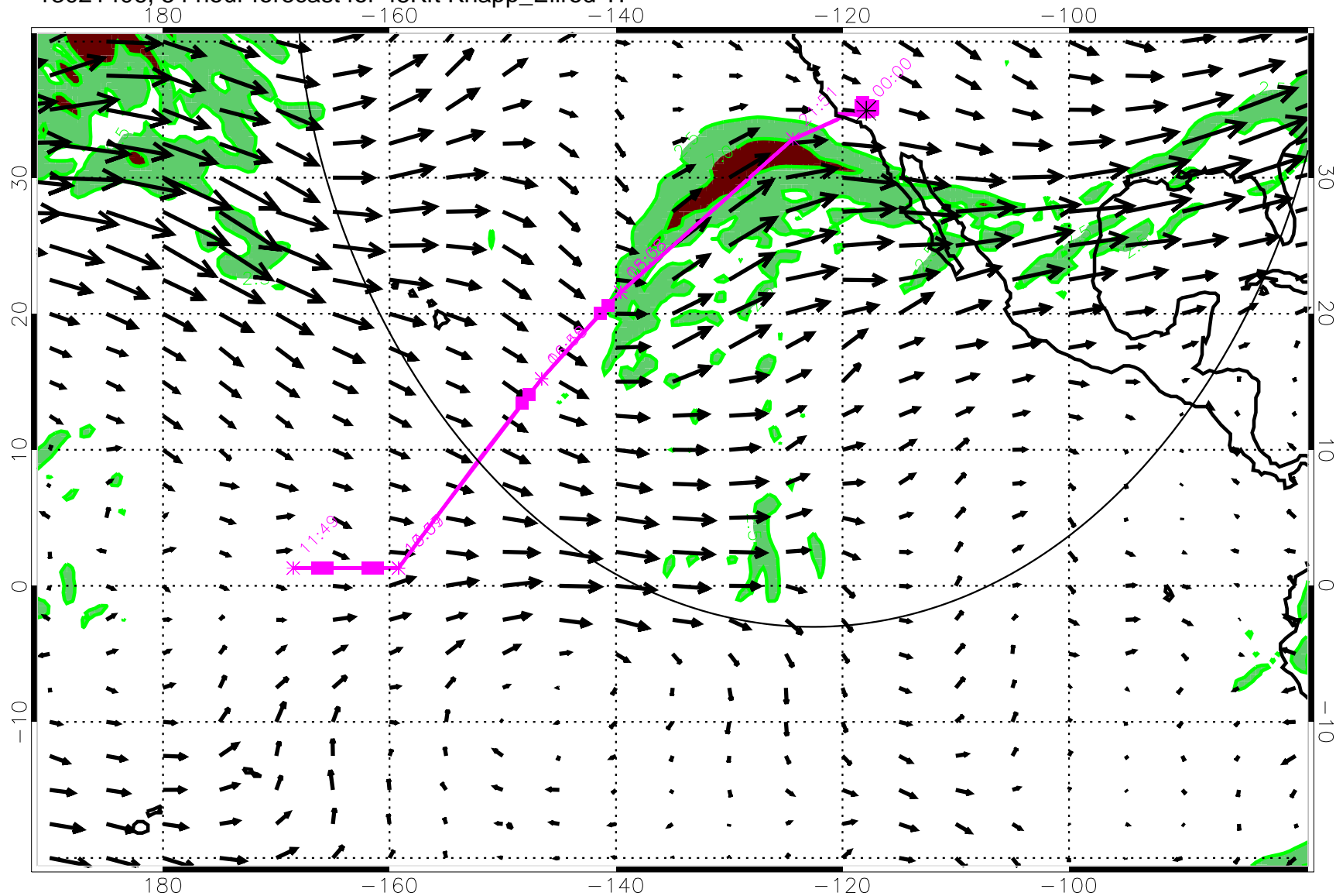
13021406, 54 hour forecast for 45Kft Knapp_Ellrod TI
