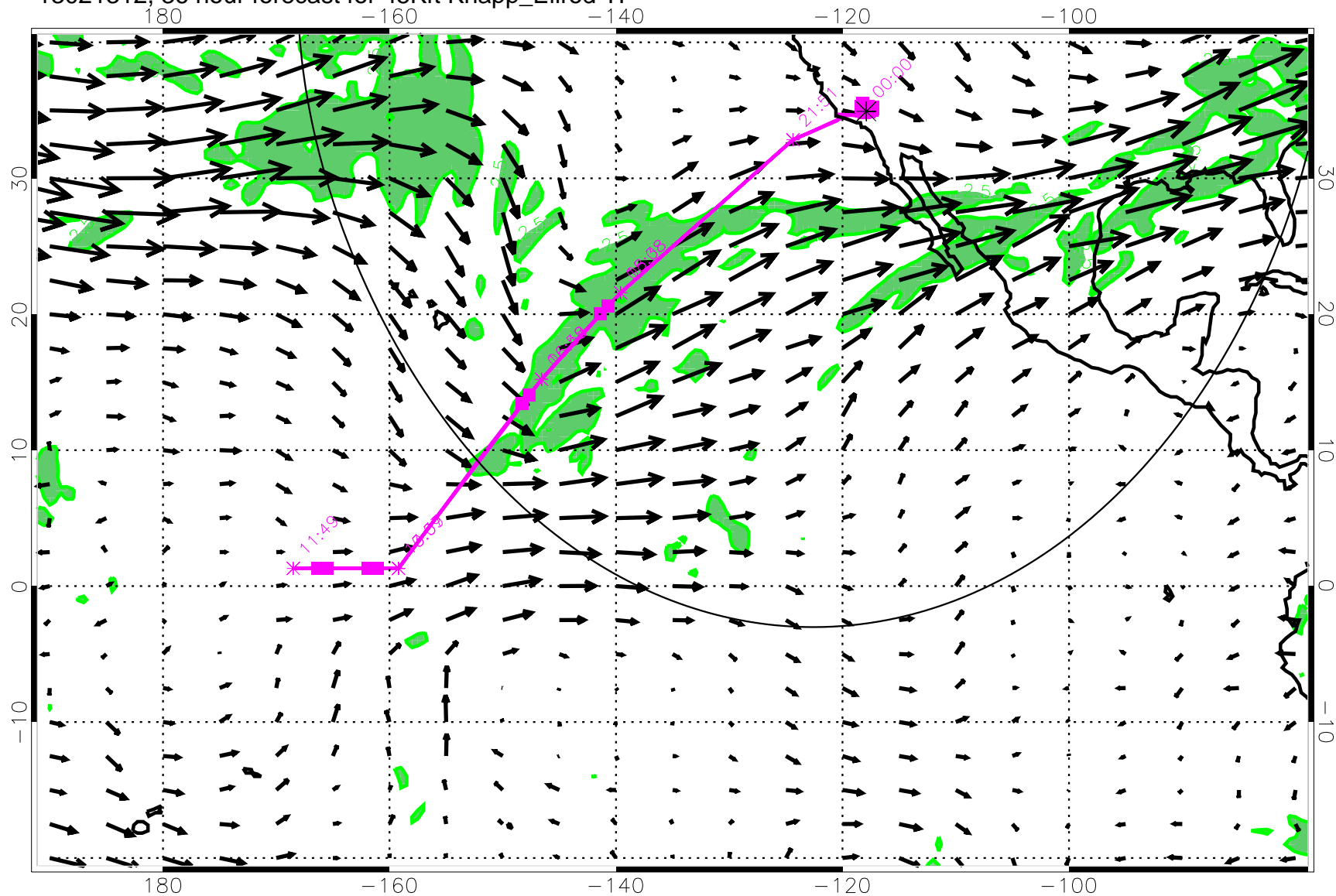
13021312, 36 hour forecast for 45Kft Knapp_Ellrod TI
