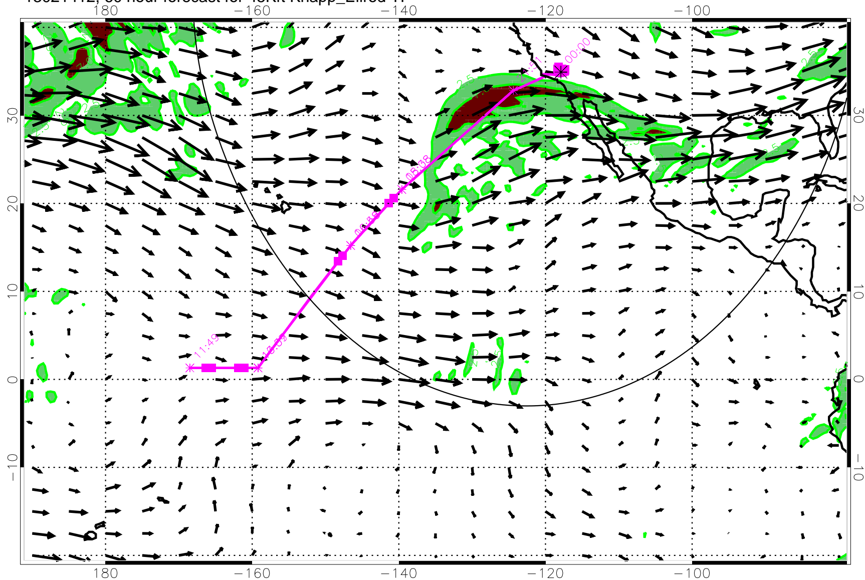
13021412, 60 hour forecast for 45Kft Knapp_Ellrod TI
