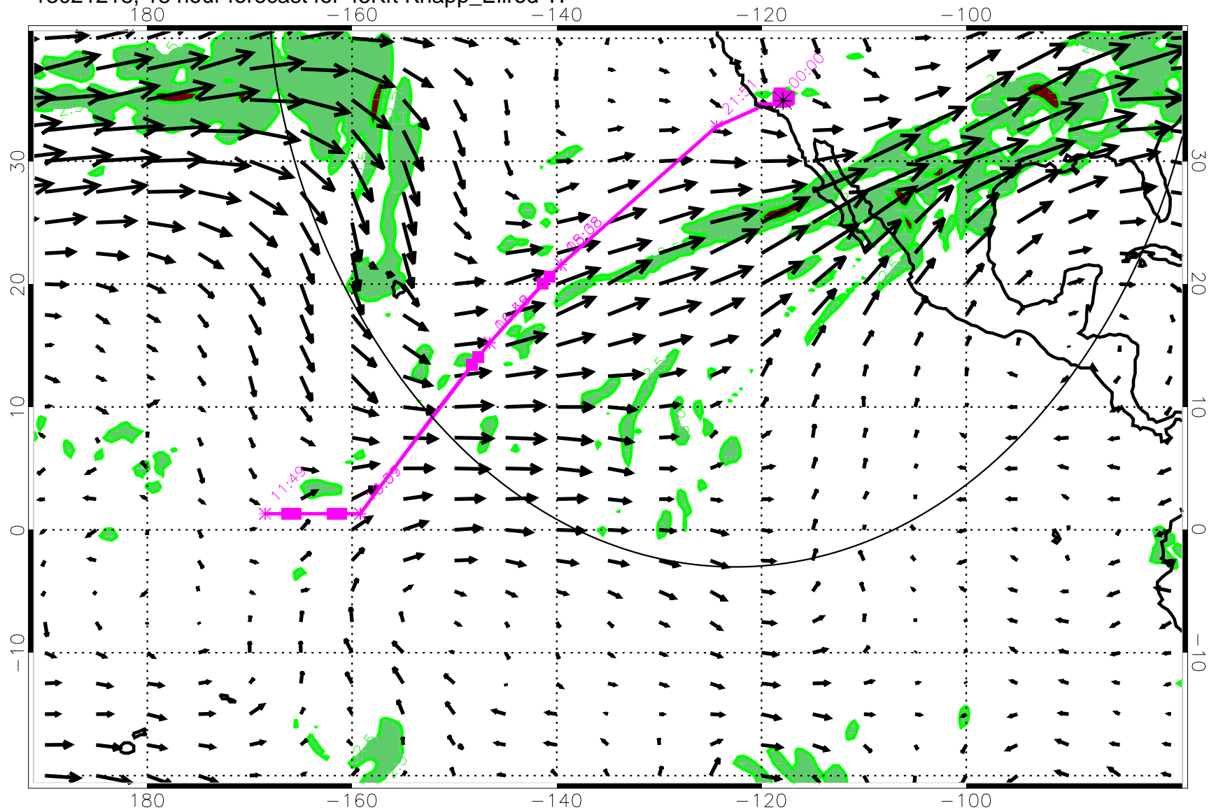
13021218, 18 hour forecast for 45Kft Knapp_Ellrod TI
