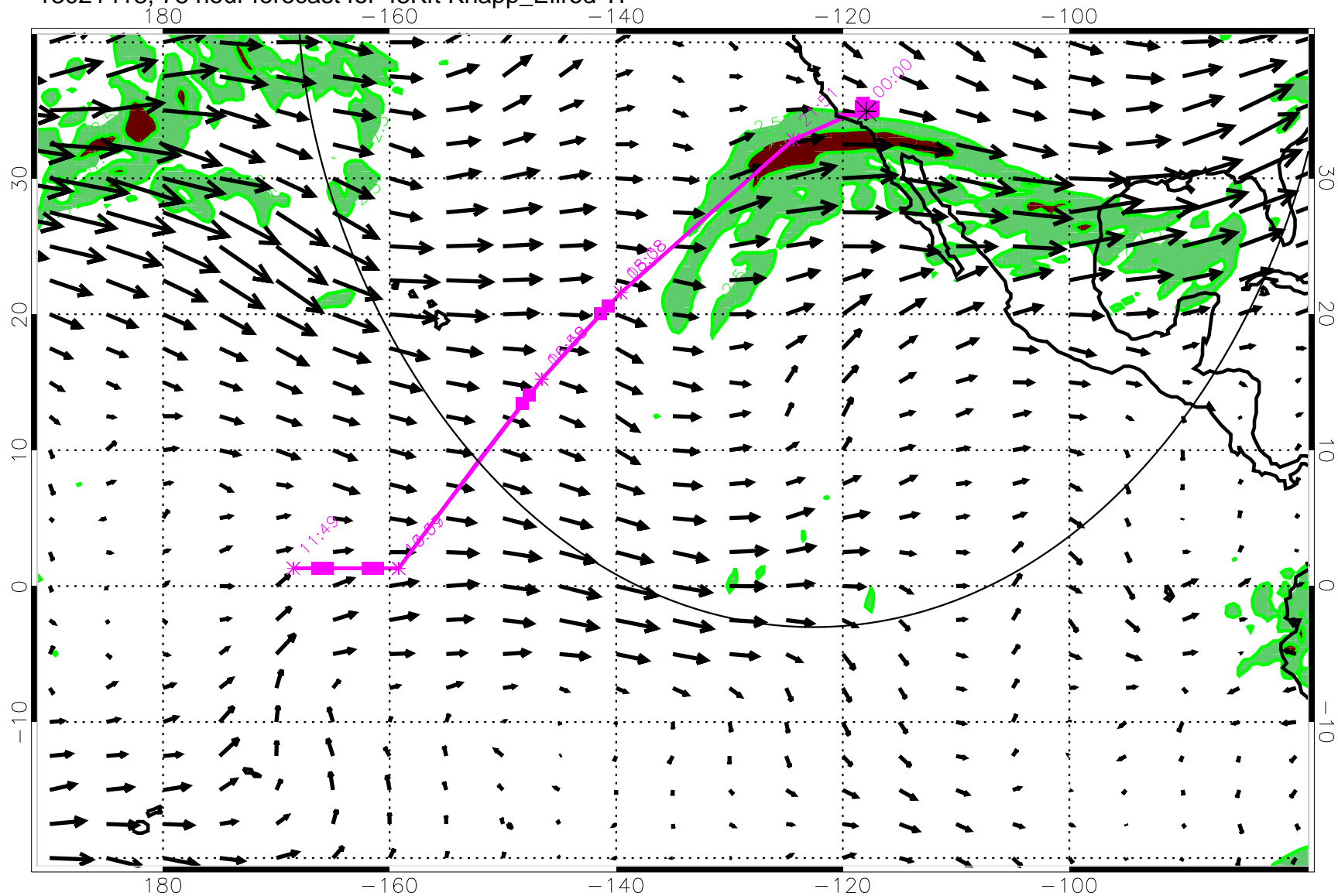
13021418, 78 hour forecast for 45Kft Knapp_Ellrod TI
