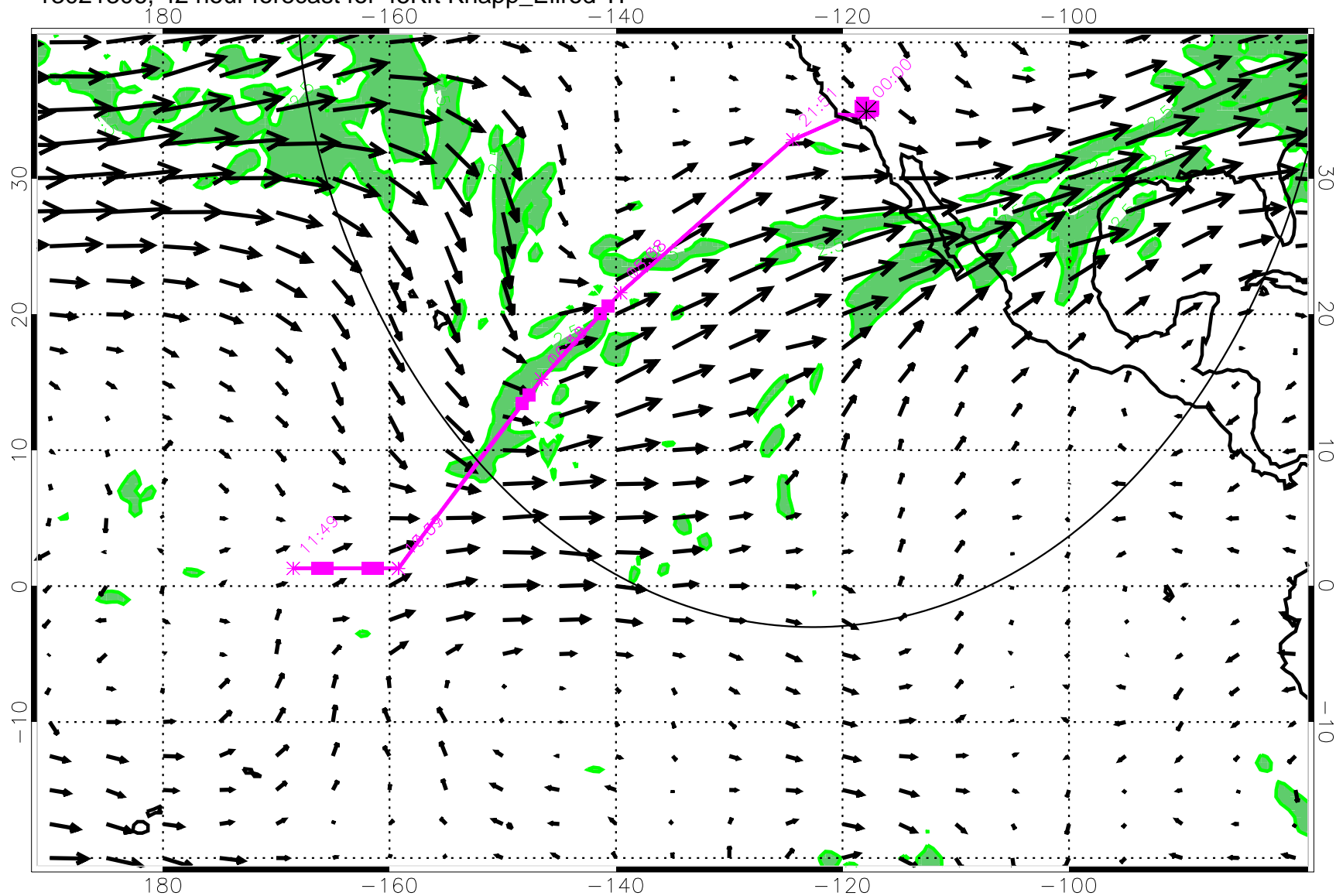
13021306, 42 hour forecast for 45Kft Knapp_Ellrod TI
