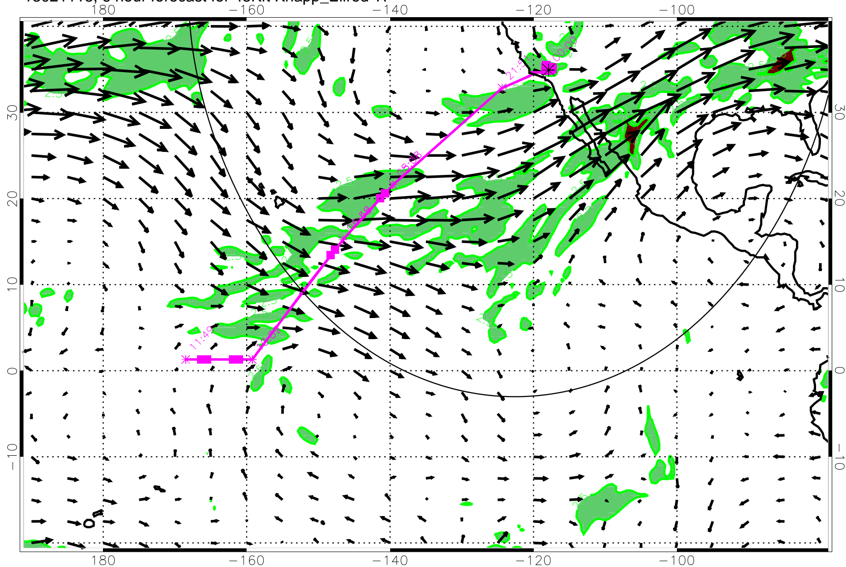
13021118, 6 hour forecast for 45Kft Knapp_Ellrod TI
