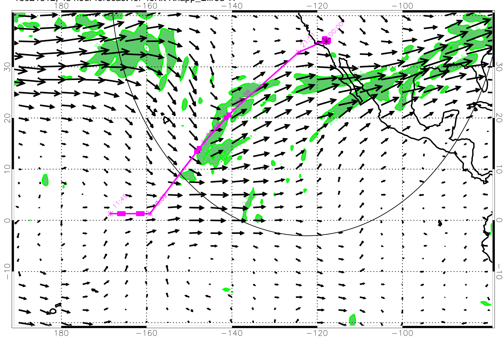
13021312, 48 hour forecast for 45Kft Knapp_Ellrod TI
