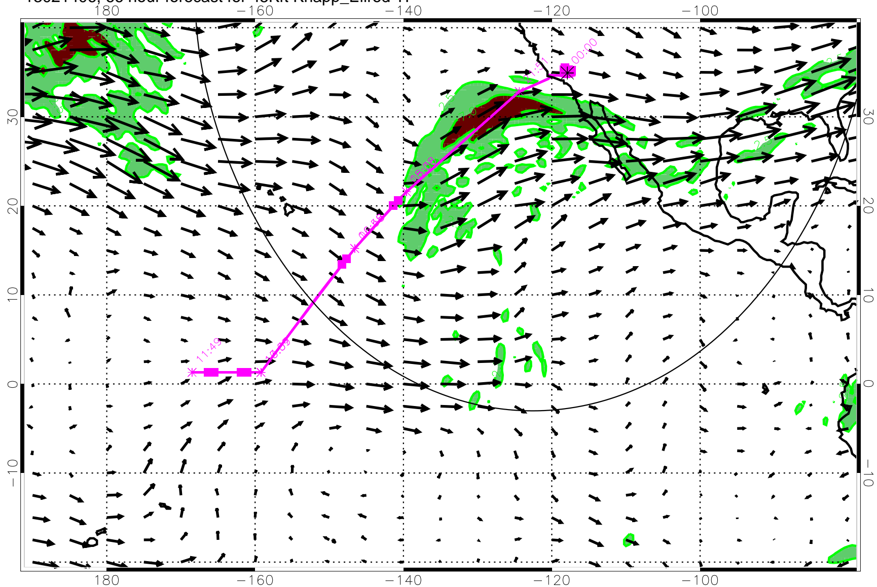
13021406, 66 hour forecast for 45Kft Knapp_Ellrod TI
