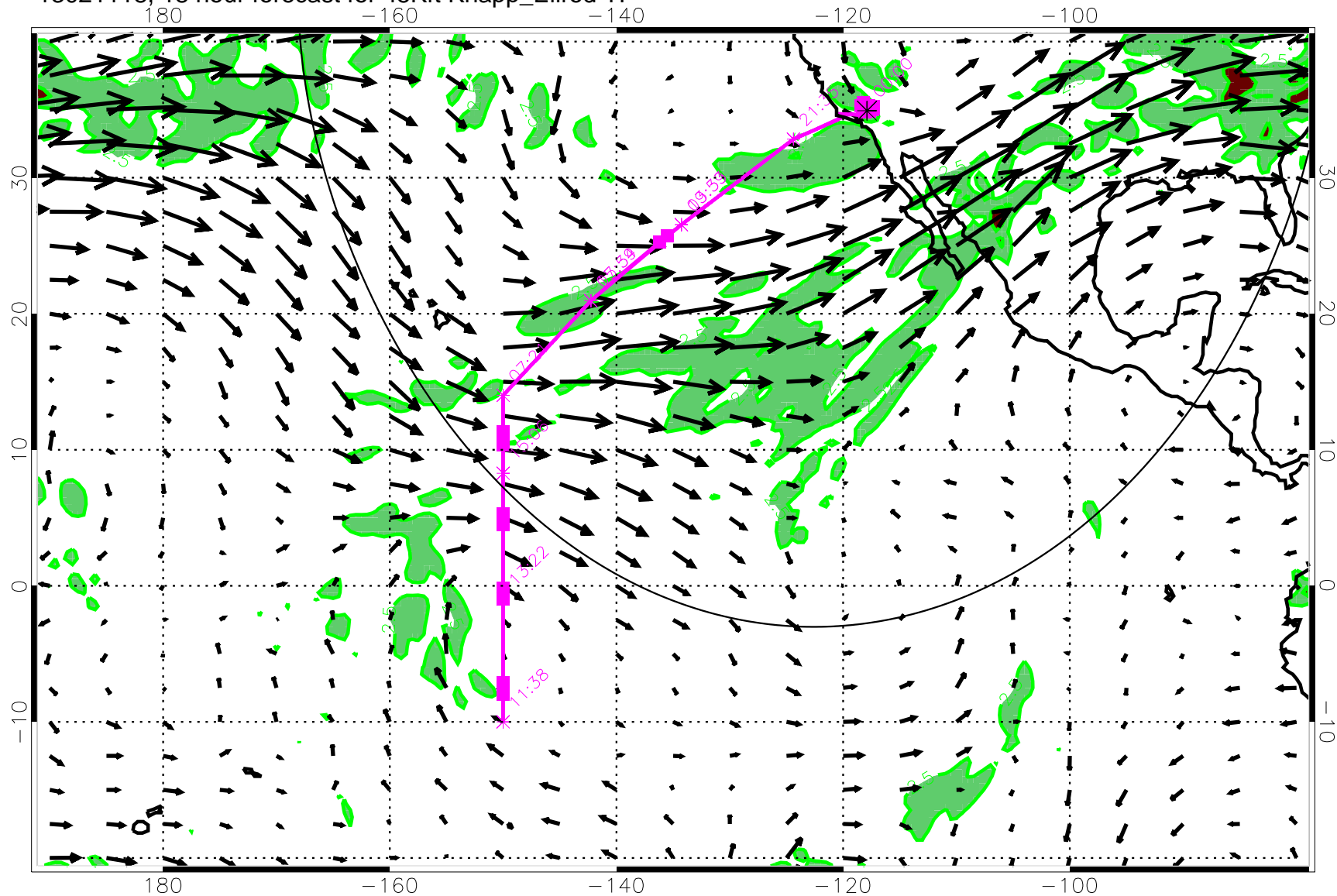
13021118, 18 hour forecast for 45Kft Knapp_Ellrod TI
