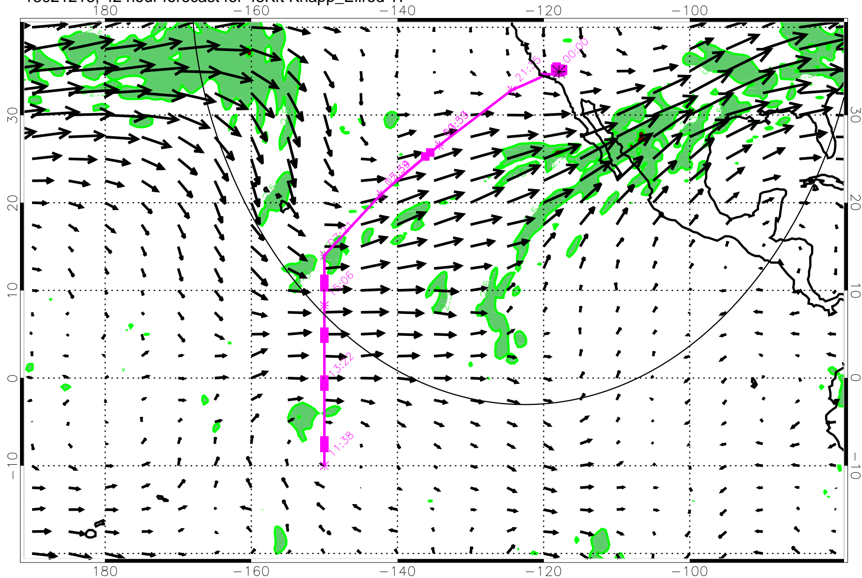
13021218, 42 hour forecast for 45Kft Knapp_Ellrod TI
