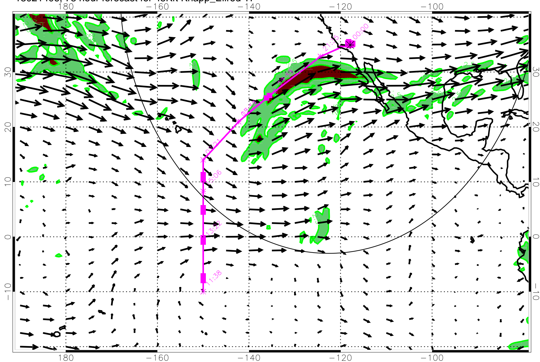
13021406, 78 hour forecast for 45Kft Knapp_Ellrod TI
