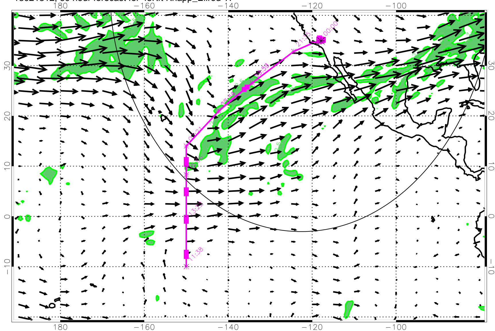
13021312, 60 hour forecast for 45Kft Knapp_Ellrod TI
