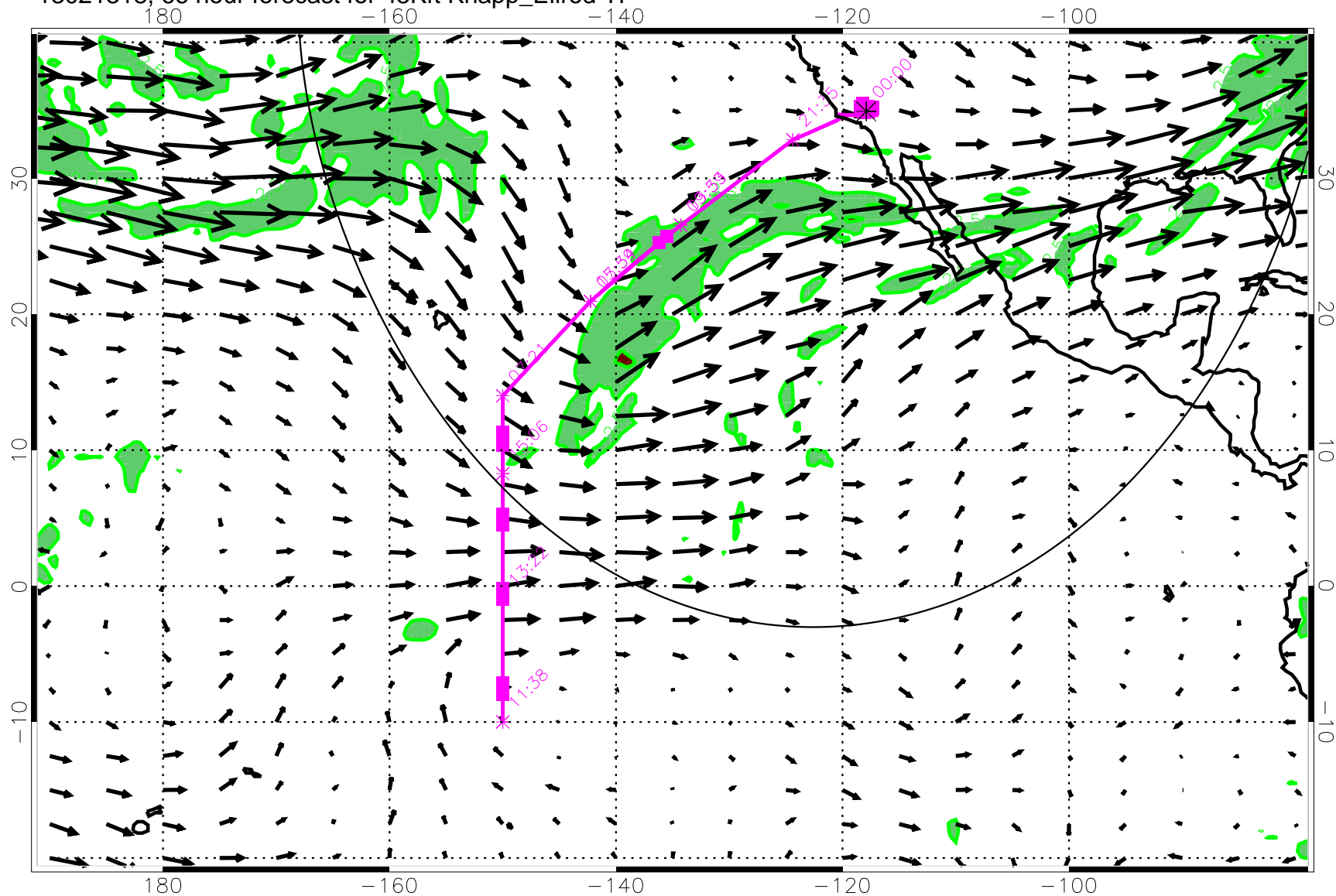
13021318, 66 hour forecast for 45Kft Knapp_Ellrod TI
