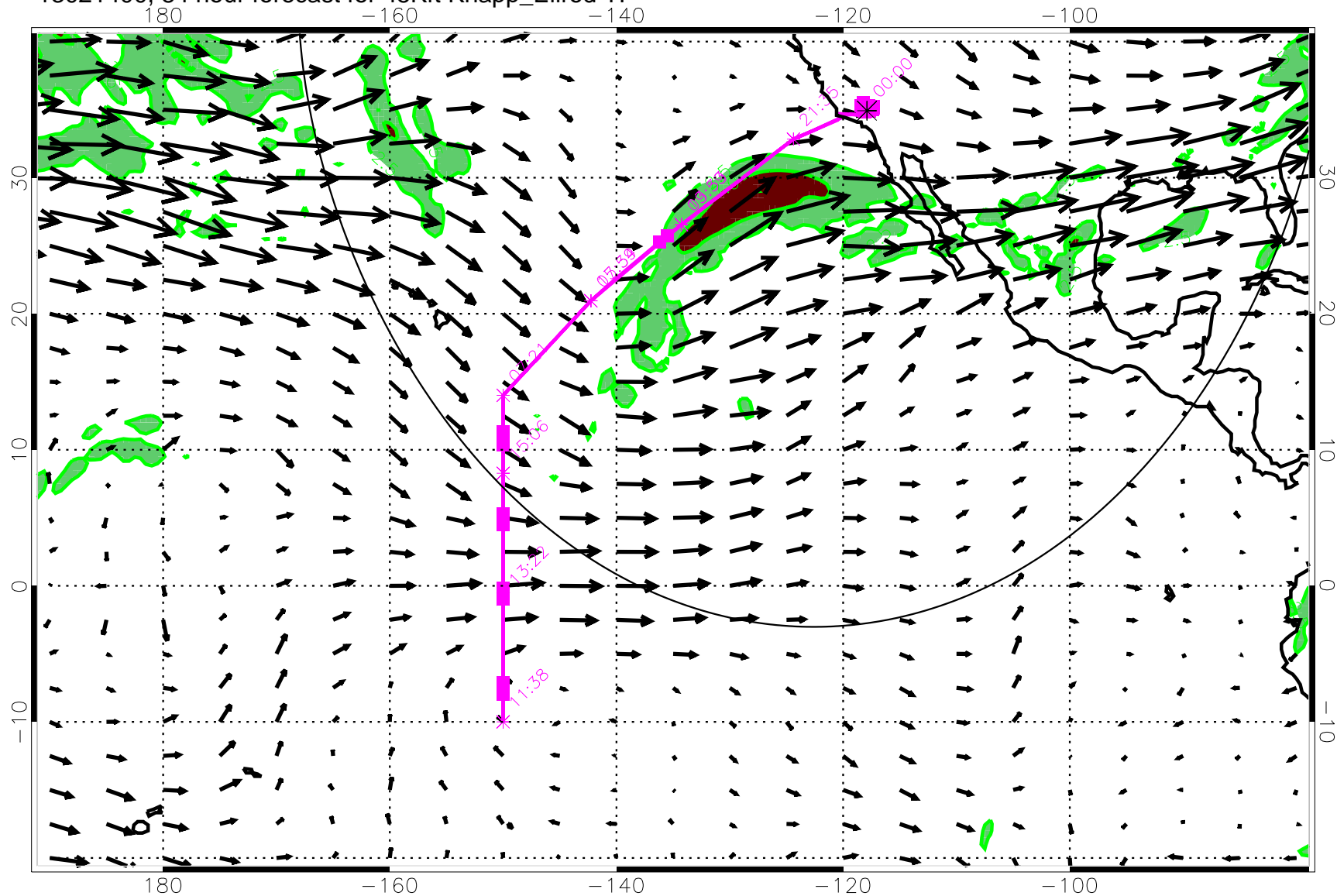
13021400, 84 hour forecast for 45Kft Knapp_Ellrod TI
