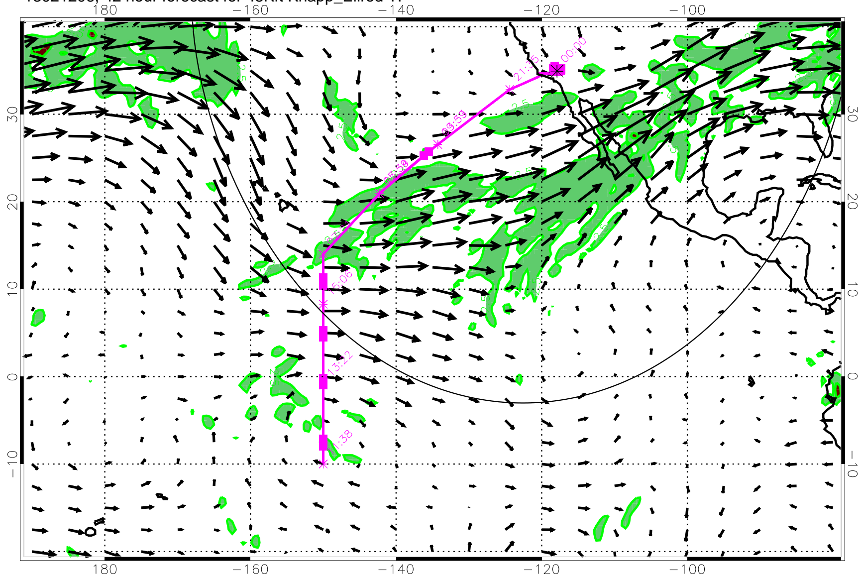
13021206, 42 hour forecast for 45Kft Knapp_Ellrod TI
