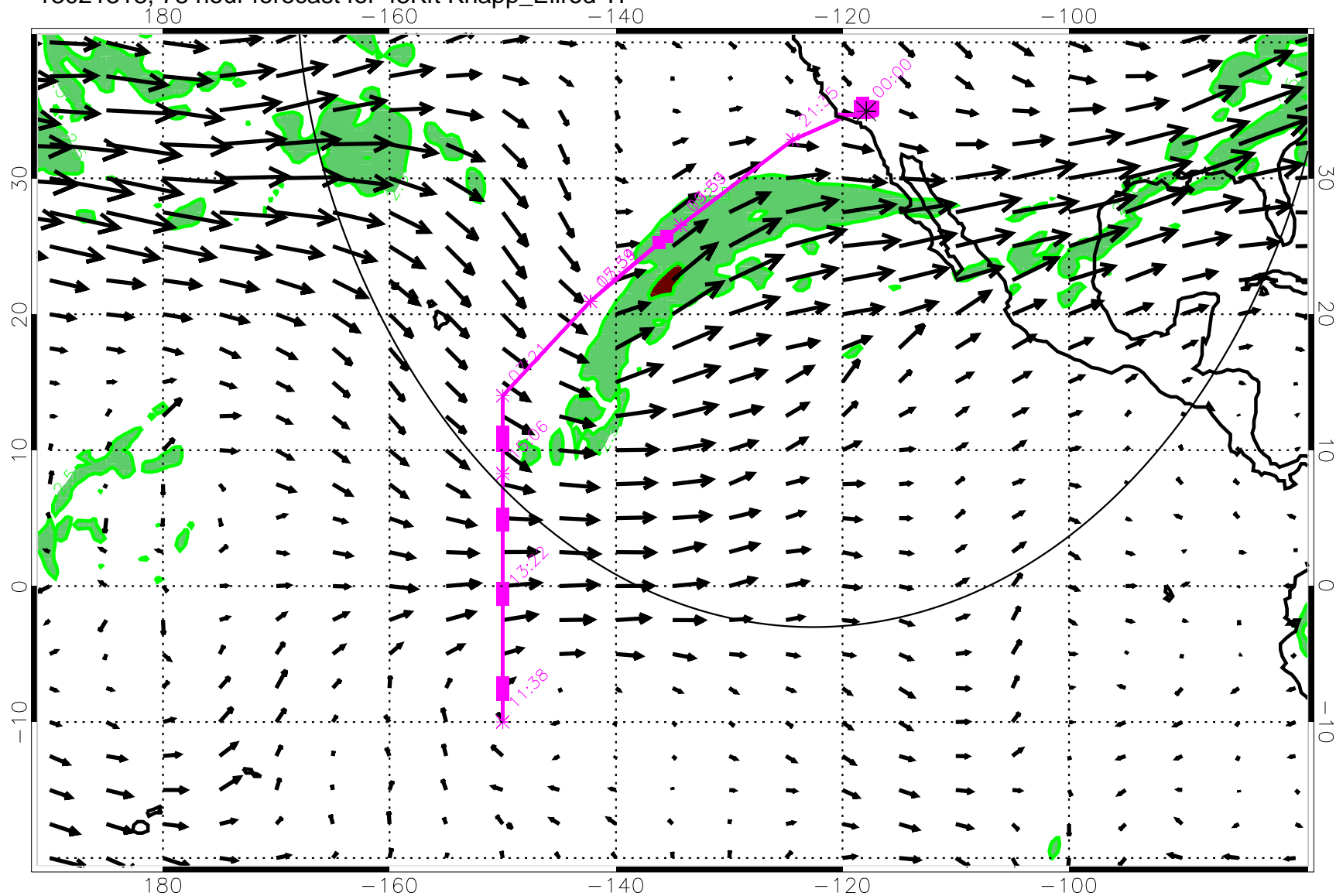
13021318, 78 hour forecast for 45Kft Knapp_Ellrod TI
