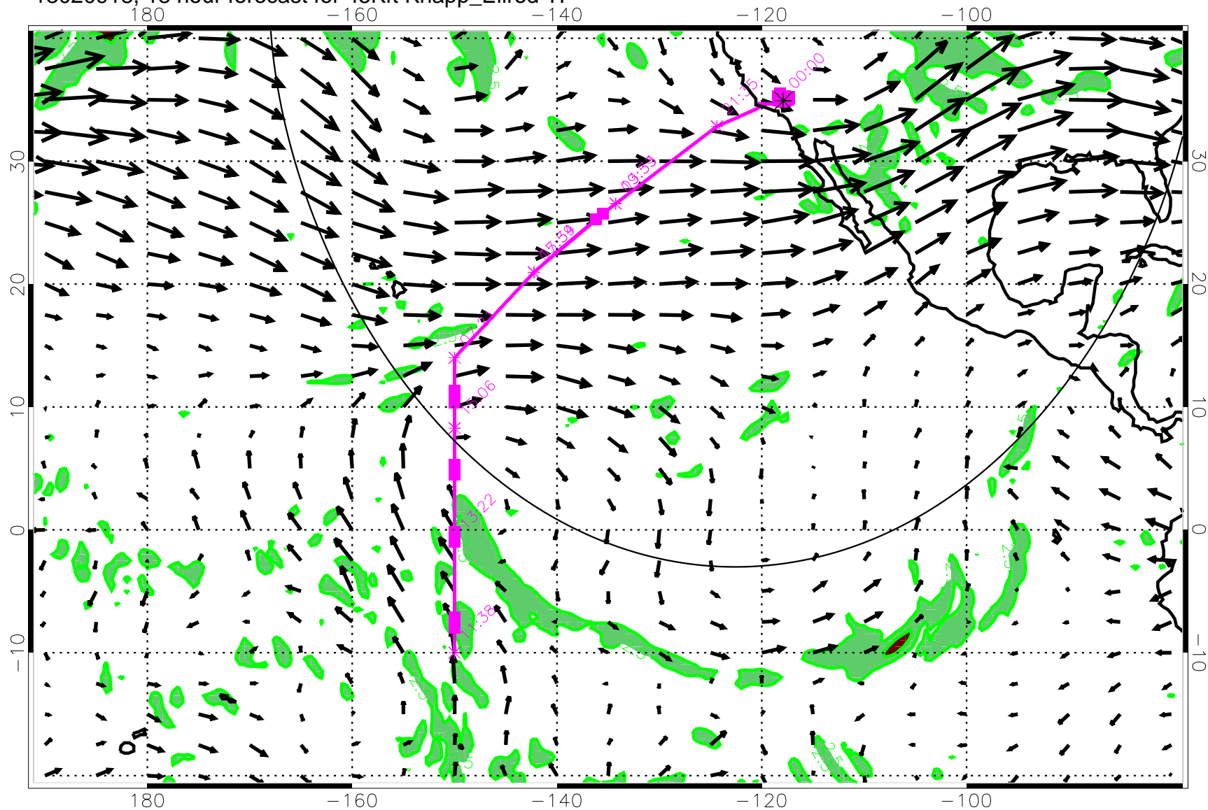
13020918, 18 hour forecast for 45Kft Knapp_Ellrod TI
