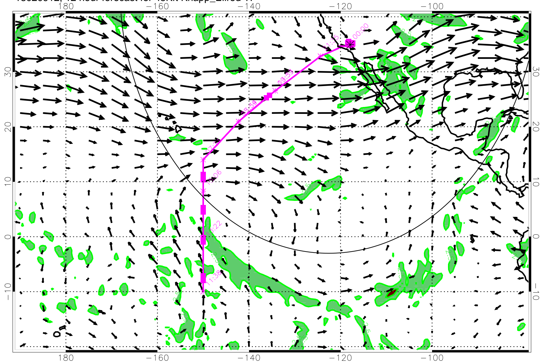
13020912, 12 hour forecast for 45Kft Knapp_Ellrod TI
