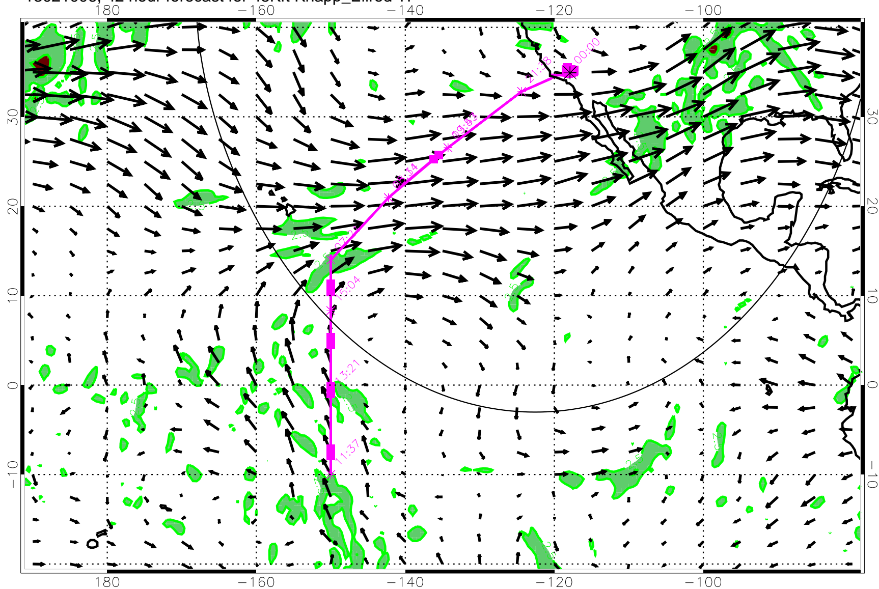
13021006, 42 hour forecast for 45Kft Knapp_Ellrod TI
