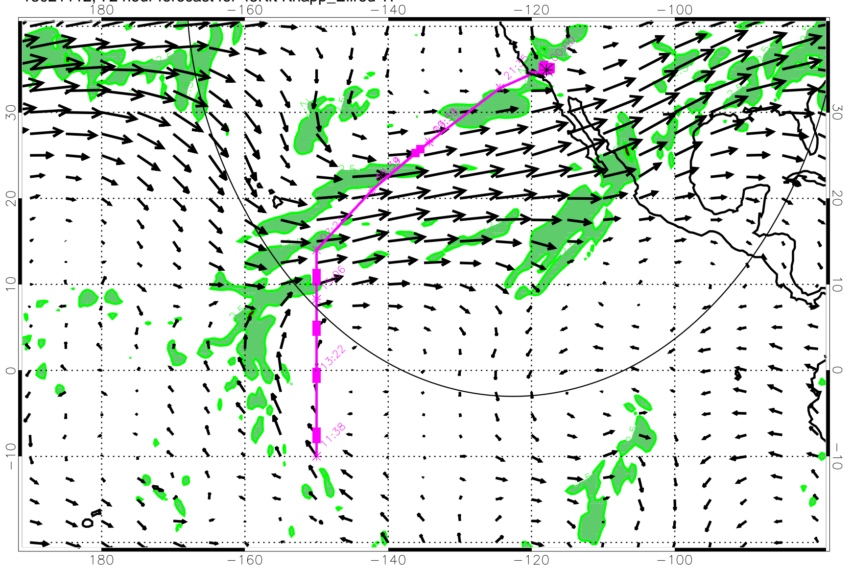
13021112, 72 hour forecast for 45Kft Knapp_Ellrod TI
